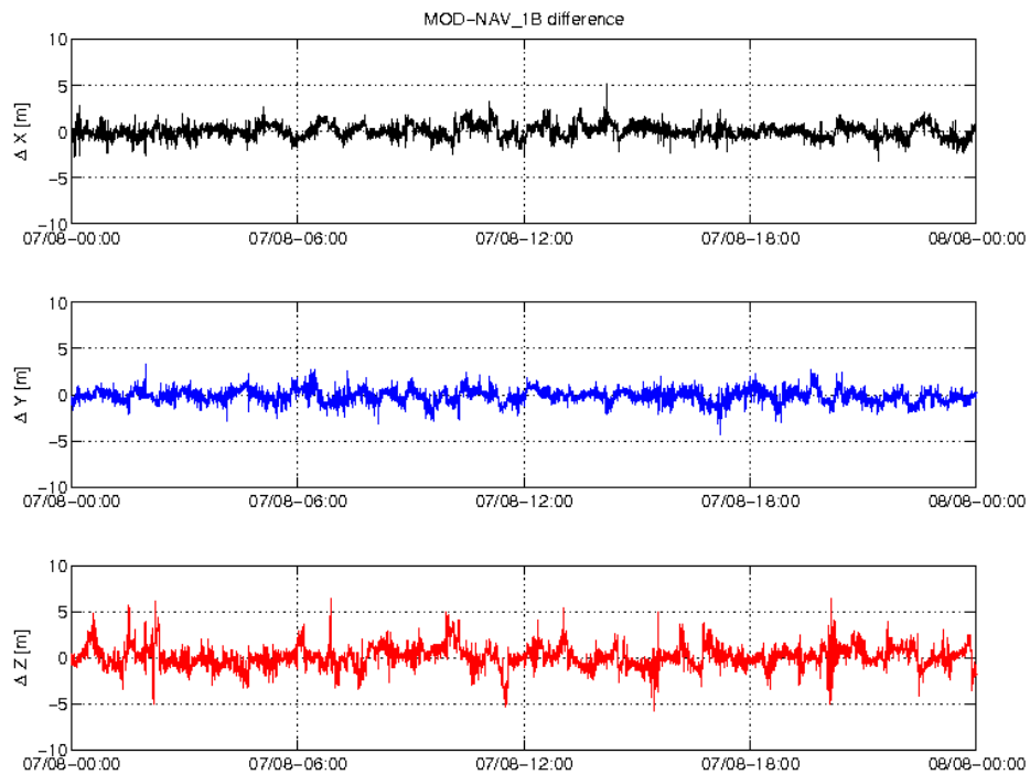
Figure 3-5: Difference MOD-GPSNAV, S/C C, 07/08. From top to bottom: X, Y and Z-axis
