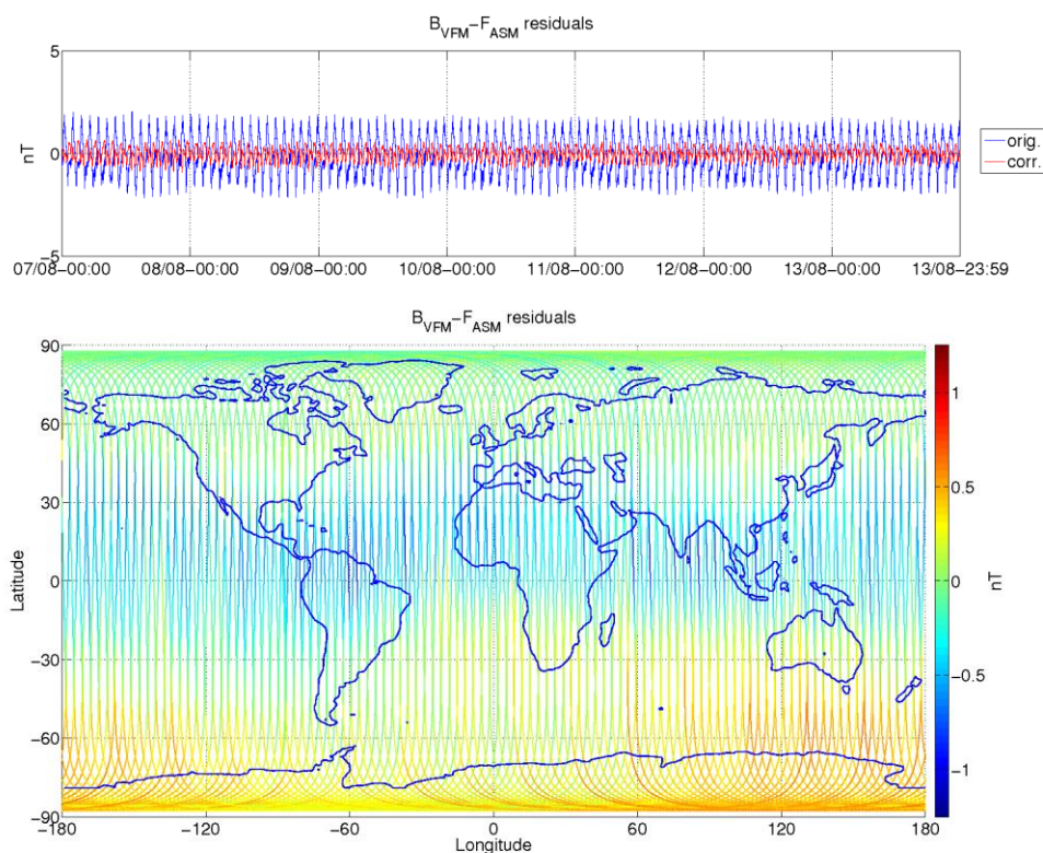
Figure 3-9: ASM-VFM residuals for S/C B, during monitoring period 07/08-13/08. In top figure are plotted: difference between |B_{VFM}| and F_{ASM} (without dB_{Sun} correction) (blue colour), and the residuals with dB_{Sun} corrections (red colour). In bottom figure residuals are presented on the world map.
