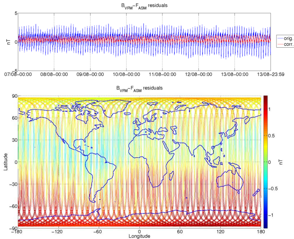
Figure 3-8: ASM-VFM residuals for S/C A, during monitoring period 07/08-13/08. In top figure are plotted: difference between |B VFM | and F ASM (without dB Sun correction) (blue colour), and the residuals with dB Sun corrections (red colour). In bottom figure residuals are presented on the world map.
