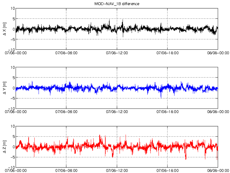
Figure 3-3: Difference MOD-GPSNAV, S/C A, 07/08. From top to bottom: X, Y and Z-axis
