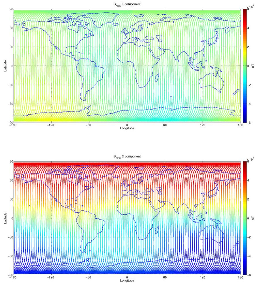
Figure 3-11: S/C B, world map plots of the geomagnetic field and components measured during monitoring period 07/08-13/08. From top to bottom: F-magnetic field from ASM measurement, B_{NEC} components (North, East, and Centre) of magnetic field from VFM measurement.
