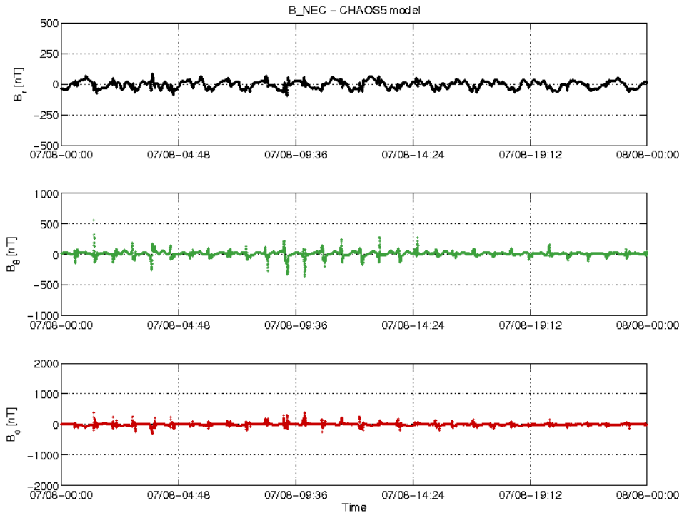
Figure 3-22: S/C C day 07/08 time series of B_{NEC} - B_{Chaos} residuals.
