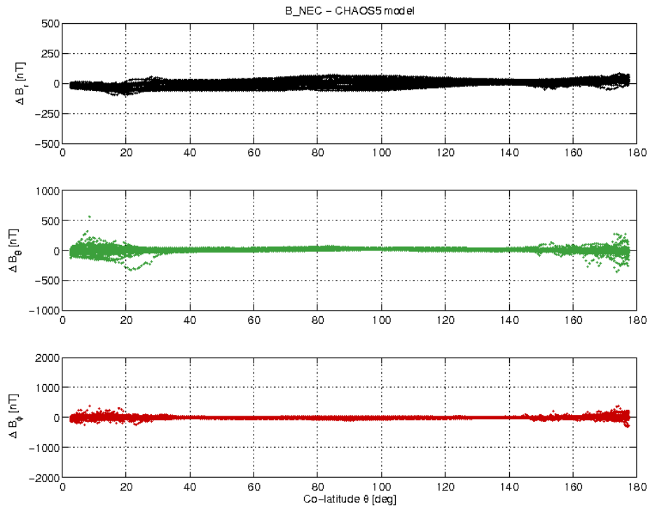
Figure 3-21: S/C C day 07/08 B_{NEC} - B_{Chaos} difference vs colatitude.
