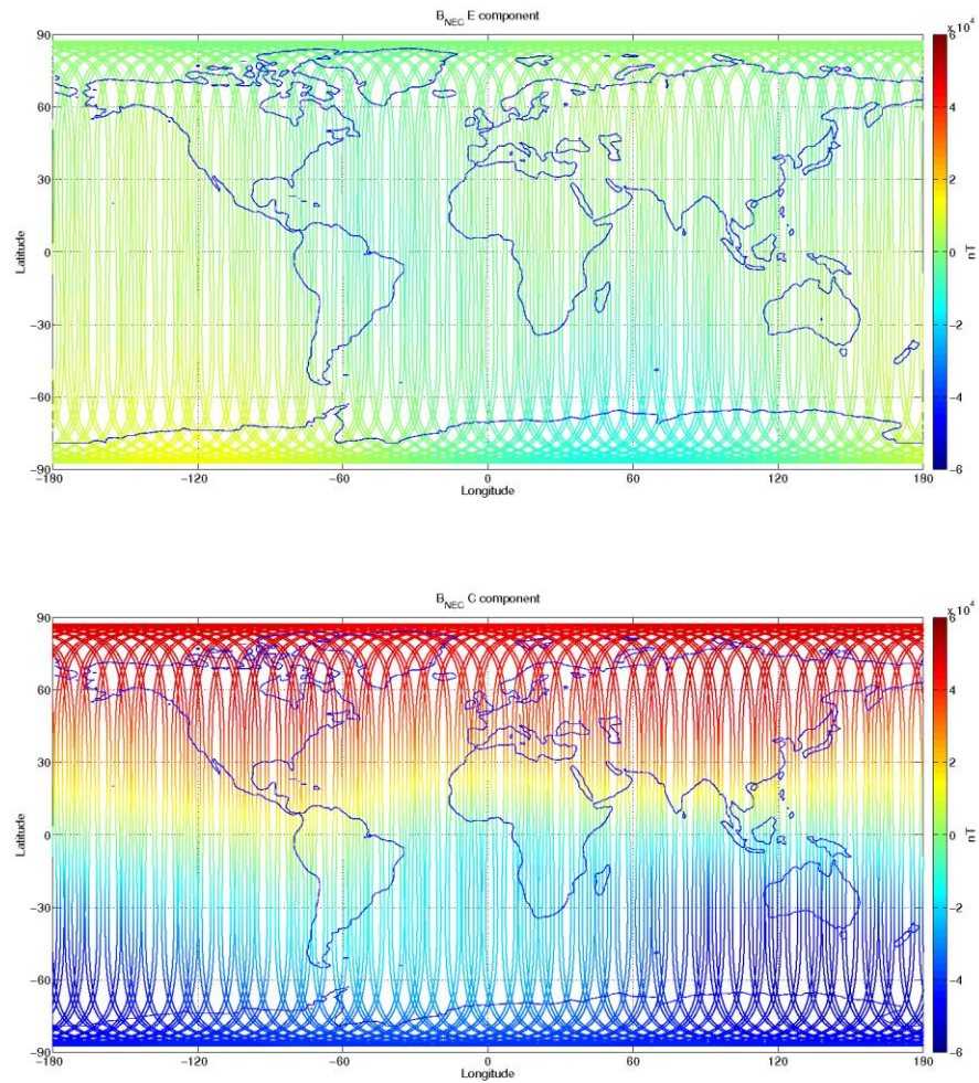
Figure 3-10: S/C A, world map plots of the geomagnetic field and components measured during monitoring period 07/08-13/08. From top to bottom: F-magnetic field from ASM measurement, B_{NEC} components (North, East, and Centre) of magnetic field from VFM measurement.
