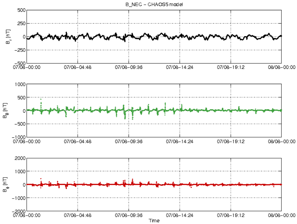
Figure 3-18: S/C A day 07/08: time series of B_{NEC} - B_{Chaos} residuals.
