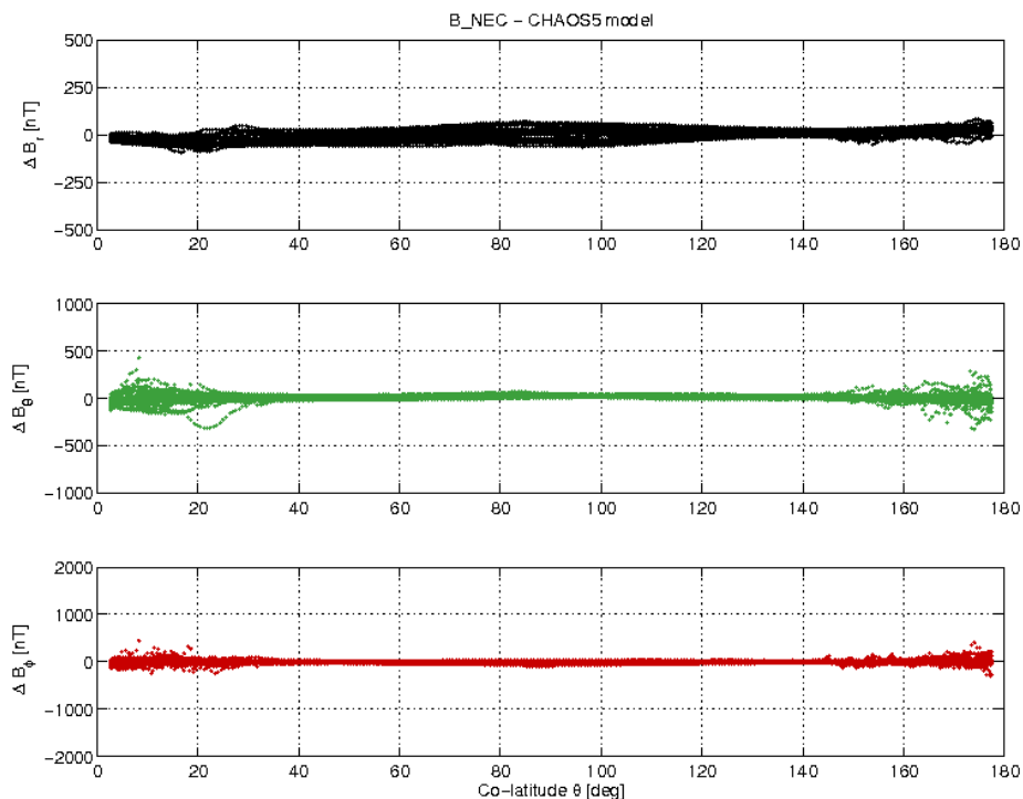
Figure 3-17: S/C A day 07/08 B_{NEC} - B_{Chaos} vs colatitude.
