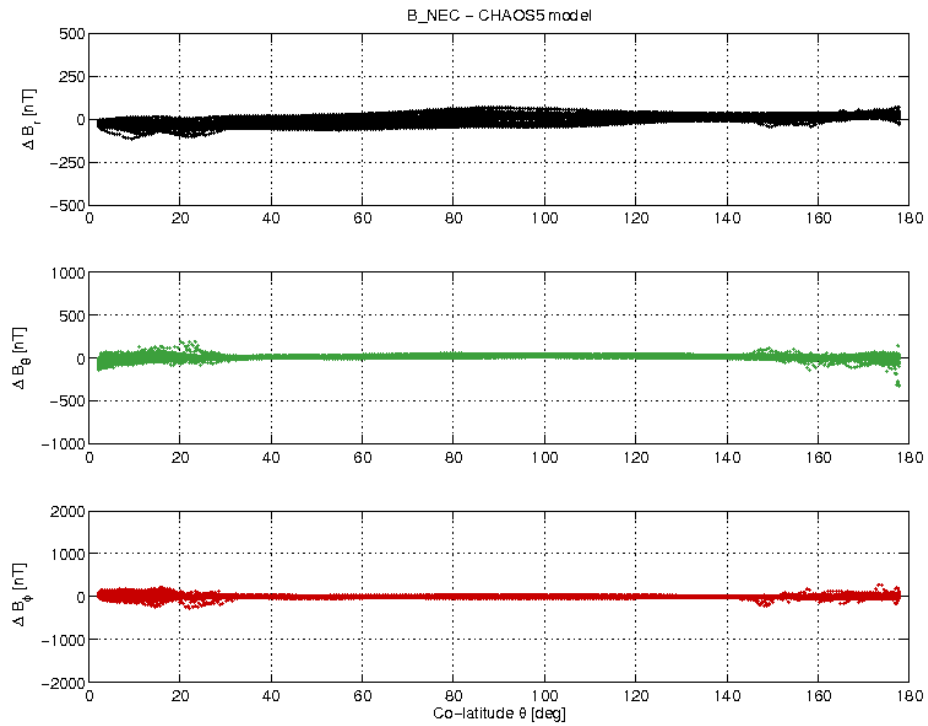
Figure 3-19: S/C B day 07/08 B_{NEC} - B_{Chaos} difference vs colatitude.
