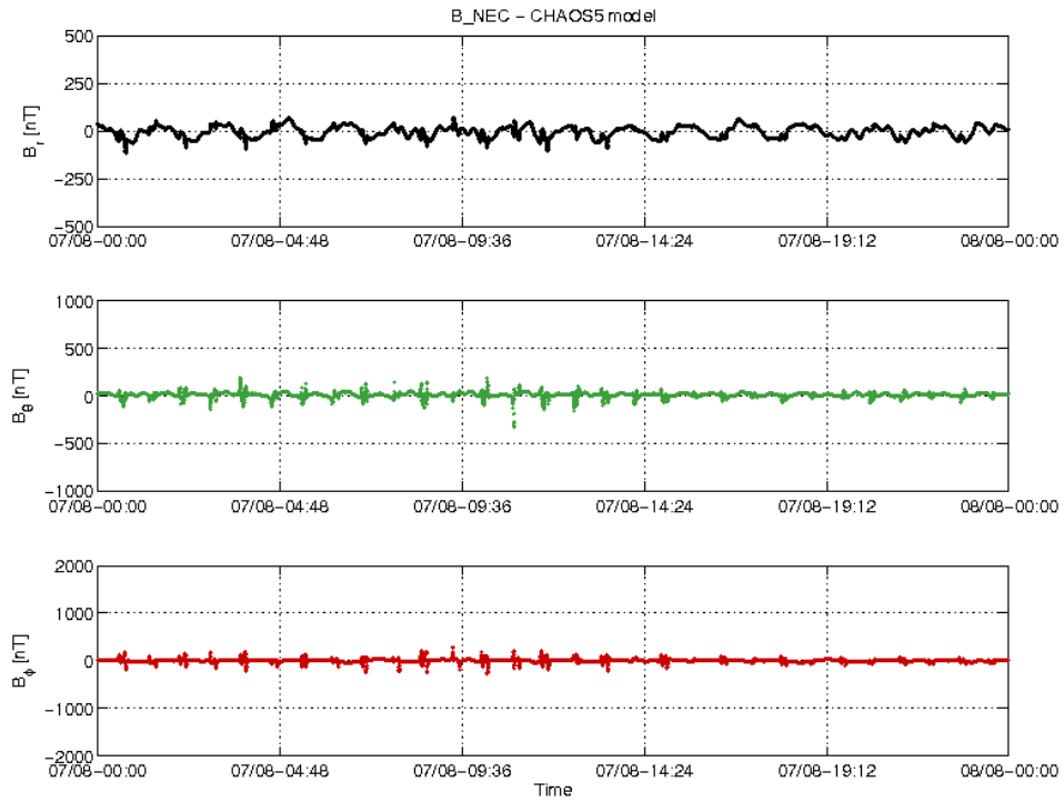
Figure 3-20: S/C B day 07/08 time series of B_{NEC} - B_{Chaos} residuals.
