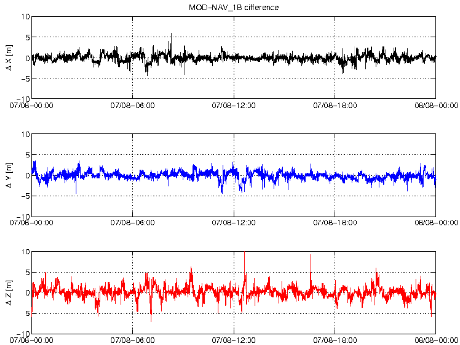
Figure 3-4: Difference MOD-GPSNAV, S/C B, 07/08. From top to bottom: X, Y and Z-axis
