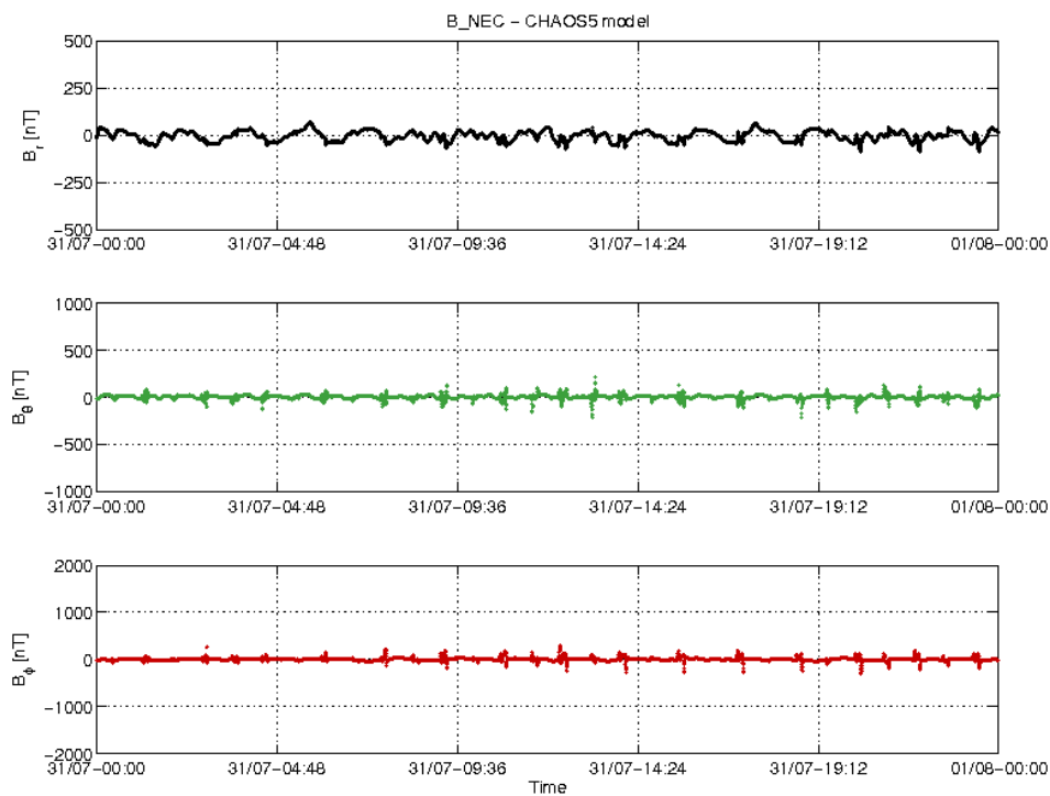
Figure 3-20: S/C B day 31/07 time series of B_{NEC} - B_{Chaos} residuals.
