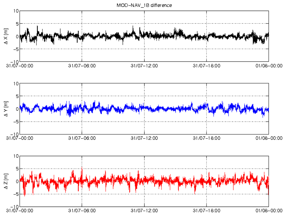
Figure 3-5: Difference MOD-GPSNAV, S/C C, 31/07. From top to bottom: X, Y and Z-axis
