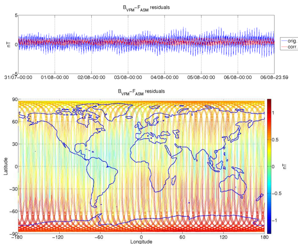
Figure 3-8: ASM-VFM residuals for S/C A, during monitoring period 31/07-06/08. In top figure are plotted: difference between |B_{VFM}| and F_{ASM} (without dB_Sun correction) (blue colour), and the residuals with dB_Sun corrections (red colour). In bottom figure residuals are presented on the world map.
