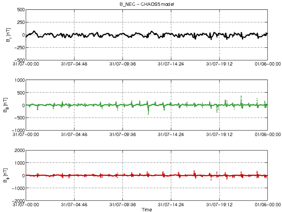
Figure 3-22: S/C C day 31/07 time series of B_{NEC} - B_{Chaos} residuals.
