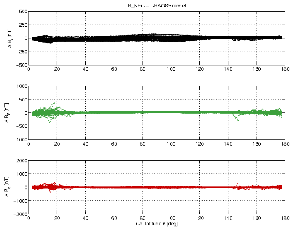
Figure 3-21: S/C C day 31/07 B_{NEC} - B_{Chaos} difference vs colatitude.
