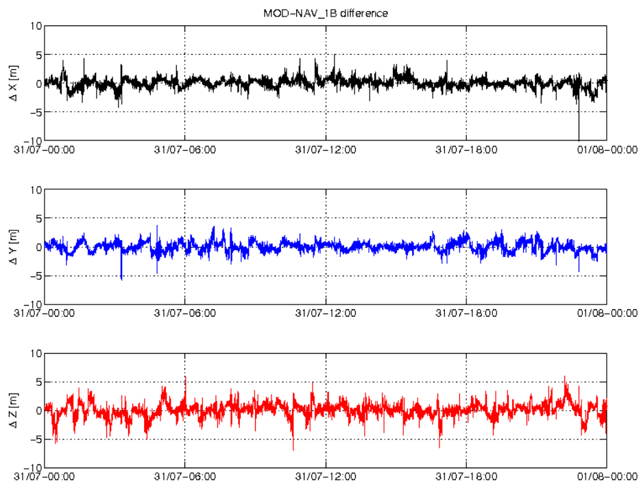
Figure 3-3: Difference MOD-GPSNAV, S/C A, 31/07. From top to bottom: X, Y and Z-axis
