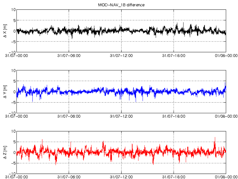
Figure 3-4: Difference MOD-GPSNAV, S/C B, 31/07. From top to bottom: X, Y and Z-axis
