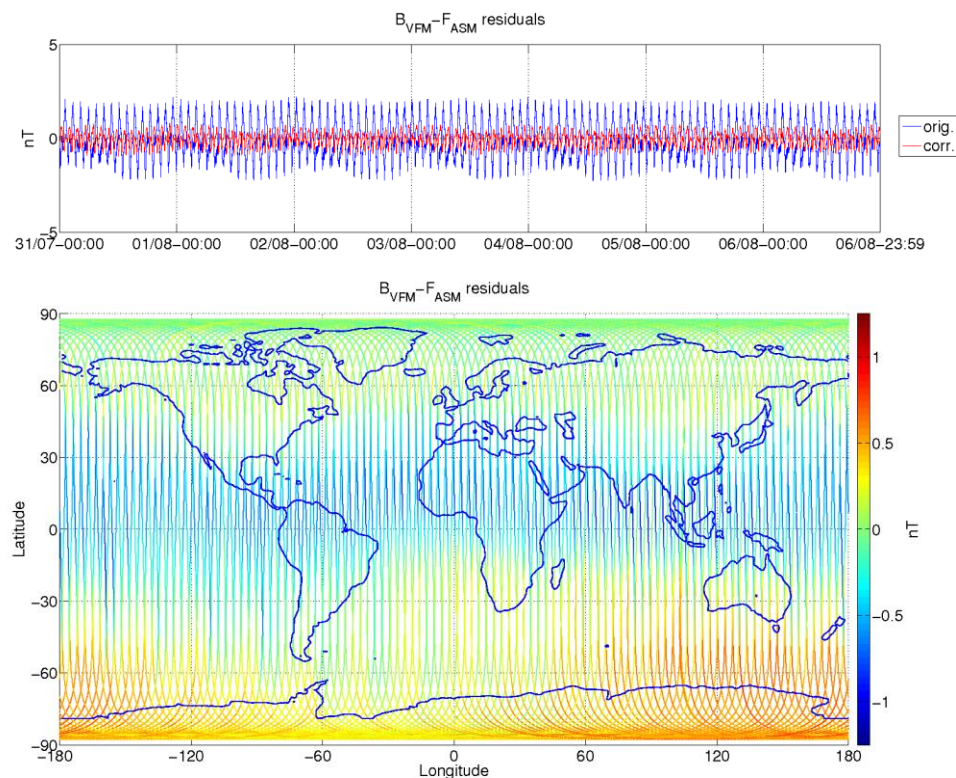
Figure 3-9: ASM-VFM residuals for S/C B, during monitoring period 31/07-06/08. In top figure are plotted: difference between |B_{VFM}| and F_{ASM} (without dB_{Sun} correction) (blue colour), and the residuals with dB_{Sun} corrections (red colour). In bottom figure residuals are presented on the world map.
