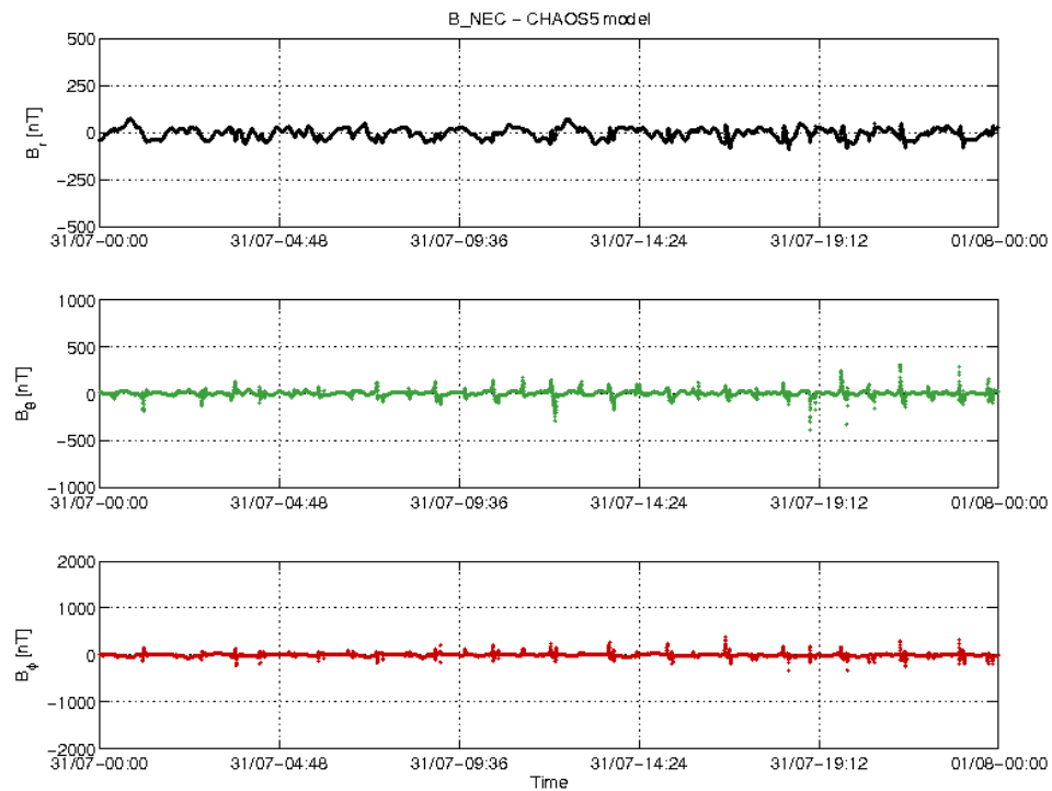
Figure 3-18: S/C A day 31/07: time series of B_{NEC} - B_{Chaos} residuals.
