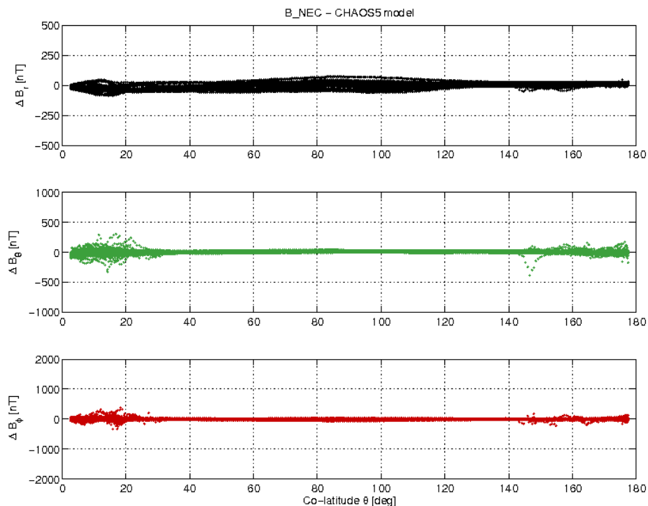
Figure 3-17: S/C A day 31/07 B_{NEC} - B_{Chaos} vs colatitude.
