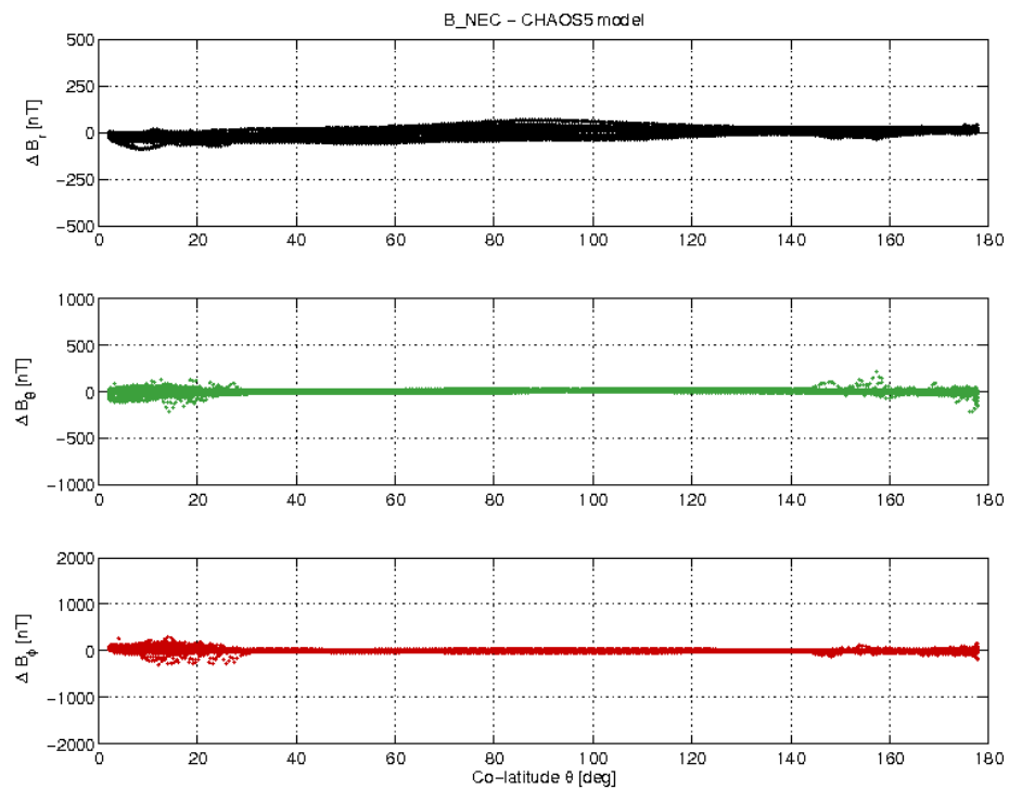
Figure 3-19: S/C B day 31/07 B_{\text{NEC}} - B_{\text{Chaos}} difference vs colatitude.
