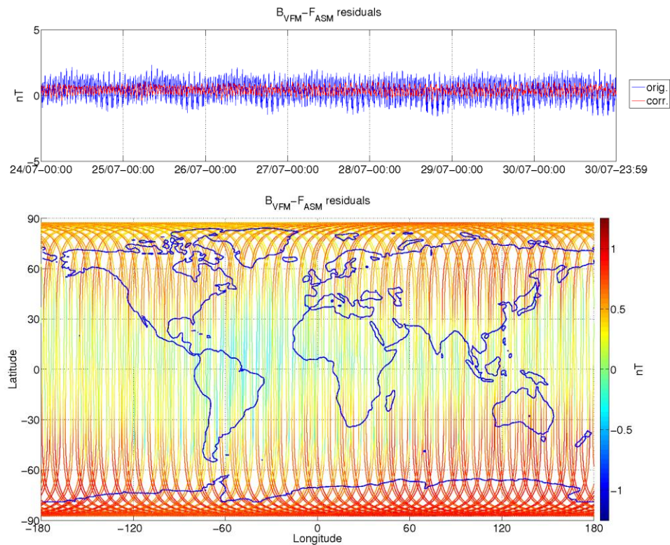
Figure 3-8: ASM-VFM residuals for S/C A, during monitoring period 24/07-30/07. In top figure are plotted: difference between |B VFM | and F ASM (without dB Sun correction) (blue colour), and the residuals with dB Sun corrections (red colour). In bottom figure residuals are presented on the world map.
