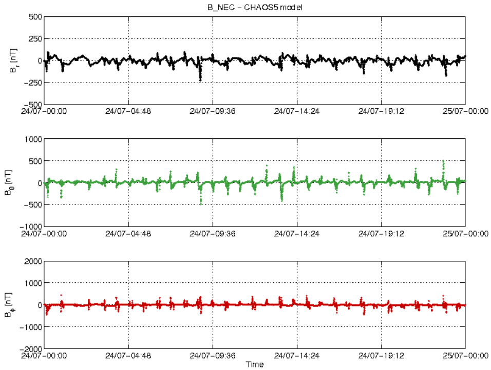
Figure 3-18: S/C A day 24/07: time series of B_{NEC} - B_{Chaos} residuals.
