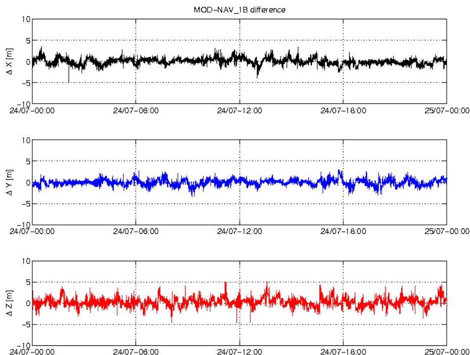
Figure 3-5: Difference MOD-GPSNAV, S/C C, 24/07. From top to bottom: X, Y and Z-axis
