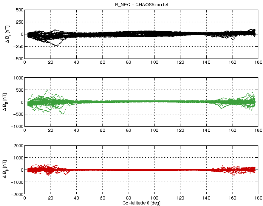
Figure 3-17: S/C A day 24/07 B_{NEC} - B_{Chaos} vs colatitude.
