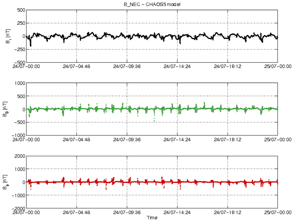
Figure 3-20: S/C B day 24/07 time series of B_{NEC} - B_{Chaos} residuals.
