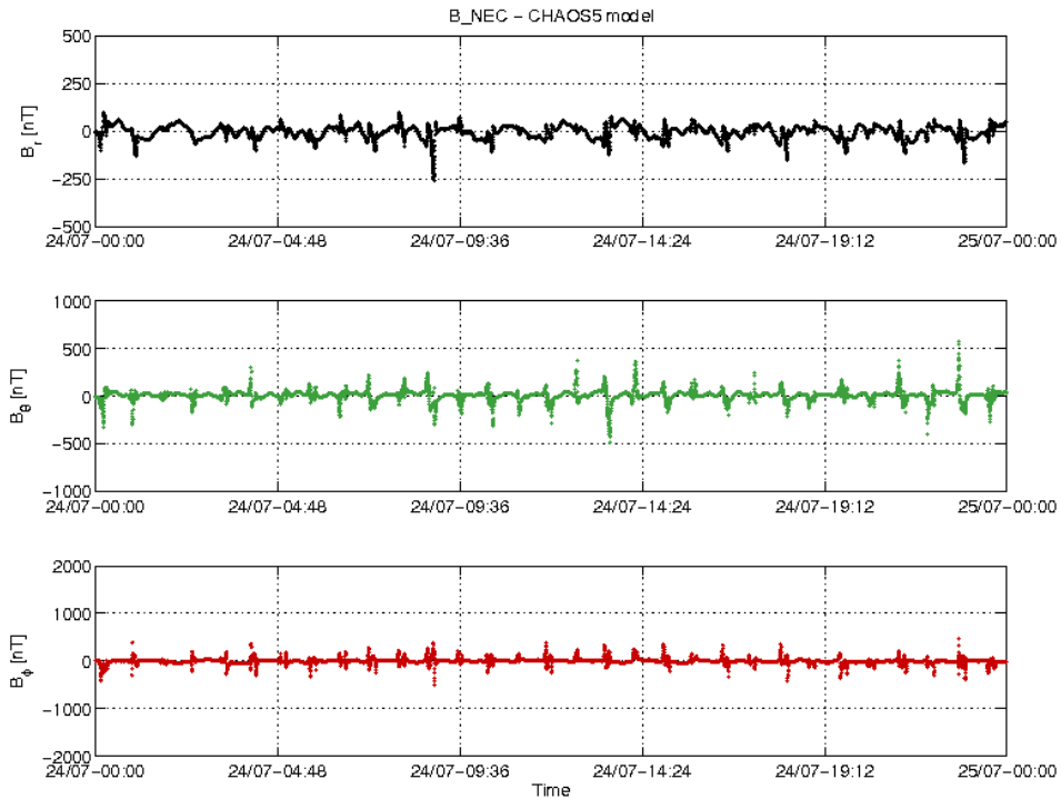
Figure 3-22: S/C C day 24/07 time series of B_{NEC} - B_{Chaos} residuals.
