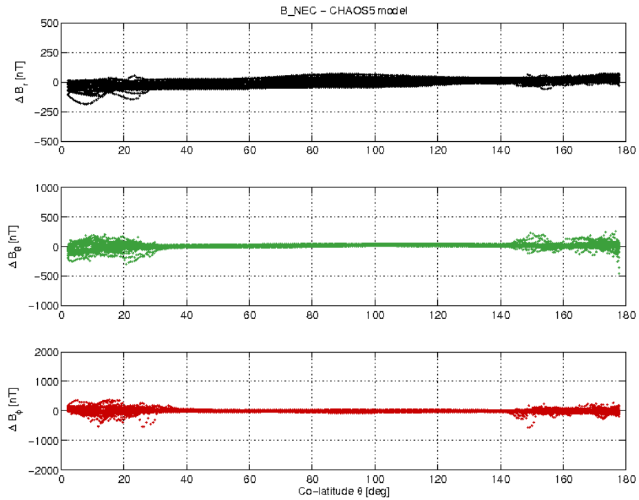
Figure 3-19: S/C B day 24/07 B_{NEC} - B_{Chaos} difference vs colatitude.
