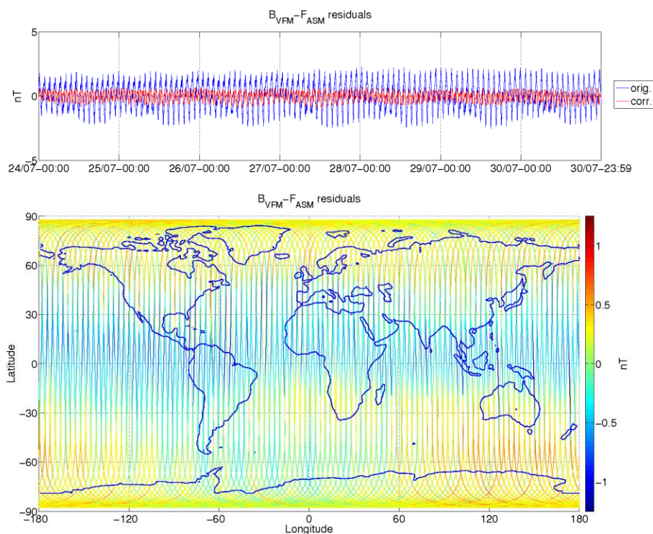
Figure 3-9: ASM-VFM residuals for S/C B, during monitoring period 24/07-30/07. In top figure are plotted: difference between |B_{VFM}| and F_{ASM} (without dB_{Sun} correction) (blue colour), and the residuals with dB_{Sun} corrections (red colour). In bottom figure residuals are presented on the world map.
