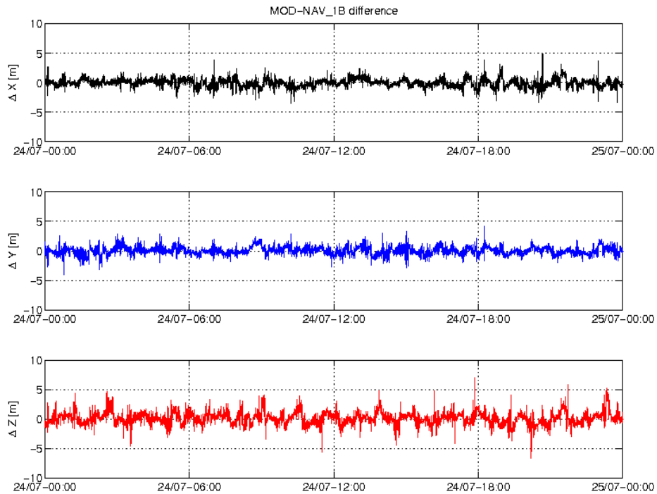
Figure 3-4: Difference MOD-GPSNAV, S/C B, 24/07. From top to bottom: X, Y and Z-axis
