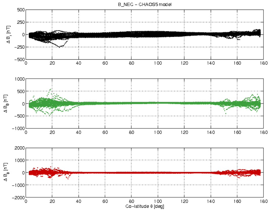
Figure 3-21: S/C C day 24/07 B NEC - B Chaos difference vs colatitude.
