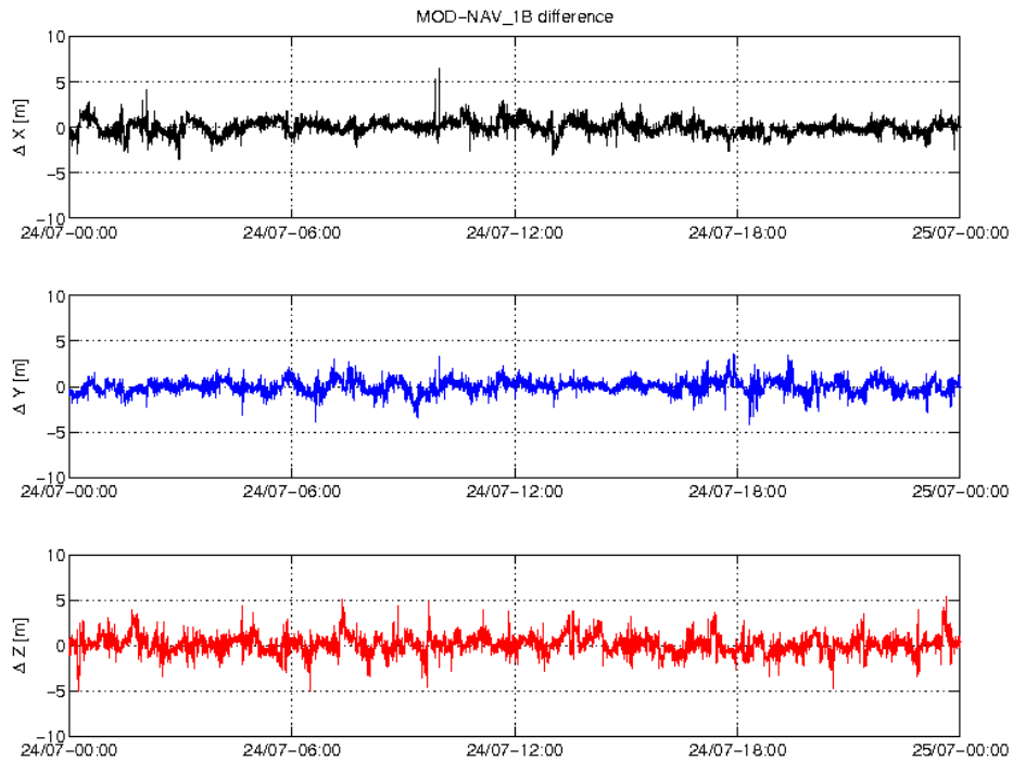
Figure 3-3: Difference MOD-GPSNAV, S/C A, 24/07. From top to bottom: X, Y and Z-axis
