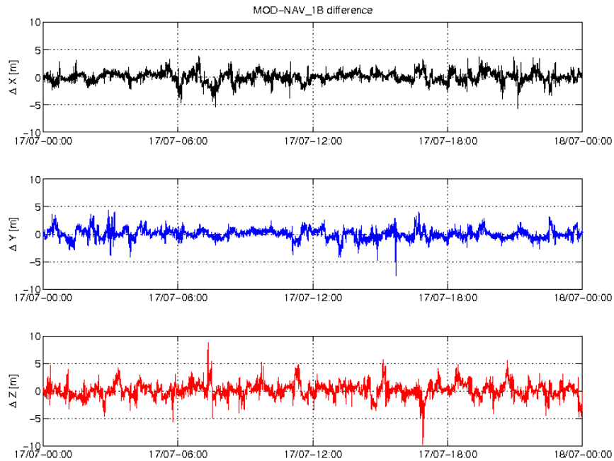
Figure 3-4: Difference MOD-GPSNAV, S/C B, 17/07. From top to bottom: X, Y and Z-axis
