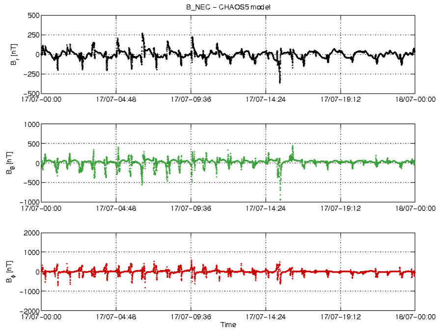
Figure 3-20: S/C B day 17/07 time series of B_{NEC} - B_{Chaos} residuals.
