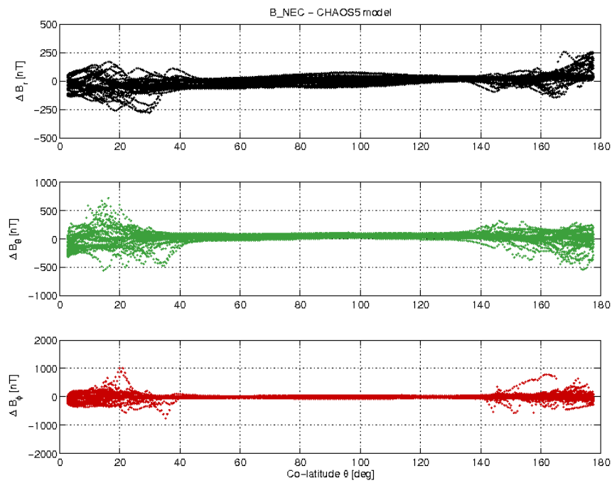
Figure 3-21: S/C C day 17/07 B_{NEC} - B_{Chaos} difference vs colatitude.
