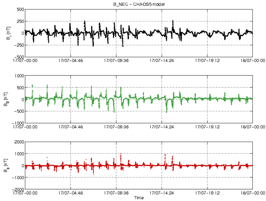
Figure 3-18: S/C A day 17/07: time series of B_{NEC} - B_{Chaos} residuals.
