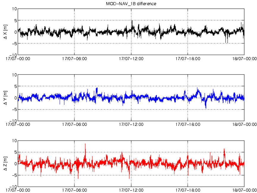
Figure 3-5: Difference MOD-GPSNAV, S/C C, 17/07. From top to bottom: X, Y and Z-axis
