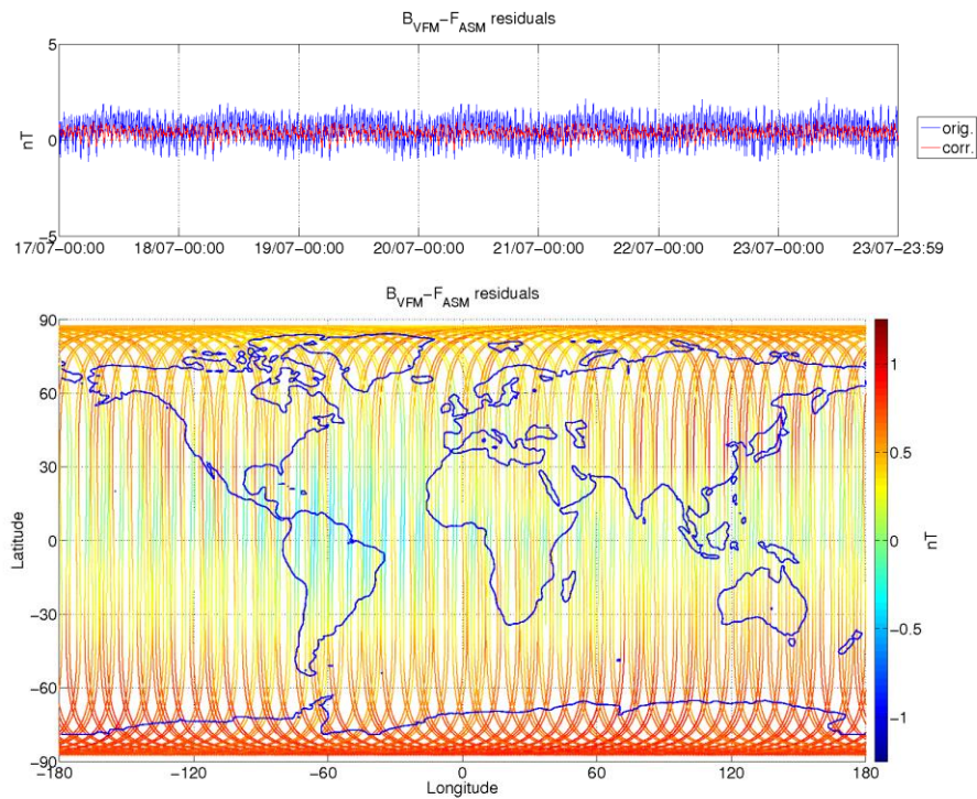
Figure 3-8: ASM-VFM residuals for S/C A, during monitoring period 17/07-23/07. In top figure are plotted: difference between |B VFM | and F ASM (without dB Sun correction) (blue colour), and the residuals with dB Sun corrections (red colour). In bottom figure residuals are presented on the world map.
