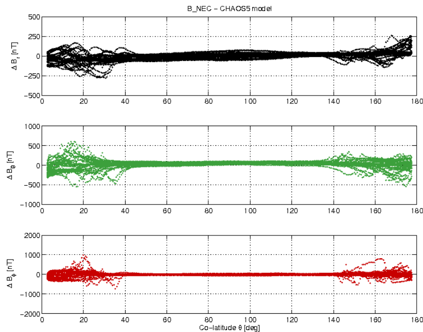
Figure 3-17: S/C A day 17/07 B_{NEC} - B_{Chaos} vs colatitude.
