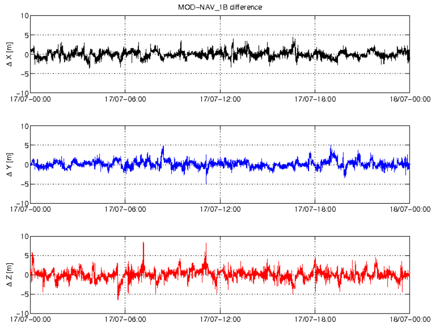
Figure 3-3: Difference MOD-GPSNAV, S/C A, 17/07. From top to bottom: X, Y and Z-axis
