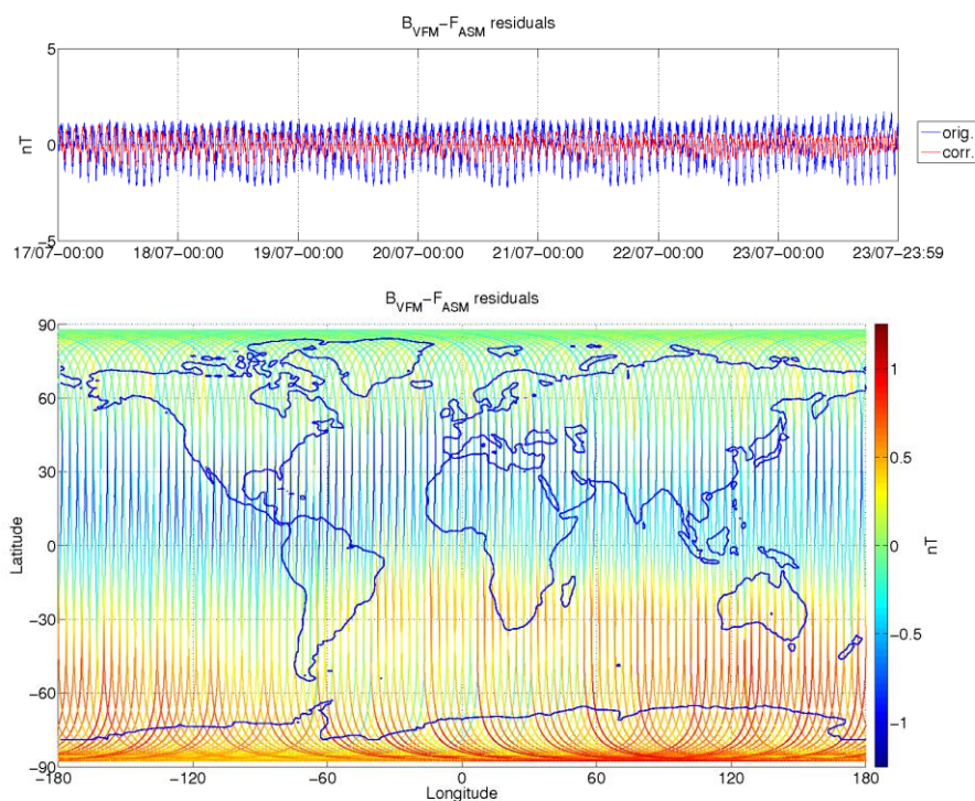
Figure 3-9: ASM-VFM residuals for S/C B, during monitoring period 17/07-23/07. In top figure are plotted: difference between |B_{VFM}| and F_{ASM} (without dB_{Sun} correction) (blue colour), and the residuals with dB_{Sun} corrections (red colour). In bottom figure residuals are presented on the world map.
