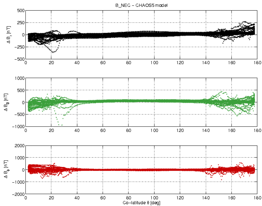
Figure 3-19: S/C B day 17/07 B_{NEC} - B_{Chaos} difference vs colatitude.
