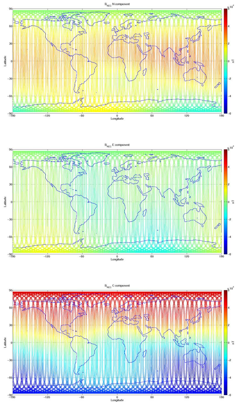
Figure 3-12: S/C C, world map plots of the geomagnetic field and components measured during monitoring period 17/07-23/07. From top to bottom: B NEC components (North, East, and Centre) of magnetic field from VFM measurement.
