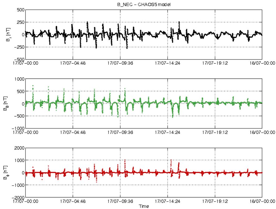
Figure 3-22: S/C C day 17/07 time series of B_{NEC} - B_{Chaos} residuals.
