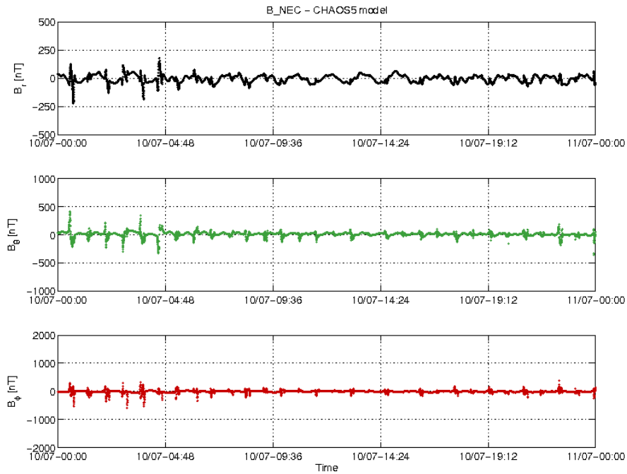
Figure 3-22: S/C C day 10/07 time series of B_{NEC} - B_{Chaos} residuals.
