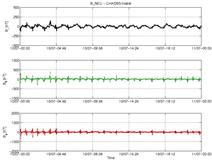
Figure 3-20: S/C B day 10/07 time series of B_{NEC} - B_{Chaos} residuals.
