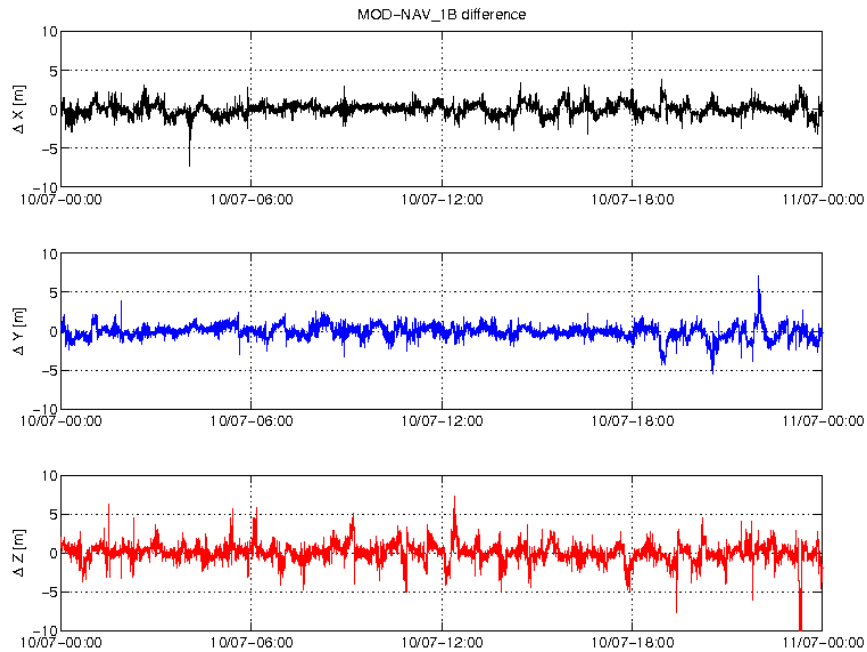
Figure 3-3: Difference MOD-GPSNAV, S/C A, 10/07. From top to bottom: X, Y and Z-axis
