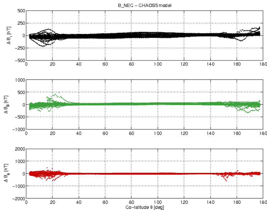
Figure 3-17: S/C A day 10/07 B_{NEC} - B_{Chaos5} vs colatitude.
