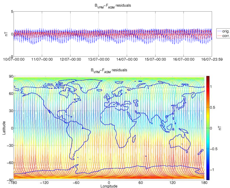
Figure 3-9: ASM-VFM residuals for S/C B, during monitoring period 10/07-16/07. In top figure are plotted: difference between |B_{VFM}| and F_{ASM} (without dB_{Sun} correction) (blue colour), and the residuals with dB_{Sun} corrections (red colour). In bottom figure residuals are presented on the world map.
