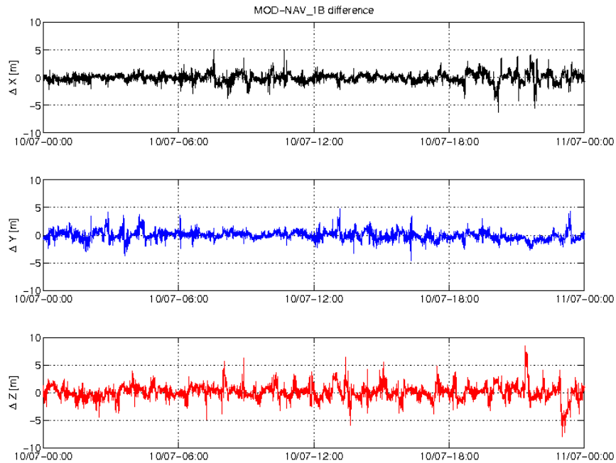
Figure 3-4: Difference MOD-GPSNAV, S/C B, 10/07. From top to bottom: X, Y and Z-axis
