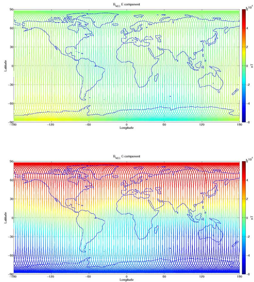
Figure 3-11: S/C B, world map plots of the geomagnetic field and components measured during monitoring period 10/07-16/07. From top to bottom: F-magnetic field from ASM measurement, B_{NEC} components (North, East, and Centre) of magnetic field from VFM measurement.
