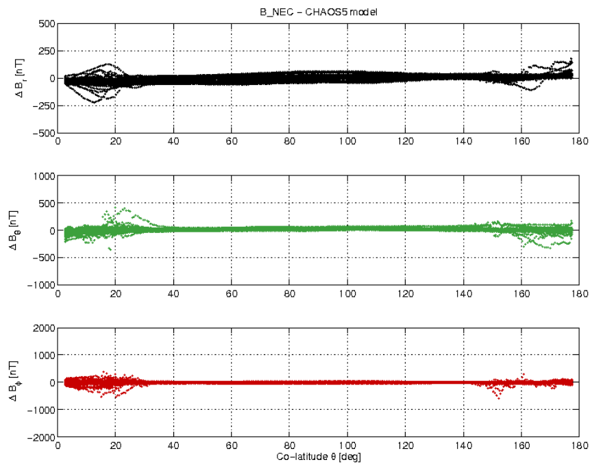
Figure 3-21: S/C C day 10/07 B_{NEC} - B_{Chaos} difference vs colatitude.
