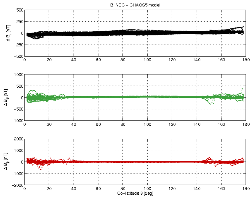
Figure 3-19: S/C B day 10/07 B_{NEC} - B_{Chaos} difference vs colatitude.
