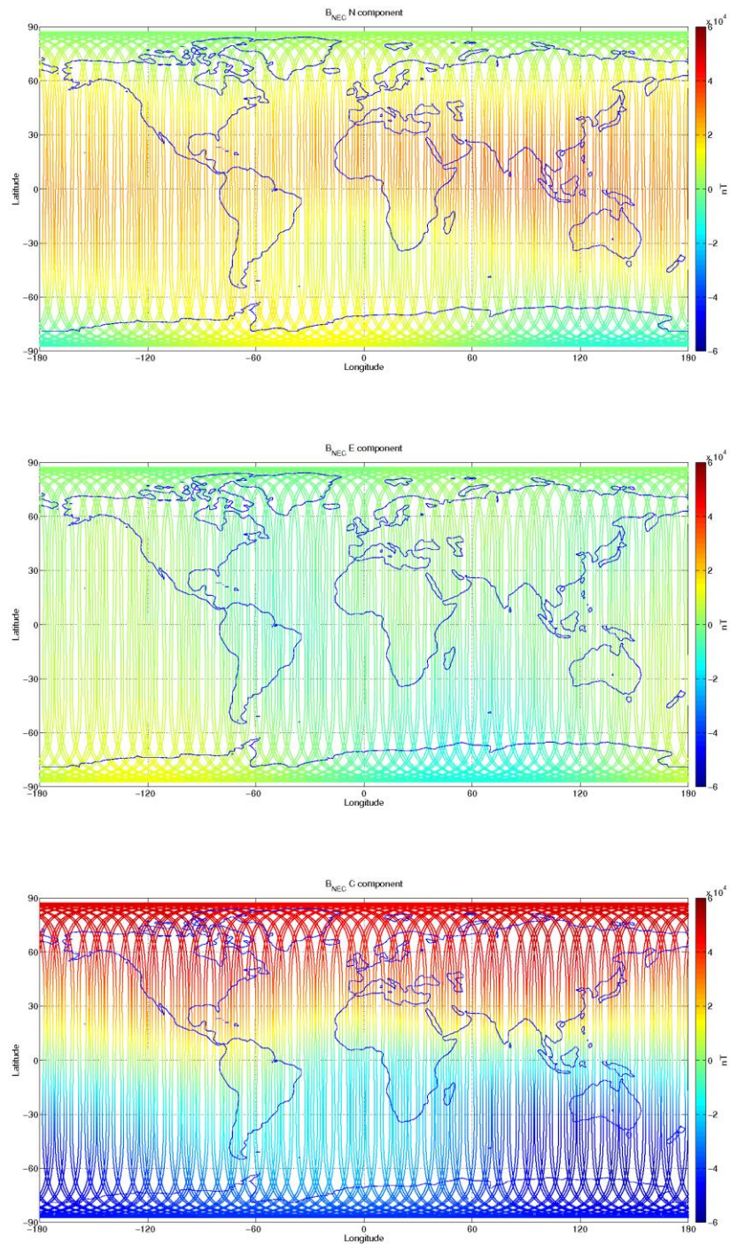
Figure 3-12: S/C C, world map plots of the geomagnetic field and components measured during monitoring period 10/07-16/07. From top to bottom: B NEC components (North, East, and Centre) of magnetic field from VFM measurement.
