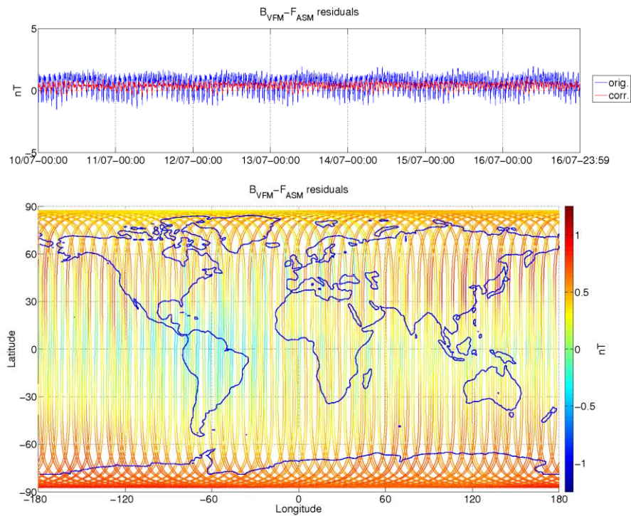
Figure 3-8: ASM-VFM residuals for S/C A, during monitoring period 10/07-16/07. In top figure are plotted: difference between |B_VFM| and F_ASM (without dB_Sun correction) (blue colour), and the residuals with dB_Sun corrections (red colour). In bottom figure residuals are presented on the world map.
