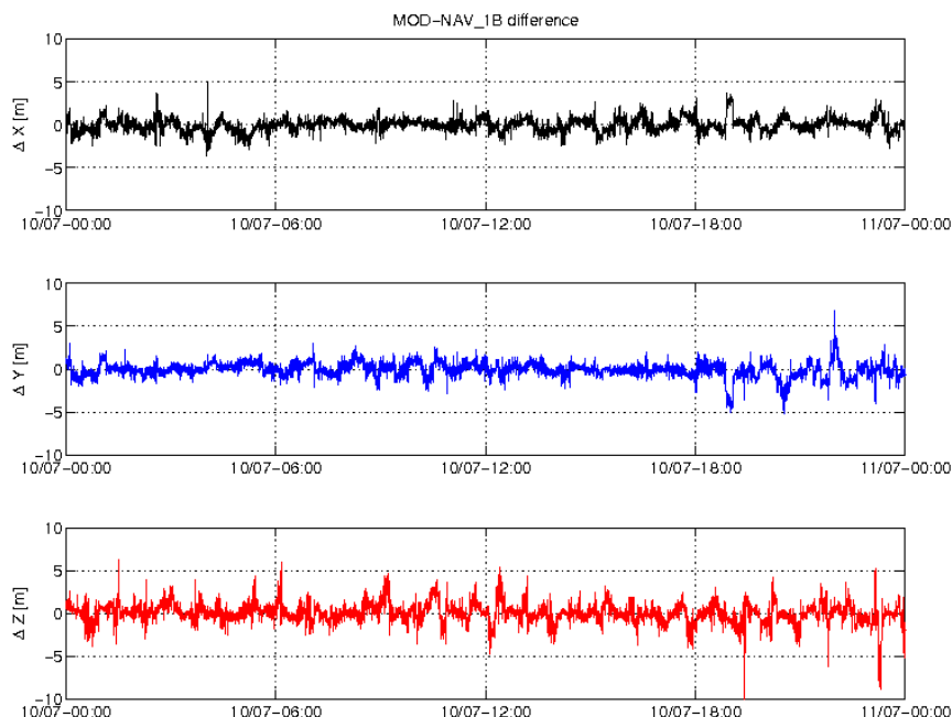
Figure 3-5: Difference MOD-GPSNAV, S/C C, 10/07. From top to bottom: X, Y and Z-axis
