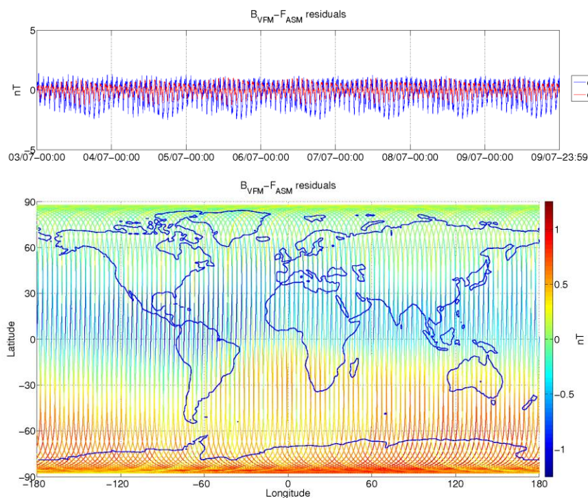
Figure 3-9: ASM-VFM residuals for S/C B, during monitoring period 03/07-09/07. In top figure are plotted: difference between |B_{VFM}| and F_{ASM} (without dB_{Sun} correction) (blue colour), and the residuals with dB_{Sun} corrections (red colour). In bottom figure residuals are presented on the world map.
