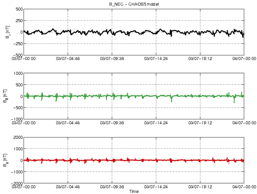
Figure 3-22: S/C C day 03/07 time series of B_{NEC} - B_{Chaos} residuals.
