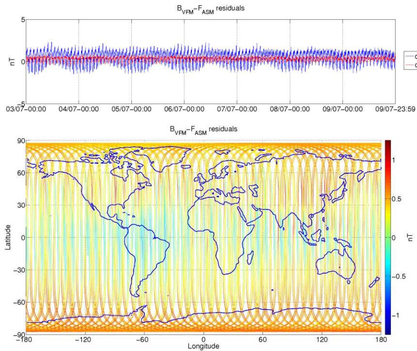
Figure 3-8: ASM-VFM residuals for S/C A, during monitoring period 03/07-09/07. In top figure are plotted: difference between |B VFM | and F ASM (without dB Sun correction) (blue colour), and the residuals with dB Sun corrections (red colour). In bottom figure residuals are presented on the world map.
