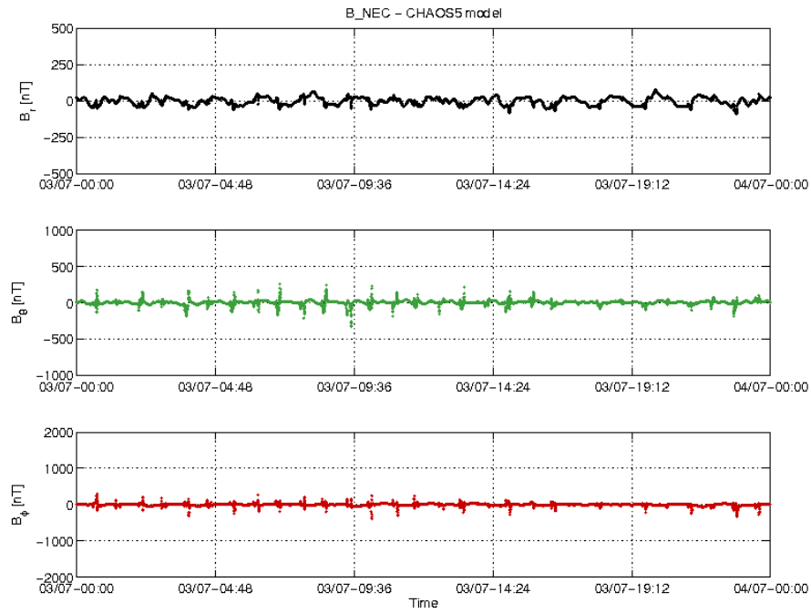
Figure 3-20: S/C B day 03/07 time series of B_{NEC} - B_{Chaos} residuals.
