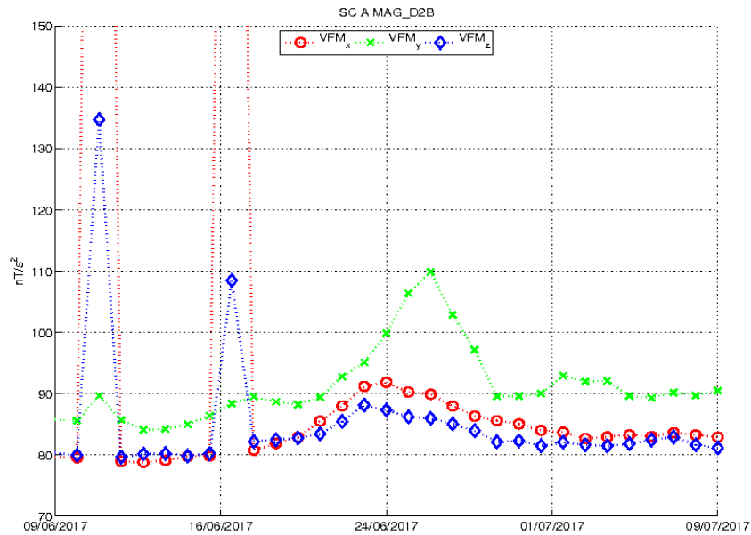
Figure 3-23: Plot of standard deviation of B components in VFM frames.
