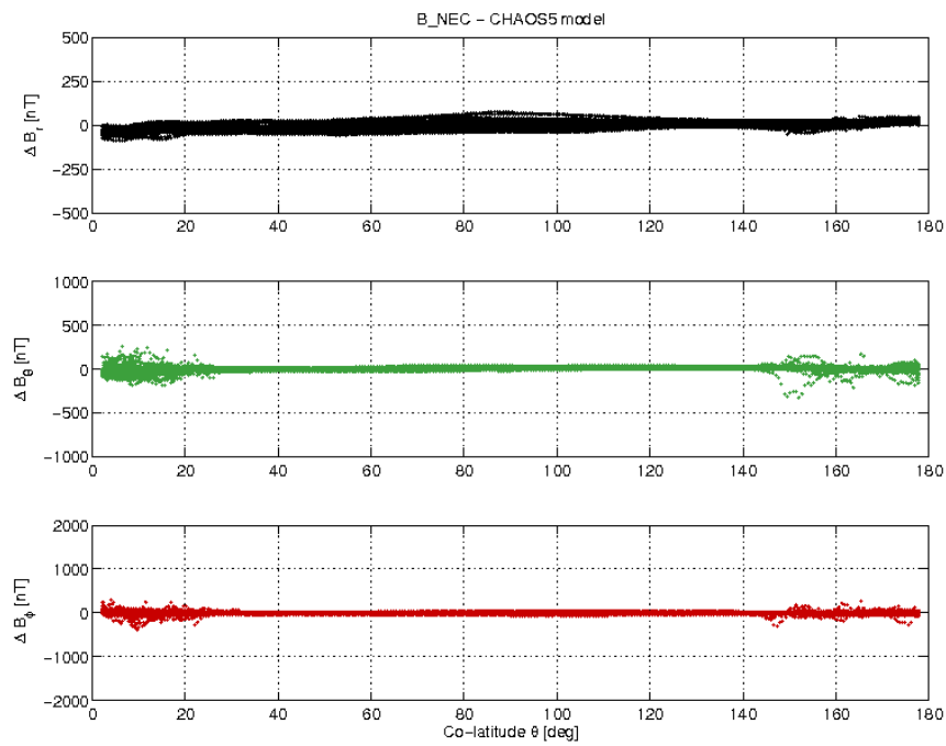
Figure 3-19: S/C B day 03/07 B_{NEC} - B_{Chaos} difference vs colatitude.
