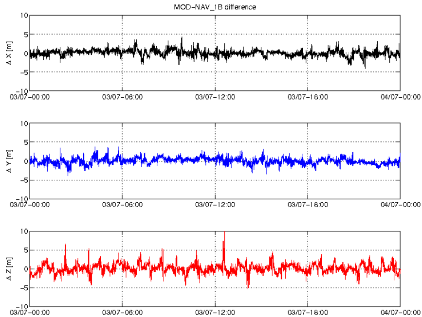
Figure 3-4: Difference MOD-GPSNAV, S/C B, 03/07. From top to bottom: X, Y and Z-axis
