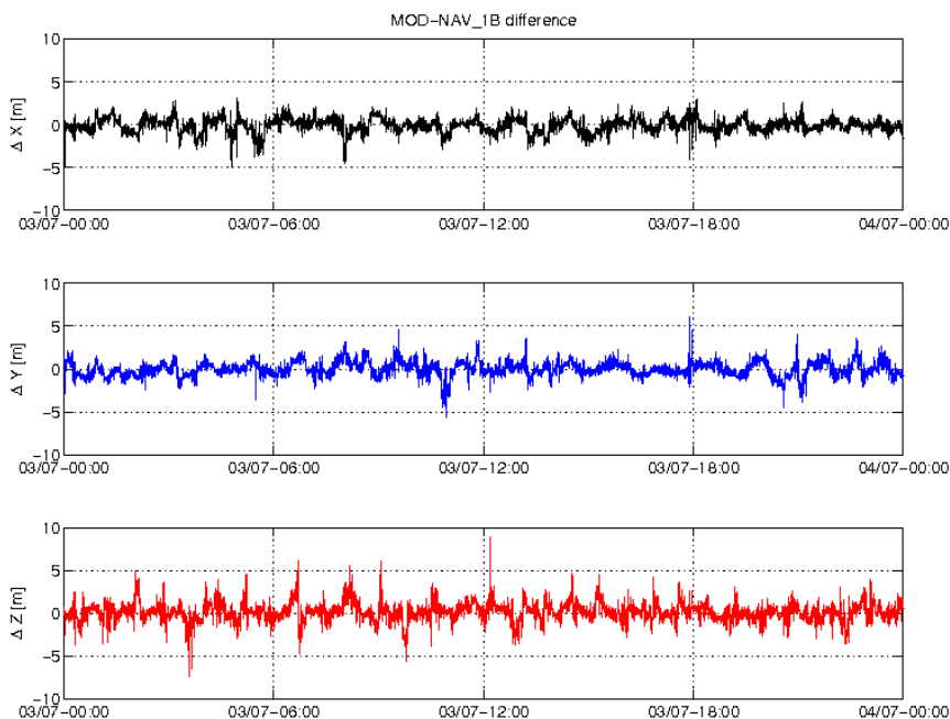
Figure 3-5: Difference MOD-GPSNAV, S/C C, 03/07. From top to bottom: X, Y and Z-axis
