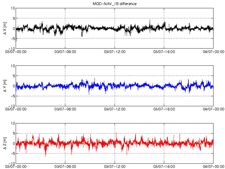
Figure 3-3: Difference MOD-GPSNAV, S/C A, 03/07. From top to bottom: X, Y and Z-axis
