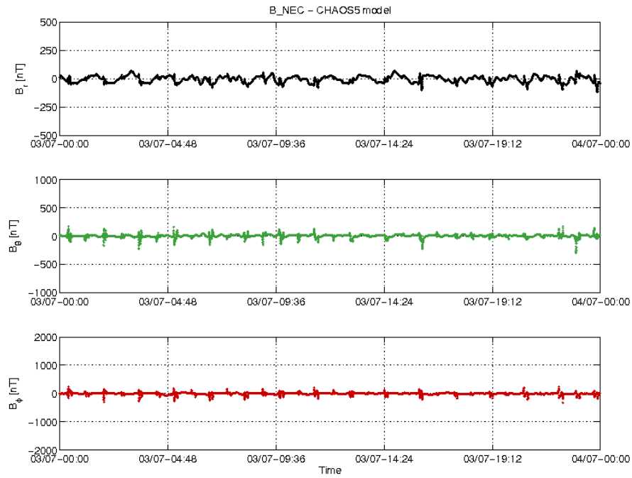
Figure 3-18: S/C A day 03/07: time series of B_{NEC} - B_{Chaos} residuals.
