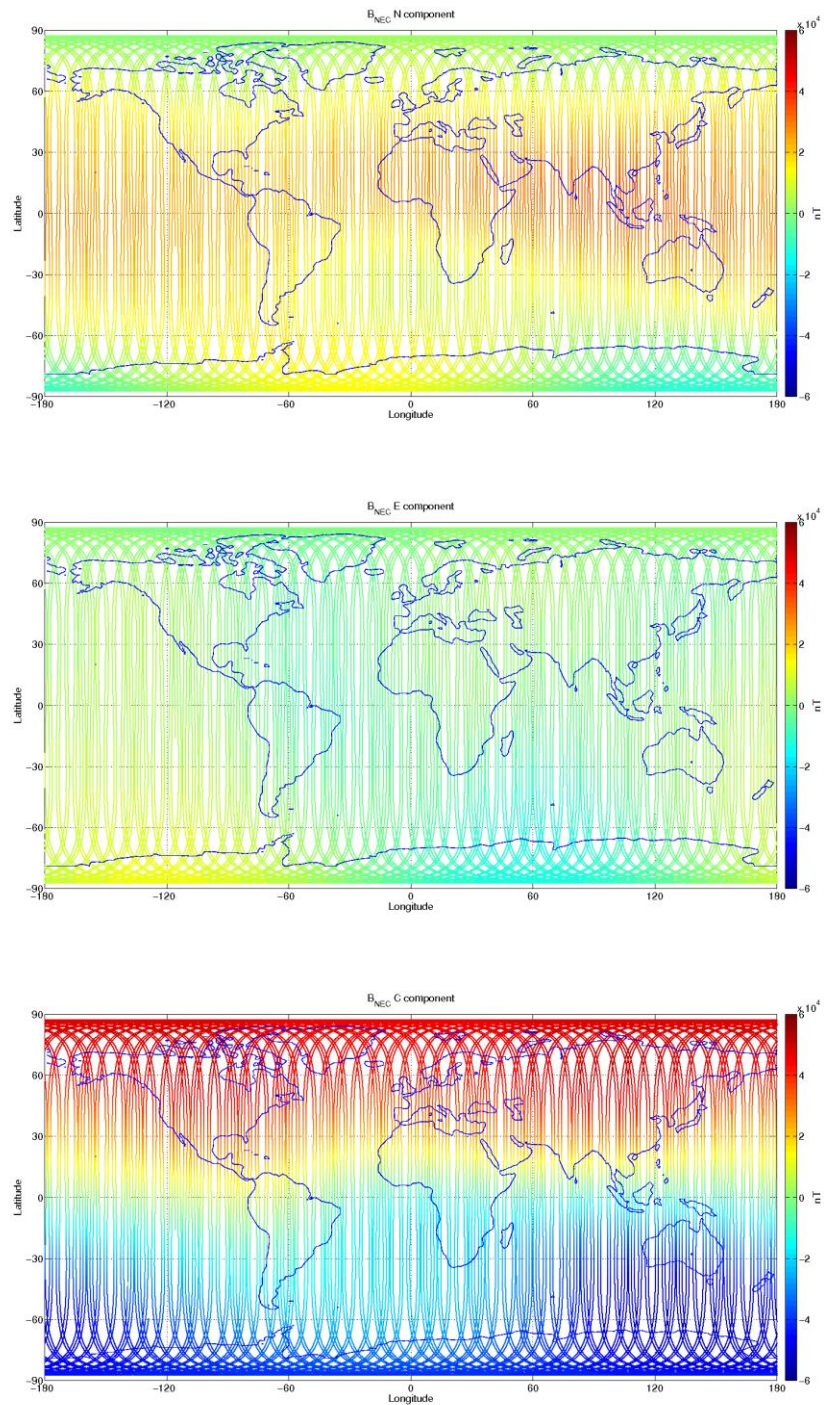
Figure 3-12: S/C C, world map plots of the geomagnetic field and components measured during monitoring period 03/07-09/07. From top to bottom: B_{NEC} components (North, East, and Centre) of magnetic field from VFM measurement.
