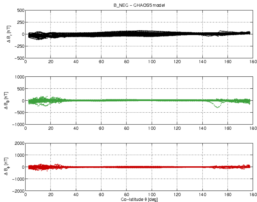
Figure 3-17: S/C A day 03/07 B_{NEC} - B_{Chaos} vs colatitude.
