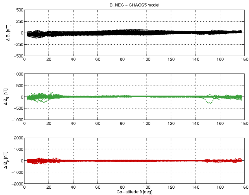
Figure 3-21: S/C C day 03/07 B_{NEC} - B_{Chaos} difference vs colatitude.
