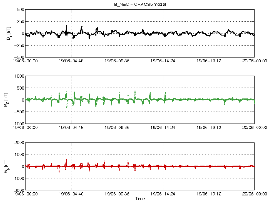
Figure 3-20: S/C B day 19/06 time series of B_{NEC} - B_{Chaos} residuals.
