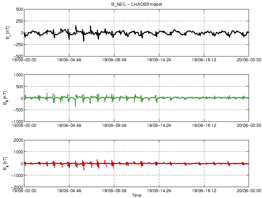
Figure 3-22: S/C C day 19/06 time series of B_{NEC} - B_{Chaos} residuals.
