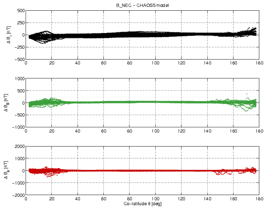
Figure 3-21: S/C C day 19/06 B_{NEC} - B_{Chaos} difference vs colatitude.
