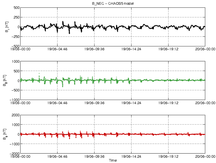
Figure 3-18: S/C A day 19/06: time series of B_{NEC} - B_{Chaos} residuals.
