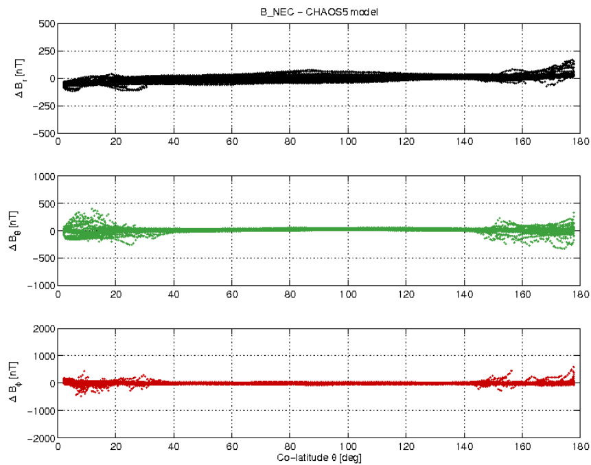
Figure 3-19: S/C B day 19/06 B_{NEC} - B_{Chaos} difference vs colatitude.
