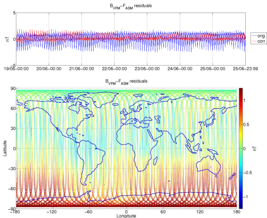
Figure 3-8: ASM-VFM residuals for S/C A, during monitoring period 19/06-25/06. In top figure are plotted: difference between |B_{VFM}| and F_{ASM} (without dB_{Sun} correction) (blue colour), and the residuals with dB_{Sun} corrections (red colour). In bottom figure residuals are presented on the world map.
