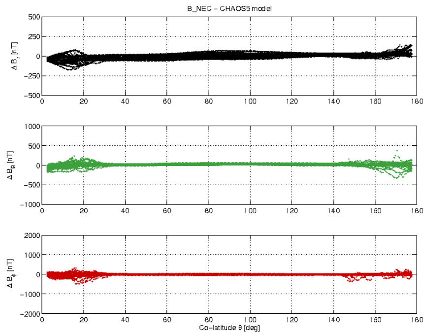
Figure 3-17: S/C A day 19/06 B_{NEC} - B_{Chaos} vs colatitude.
