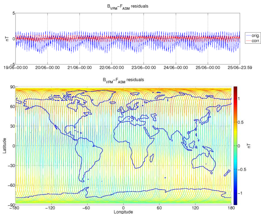
Figure 3-9: ASM-VFM residuals for S/C B, during monitoring period 19/06-25/06. In top figure are plotted: difference between |B_{VFM}| and F_{ASM} (without dB_{Sun} correction) (blue colour), and the residuals with dB_{Sun} corrections (red colour). In bottom figure residuals are presented on the world map.
