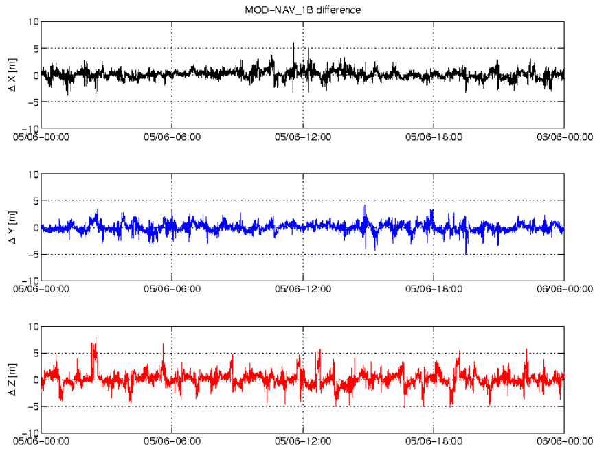
Figure 3-4: Difference MOD-GPSNAV, S/C B, 05/06. From top to bottom: X, Y and Z-axis
