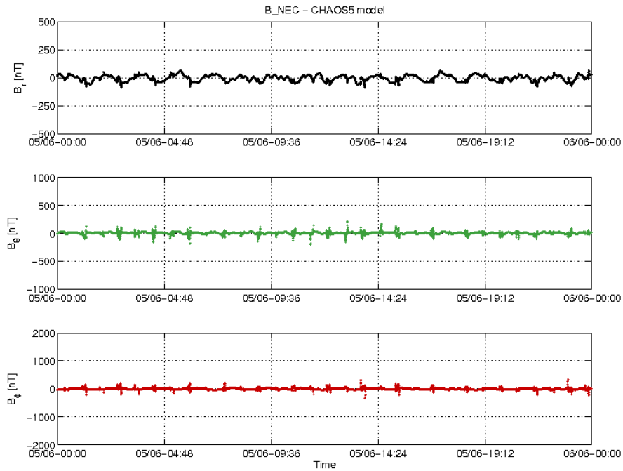
Figure 3-22: S/C C day 05/06 time series of B_{NEC} - B_{Chaos} residuals.
