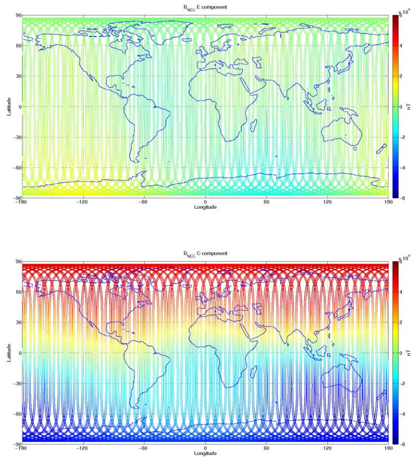
Figure 3-10: S/C A, world map plots of the geomagnetic field and components measured during monitoring period 05/06-11/06. From top to bottom: F-magnetic field from ASM measurement, B NEC components (North, East, and Centre) of magnetic field from VFM measurement.
