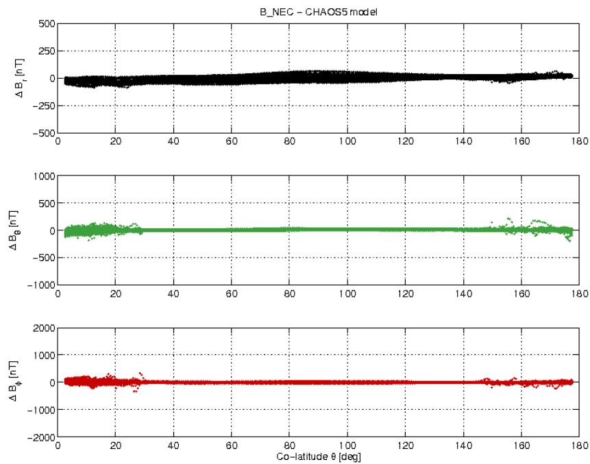
Figure 3-21: S/C C day 05/06 B_{NEC} - B_{Chaos} difference vs colatitude.
