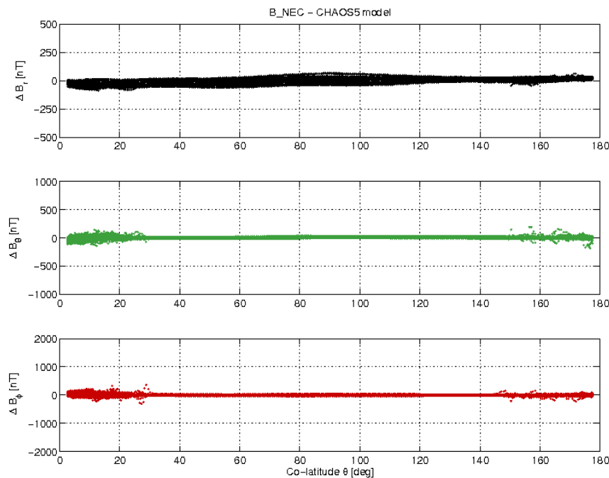
Figure 3-17: S/C A day 05/06 B_{NEC} - B_{Chaos5} vs colatitude.
