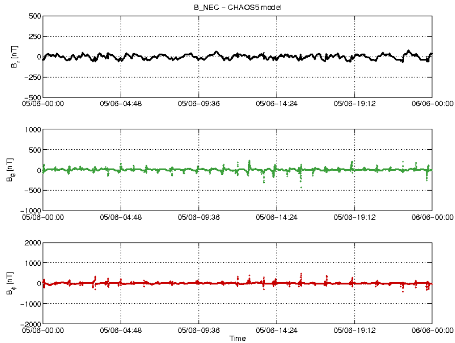
Figure 3-20: S/C B day 05/06 time series of B_{NEC} - B_{Chaos} residuals.
