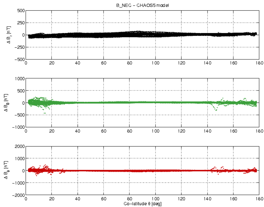
Figure 3-19: S/C B day 05/06 B_{NEC} - B_{Chaos} difference vs colatitude.
