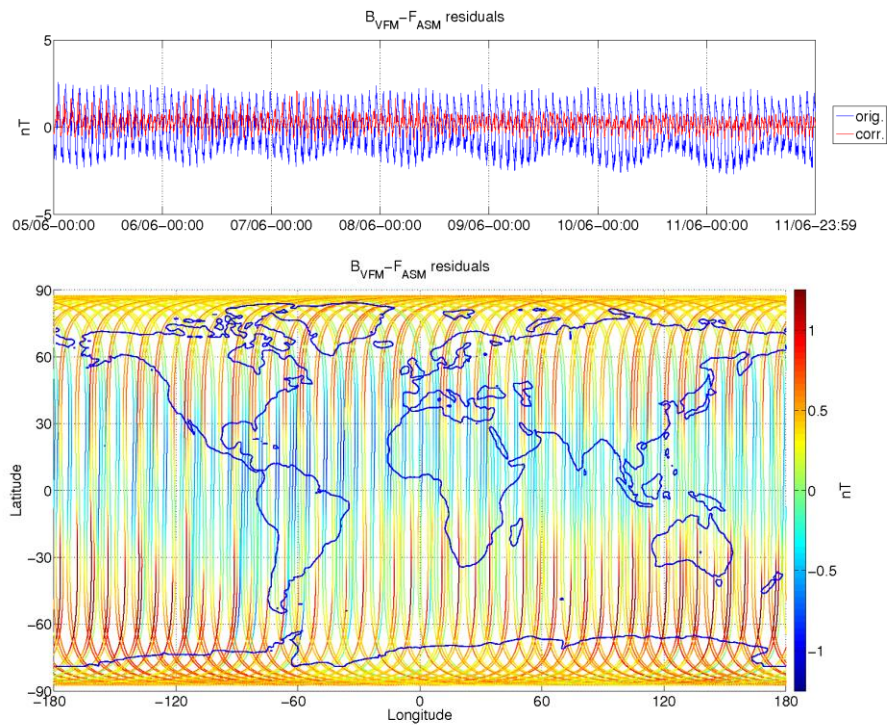
Figure 3-8: ASM-VFM residuals for S/C A, during monitoring period 05/06-11/06. In top figure are plotted: difference between |B VFM | and F ASM (without dB Sun correction) (blue colour), and the residuals with dB Sun corrections (red colour). In bottom figure residuals are presented on the world map.
