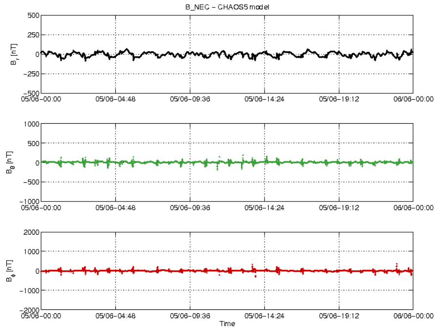
Figure 3-18: S/C A day 05/06: time series of B_{NEC} - B_{Chaos} residuals.
