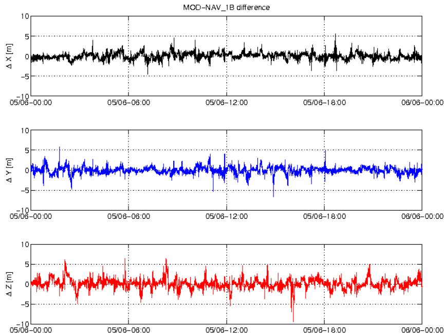
Figure 3-5: Difference MOD-GPSNAV, S/C C, 05/06. From top to bottom: X, Y and Z-axis
