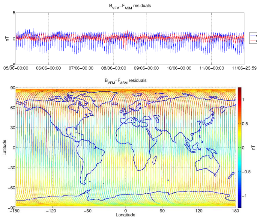
Figure 3-9: ASM-VFM residuals for S/C B, during monitoring period 05/06-11/06. In top figure are plotted: difference between |B_{VFM}| and F_{ASM} (without dB_{Sun} correction) (blue colour), and the residuals with dB_{Sun} corrections (red colour). In bottom figure residuals are presented on the world map.
