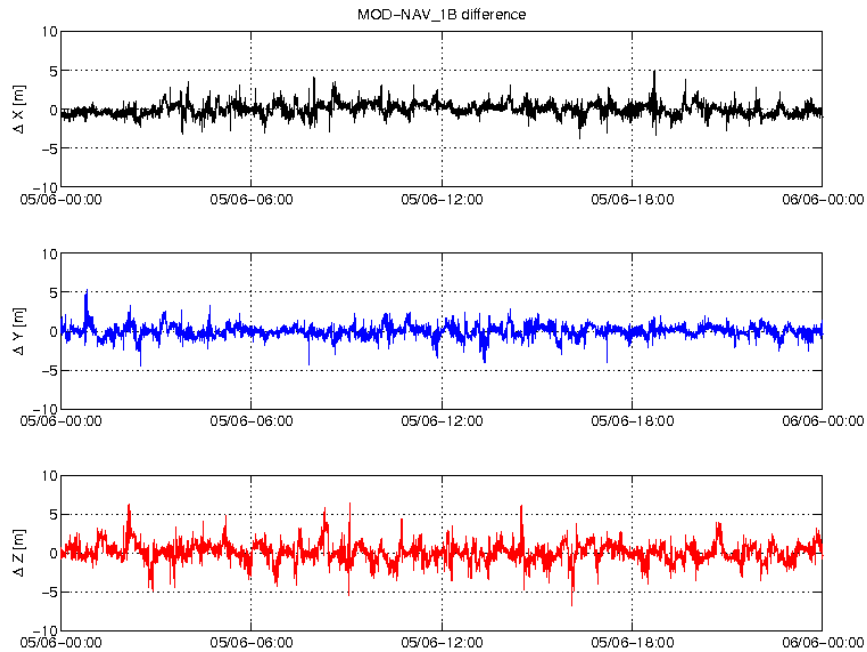
Figure 3-3: Difference MOD-GPSNAV, S/C A, 05/06. From top to bottom: X, Y and Z-axis
