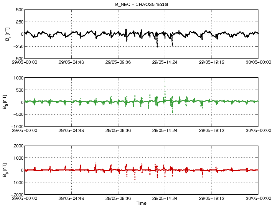
Figure 3-22: S/C C day 29/05 time series of B_{NEC} - B_{Chaos} residuals.
