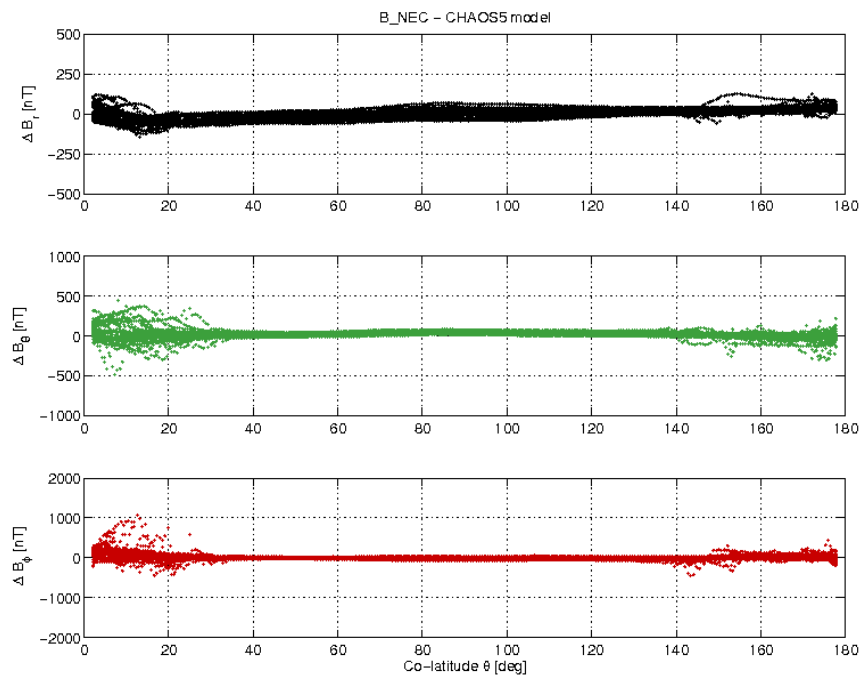
Figure 3-19: S/C B day 29/05 B_{NEC} - B_{Chaos} difference vs colatitude.
