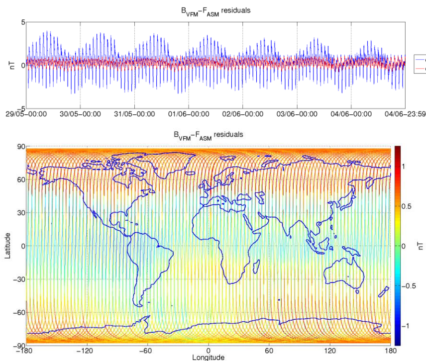
Figure 3-9: ASM-VFM residuals for S/C B, during monitoring period 29/05-04/06. In top figure are plotted: difference between |B\_VFM| and F\_ASM (without dB\_Sun correction) (blue colour), and the residuals with dB\_Sun corrections (red colour). In bottom figure residuals are presented on the world map.
