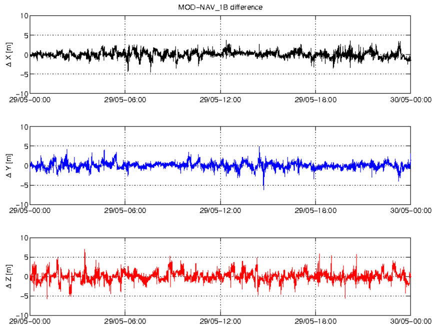
Figure 3-3: Difference MOD-GPSNAV, S/C A, 29/05. From top to bottom: X, Y and Z-axis
