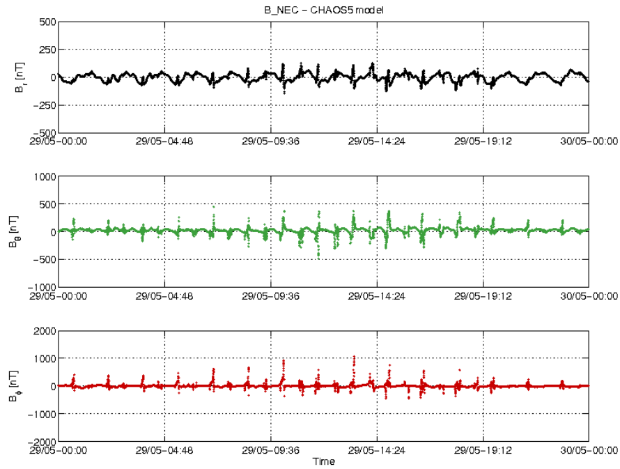
Figure 3-20: S/C B day 29/05 time series of B_{NEC} - B_{Chaos} residuals.
