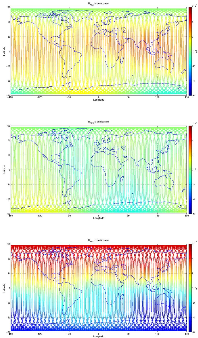
Figure 3-12: S/C C, world map plots of the geomagnetic field and components measured during monitoring period 29/05-04/06. From top to bottom: B_{NEC} components (North, East, and Centre) of magnetic field from VFM measurement.
