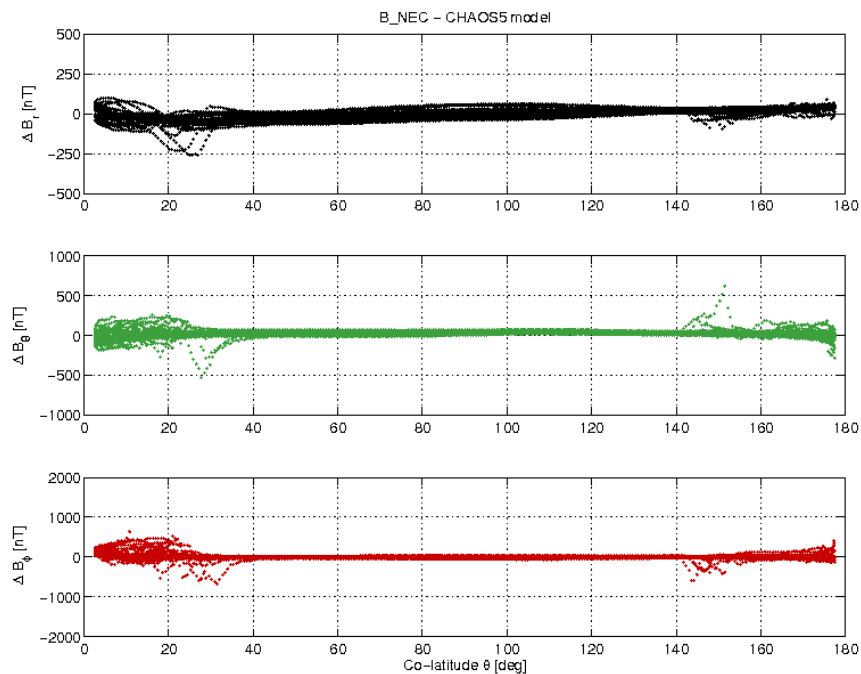
Figure 3-17: S/C A day 29/05 B_{NEC} - B_{Chaos} vs colatitude.
