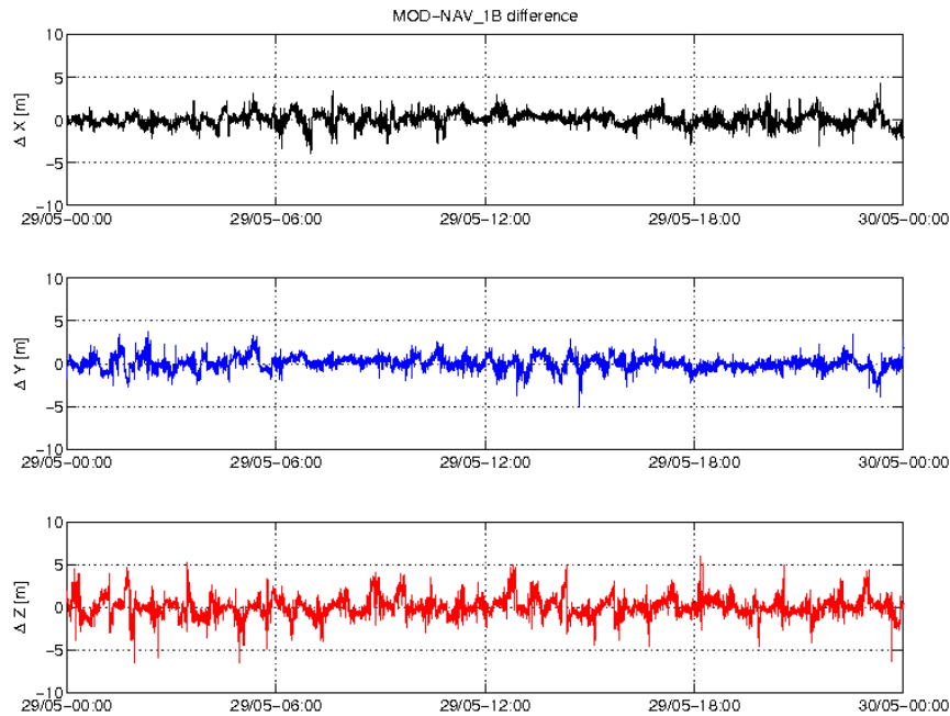
Figure 3-5: Difference MOD-GPSNAV, S/C C, 29/05. From top to bottom: X, Y and Z-axis
