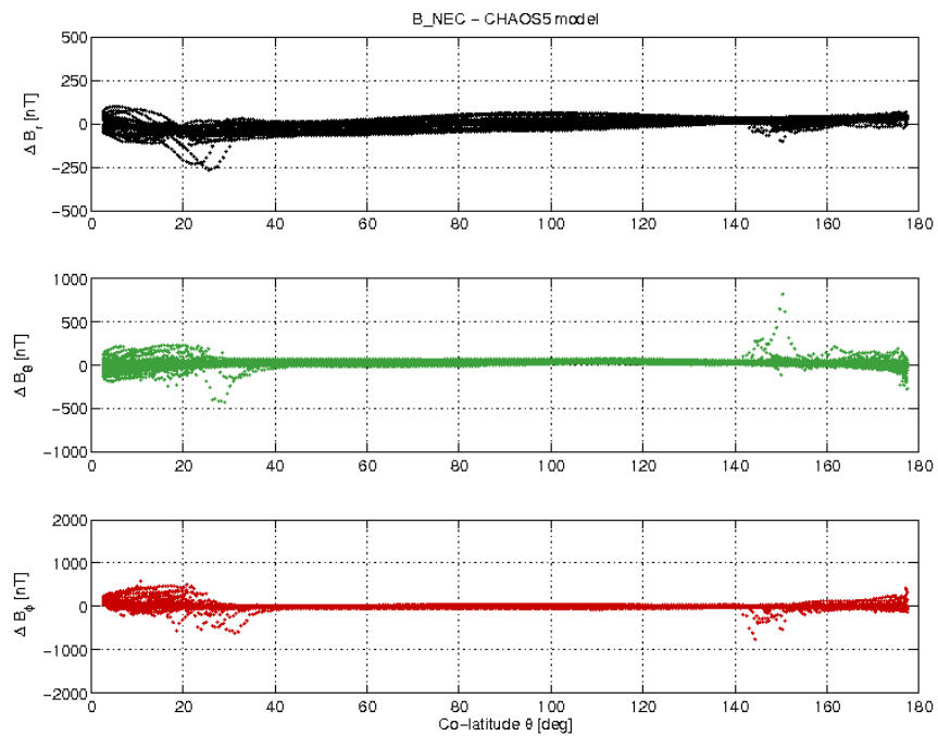
Figure 3-21: S/C C day 29/05 B_{NEC} - B_{Chaos} difference vs colatitude.
