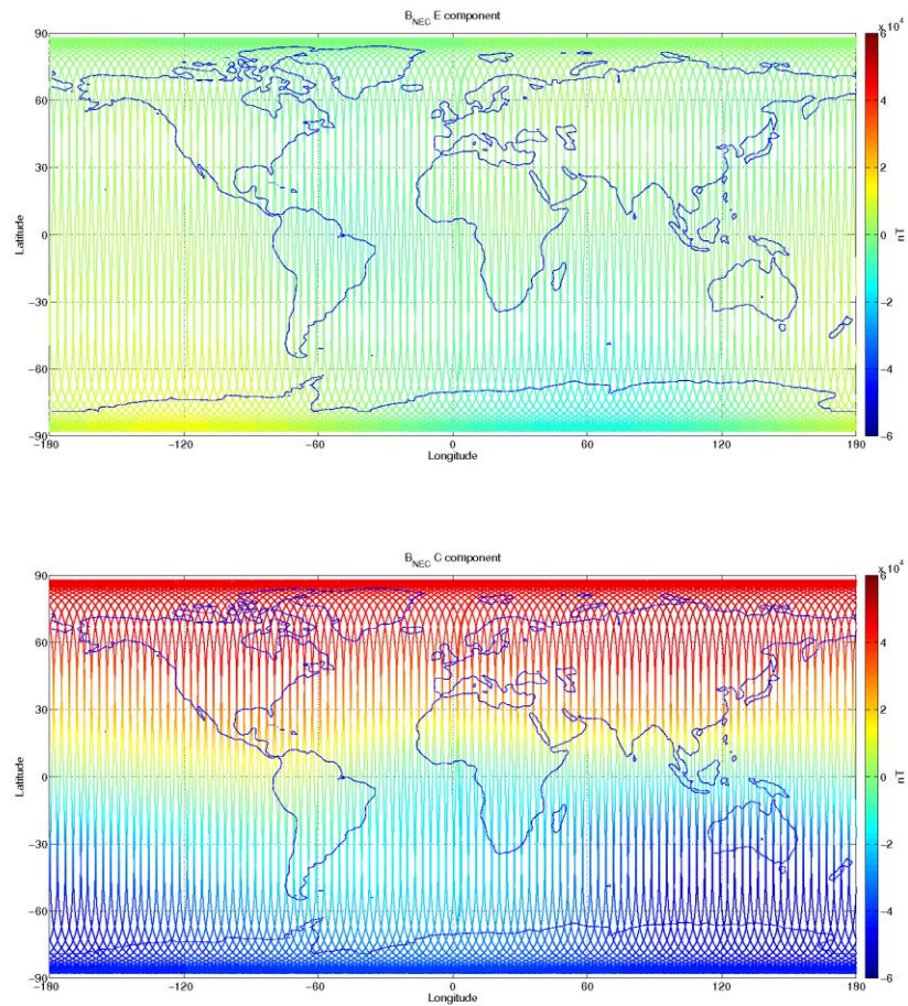
Figure 3-11: S/C B, world map plots of the geomagnetic field and components measured during monitoring period 29/05-04/06. From top to bottom: F-magnetic field from ASM measurement, B_{NEC} components (North, East, and Centre) of magnetic field from VFM measurement.
