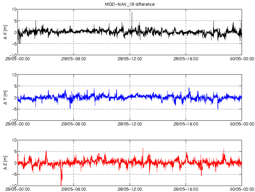
Figure 3-4: Difference MOD-GPSNAV, S/C B, 29/05. From top to bottom: X, Y and Z-axis
