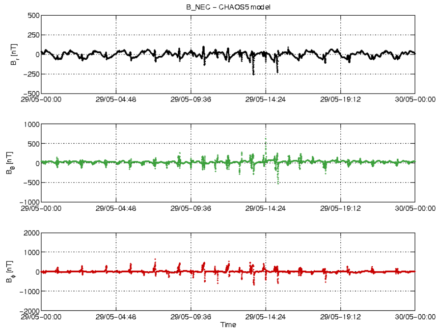
Figure 3-18: S/C A day 29/05: time series of B_{NEC} - B_{Chaos} residuals.
