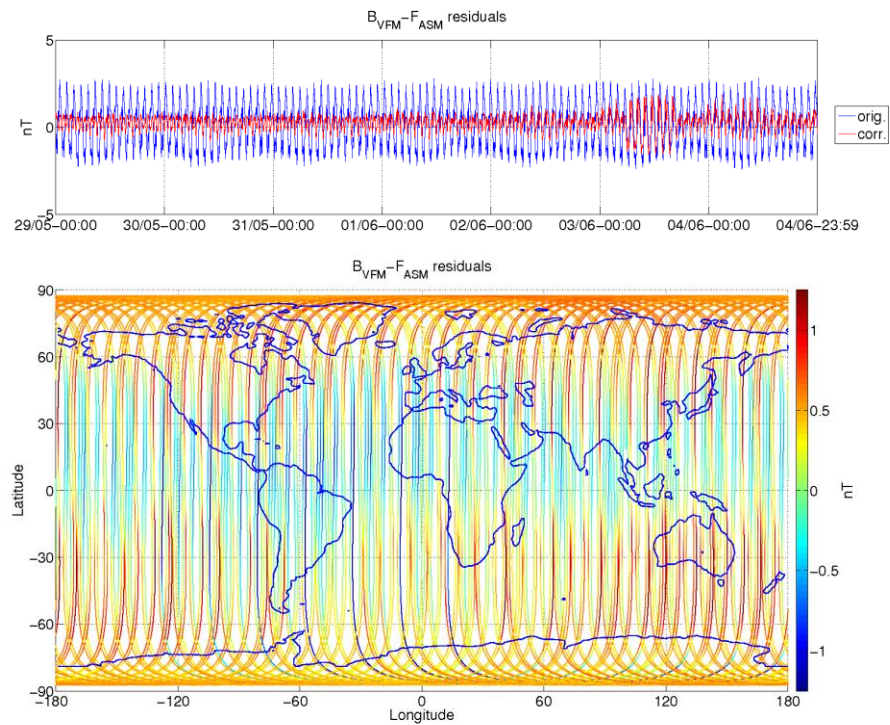
Figure 3-8: ASM-VFM residuals for S/C A, during monitoring period 29/05-04/06. In top figure are plotted: difference between |B_{VFM}| and F_{ASM} (without dB_{Sun} correction) (blue colour), and the residuals with dB_{Sun} corrections (red colour). In bottom figure residuals are presented on the world map.
