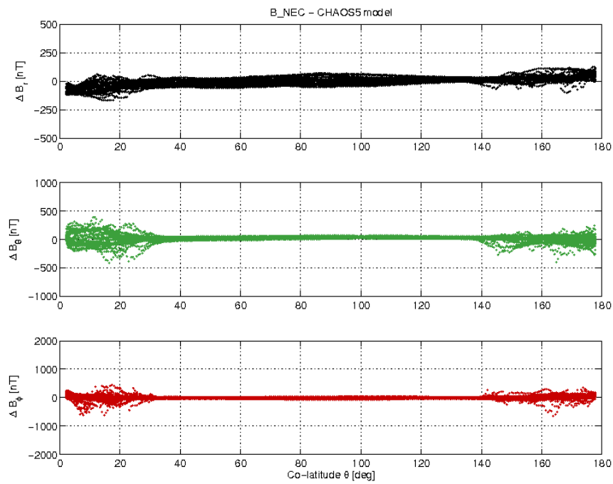
Figure 3-19: S/C B day 22/05 B_{NEC} - B_{Chaos} difference vs colatitude.
