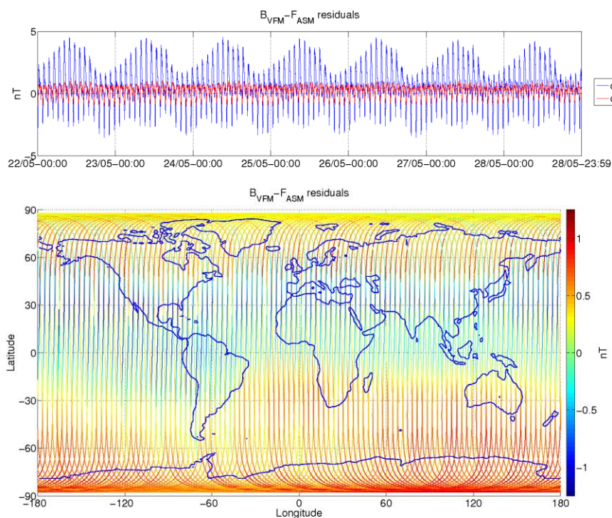
Figure 3-9: ASM-VFM residuals for S/C B, during monitoring period 22/05-28/05. In top figure are plotted: difference between |B VFM | and F ASM (without dB Sun correction) (blue colour), and the residuals with dB Sun corrections (red colour). In bottom figure residuals are presented on the world map.
