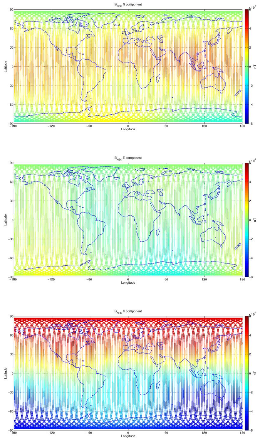
Figure 3-12: S/C C, world map plots of the geomagnetic field and components measured during monitoring period 22/05-28/05. From top to bottom: B NEC components (North, East, and Centre) of magnetic field from VFM measurement.
