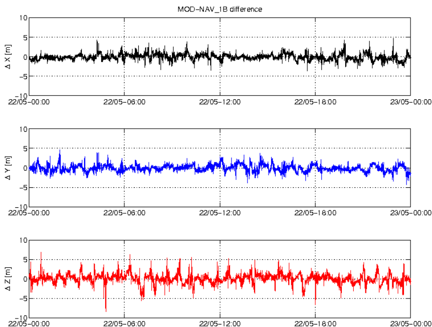
Figure 3-5: Difference MOD-GPSNAV, S/C C, 22/05. From top to bottom: X, Y and Z-axis
