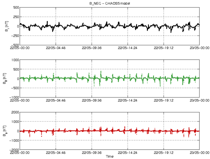
Figure 3-20: S/C B day 22/05 time series of B_{NEC} - B_{Chaos} residuals.
