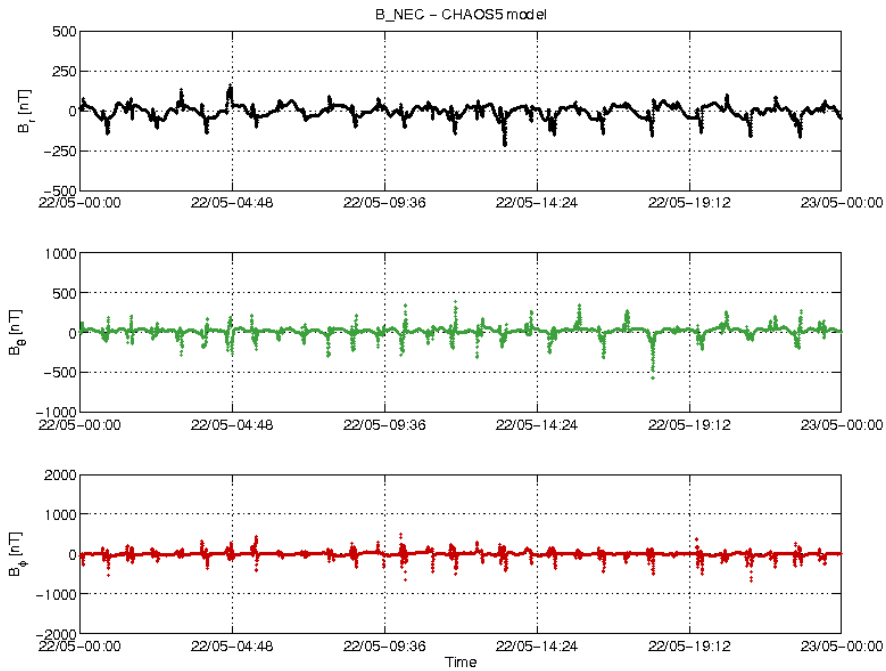
Figure 3-22: S/C C day 22/05 time series of B_{NEC} - B_{Chaos} residuals.
