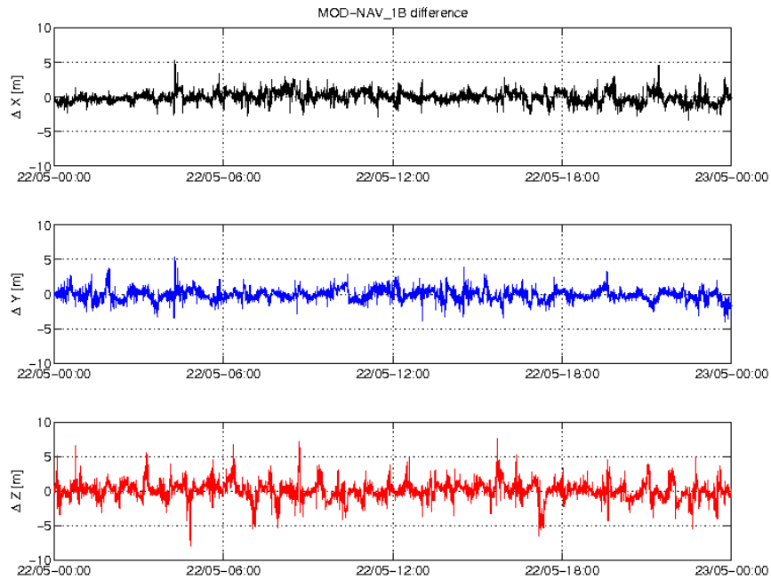
Figure 3-3: Difference MOD-GPSNAV, S/C A, 22/05. From top to bottom: X, Y and Z-axis
