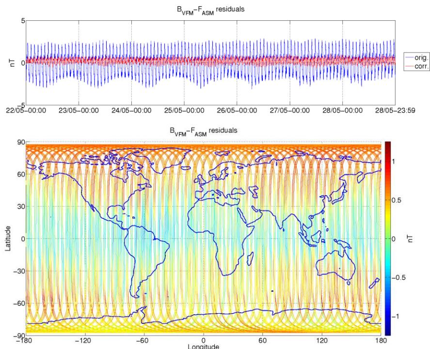
Figure 3-8: ASM-VFM residuals for S/C A, during monitoring period 22/05-28/05. In top figure are plotted: difference between |B_{VFM}| and F_{ASM} (without dB_{Sun} correction) (blue colour), and the residuals with dB_{Sun} corrections (red colour). In bottom figure residuals are presented on the world map.
