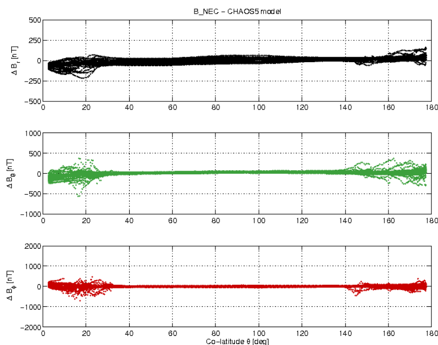
Figure 3-17: S/C A day 22/05 B_{NEC} - B_{Chaos5} vs colatitude.
