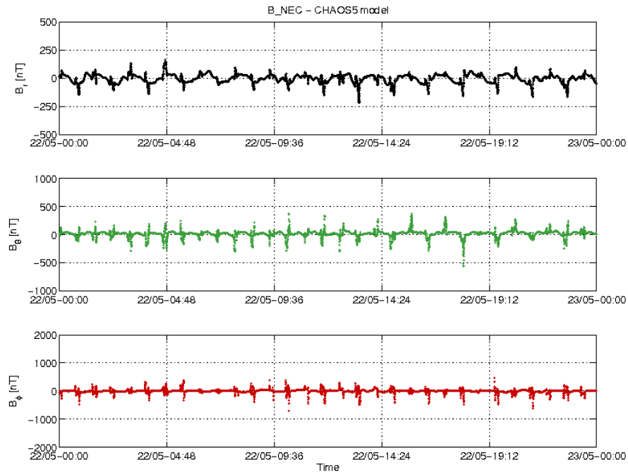
Figure 3-18: S/C A day 22/05: time series of B_{NEC} - B_{Chaos} residuals.
