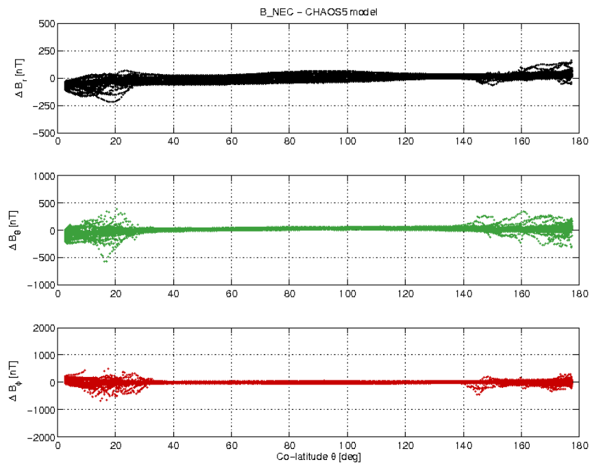
Figure 3-21: S/C C day 22/05 B_{NEC} - B_{Chaos} difference vs colatitude.
