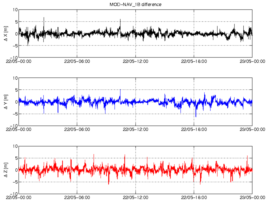
Figure 3-4: Difference MOD-GPSNAV, S/C B, 22/05. From top to bottom: X, Y and Z-axis
