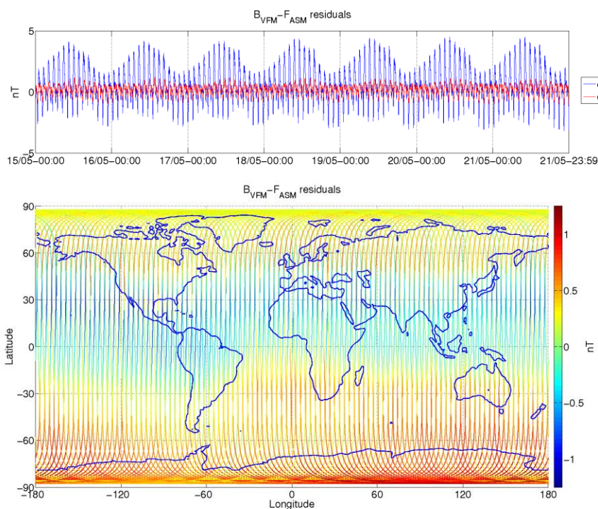
Figure 3-9: ASM-VFM residuals for S/C B, during monitoring period 15/05-21/05. In top figure are plotted: difference between |B_{VFM}| and F_{ASM} (without dB_{Sun} correction) (blue colour), and the residuals with dB_{Sun} corrections (red colour). In bottom figure residuals are presented on the world map.
