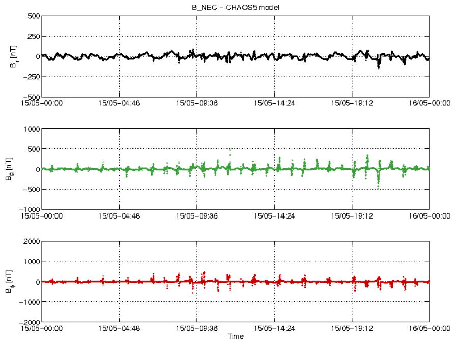
Figure 3-22: S/C C day 15/05 time series of B_{NEC} - B_{Chaos} residuals.
