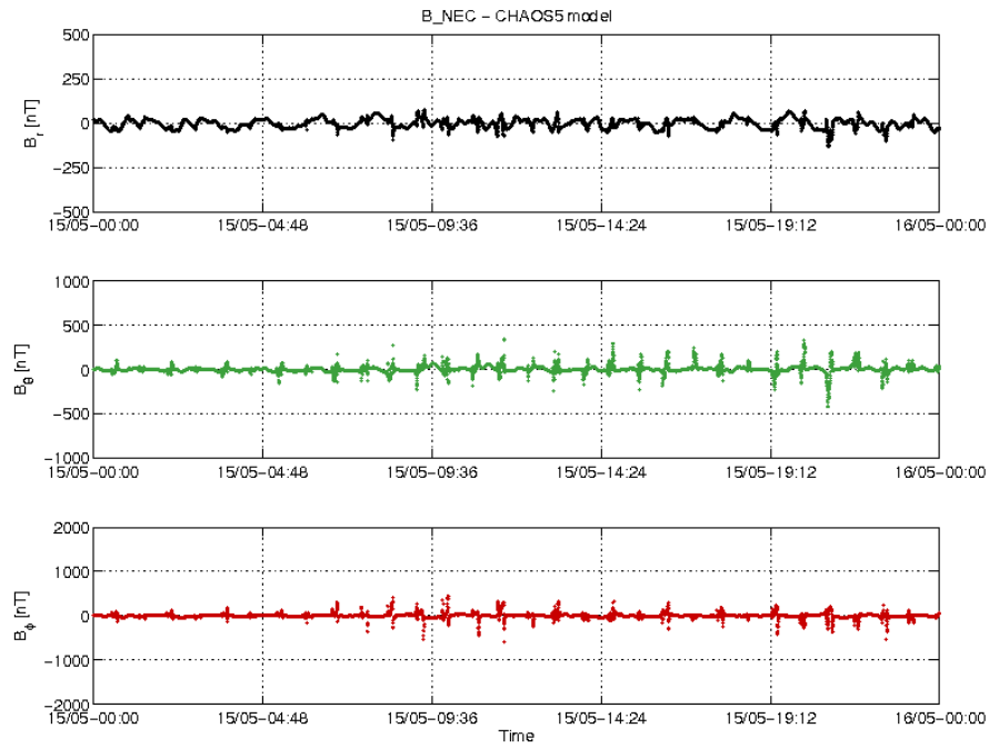
Figure 3-18: S/C A day 15/05: time series of B_{NEC} - B_{Chaos} residuals.
