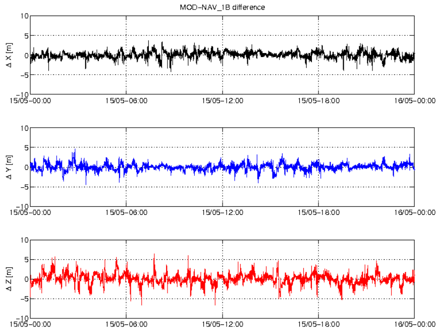
Figure 3-3: Difference MOD-GPSNAV, S/C A, 15/05. From top to bottom: X, Y and Z-axis
