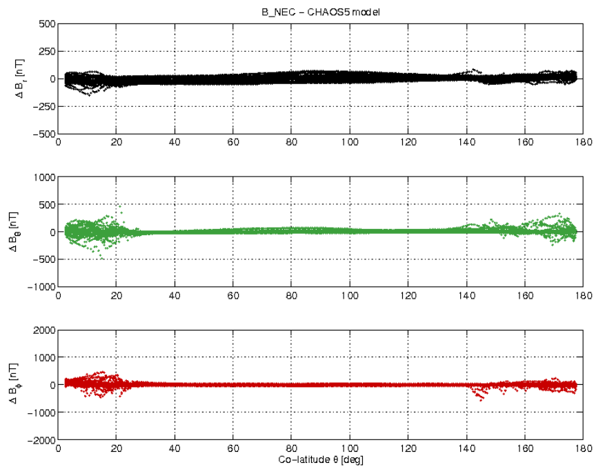
Figure 3-21: S/C C day 15/05 B_{NEC} - B_{Chaos} difference vs colatitude.
