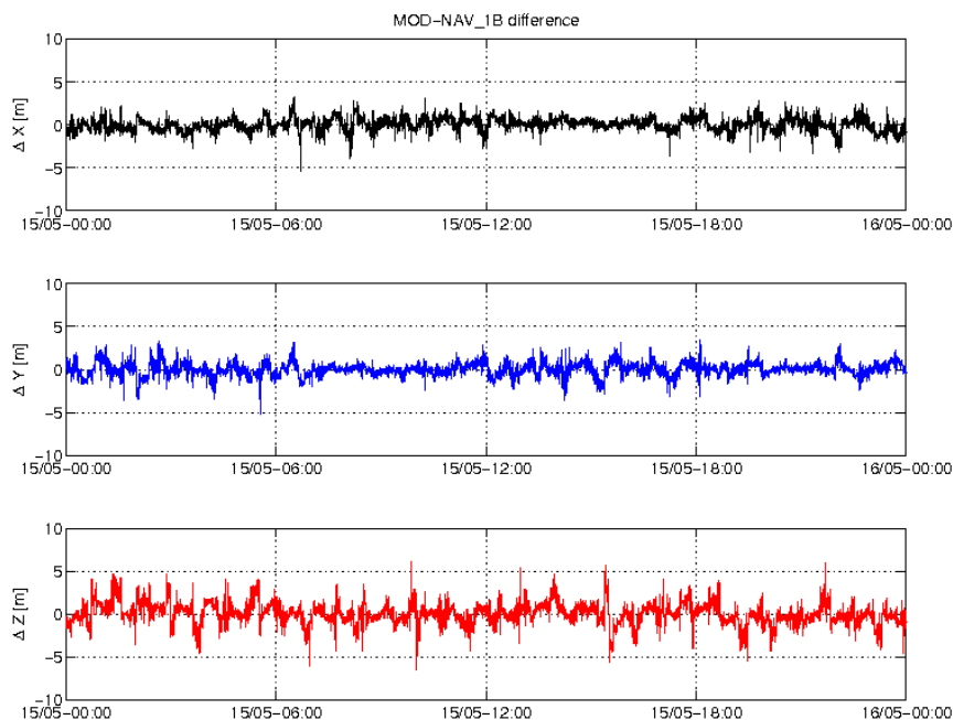
Figure 3-5: Difference MOD-GPSNAV, S/C C, 15/05. From top to bottom: X, Y and Z-axis
