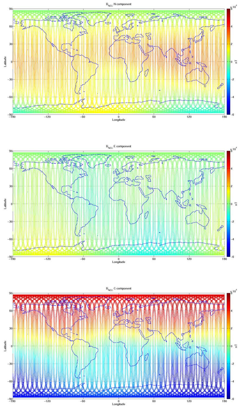
Figure 3-12: S/C C, world map plots of the geomagnetic field and components measured during monitoring period 15/05-21/05. From top to bottom: B_{NEC} components (North, East, and Centre) of magnetic field from VFM measurement.
