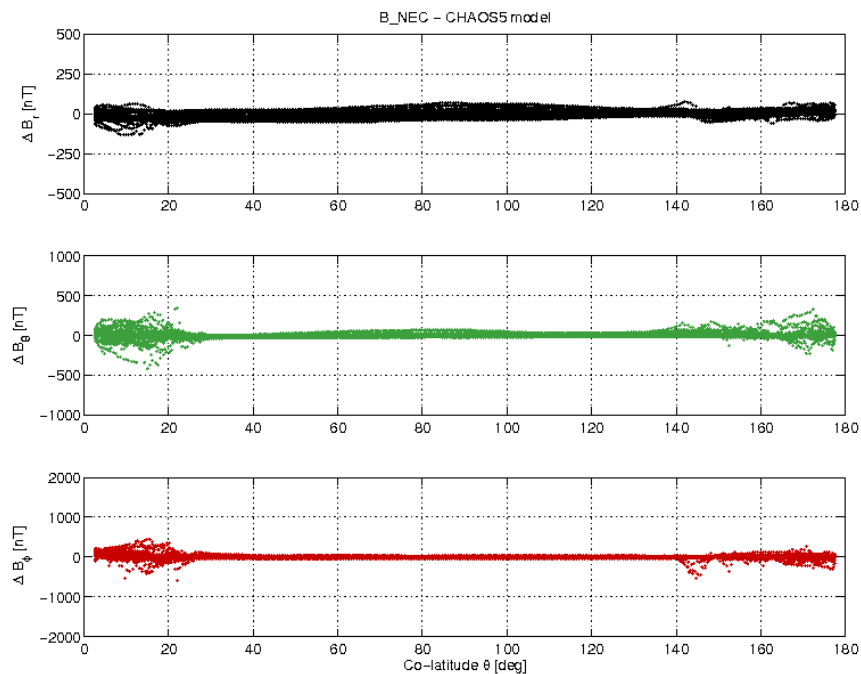
Figure 3-17: S/C A day 15/05 B_{NEC} - B_{Chaos5} vs colatitude.
