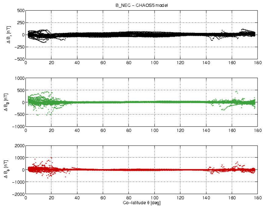
Figure 3-19: S/C B day 15/05 B_{NEC} - B_{Chaos} difference vs colatitude.
