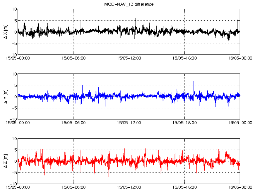
Figure 3-4: Difference MOD-GPSNAV, S/C B, 15/05. From top to bottom: X, Y and Z-axis
