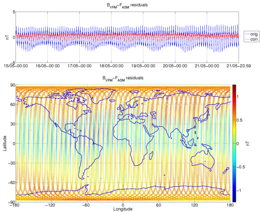
Figure 3-8: ASM-VFM residuals for S/C A, during monitoring period 15/05-21/05. In top figure are plotted: difference between |B_{VFM}| and F_{ASM} (without dB_{Sun} correction) (blue colour), and the residuals with dB_{Sun} corrections (red colour). In bottom figure residuals are presented on the world map.
