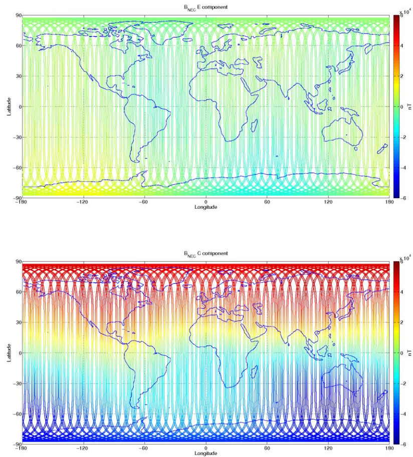
Figure 3-10: S/C A, world map plots of the geomagnetic field and components measured during monitoring period 15/05-21/05. From top to bottom: F-magnetic field from ASM measurement, B_{NEC} components (North, East, and Centre) of magnetic field from VFM measurement.
