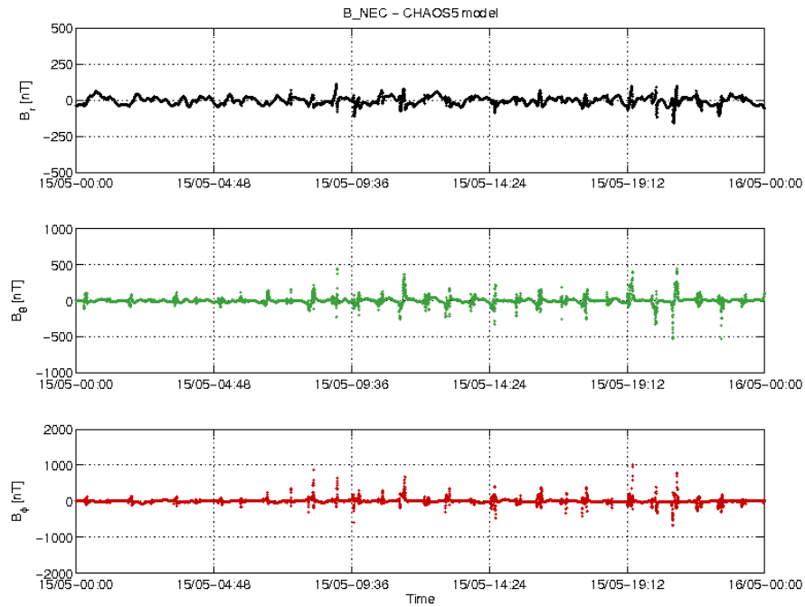
Figure 3-20: S/C B day 15/05 time series of B_{NEC} - B_{Chaos} residuals.
