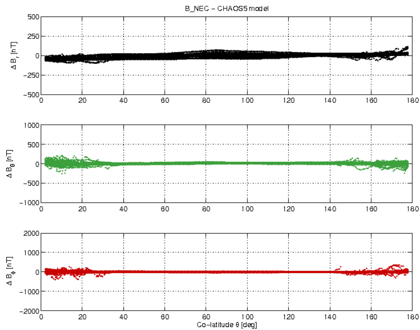
Figure 3-19: S/C B day 08/05 B_{NEC} - B_{Chaos} difference vs colatitude.
