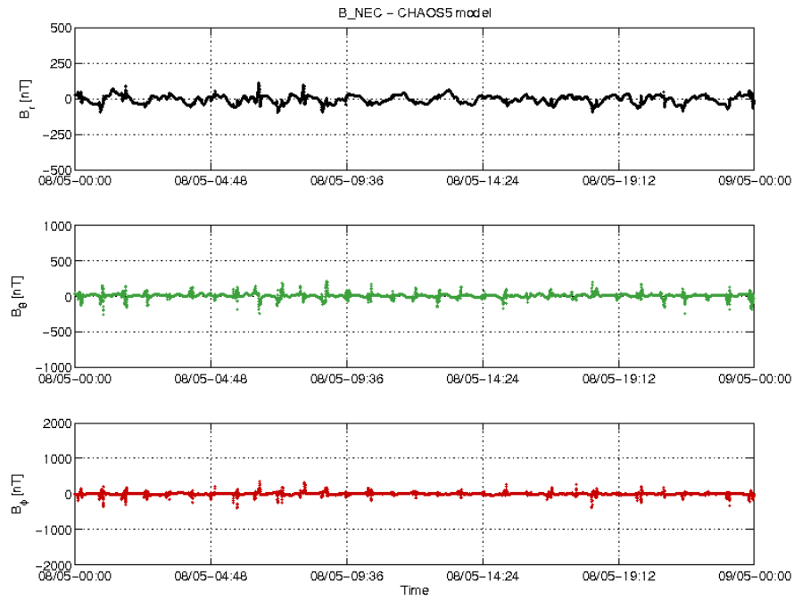
Figure 3-20: S/C B day 08/05 time series of B_{NEC} - B_{Chaos} residuals.
