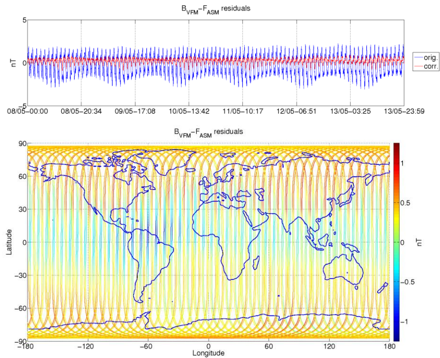
Figure 3-8: ASM-VFM residuals for S/C A, during monitoring period 08/05-14/05. In top figure are plotted: difference between |B_{VFM}| and F_{ASM} (without dB_{Sun} correction) (blue colour), and the residuals with dB_{Sun} corrections (red colour). In bottom figure residuals are presented on the world map.
