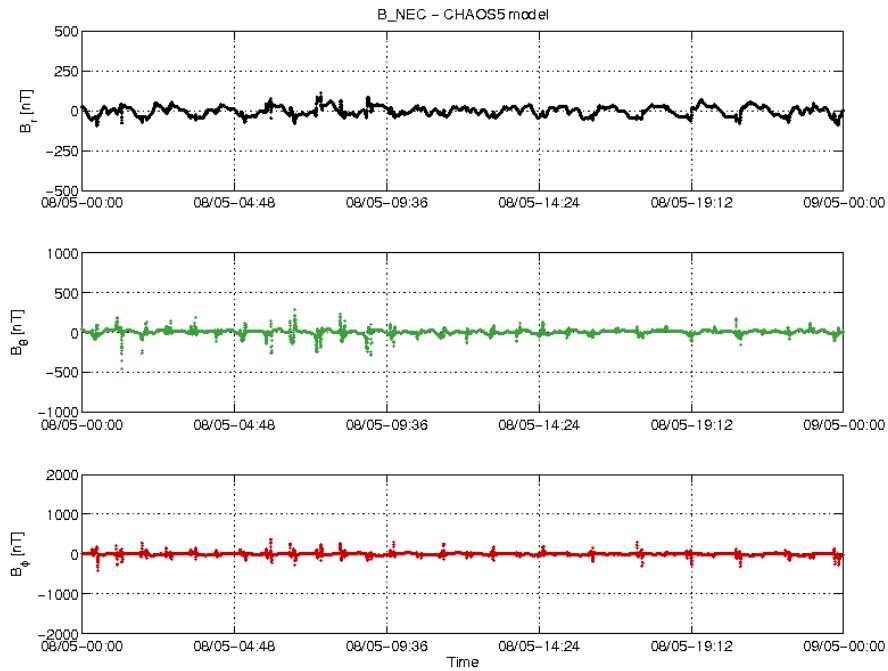
Figure 3-22: S/C C day 08/05 time series of B_{NEC} - B_{Chaos} residuals.
