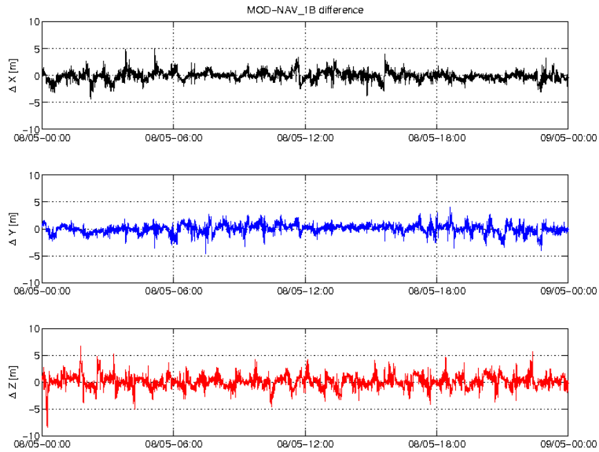
Figure 3-4: Difference MOD-GPSNAV, S/C B, 08/05. From top to bottom: X, Y and Z-axis
