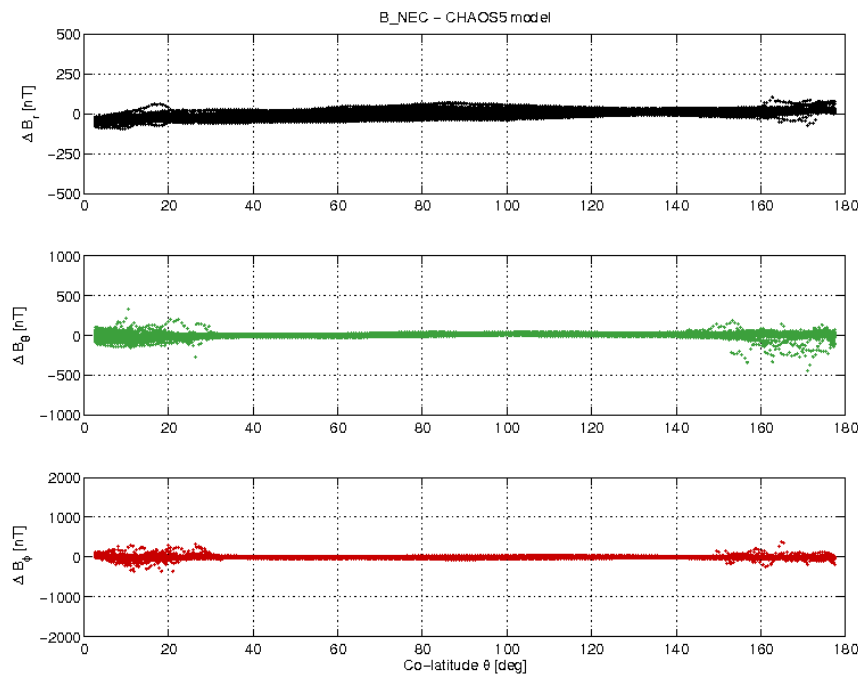
Figure 3-17: S/C A day 08/05 B_{NEC} - B_{Chaos5} vs colatitude.
