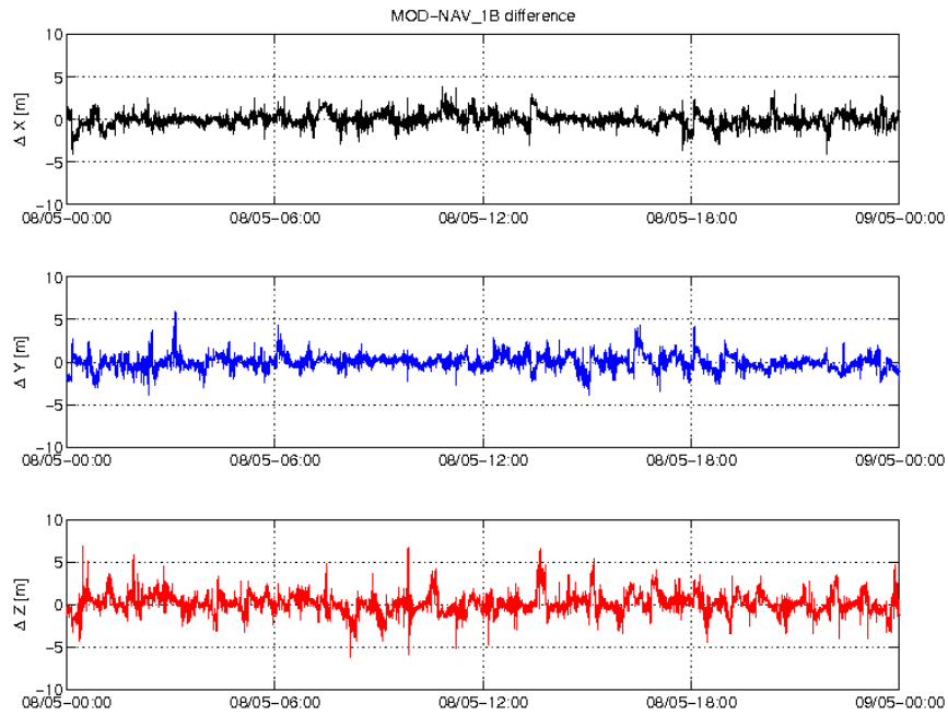
Figure 3-3: Difference MOD-GPSNAV, S/C A, 08/05. From top to bottom: X, Y and Z-axis
