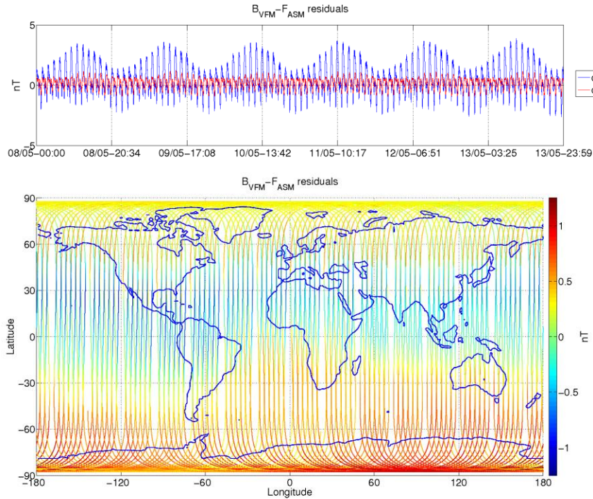
Figure 3-9: ASM-VFM residuals for S/C B, during monitoring period 08/05-14/05. In top figure are plotted: difference between |B\_VFM| and F\_ASM (without dB\_Sun correction) (blue colour), and the residuals with dB\_Sun corrections (red colour). In bottom figure residuals are presented on the world map.
