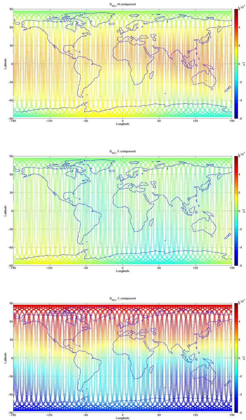
Figure 3-12: S/C C, world map plots of the geomagnetic field and components measured during monitoring period 08/05-14/05. From top to bottom: B NEC components (North, East, and Centre) of magnetic field from VFM measurement.
