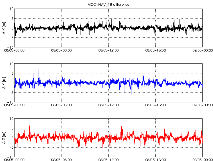
Figure 3-5: Difference MOD-GPSNAV, S/C C, 08/05. From top to bottom: X, Y and Z-axis
