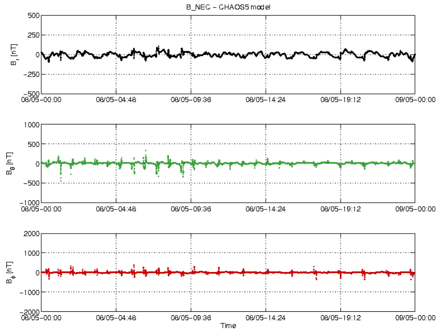
Figure 3-18: S/C A day 08/05: time series of B_{NEC} - B_{Chaos} residuals.
