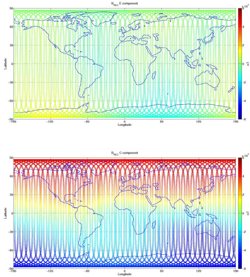
Figure 3-10: S/C A, world map plots of the geomagnetic field and components measured during monitoring period 08/05-14/05. From top to bottom: F-magnetic field from ASM measurement, B_{NEC} components (North, East, and Centre) of magnetic field from VFM measurement.
