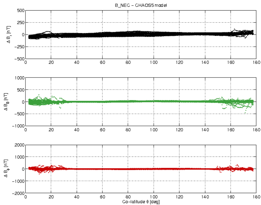
Figure 3-21: S/C C day 08/05 B_{NEC} - B_{Chaos} difference vs colatitude.
