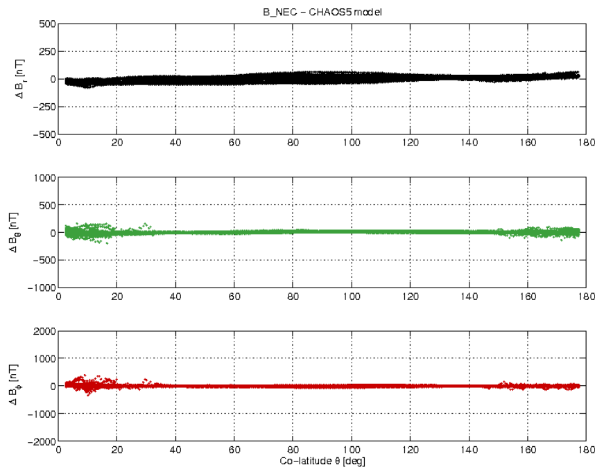
Figure 3-17: S/C A day 01/05 B_{NEC} - B_{Chaos} vs colatitude.
