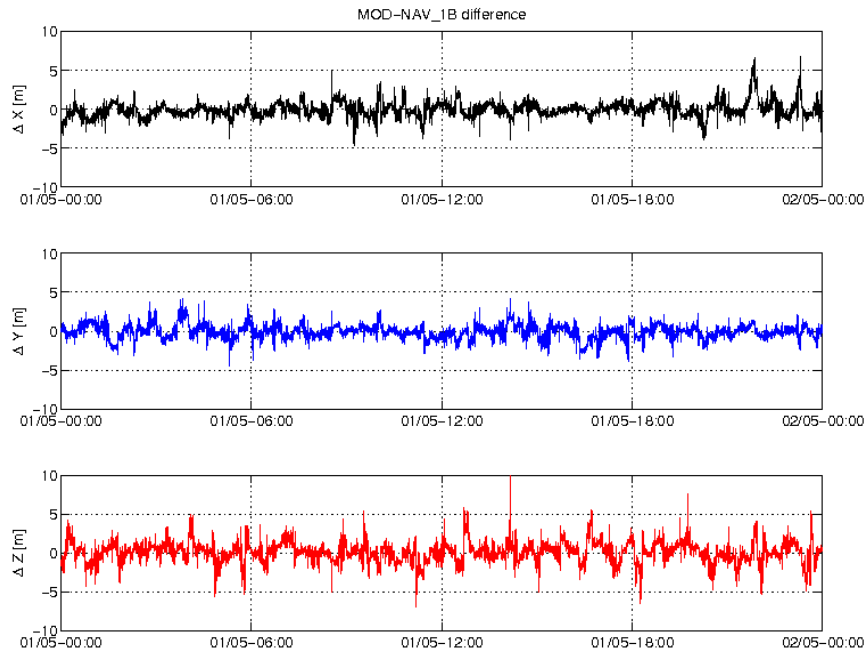
Figure 3-3: Difference MOD-GPSNAV, S/C A, 01/05. From top to bottom: X, Y and Z-axis
