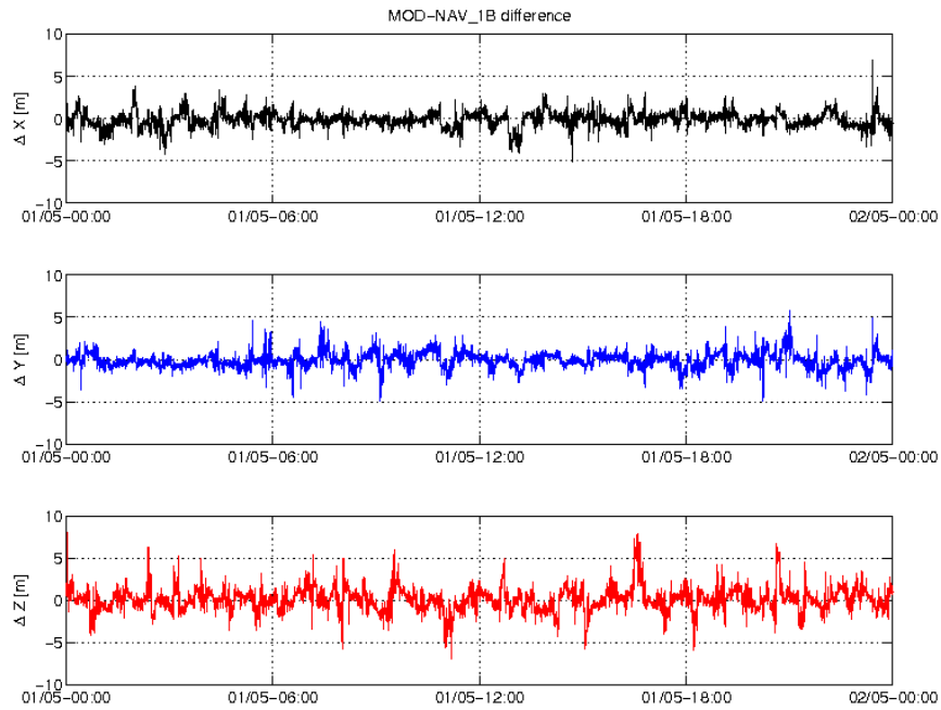
Figure 3-4: Difference MOD-GPSNAV, S/C B, 01/05. From top to bottom: X, Y and Z-axis
