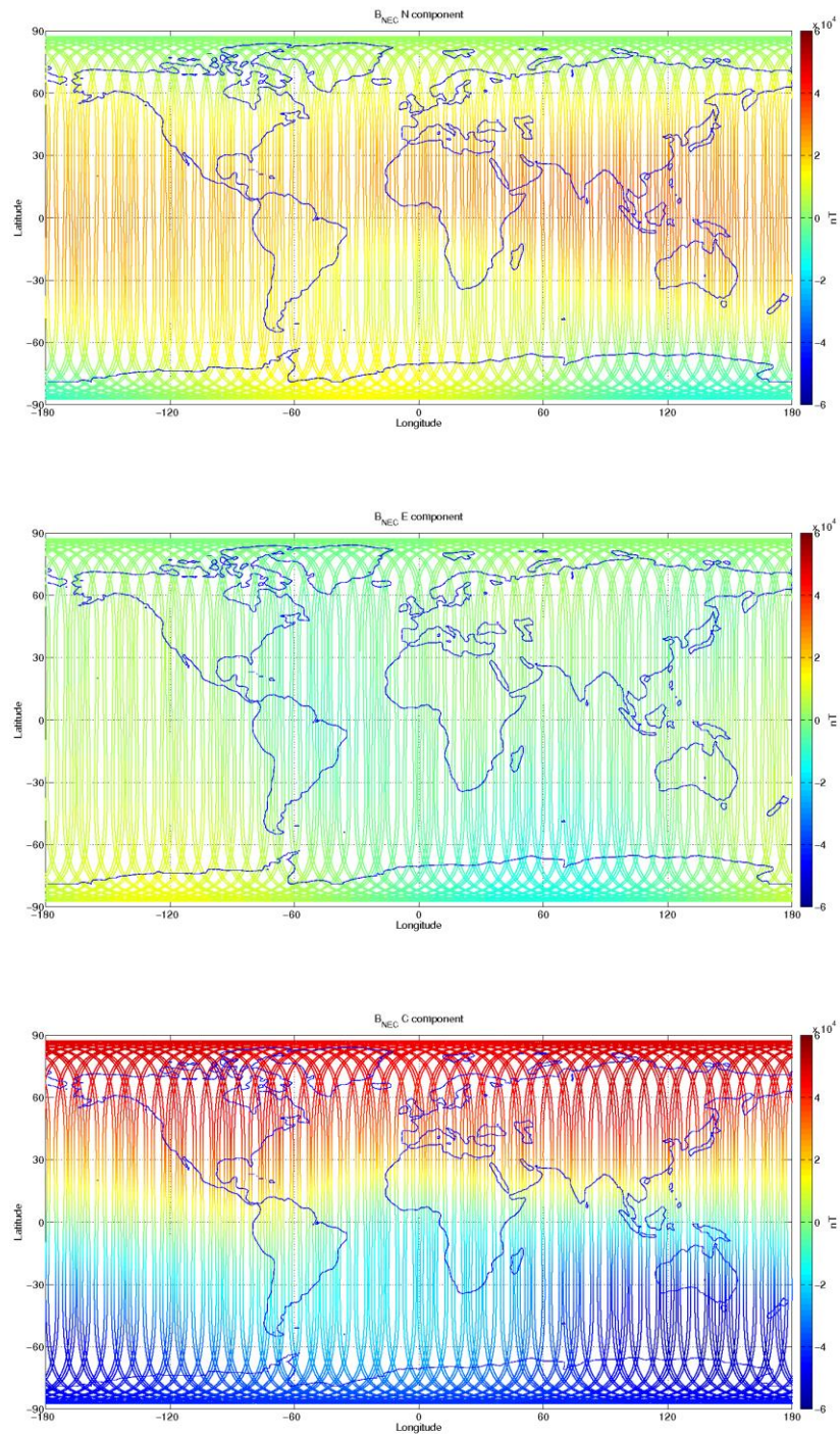
Figure 3-12: S/C C, world map plots of the geomagnetic field and components measured during monitoring period 01/05-07/05. From top to bottom: B NEC components (North, East, and Centre) of magnetic field from VFM measurement.
