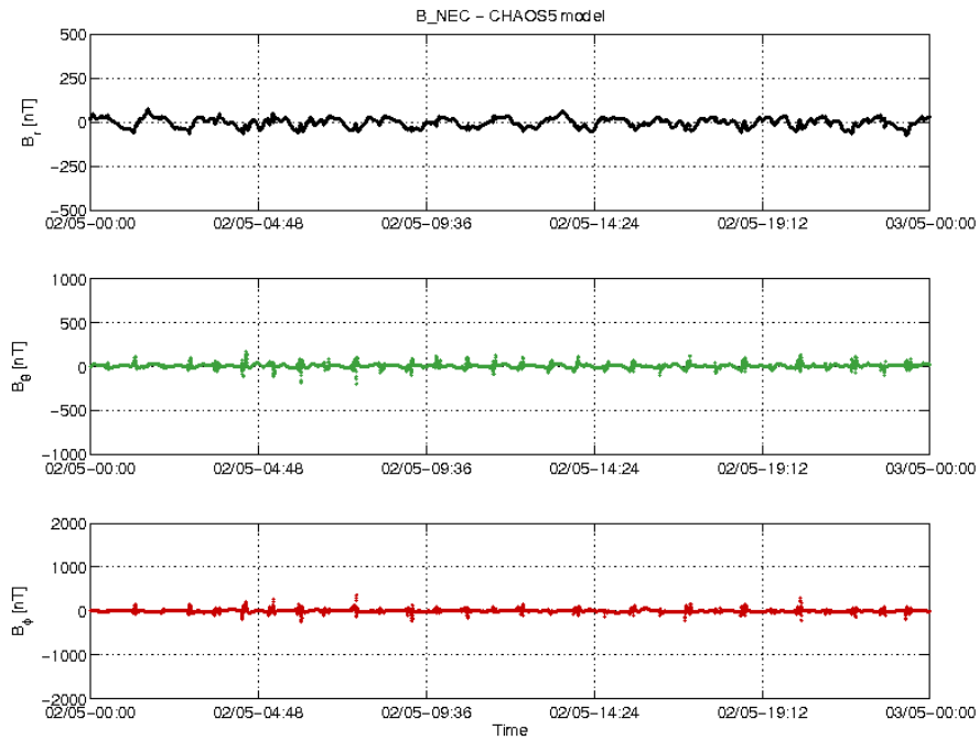
Figure 3-20: S/C B day 01/05 time series of B_{NEC} - B_{Chaos} residuals.
