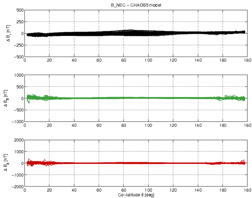
Figure 3-19: S/C B day 01/05 B_{NEC} - B_{Chaos} difference vs colatitude.
