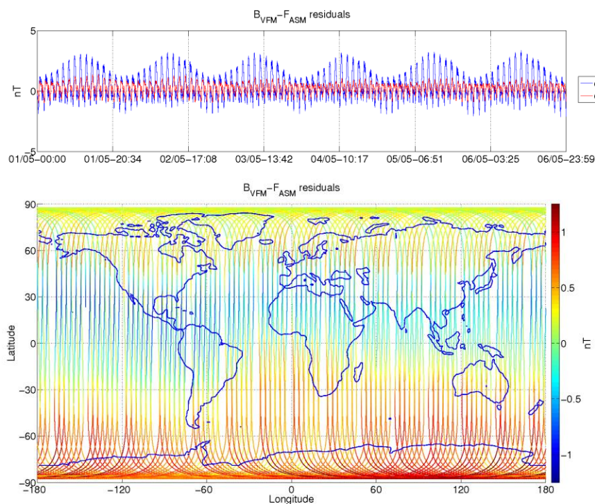
Figure 3-9: ASM-VFM residuals for S/C B, during monitoring period 01/05-07/05. In top figure are plotted: difference between |B_{VFM}| and F_{ASM} (without dB_{Sun} correction) (blue colour), and the residuals with dB_{Sun} corrections (red colour). In bottom figure residuals are presented on the world map.
