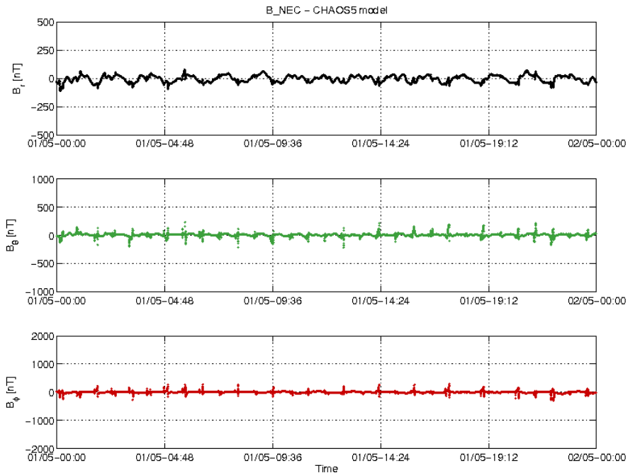
Figure 3-22: S/C C day 01/05 time series of B_{NEC} - B_{Chaos} residuals.
