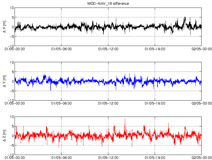
Figure 3-5: Difference MOD-GPSNAV, S/C C, 01/05. From top to bottom: X, Y and Z-axis
