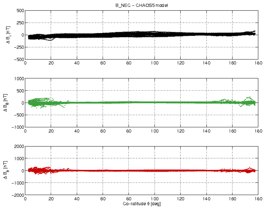
Figure 3-21: S/C C day 01/05 B_{NEC} - B_{Chaos} difference vs colatitude.
