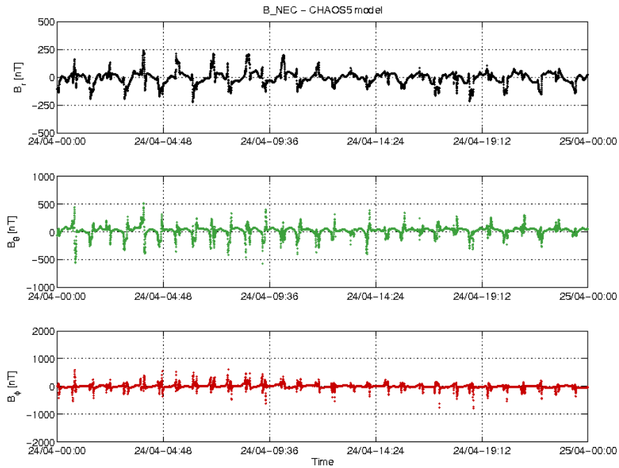
Figure 3-22: S/C C day 24/04 time series of B_{NEC} - B_{Chaos} residuals.
