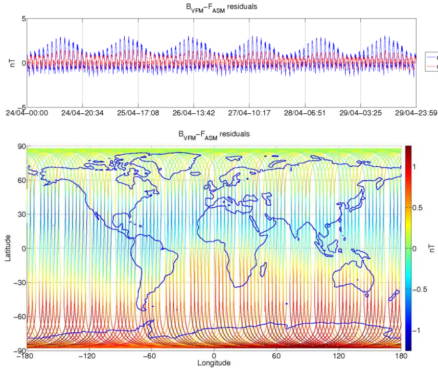
Figure 3-9: ASM-VFM residuals for S/C B, during monitoring period 24/04-30/04. In top figure are plotted: difference between |B\_VFM| and F\_ASM (without dB\_Sun correction) (blue colour), and the residuals with dB\_Sun corrections (red colour). In bottom figure residuals are presented on the world map.
