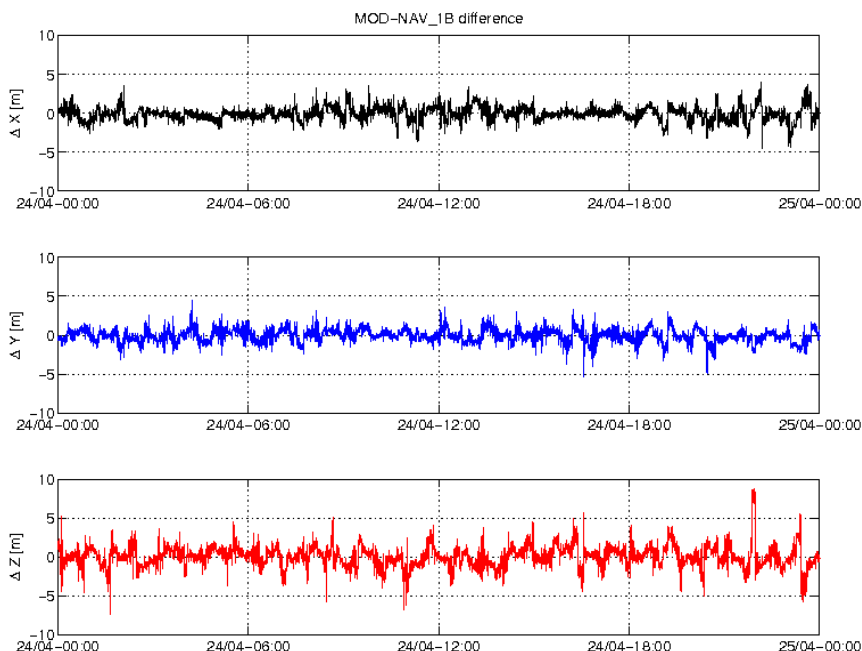
Figure 3-5: Difference MOD-GPSNAV, S/C C, 24/04. From top to bottom: X, Y and Z-axis
