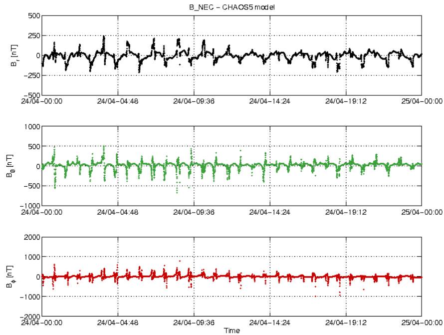
Figure 3-18: S/C A day 24/04: time series of B_{NEC} - B_{Chaos} residuals.
