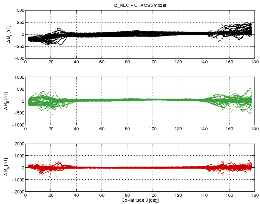
Figure 3-21: S/C C day 24/04 B_{NEC} - B_{Chaos} difference vs colatitude.
