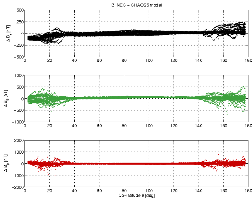
Figure 3-17: S/C A day 24/04 B_{NEC} - B_{Chaos5} vs colatitude.
