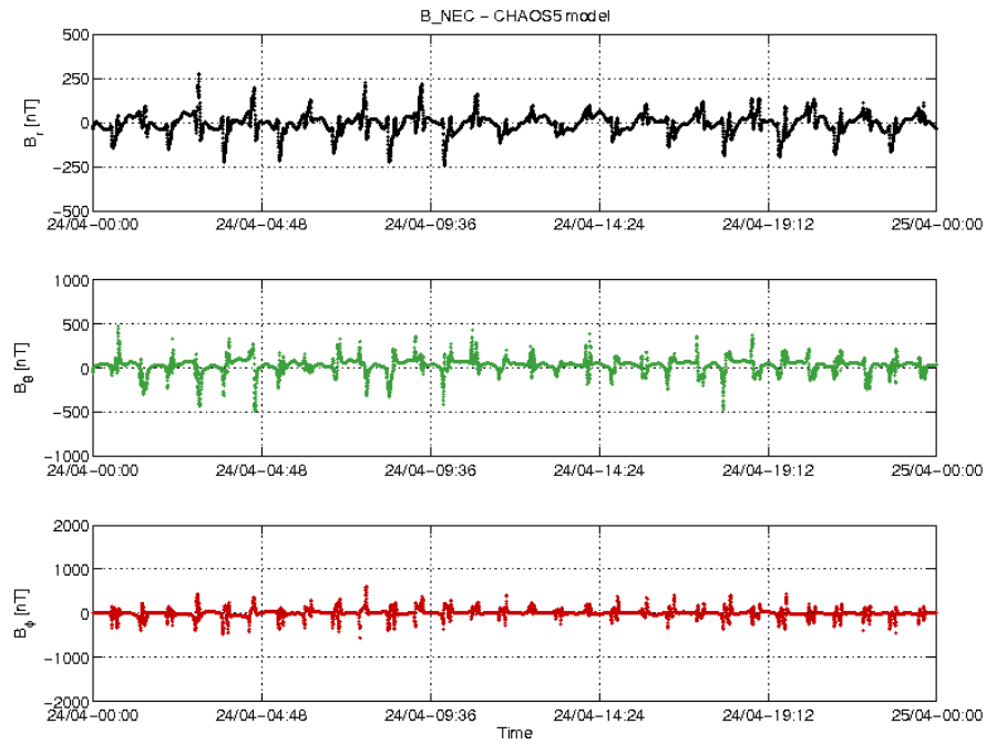
Figure 3-20: S/C B day 24/04 time series of B_{NEC} - B_{Chaos} residuals.
