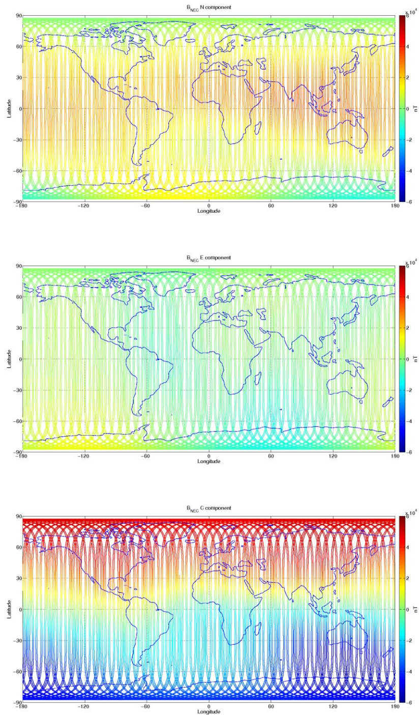
Figure 3-12: S/C C, world map plots of the geomagnetic field and components measured during monitoring period 24/04-30/04. From top to bottom: B NEC components (North, East, and Centre) of magnetic field from VFM measurement.
