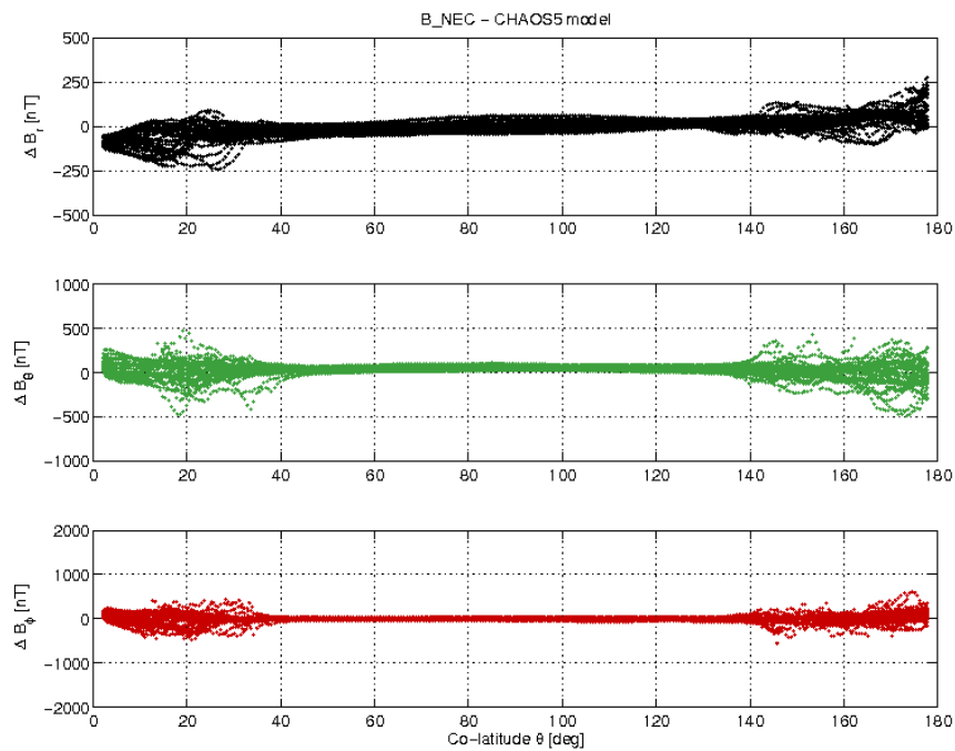
Figure 3-19: S/C B day 24/04 B_{NEC} - B_{Chaos} difference vs colatitude.
