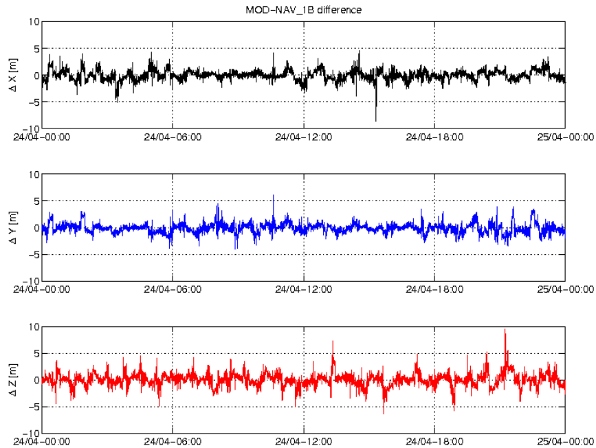
Figure 3-4: Difference MOD-GPSNAV, S/C B, 24/04. From top to bottom: X, Y and Z-axis
