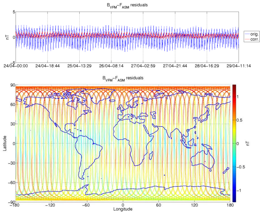
Figure 3-8: ASM-VFM residuals for S/C A, during monitoring period 24/04-30/04. In top figure are plotted: difference between |B_{VFM}| and F_{ASM} (without dB_{Sun} correction) (blue colour), and the residuals with dB_{Sun} corrections (red colour). In bottom figure residuals are presented on the world map.
