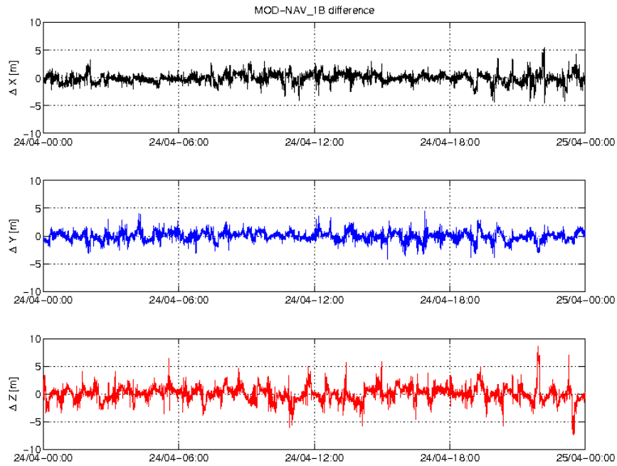
Figure 3-3: Difference MOD-GPSNAV, S/C A, 24/04. From top to bottom: X, Y and Z-axis
