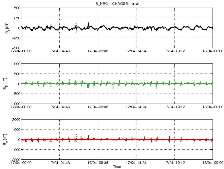
Figure 3-18: S/C A day 17/04: time series of B_{NEC} - B_{Chaos} residuals.
