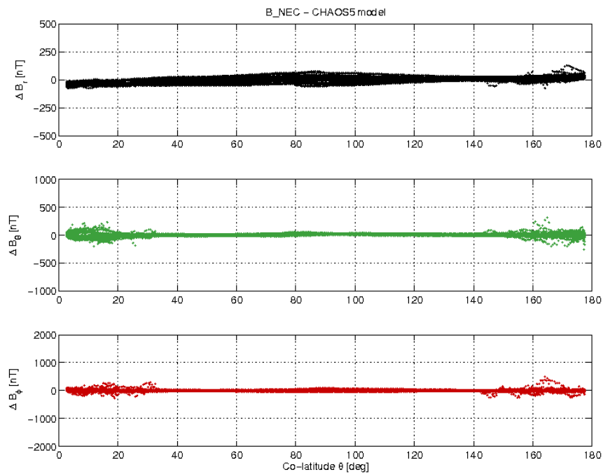
Figure 3-21: S/C C day 17/04 B_{NEC} - B_{Chaos} difference vs colatitude.
