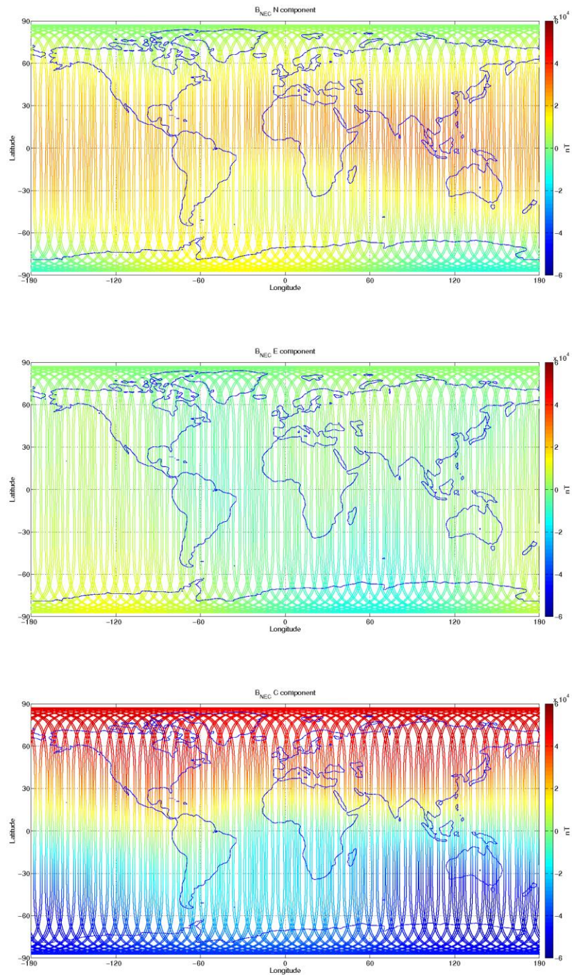
Figure 3-12: S/C C, world map plots of the geomagnetic field and components measured during monitoring period 17/04-23/04. From top to bottom: B NEC components (North, East, and Centre) of magnetic field from VFM measurement.
