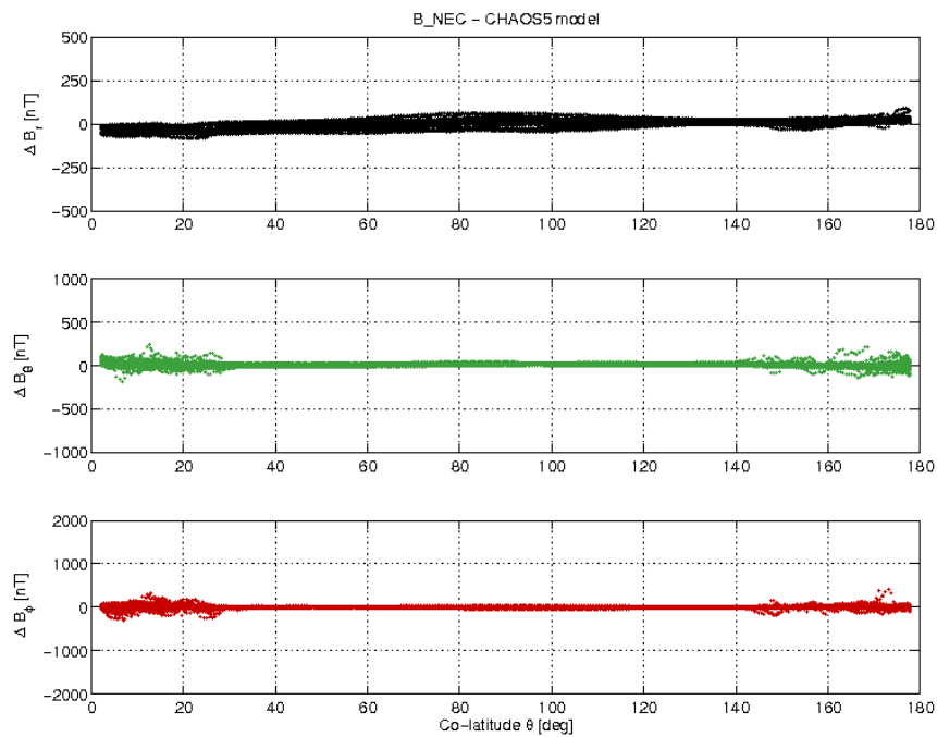
Figure 3-19: S/C B day 17/04 B_{NEC} - B_{Chaos} difference vs colatitude.
