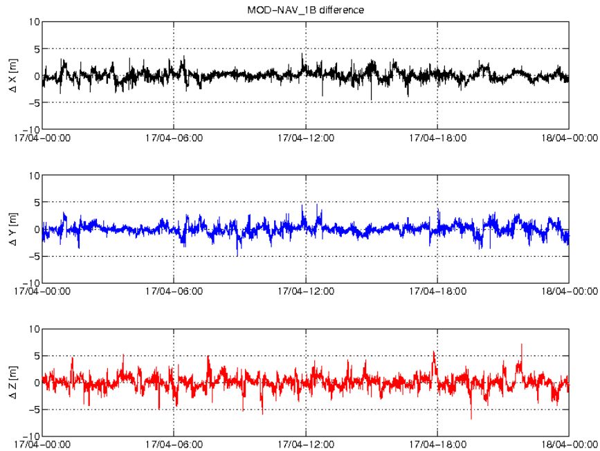
Figure 3-4: Difference MOD-GPSNAV, S/C B, 17/04. From top to bottom: X, Y and Z-axis
