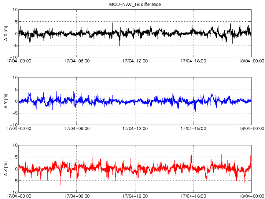
Figure 3-3: Difference MOD-GPSNAV, S/C A, 17/04. From top to bottom: X, Y and Z-axis
