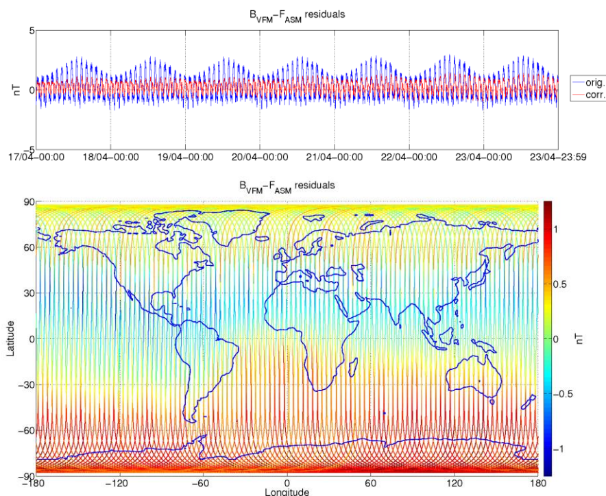
Figure 3-9: ASM-VFM residuals for S/C B, during monitoring period 17/04-23/04. In top figure are plotted: difference between |B_{VFM}| and F_{ASM} (without dB_{Sun} correction) (blue colour), and the residuals with dB_{Sun} corrections (red colour). In bottom figure residuals are presented on the world map.
