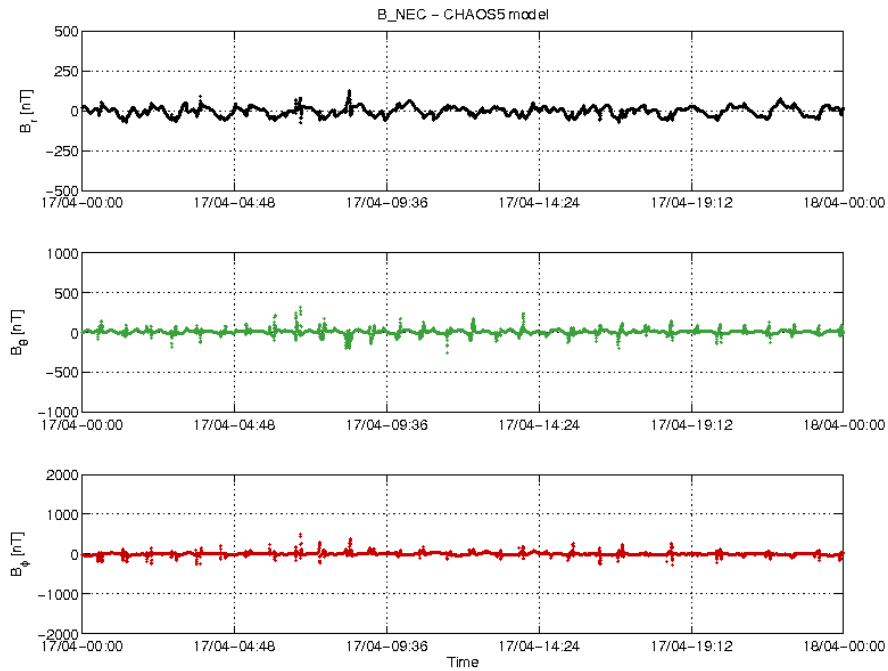
Figure 3-22: S/C C day 17/04 time series of B_{NEC} - B_{Chaos} residuals.
