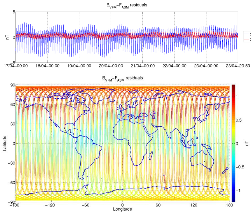
Figure 3-8: ASM-VFM residuals for S/C A, during monitoring period 17/04-23/04. In top figure are plotted: difference between |B_{VFM}| and F_{ASM} (without dB_Sun correction) (blue colour), and the residuals with dB_Sun corrections (red colour). In bottom figure residuals are presented on the world map.
