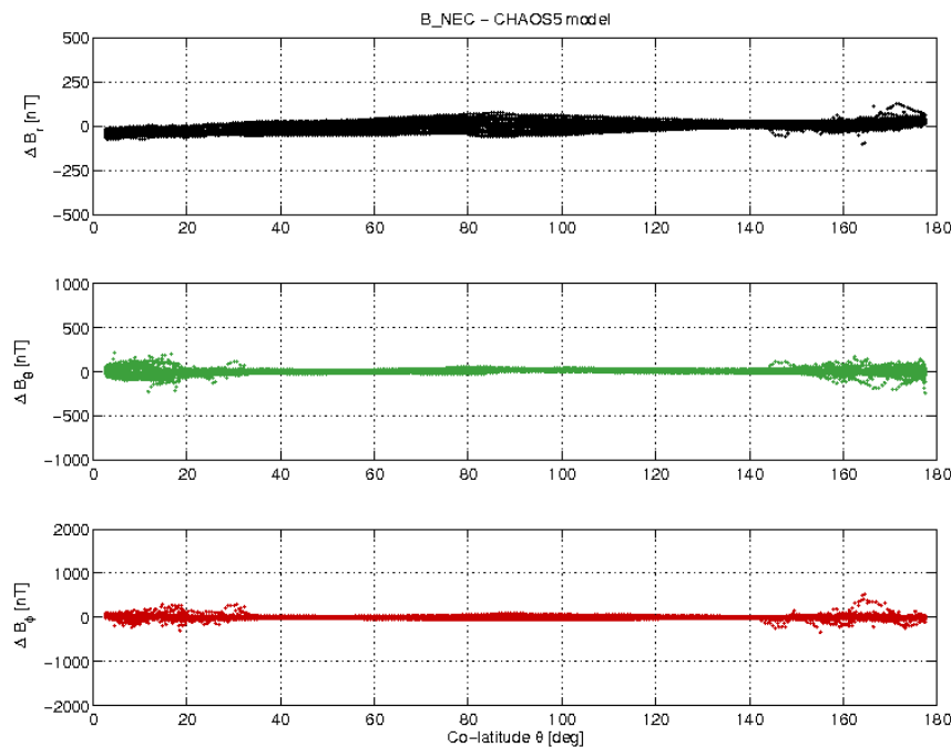
Figure 3-17: S/C A day 17/04 B_{NEC} - B_{Chaos} vs colatitude.
