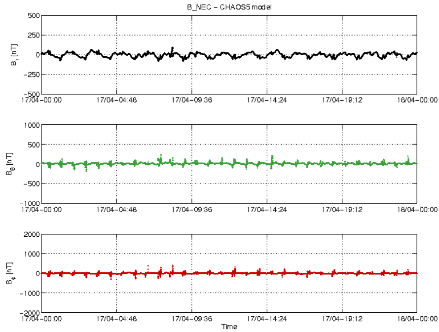
Figure 3-20: S/C B day 17/04 time series of B_{NEC} - B_{Chaos} residuals.
