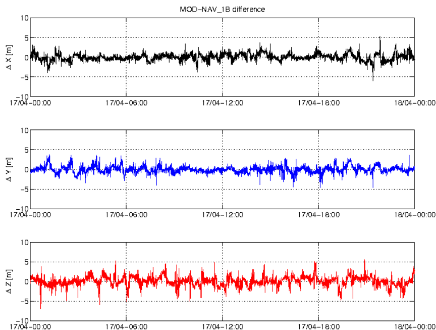
Figure 3-5: Difference MOD-GPSNAV, S/C C, 17/04. From top to bottom: X, Y and Z-axis
