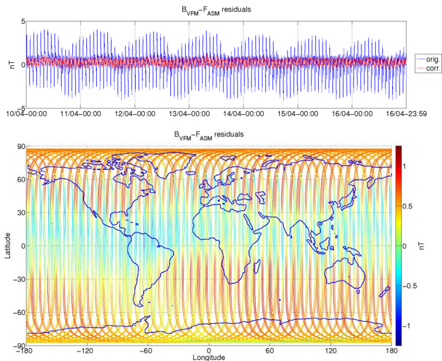
Figure 3-8: ASM-VFM residuals for S/C A, during monitoring period 10/04-16/04. In top figure are plotted: difference between |B_{VFM}| and F_{ASM} (without dB_{Sun} correction) (blue colour), and the residuals with dB_{Sun} corrections (red colour). In bottom figure residuals are presented on the world map.
