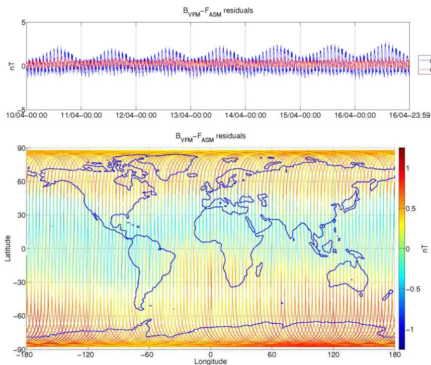
Figure 3-9: ASM-VFM residuals for S/C B, during monitoring period 10/04-16/04. In top figure are plotted: difference between |B_{VFM}| and F_{ASM} (without dB_{Sun} correction) (blue colour), and the residuals with dB_{Sun} corrections (red colour). In bottom figure residuals are presented on the world map.
