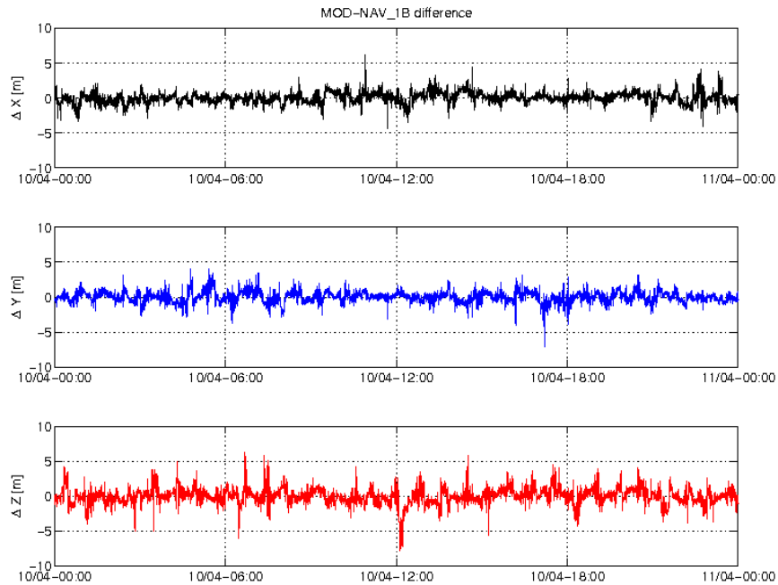
Figure 3-3: Difference MOD-GPSNAV, S/C A, 10/04. From top to bottom: X, Y and Z-axis
