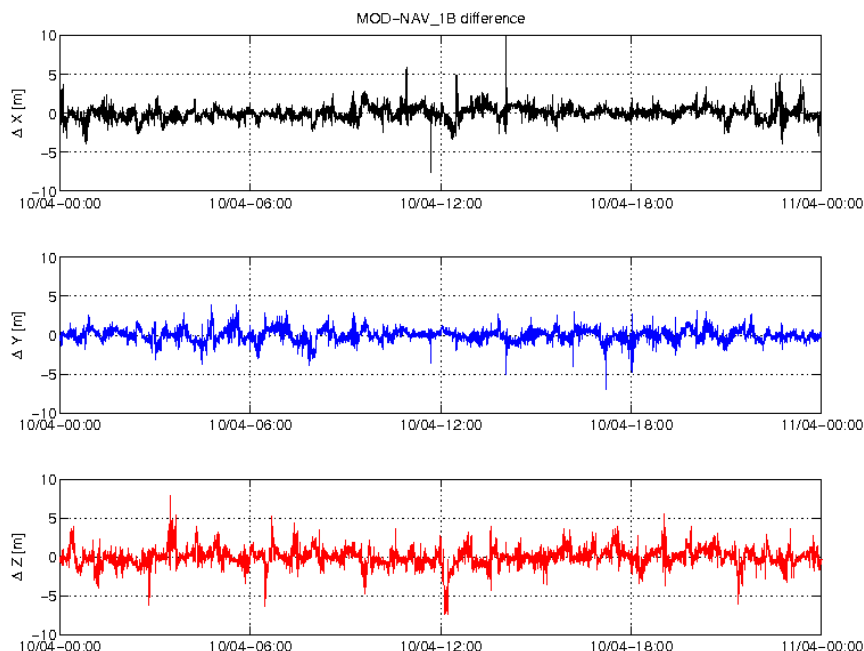
Figure 3-5: Difference MOD-GPSNAV, S/C C, 10/04. From top to bottom: X, Y and Z-axis
