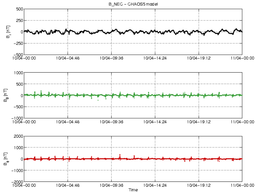
Figure 3-18: S/C A day 10/04: time series of B_{NEC} - B_{Chaos} residuals.
