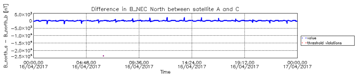
Figure 3-14: Difference in B_{NEC} North component between S/C A and S/C C.
