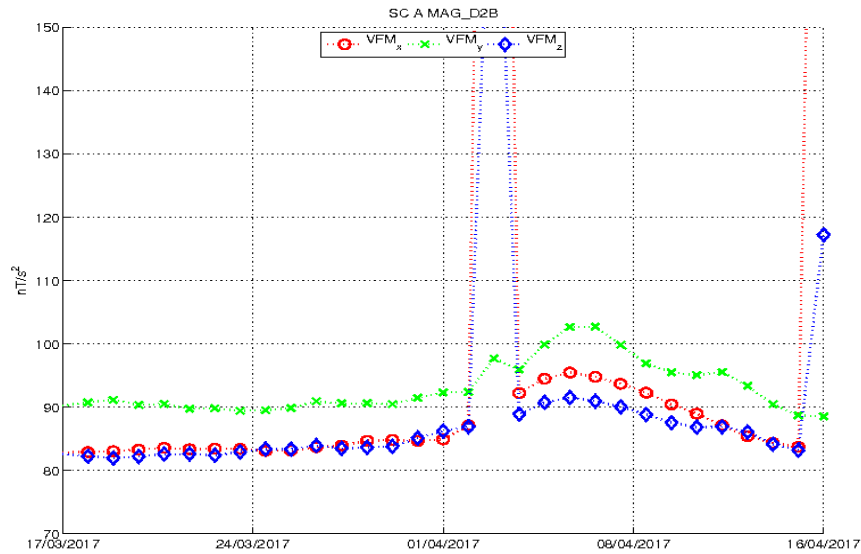
Figure 3-23: Plot of standard deviation of B components in VFM frames.
