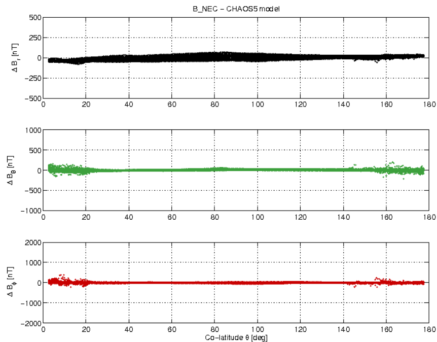
Figure 3-17: S/C A day 10/04 B_{NEC} - B_{Chaos} vs colatitude.
