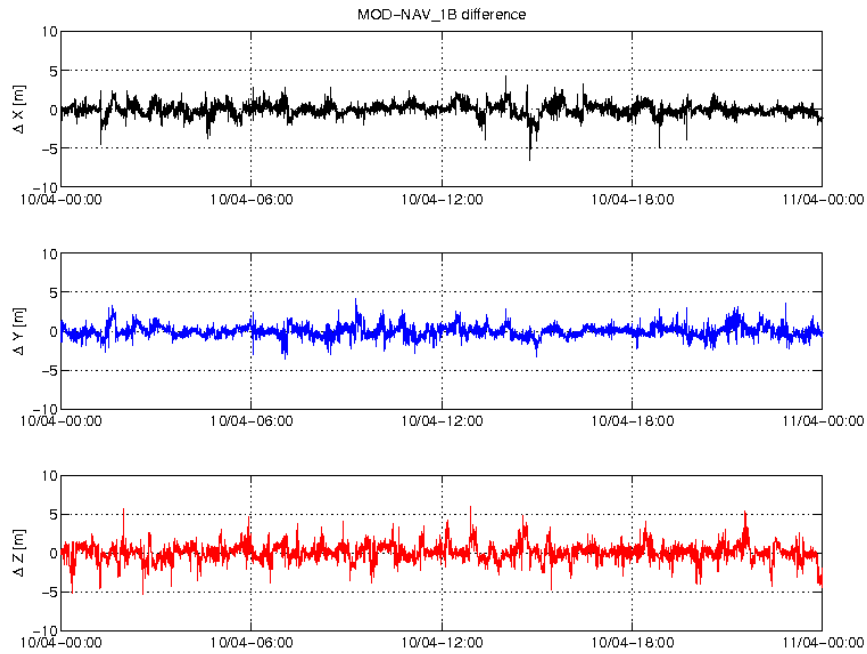
Figure 3-4: Difference MOD-GPSNAV, S/C B, 10/04. From top to bottom: X, Y and Z-axis
