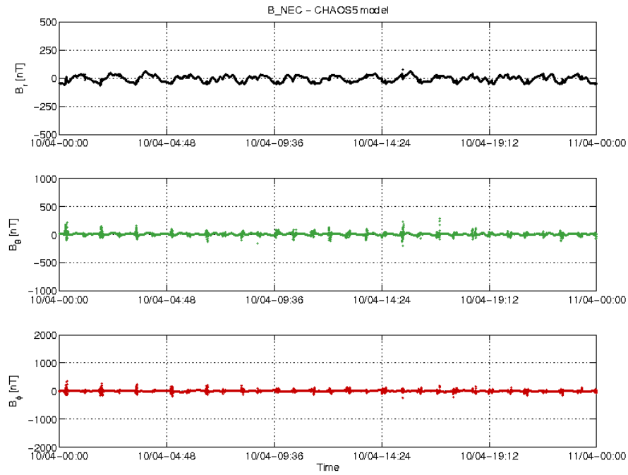
Figure 3-20: S/C B day 10/04 time series of B_{NEC} - B_{Chaos} residuals.
