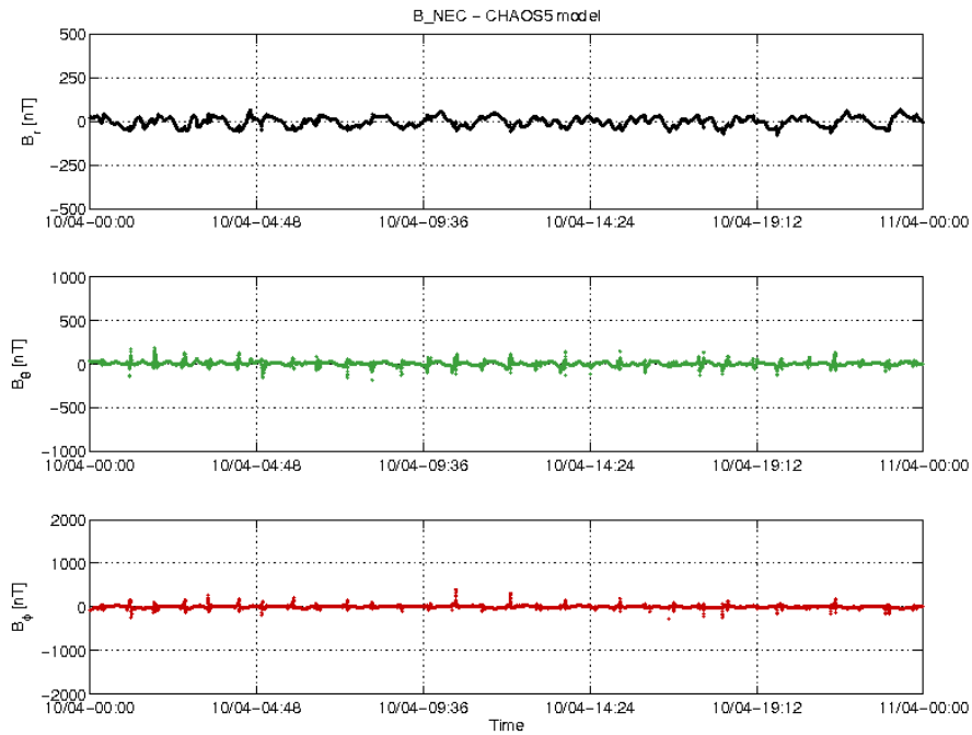
Figure 3-22: S/C C day 10/04 time series of B_{NEC} - B_{Chaos} residuals.
