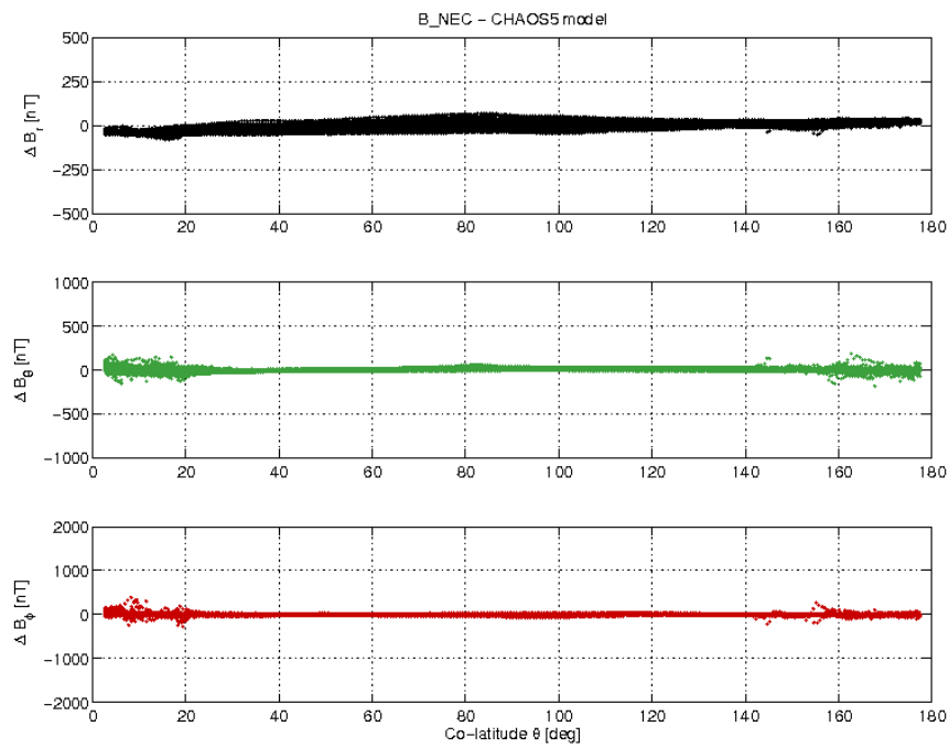
Figure 3-21: S/C C day 10/04 B_{NEC} - B_{Chaos} difference vs colatitude.
