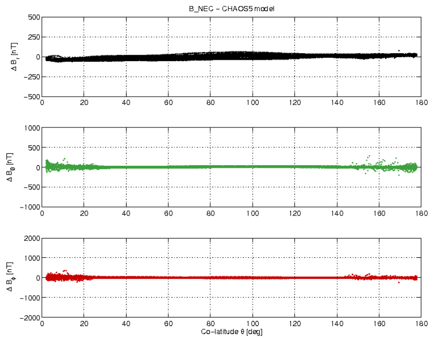
Figure 3-19: S/C B day 10/04 B_{NEC} - B_{Chaos} difference vs colatitude.
