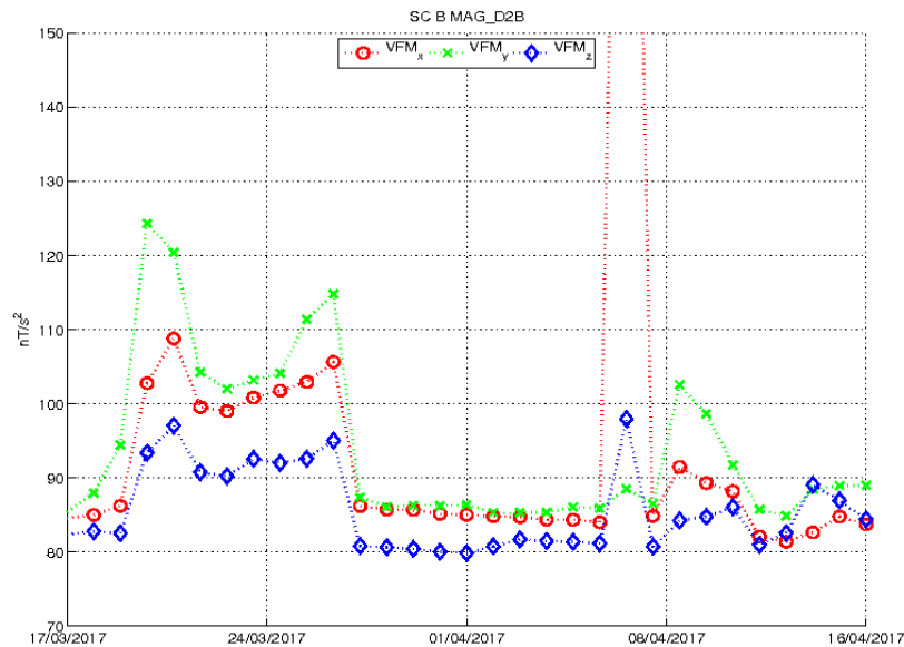
Figure 3-24: Plot of standard deviation of B components in VFM frames.
