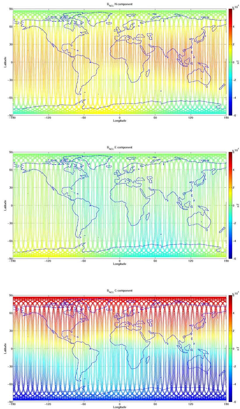
Figure 3-12: S/C C, world map plots of the geomagnetic field and components measured during monitoring period 10/04-16/04. From top to bottom: B_{NEC} components (North, East, and Centre) of magnetic field from VFM measurement.
