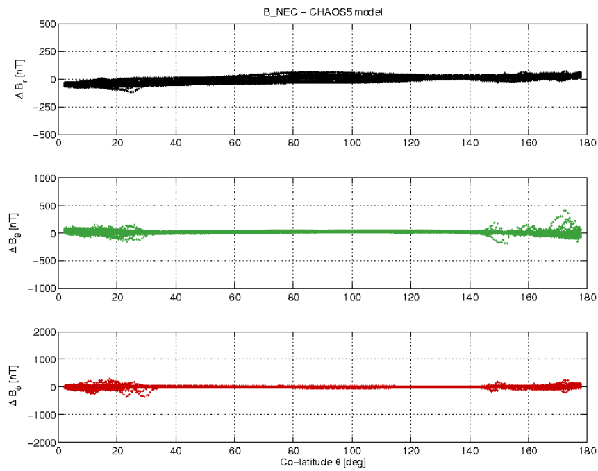
Figure 3-19: S/C B day 03/04 B_{NEC} - B_{Chaos} difference vs colatitude.
