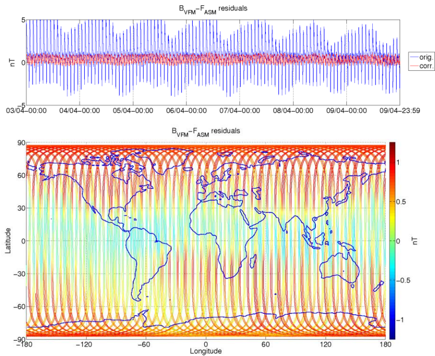
Figure 3-8: ASM-VFM residuals for S/C A, during monitoring period 03/04-09/04. In top figure are plotted: difference between |B VFM | and F ASM (without dB Sun correction) (blue colour), and the residuals with dB Sun corrections (red colour). In bottom figure residuals are presented on the world map.
