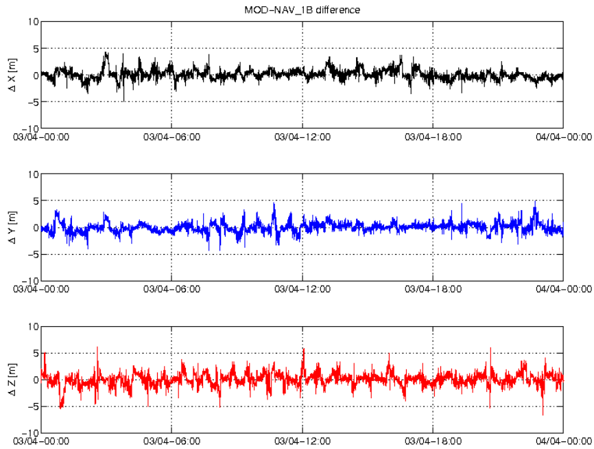
Figure 3-4: Difference MOD-GPSNAV, S/C B, 03/04. From top to bottom: X, Y and Z-axis
