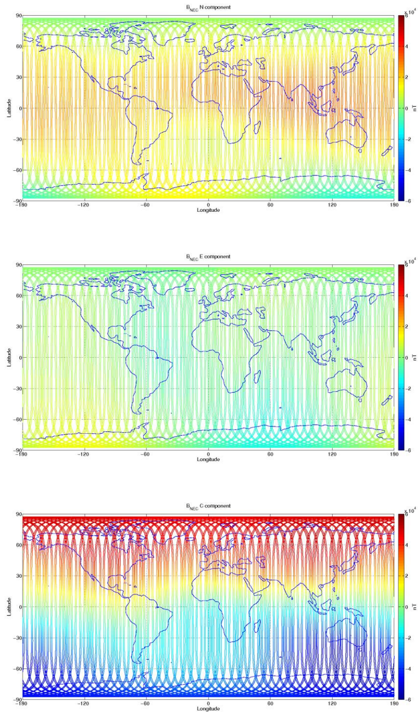
Figure 3-12: S/C C, world map plots of the geomagnetic field and components measured during monitoring period 03/04-09/04. From top to bottom: B_{NEC} components (North, East, and Centre) of magnetic field from VFM measurement.
