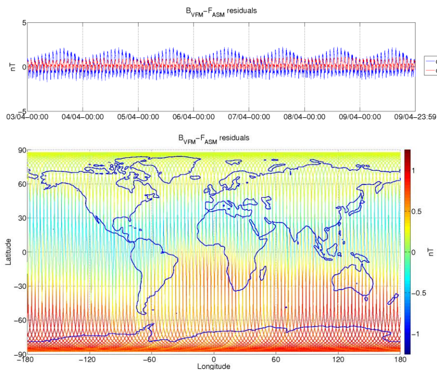
Figure 3-9: ASM-VFM residuals for S/C B, during monitoring period 03/04-09/04. In top figure are plotted: difference between |B_{VFM}| and F_{ASM} (without dB_{Sun} correction) (blue colour), and the residuals with dB_{Sun} corrections (red colour). In bottom figure residuals are presented on the world map.
