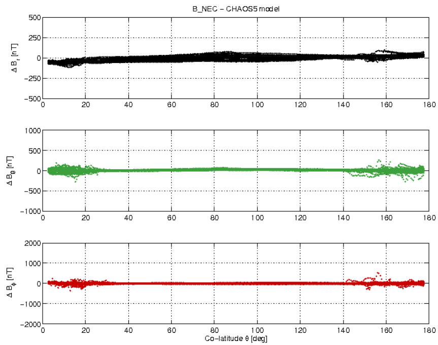
Figure 3-21: S/C C day 03/04 B_{NEC} - B_{Chaos} difference vs colatitude.
