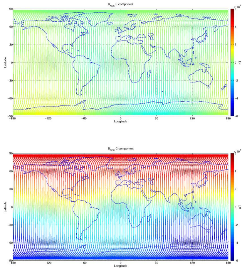
Figure 3-11: S/C B, world map plots of the geomagnetic field and components measured during monitoring period 03/04-09/04. From top to bottom: F-magnetic field from ASM measurement, B_{NEC} components (North, East, and Centre) of magnetic field from VFM measurement.
