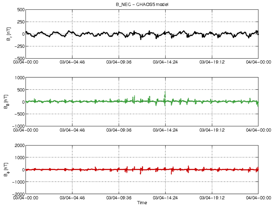
Figure 3-20: S/C B day 03/04 time series of B_{NEC} - B_{Chaos} residuals.
