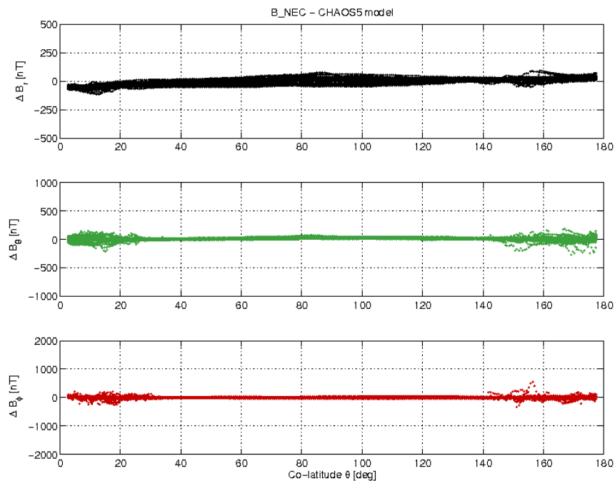
Figure 3-17: S/C A day 03/04 B_{NEC} - B_{Chaos} vs colatitude.
