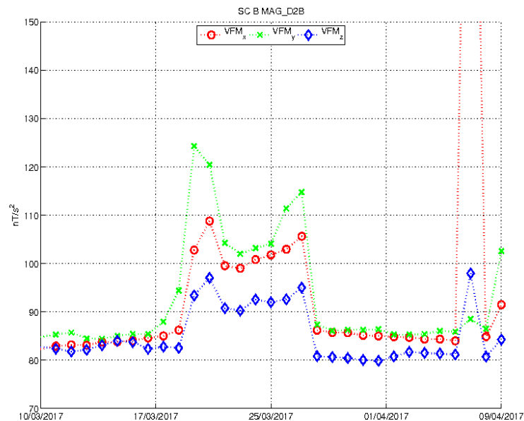
Figure 3-24: Plot of standard deviation of B components in VFM frames.
