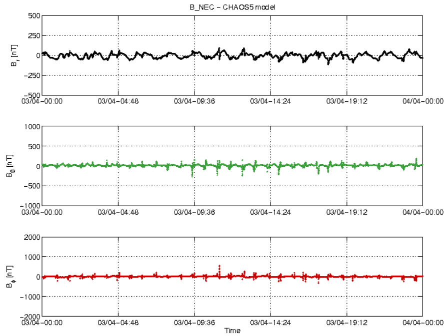
Figure 3-18: S/C A day 03/04: time series of B_{NEC} - B_{Chaos} residuals.
