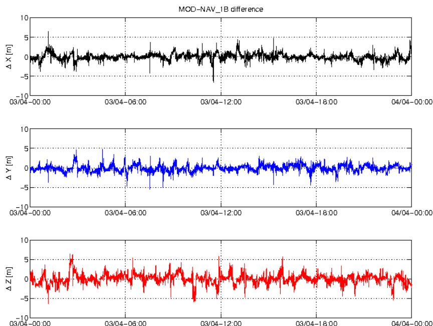
Figure 3-5: Difference MOD-GPSNAV, S/C C, 03/04. From top to bottom: X, Y and Z-axis
