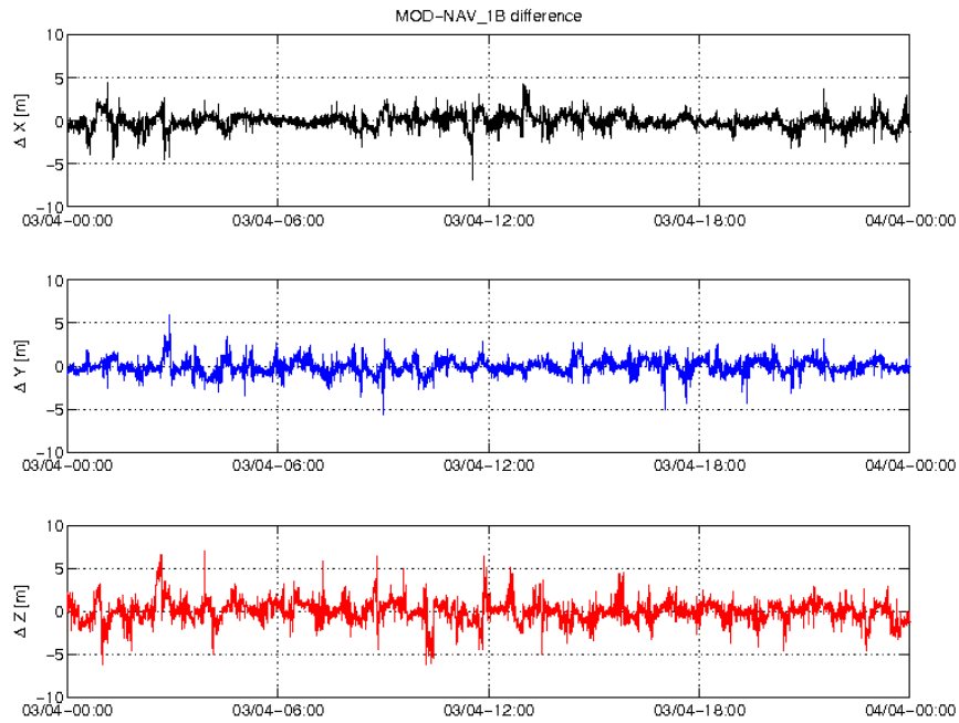
Figure 3-3: Difference MOD-GPSNAV, S/C A, 03/04. From top to bottom: X, Y and Z-axis
