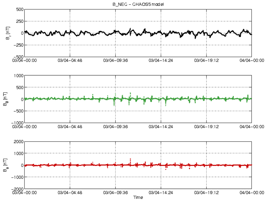
Figure 3-22: S/C C day 03/04 time series of B_{NEC} - B_{Chaos} residuals.
