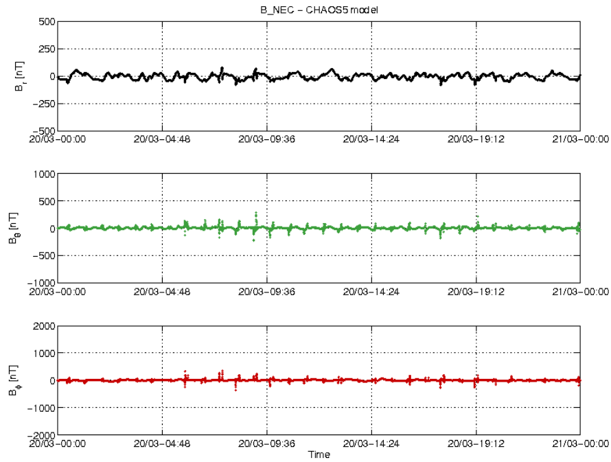
Figure 3-18: S/C A day 20/03: time series of B_{NEC} - B_{Chaos} residuals.
