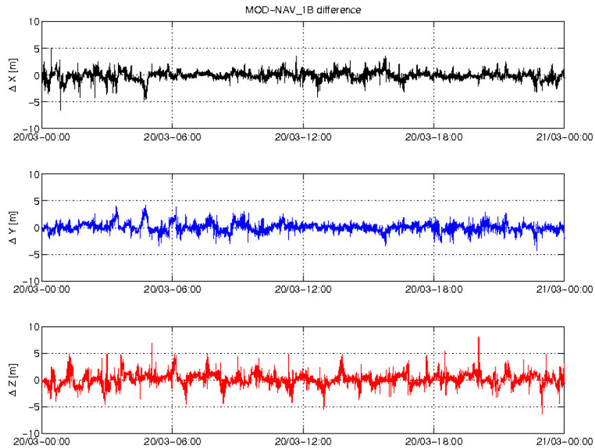
Figure 3-3: Difference MOD-GPSNAV, S/C A, 20/03. From top to bottom: X, Y and Z-axis
