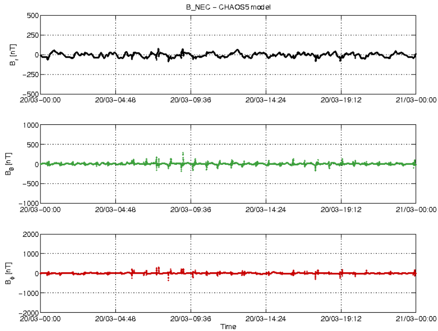
Figure 3-22: S/C C day 20/03 time series of B_{NEC} - B_{Chaos} residuals.
