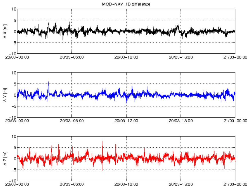
Figure 3-4: Difference MOD-GPSNAV, S/C B, 20/03. From top to bottom: X, Y and Z-axis
