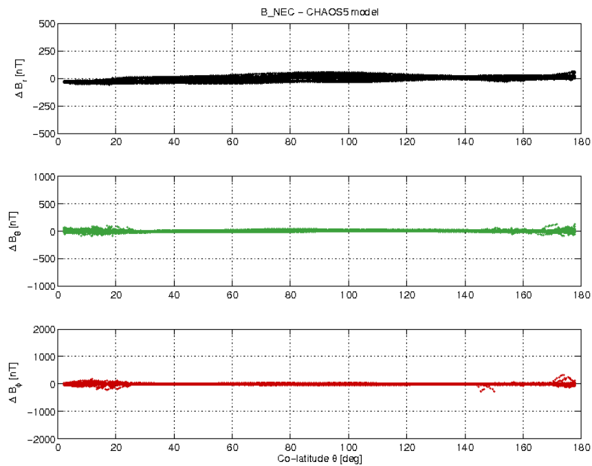
Figure 3-19: S/C B day 20/03 B_{NEC} - B_{Chaos} difference vs colatitude.
