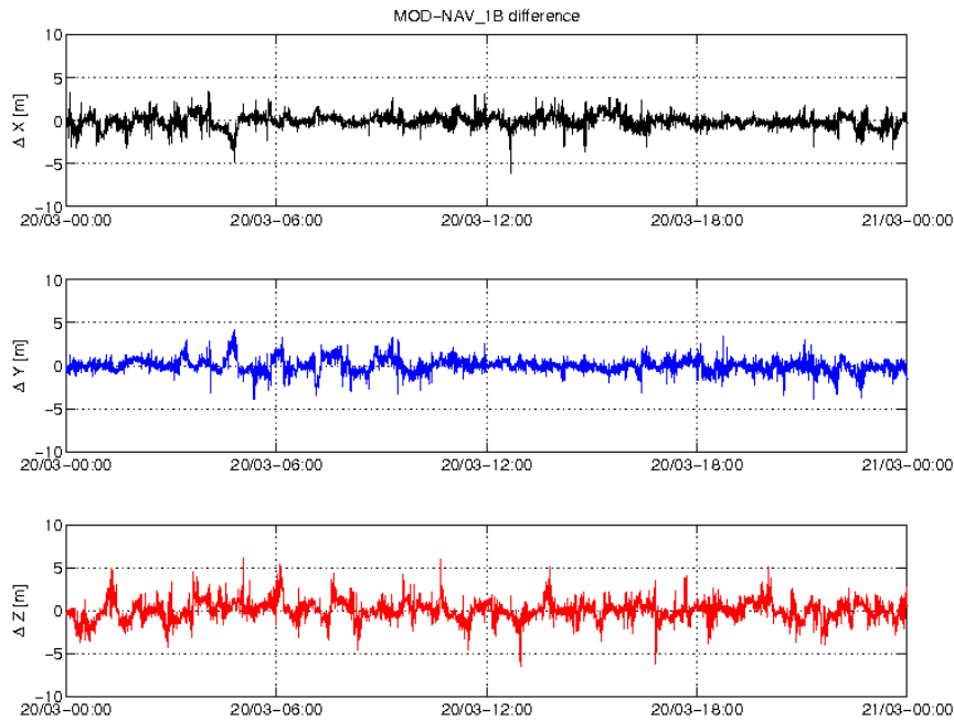
Figure 3-5: Difference MOD-GPSNAV, S/C C, 20/03. From top to bottom: X, Y and Z-axis
