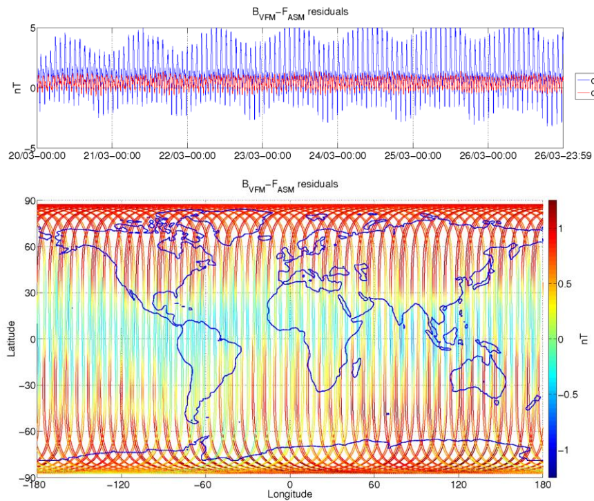
Figure 3-8: ASM-VFM residuals for S/C A, during monitoring period 20/03-26/03. In top figure are plotted: difference between |B_{VFM}| and F_{ASM} (without dB_{Sun} correction) (blue colour), and the residuals with dB_{Sun} corrections (red colour). In bottom figure residuals are presented on the world map.
