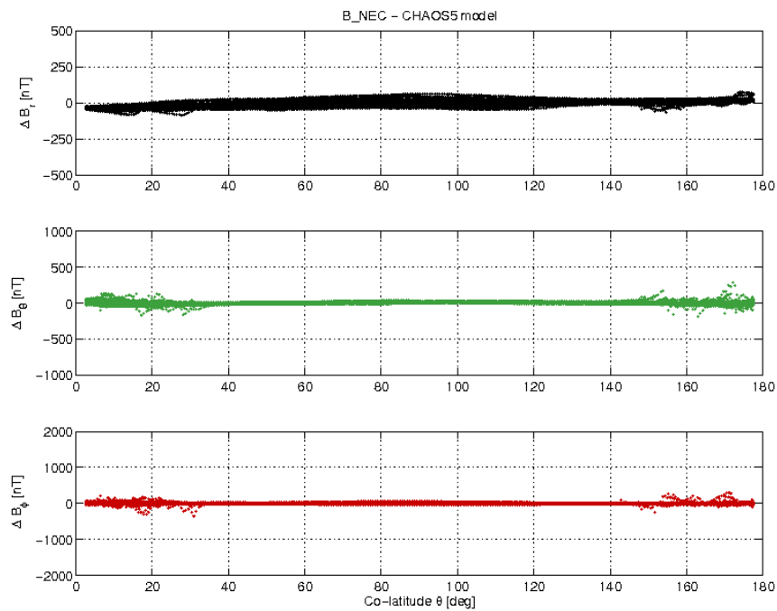
Figure 3-21: S/C C day 20/03 B_{NEC} - B_{Chaos} difference vs colatitude.
