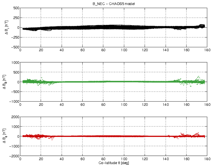
Figure 3-17: S/C A day 20/03 B_{NEC} - B_{Chaos} vs colatitude.
