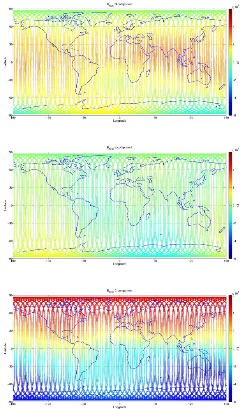
Figure 3-12: S/C C, world map plots of the geomagnetic field and components measured during monitoring period 20/03-26/03. From top to bottom: B NEC components (North, East, and Centre) of magnetic field from VFM measurement.
