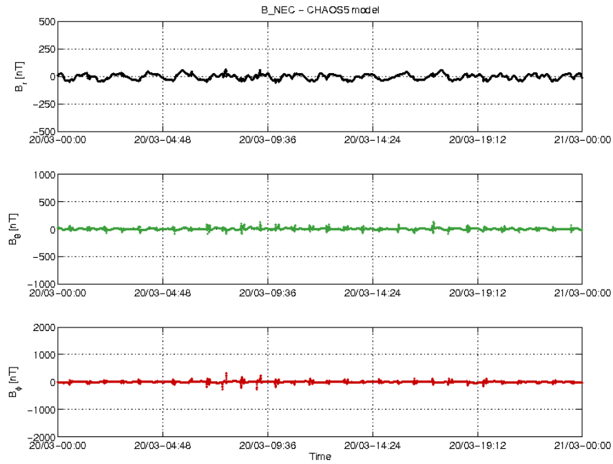
Figure 3-20: S/C B day 20/03 time series of B_{NEC} - B_{Chaos} residuals.
