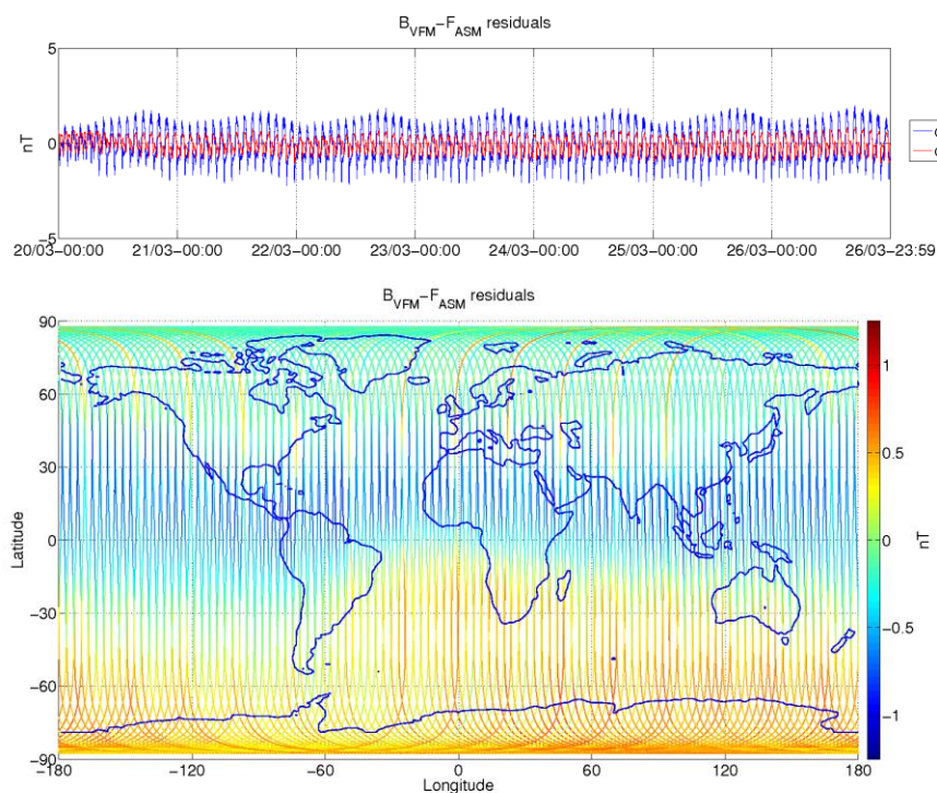
Figure 3-9: ASM-VFM residuals for S/C B, during monitoring period 20/03-26/03. In top figure are plotted: difference between |B_{VFM}| and F_{ASM} (without dB_{Sun} correction) (blue colour), and the residuals with dB_{Sun} corrections (red colour). In bottom figure residuals are presented on the world map.
