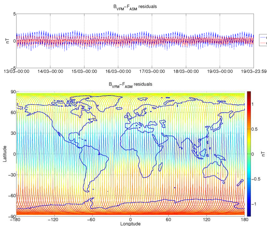
Figure 3-9: ASM-VFM residuals for S/C B, during monitoring period 13/03-19/03. In top figure are plotted: difference between |B_{VFM}| and F_{ASM} (without dB_{Sun} correction) (blue colour), and the residuals with dB_{Sun} corrections (red colour). In bottom figure residuals are presented on the world map.
