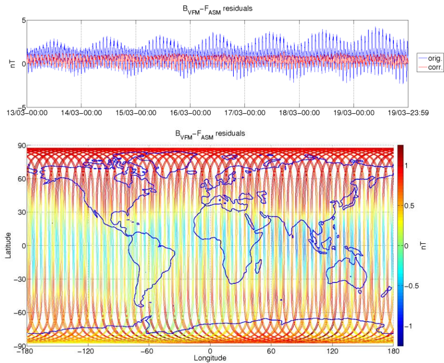
Figure 3-8: ASM-VFM residuals for S/C A, during monitoring period 13/03-19/03. In top figure are plotted: difference between |B VFM | and F ASM (without dB Sun correction) (blue colour), and the residuals with dB Sun corrections (red colour). In bottom figure residuals are presented on the world map.
