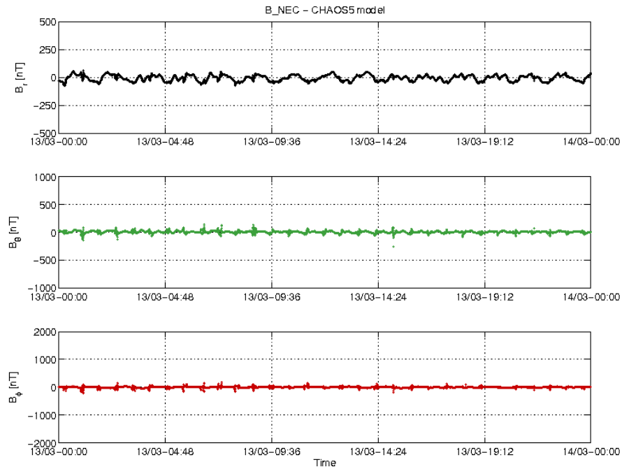
Figure 3-18: S/C A day 13/03: time series of B_{NEC} - B_{Chaos} residuals.
