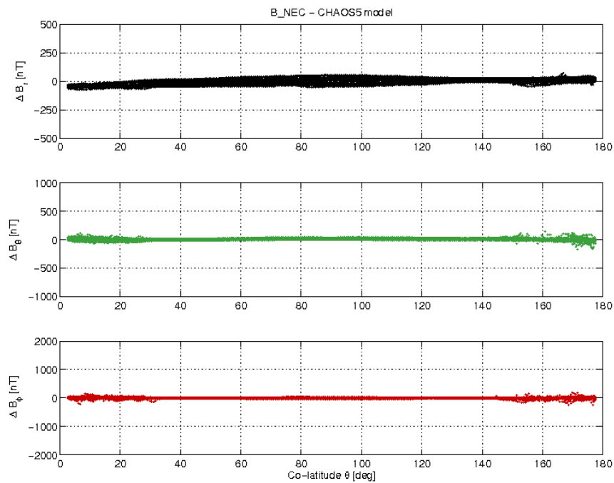
Figure 3-21: S/C C day 13/03 B_{NEC} - B_{Chaos} difference vs colatitude.
