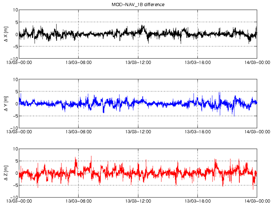
Figure 3-3: Difference MOD-GPSNAV, S/C A, 13/03. From top to bottom: X, Y and Z-axis
