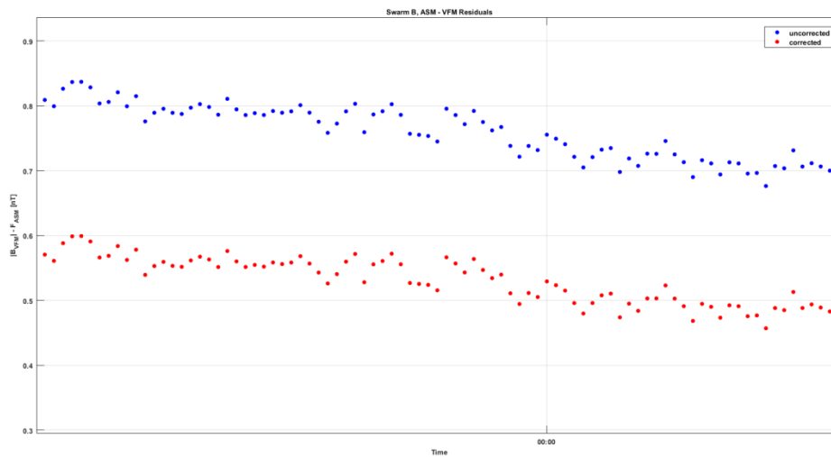
Figure 26: Trend of ASM-VFM residual for S/C B (zoomed for daybreak 14/03 – 15/03).
