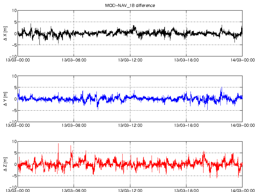
Figure 3-5: Difference MOD-GPSNAV, S/C C, 13/03. From top to bottom: X, Y and Z-axis
