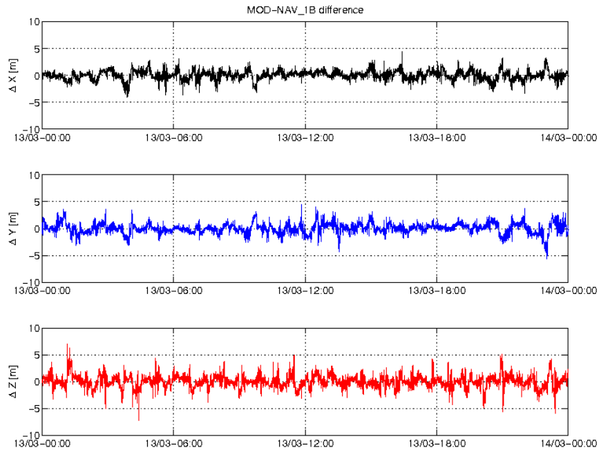
Figure 3-4: Difference MOD-GPSNAV, S/C B, 13/03. From top to bottom: X, Y and Z-axis
