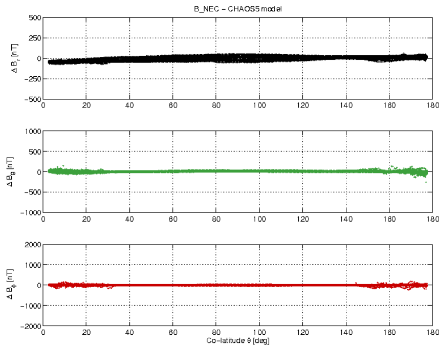
Figure 3-17: S/C A day 13/03 B_{NEC} - B_{Chaos} vs colatitude.
