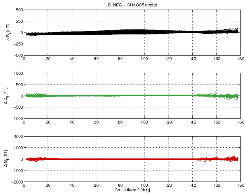
Figure 3-19: S/C B day 13/03 B_{NEC} - B_{Chaos} difference vs colatitude.
