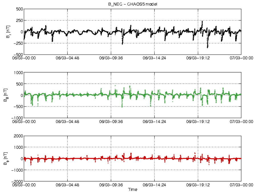
Figure 3-18: S/C A day 06/03: time series of B_{NEC} - B_{Chaos} residuals.
