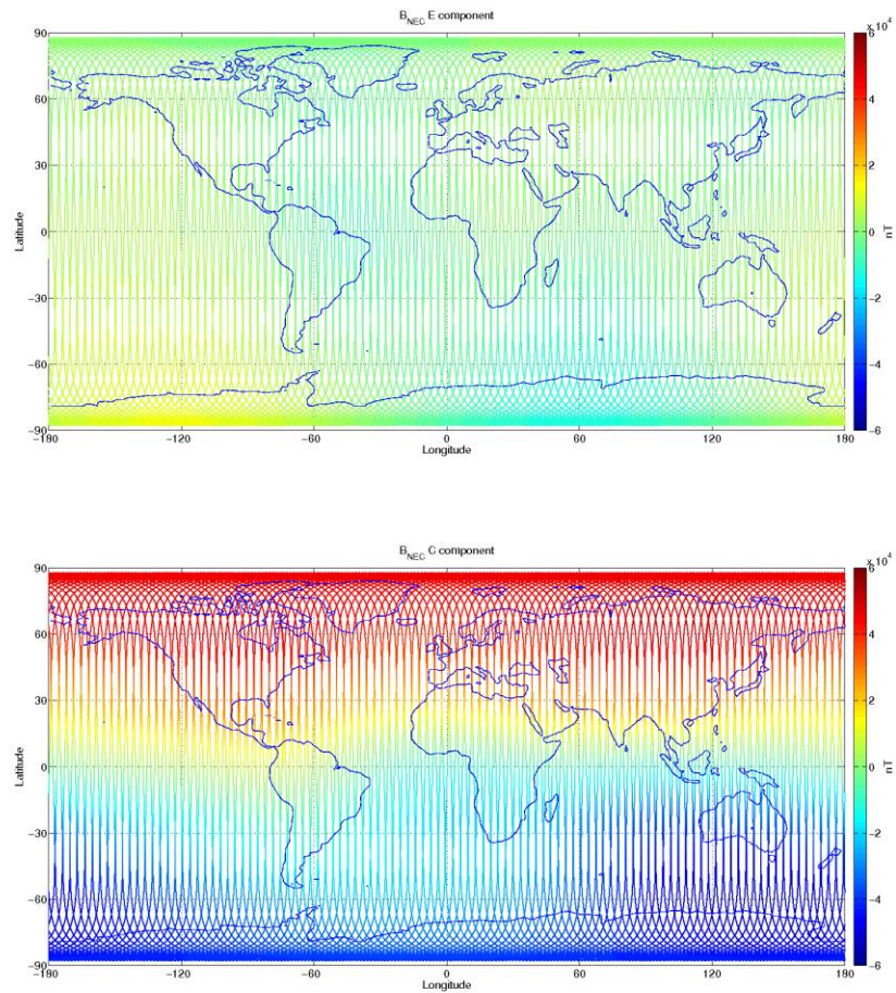
Figure 3-11: S/C B, world map plots of the geomagnetic field and components measured during monitoring period 06/03-12/03. From top to bottom: F-magnetic field from ASM measurement, B_{NEC} components (North, East, and Centre) of magnetic field from VFM measurement.
