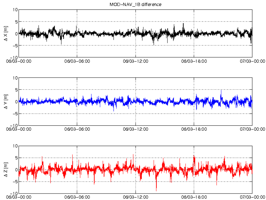
Figure 3-3: Difference MOD-GPSNAV, S/C A, 06/03. From top to bottom: X, Y and Z-axis
