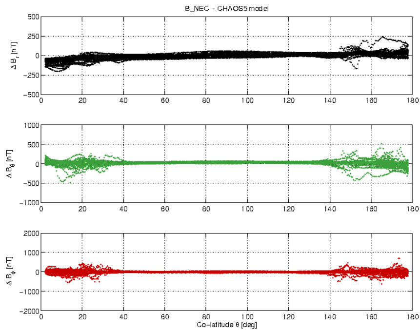
Figure 3-19: S/C B day 06/03 B_{NEC} - B_{Chaos} difference vs colatitude.
