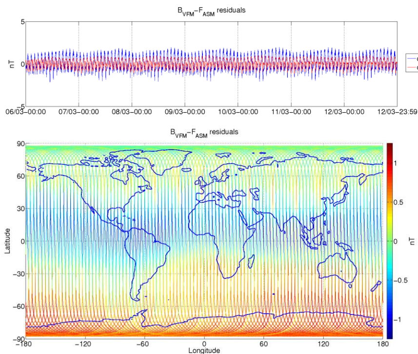
Figure 3-9: ASM-VFM residuals for S/C B, during monitoring period 06/03-12/03. In top figure are plotted: difference between |B_VFM| and F_ASM (without dB_Sun correction) (blue colour), and the residuals with dB_Sun corrections (red colour). In bottom figure residuals are presented on the world map.
