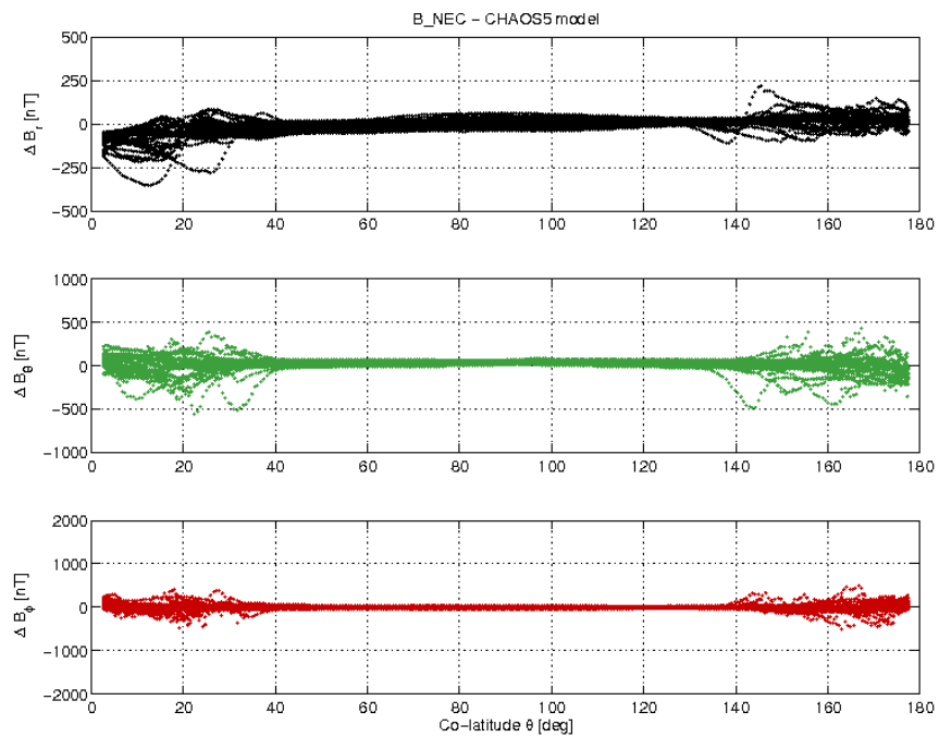
Figure 3-21: S/C C day 06/03 B_{NEC} - B_{Chaos} difference vs colatitude.
