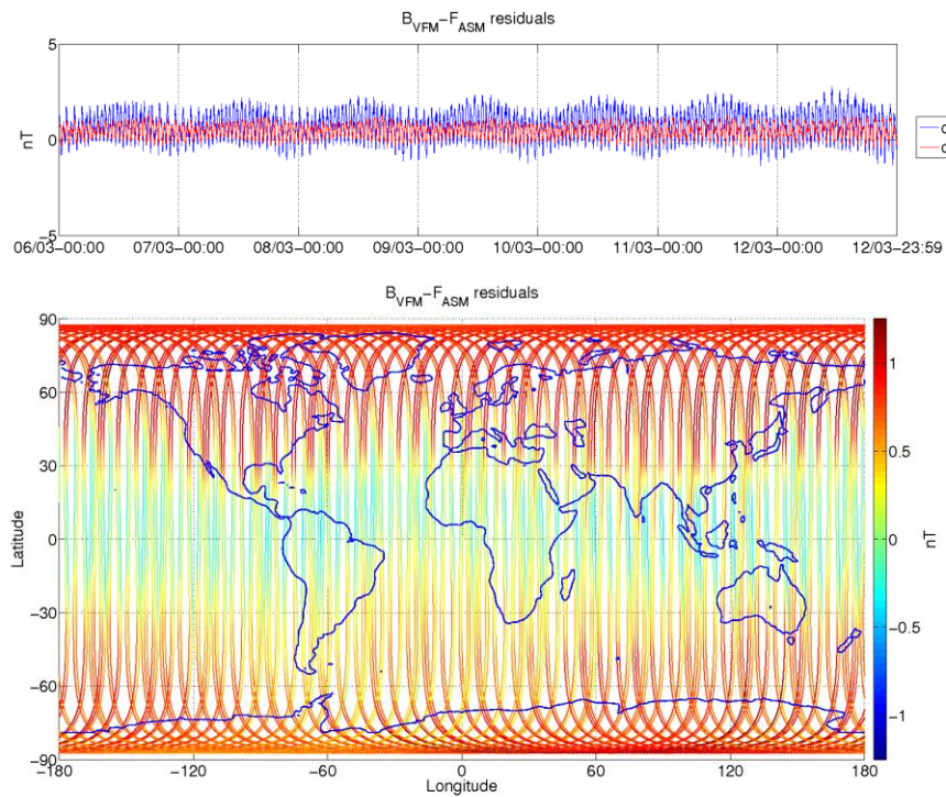
Figure 3-8: ASM-VFM residuals for S/C A, during monitoring period 06/03-12/03. In top figure are plotted: difference between |B VFM | and F ASM (without dB Sun correction) (blue colour), and the residuals with dB Sun corrections (red colour). In bottom figure residuals are presented on the world map.
