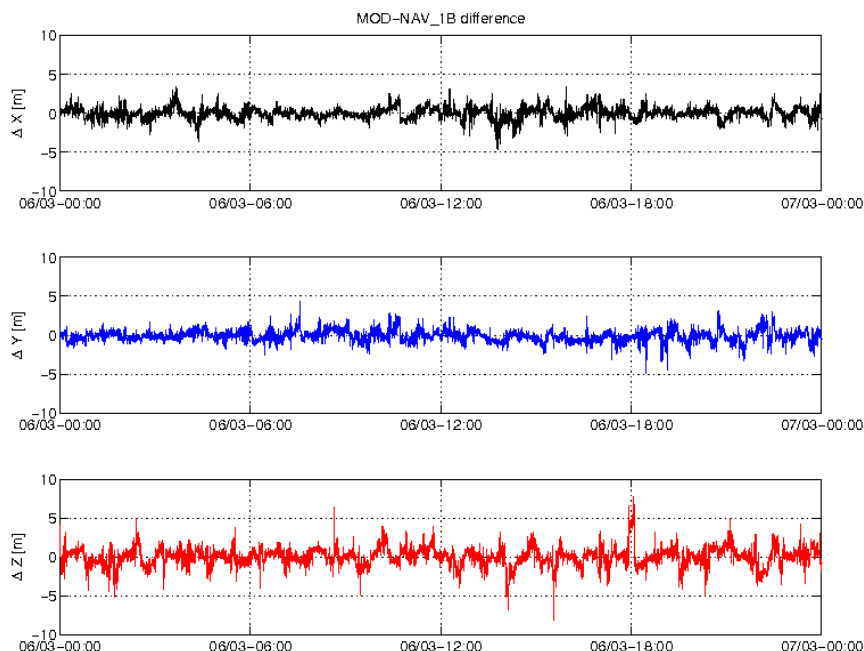
Figure 3-5: Difference MOD-GPSNAV, S/C C, 06/03. From top to bottom: X, Y and Z-axis
