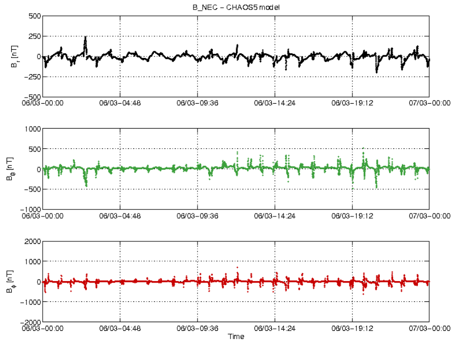
Figure 3-20: S/C B day 06/03 time series of B_{NEC} - B_{Chaos} residuals.
