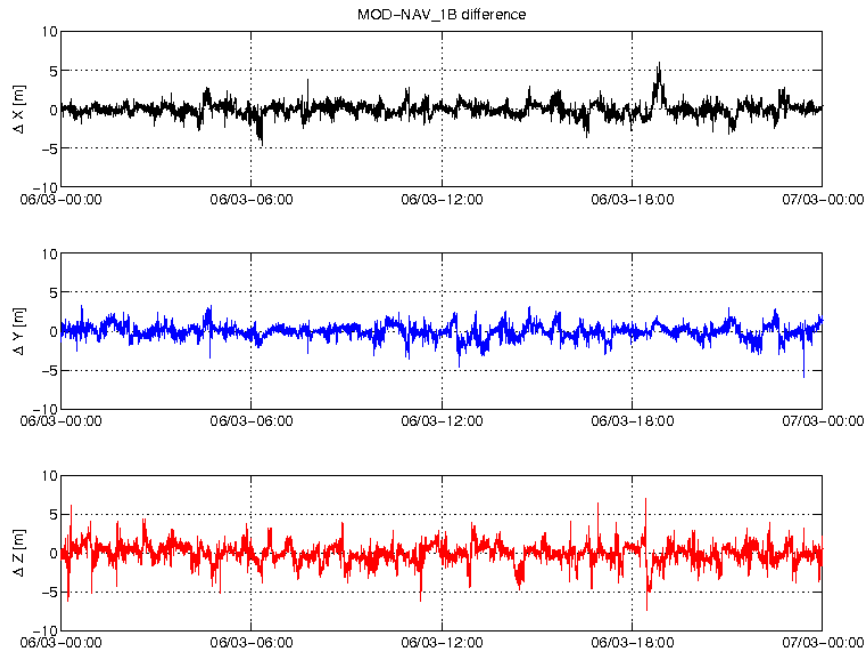
Figure 3-4: Difference MOD-GPSNAV, S/C B, 06/03. From top to bottom: X, Y and Z-axis
