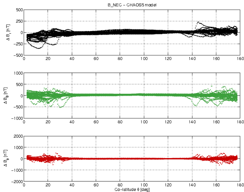
Figure 3-17: S/C A day 06/03 B_{NEC} - B_{Chaos} vs colatitude.
