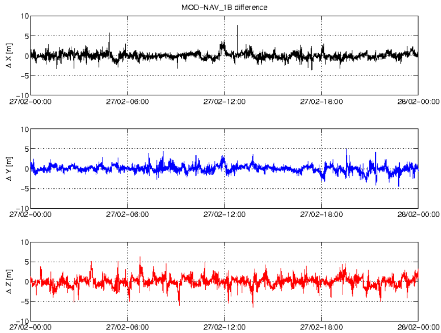
Figure 3-3: Difference MOD-GPSNAV, S/C A, 27/02. From top to bottom: X, Y and Z-axis
