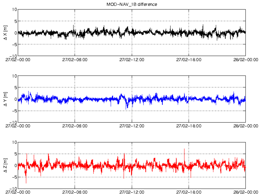
Figure 3-4: Difference MOD-GPSNAV, S/C B, 27/02. From top to bottom: X, Y and Z-axis
