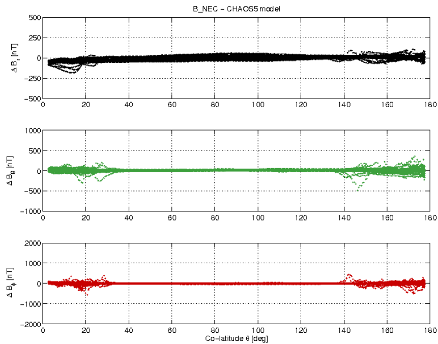
Figure 3-21: S/C C day 27/02 B_{NEC} - B_{Chaos} difference vs colatitude.
