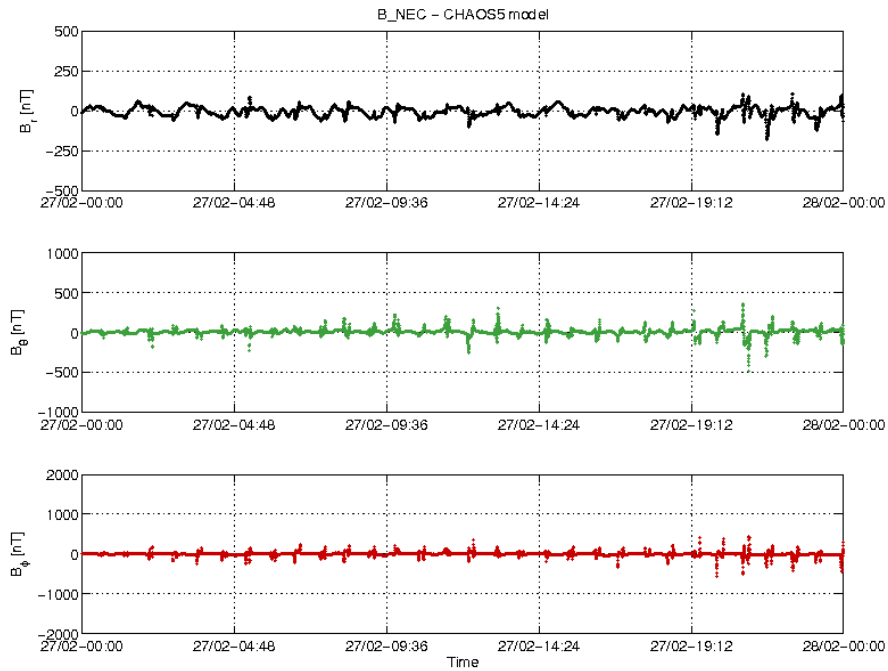
Figure 3-22: S/C C day 27/02 time series of B_{NEC} - B_{Chaos} residuals.
