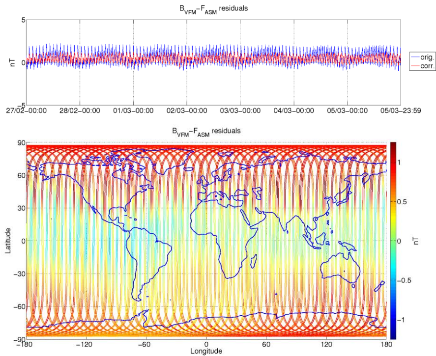
Figure 3-8: ASM-VFM residuals for S/C A, during monitoring period 27/02-05/03. In top figure are plotted: difference between |B VFM | and F ASM (without dB Sun correction) (blue colour), and the residuals with dB Sun corrections (red colour). In bottom figure residuals are presented on the world map.
