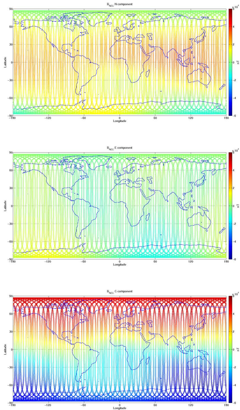
Figure 3-12: S/C C, world map plots of the geomagnetic field and components measured during monitoring period 27/02-05/03. From top to bottom: B_{NEC} components (North, East, and Centre) of magnetic field from VFM measurement.
