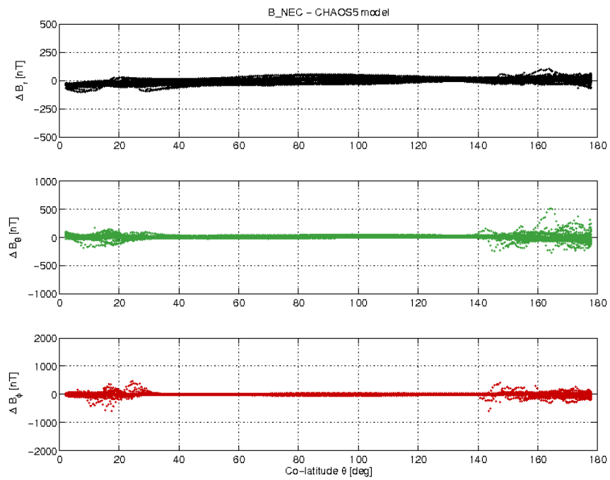
Figure 3-19: S/C B day 27/02 B_{NEC} - B_{Chaos} difference vs colatitude.
