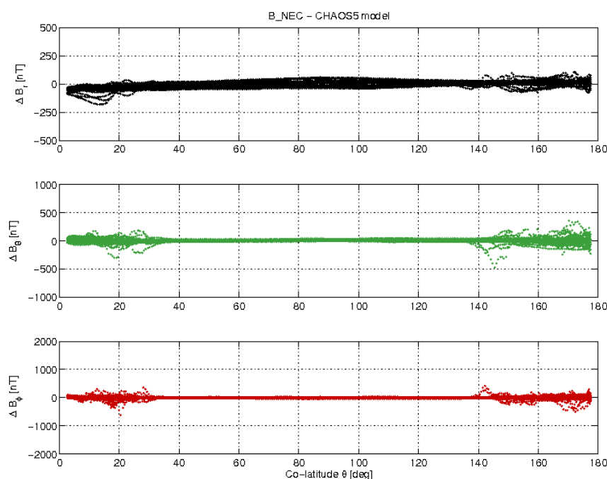
Figure 3-17: S/C A day 27/02 B_{NEC} - B_{Chaos5} vs colatitude.
