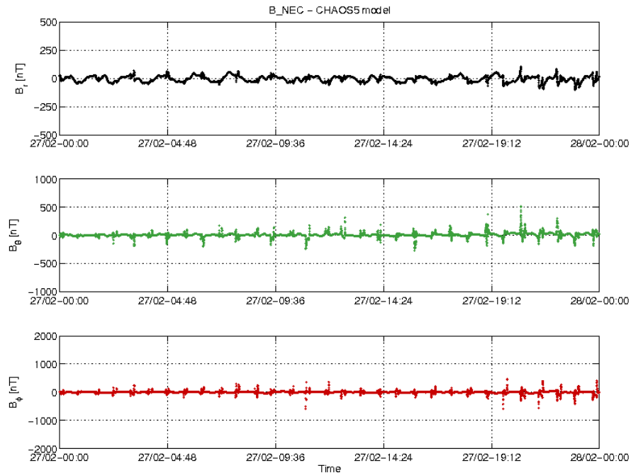
Figure 3-20: S/C B day 27/02 time series of B_{NEC} - B_{Chaos} residuals.
