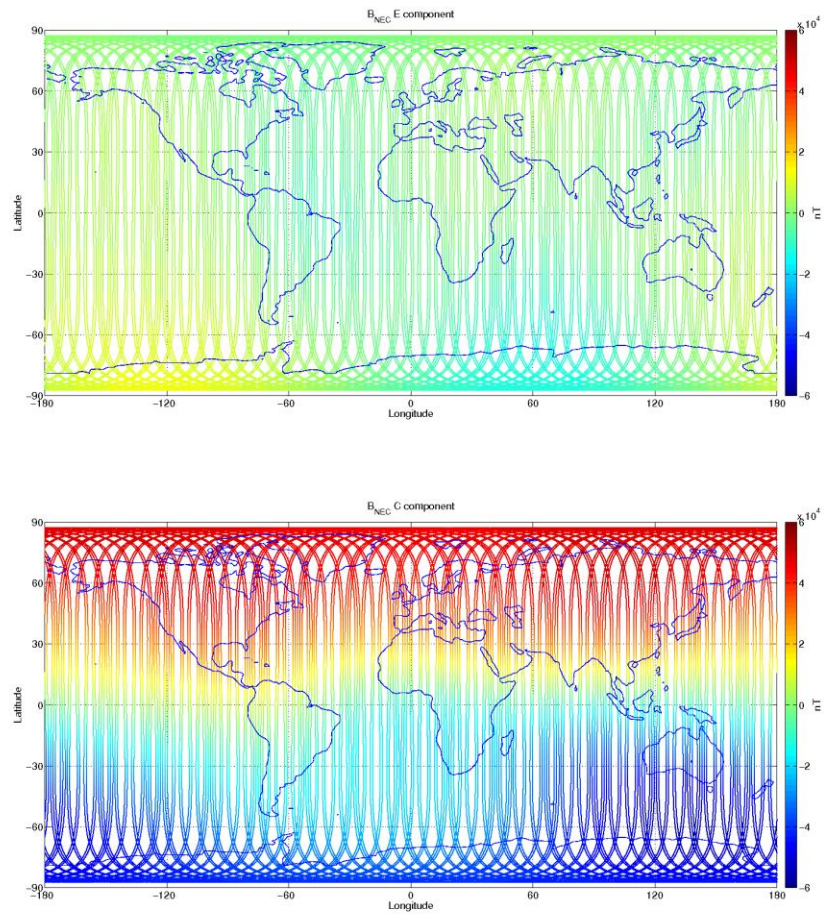
Figure 3-10: S/C A, world map plots of the geomagnetic field and components measured during monitoring period 27/02-05/03. From top to bottom: F-magnetic field from ASM measurement, B_{NEC} components (North, East, and Centre) of magnetic field from VFM measurement.
