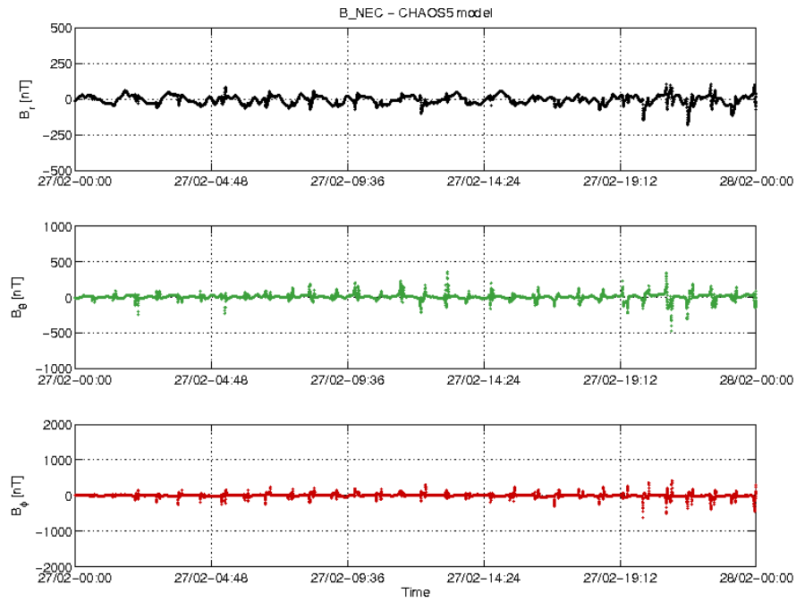
Figure 3-18: S/C A day 27/02: time series of B_{NEC} - B_{Chaos} residuals.
