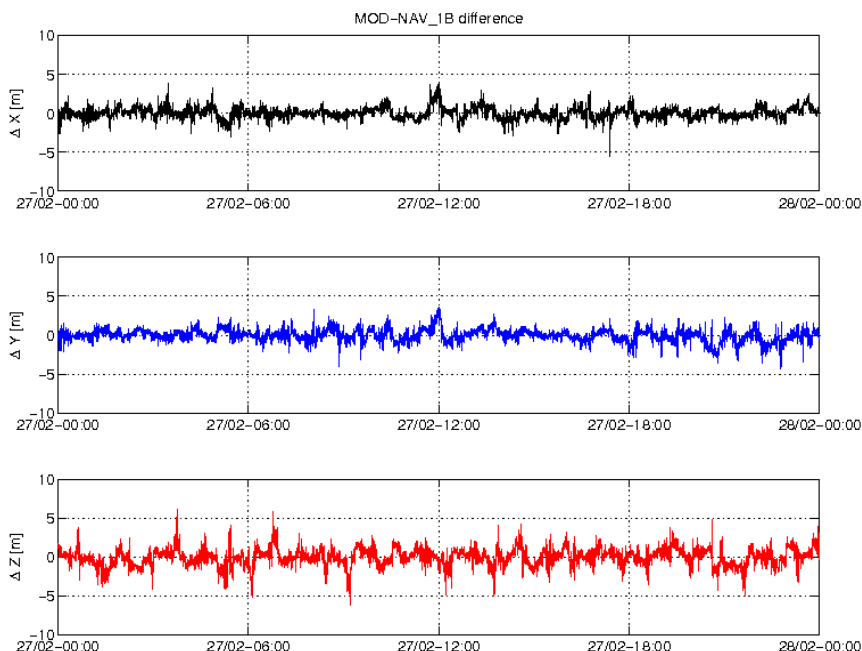
Figure 3-5: Difference MOD-GPSNAV, S/C C, 27/02. From top to bottom: X, Y and Z-axis
