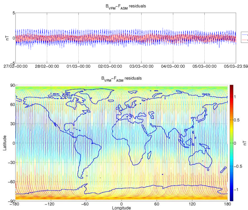
Figure 3-9: ASM-VFM residuals for S/C B, during monitoring period 27/02-05/03. In top figure are plotted: difference between |B_{VFM}| and F_{ASM} (without dB_{Sun} correction) (blue colour), and the residuals with dB_{Sun} corrections (red colour). In bottom figure residuals are presented on the world map.
