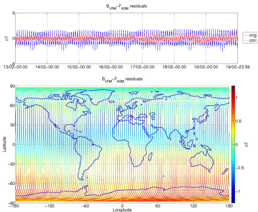
Figure 3-9: ASM-VFM residuals for S/C B, during monitoring period 13/02-19/02. In top figure are plotted: difference between |B_{VFM}| and F_{ASM} (without dB_{Sun} correction) (blue colour), and the residuals with dB_{Sun} corrections (red colour). In bottom figure residuals are presented on the world map.
