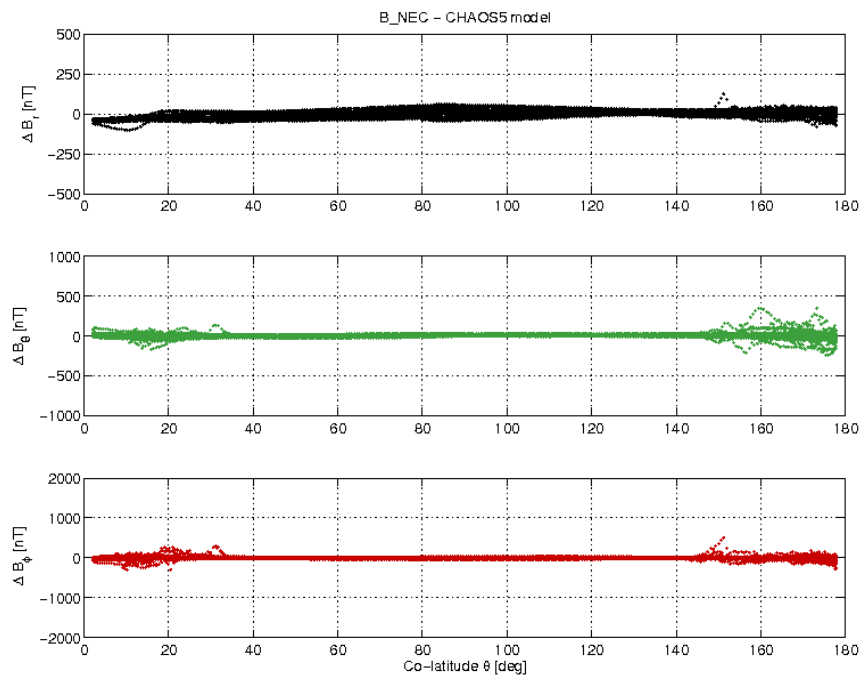
Figure 3-19: S/C B day 13/02 B_{NEC} - B_{Chaos} difference vs colatitude.
