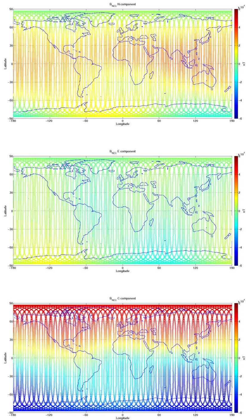
Figure 3-12: S/C C, world map plots of the geomagnetic field and components measured during monitoring period 13/02-19/02. From top to bottom: B NEC components (North, East, and Centre) of magnetic field from VFM measurement.
