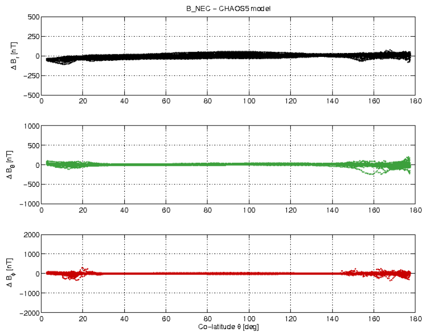
Figure 3-21: S/C C day 13/02 B_{NEC} - B_{Chaos} difference vs colatitude.
