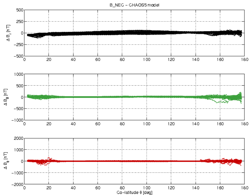
Figure 3-17: S/C A day 13/02 B_{NEC} - B_{Chaos} vs colatitude.
