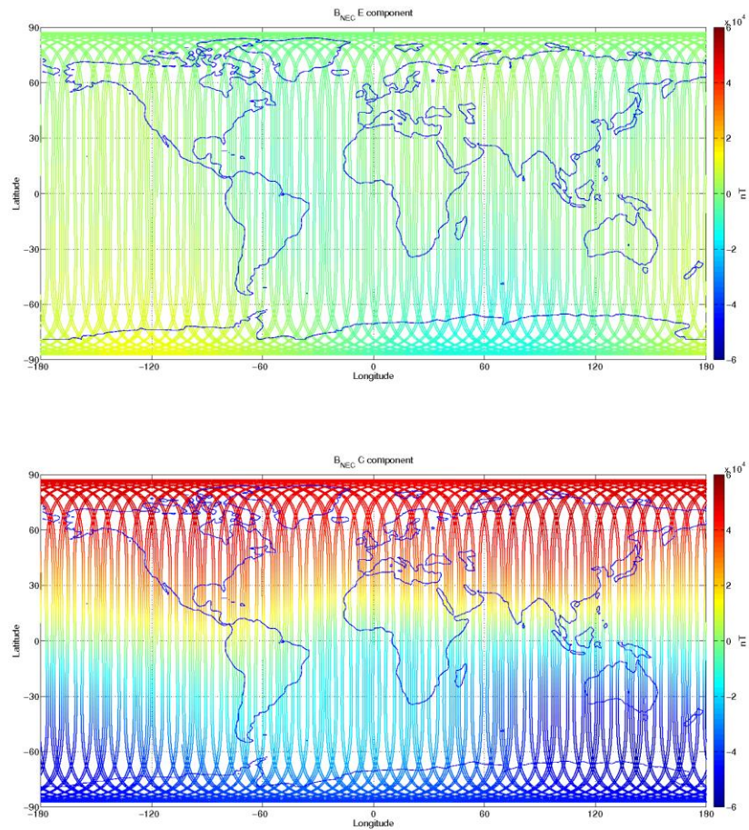
Figure 3-10: S/C A, world map plots of the geomagnetic field and components measured during monitoring period 13/02-19/02. From top to bottom: F-magnetic field from ASM measurement, B_{NEC} components (North, East, and Centre) of magnetic field from VFM measurement.
