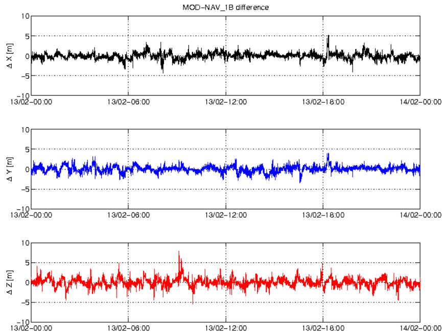
Figure 3-4: Difference MOD-GPSNAV, S/C B, 13/02. From top to bottom: X, Y and Z-axis
