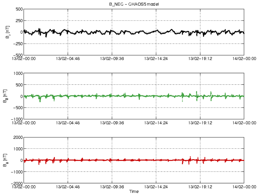
Figure 3-22: S/C C day 13/02 time series of B_{NEC} - B_{Chaos} residuals.
