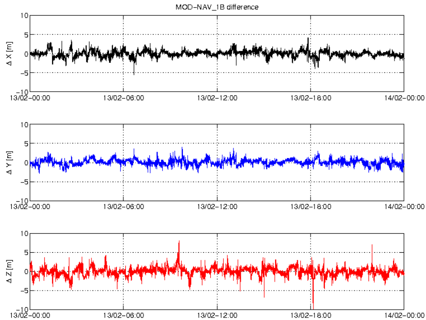
Figure 3-3: Difference MOD-GPSNAV, S/C A, 13/02. From top to bottom: X, Y and Z-axis
