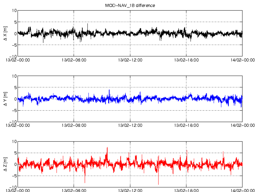
Figure 3-5: Difference MOD-GPSNAV, S/C C, 13/02. From top to bottom: X, Y and Z-axis
