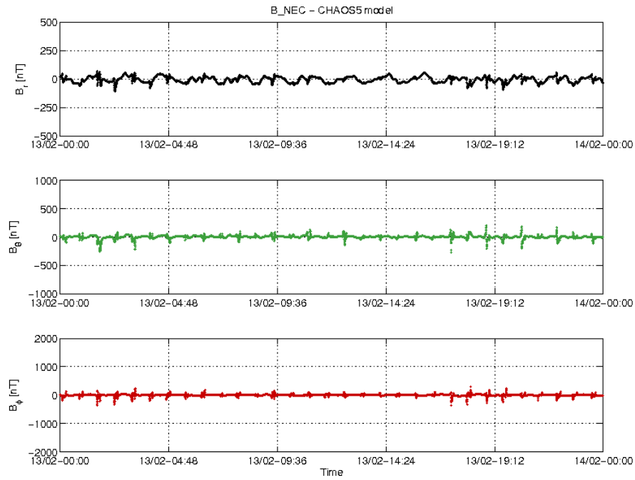
Figure 3-18: S/C A day 13/02: time series of B_{NEC} - B_{Chaos} residuals.
