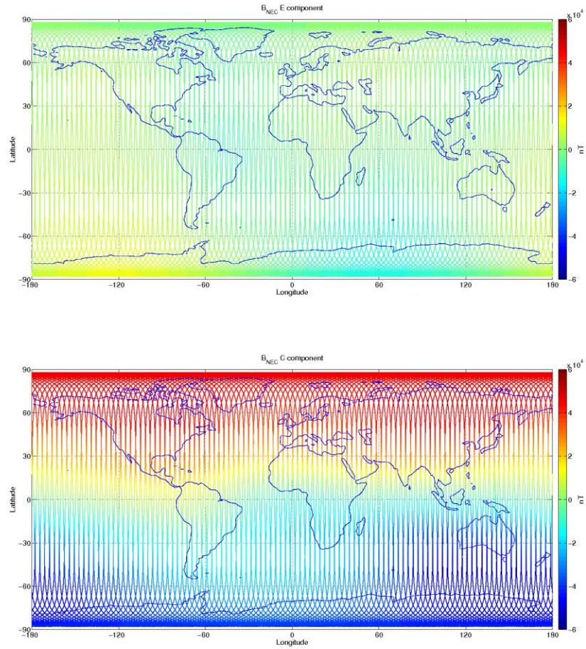
Figure 3-11: S/C B, world map plots of the geomagnetic field and components measured during monitoring period 13/02-19/02. From top to bottom: F-magnetic field from ASM measurement, B_{NEC} components (North, East, and Centre) of magnetic field from VFM measurement.
