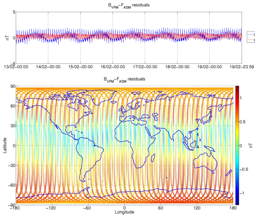
Figure 3-8: ASM-VFM residuals for S/C A, during monitoring period 13/02-19/02. In top figure are plotted: difference between |B_{VFM}| and F_{ASM} (without dB_{Sun} correction) (blue colour), and the residuals with dB_{Sun} corrections (red colour). In bottom figure residuals are presented on the world map.
