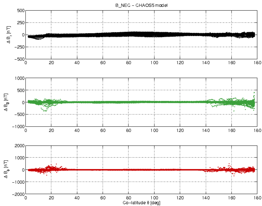
Figure 3-19: S/C B day 30/01 B_{NEC} - B_{Chaos} difference vs colatitude.
