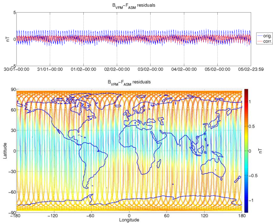
Figure 3-8: ASM-VFM residuals for S/C A, during monitoring period 30/01-05/02. In top figure are plotted: difference between |B VFM | and F ASM (without dB Sun correction) (blue colour), and the residuals with dB Sun corrections (red colour). In bottom figure residuals are presented on the world map.
