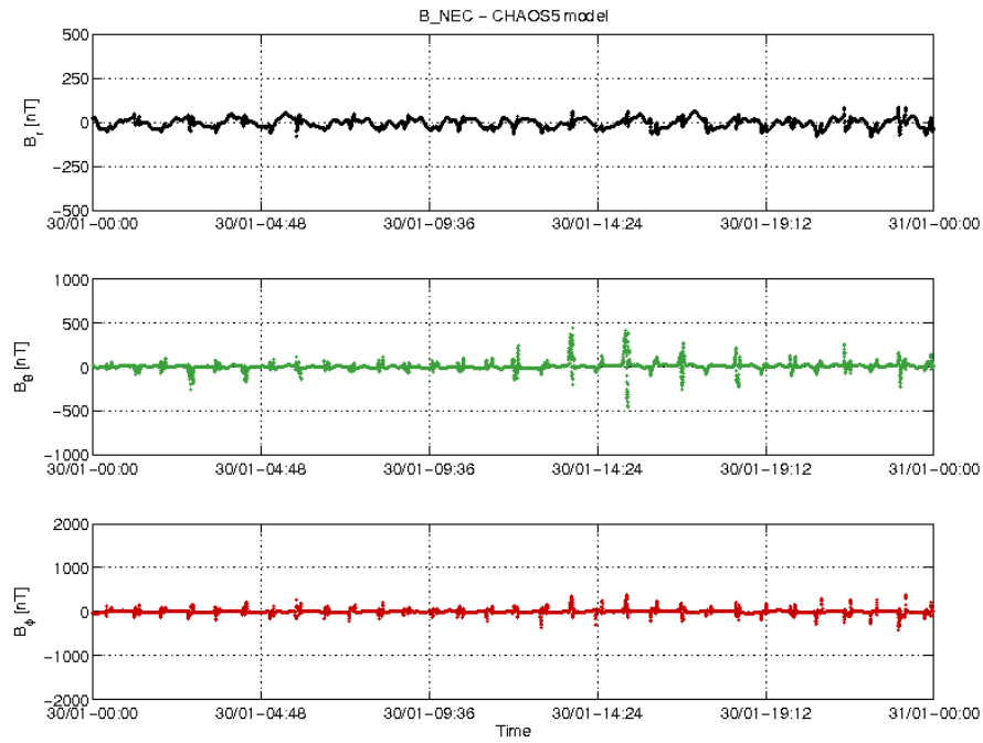
Figure 3-18: S/C A day 30/01: time series of B_{NEC} - B_{Chaos} residuals.
