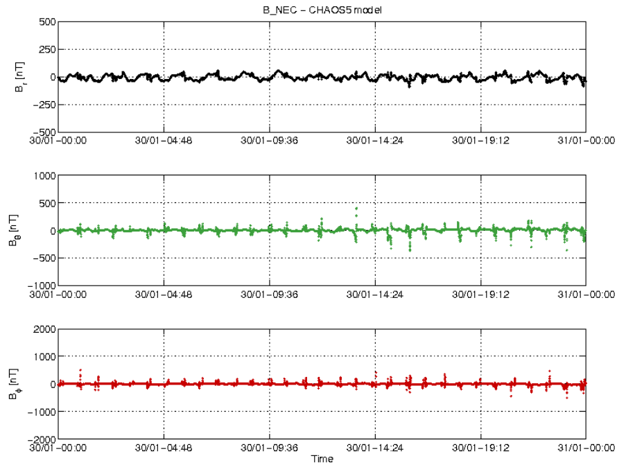
Figure 3-20: S/C B day 30/01 time series of B_{NEC} - B_{Chaos} residuals.
