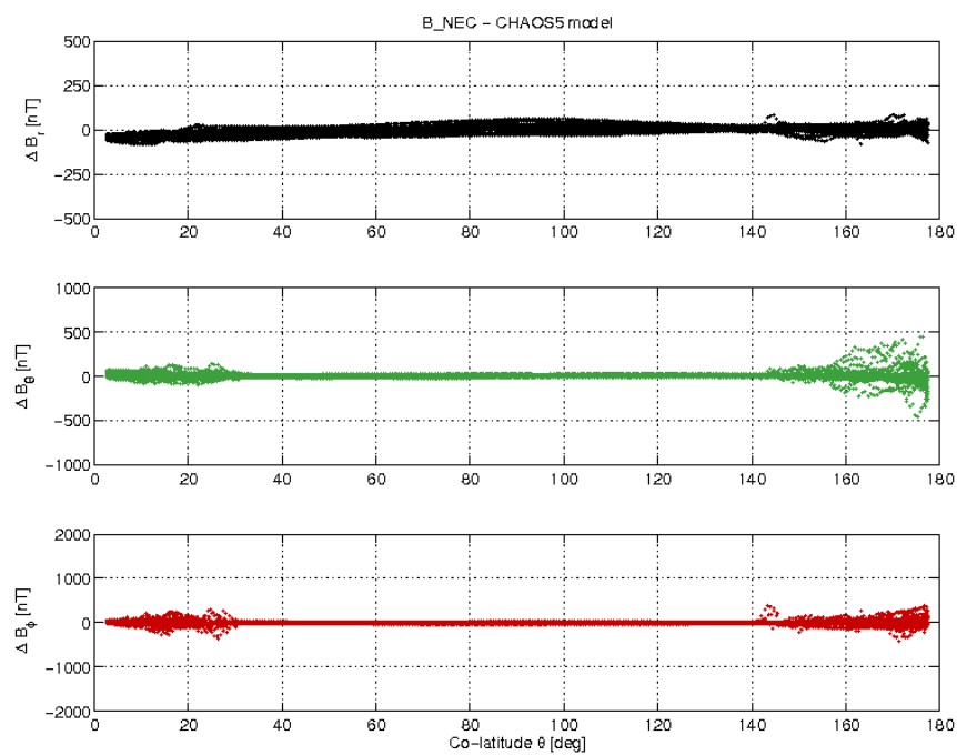
Figure 3-17: S/C A day 30/01 B_{NEC} - B_{Chaos} vs colatitude.
