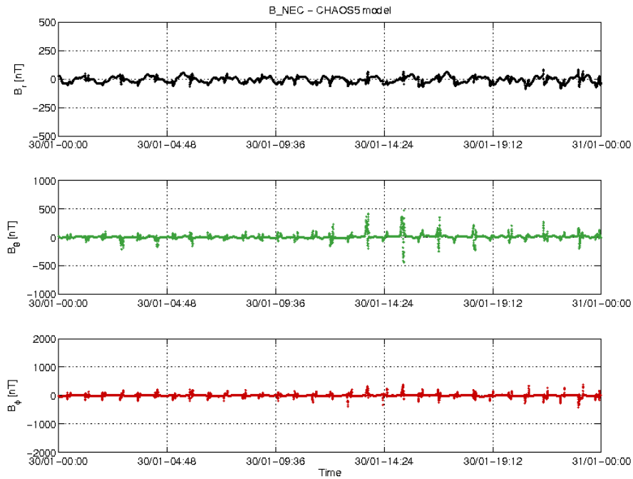
Figure 3-22: S/C C day 30/01 time series of B_{NEC} - B_{Chaos} residuals.
