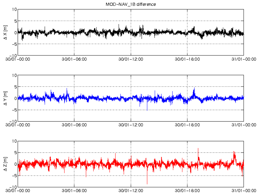
Figure 3-4: Difference MOD-GPSNAV, S/C B, 30/01. From top to bottom: X, Y and Z-axis
