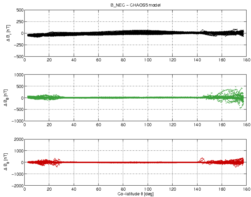
Figure 3-21: S/C C day 30/01 B_{NEC} - B_{Chaos} difference vs colatitude.
