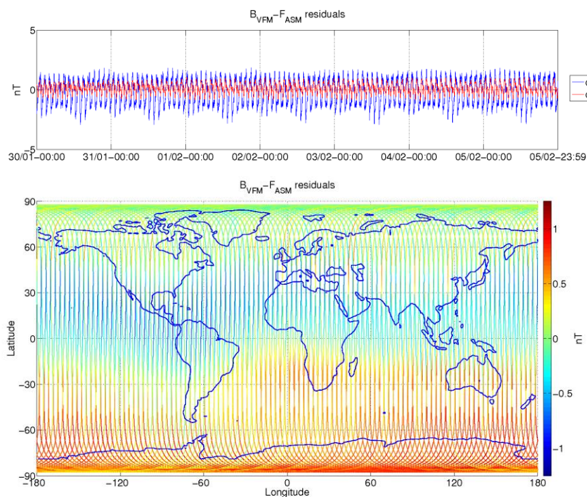
Figure 3-9: ASM-VFM residuals for S/C B, during monitoring period 30/01-05/02. In top figure are plotted: difference between |B_{VFM}| and F_{ASM} (without dB_{Sun} correction) (blue colour), and the residuals with dB_{Sun} corrections (red colour). In bottom figure residuals are presented on the world map.
