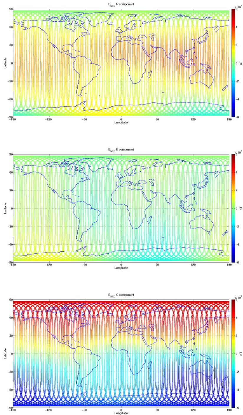
Figure 3-12: S/C C, world map plots of the geomagnetic field and components measured during monitoring period 30/01-05/02. From top to bottom: B_{NEC} components (North, East, and Centre) of magnetic field from VFM measurement.
