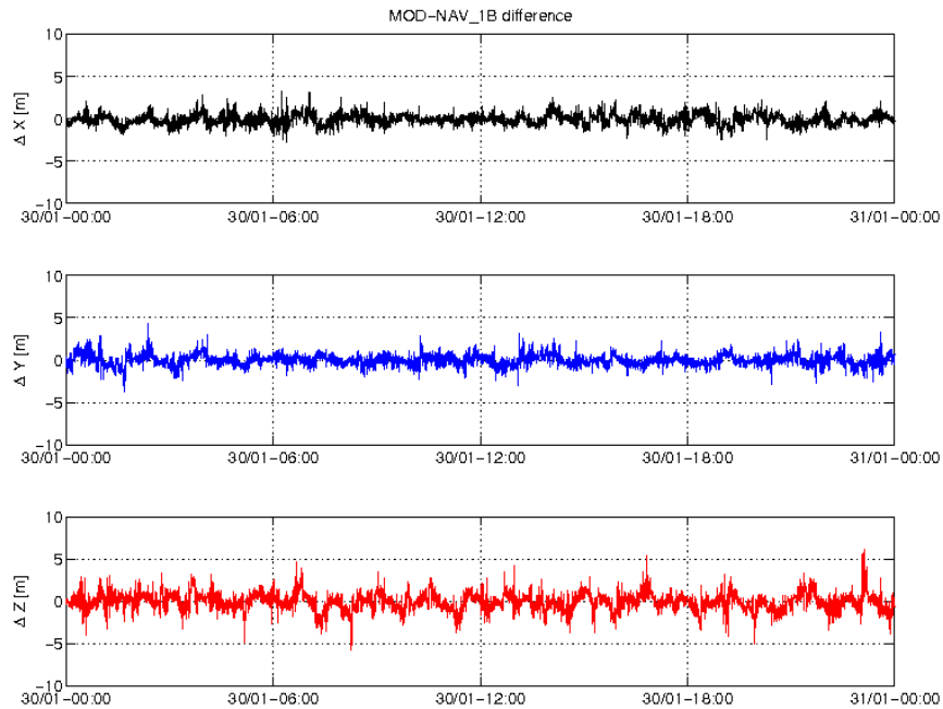
Figure 3-3: Difference MOD-GPSNAV, S/C A, 30/01. From top to bottom: X, Y and Z-axis
