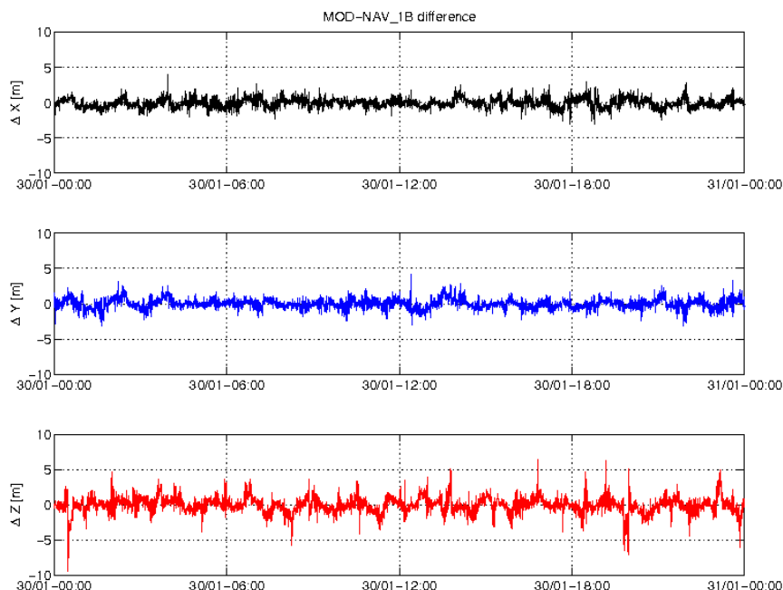
Figure 3-5: Difference MOD-GPSNAV, S/C C, 30/01. From top to bottom: X, Y and Z-axis
