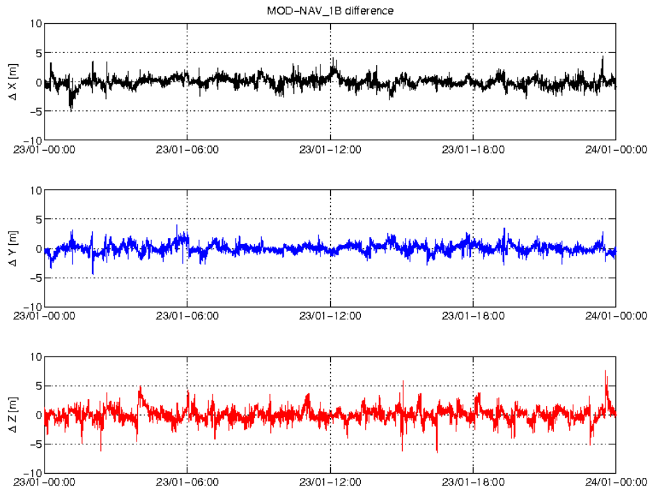
Figure 3-4: Difference MOD-GPSNAV, S/C B, 23/01. From top to bottom: X, Y and Z-axis
