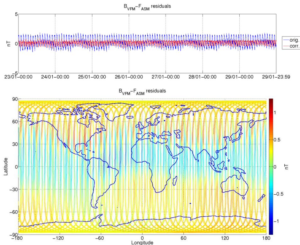
Figure 3-8: ASM-VFM residuals for S/C A, during monitoring period 23/01-29/01. In top figure are plotted: difference between |B_{VFM}| and F_{ASM} (without dB_{Sun} correction) (blue colour), and the residuals with dB_{Sun} corrections (red colour). In bottom figure residuals are presented on the world map.
