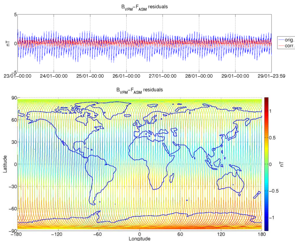
Figure 3-9: ASM-VFM residuals for S/C B, during monitoring period 23/01-29/01. In top figure are plotted: difference between |B_{VFM}| and F_{ASM} (without dB_{Sun} correction) (blue colour), and the residuals with dB_{Sun} corrections (red colour). In bottom figure residuals are presented on the world map.
