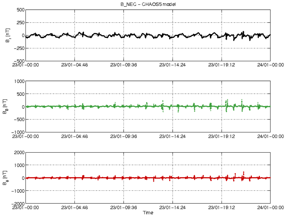
Figure 3-22: S/C C day 23/01 time series of B_{NEC} - B_{Chaos} residuals.
