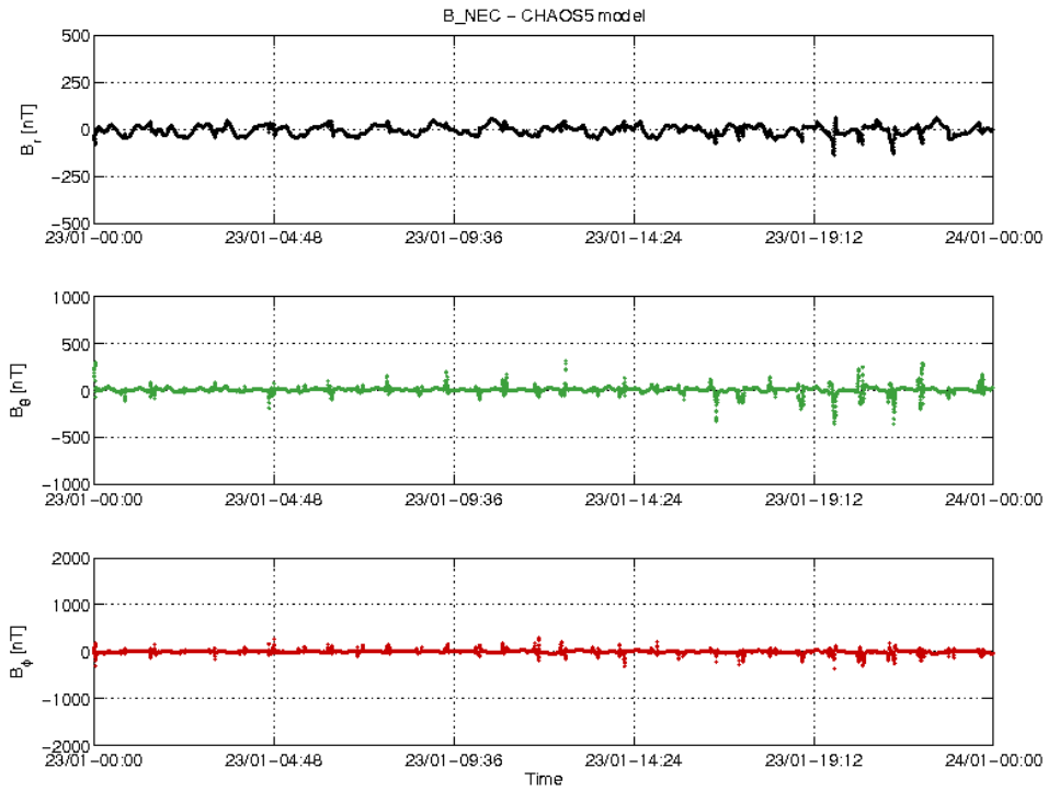
Figure 3-20: S/C B day 23/01 time series of B_{NEC} - B_{Chaos} residuals.
