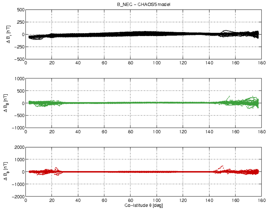
Figure 3-21: S/C C day 23/01 B_{NEC} - B_{Chaos} difference vs colatitude.
