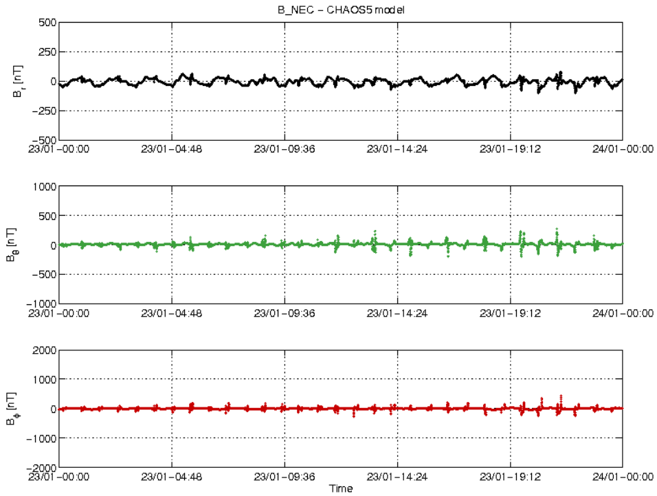
Figure 3-18: S/C A day 23/01: time series of B_{NEC} - B_{Chaos} residuals.
