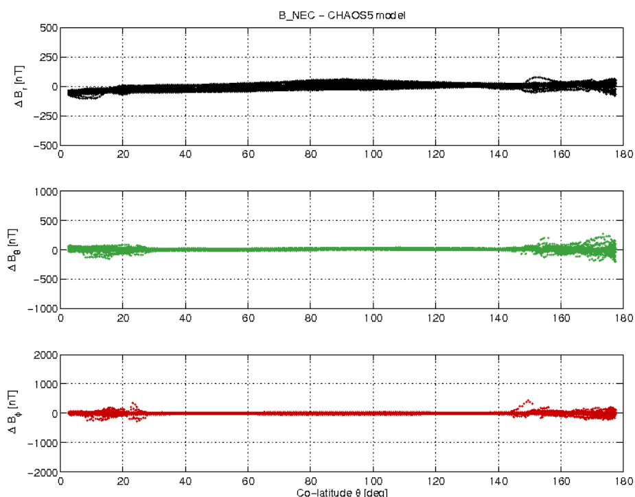
Figure 3-17: S/C A day 23/01 B_{NEC} - B_{Chaos} vs colatitude.
