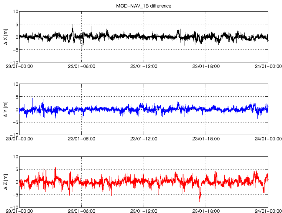
Figure 3-5: Difference MOD-GPSNAV, S/C C, 23/01. From top to bottom: X, Y and Z-axis
