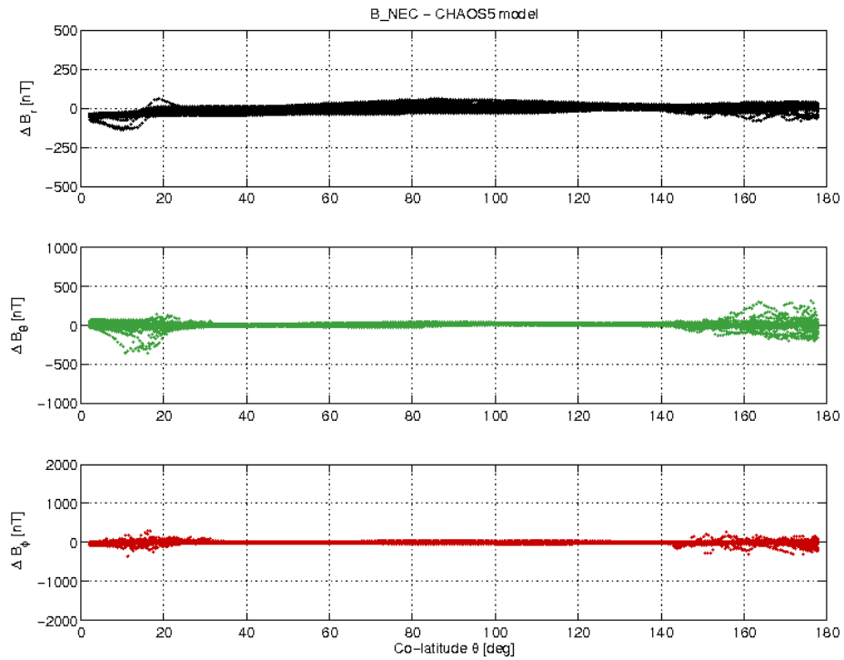
Figure 3-19: S/C B day 23/01 B_{NEC} - B_{Chaos} difference vs colatitude.
