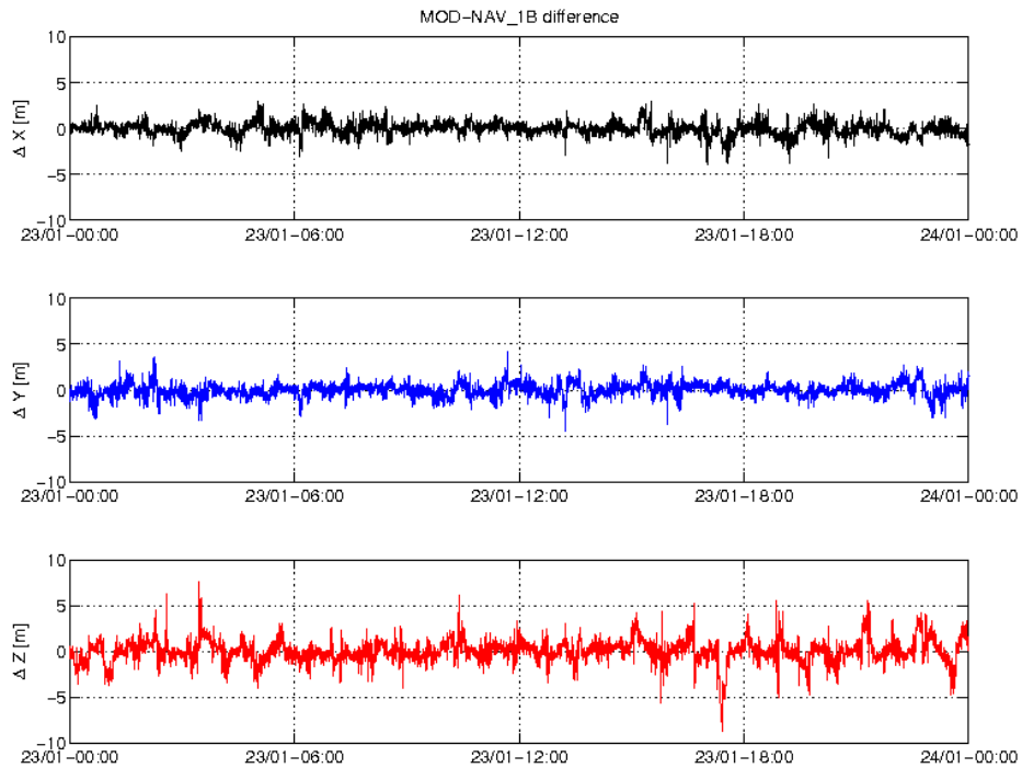
Figure 3-3: Difference MOD-GPSNAV, S/C A, 23/01. From top to bottom: X, Y and Z-axis
