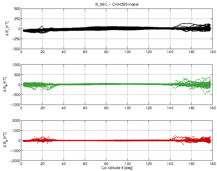
Figure 3-19: S/C B day 02/01 B_{NEC} - B_{Chaos} difference vs colatitude.
