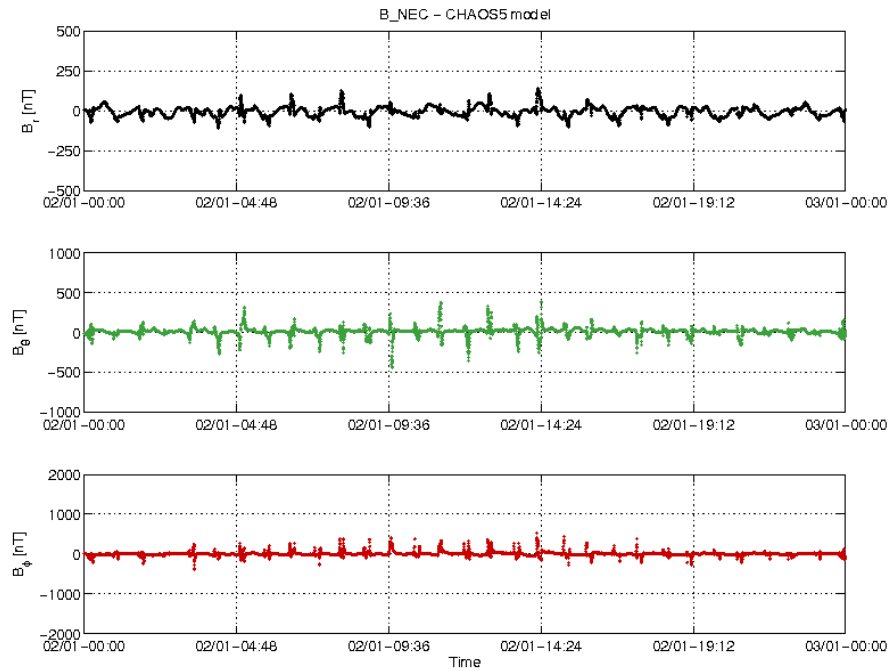
Figure 3-20: S/C B day 02/01 time series of B_{NEC} - B_{Chaos} residuals.
