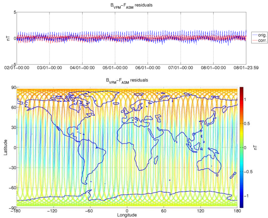
Figure 3-8: ASM-VFM residuals for S/C A, during monitoring period 02/01-08/01. In top figure are plotted: difference between |B_{VFM}| and F_{ASM} (without dB_{Sun} correction) (blue colour), and the residuals with dB_{Sun} corrections (red colour). In bottom figure residuals are presented on the world map.
