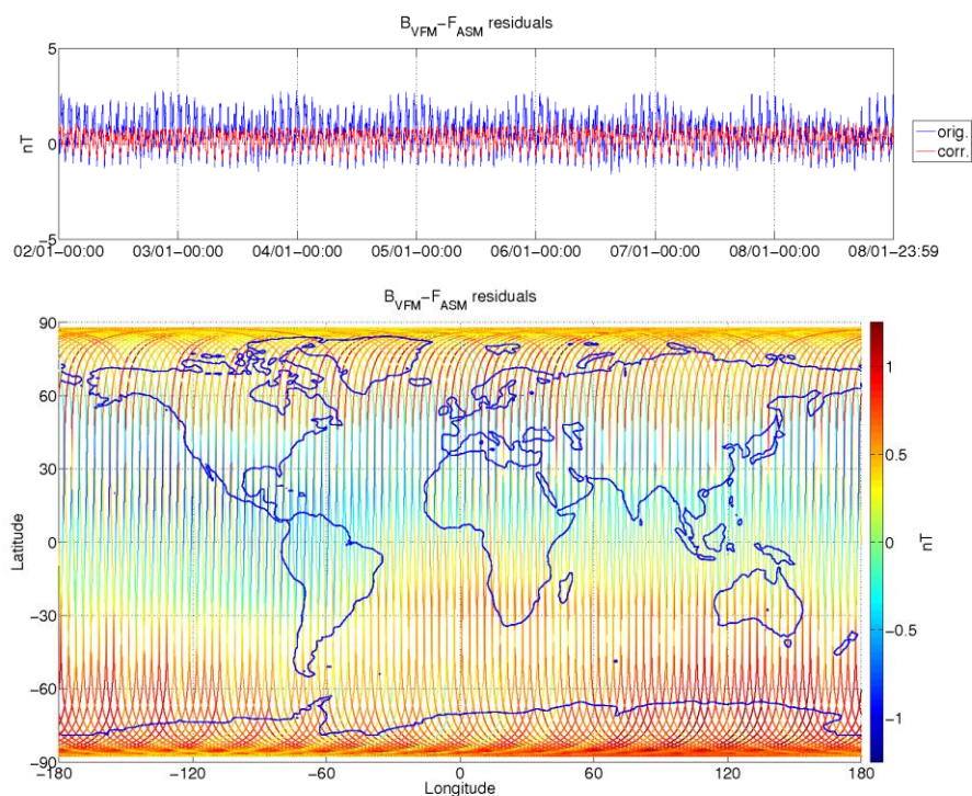
Figure 3-9: ASM-VFM residuals for S/C B, during monitoring period 02/01-08/01. In top figure are plotted: difference between |B_{VFM}| and F_{ASM} (without dB_{Sun} correction) (blue colour), and the residuals with dB_{Sun} corrections (red colour). In bottom figure residuals are presented on the world map.
