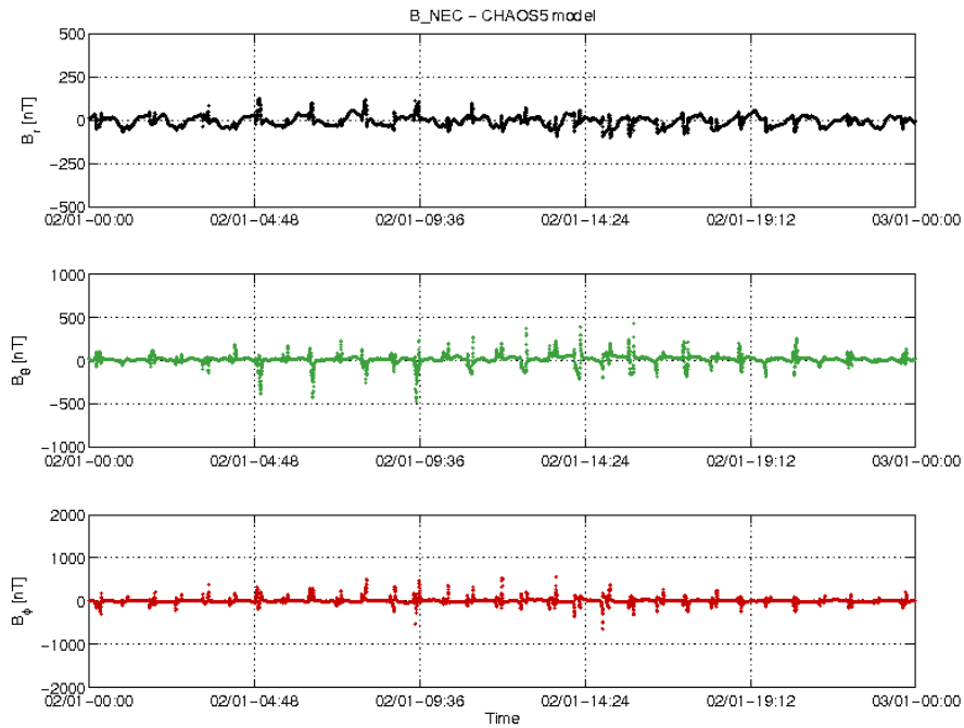
Figure 3-22: S/C C day 02/01 time series of B_{NEC} - B_{Chaos} residuals.
