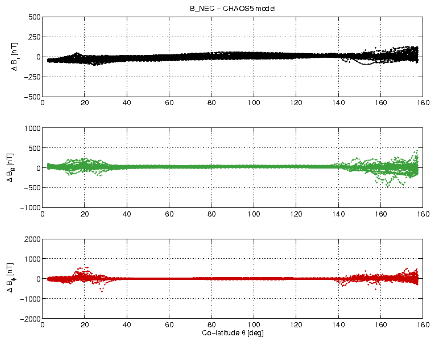
Figure 3-21: S/C C day 02/01 B_{NEC} - B_{Chaos} difference vs colatitude.
