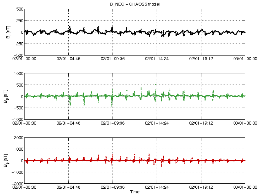
Figure 3-18: S/C A day 02/01: time series of B_{NEC} - B_{Chaos} residuals.
