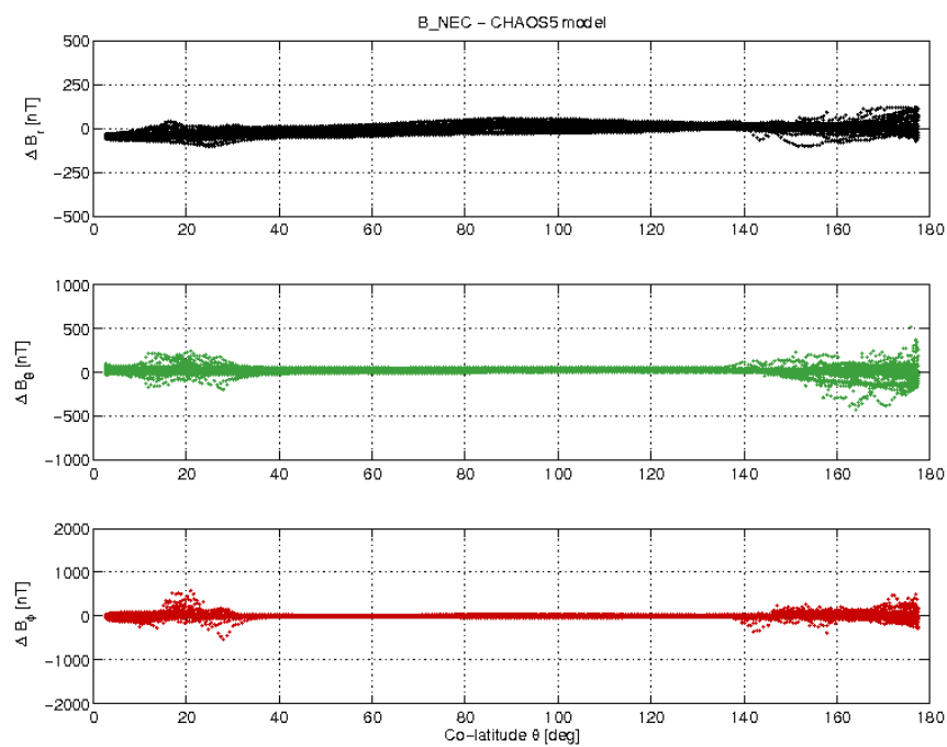
Figure 3-17: S/C A day 02/01 B_{NEC} - B_{Chaos} vs colatitude.
