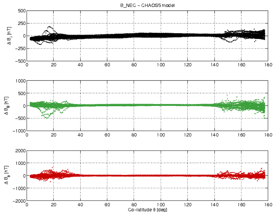
Figure 3-17: S/C A day 26/12 B_{NEC} - B_{Chaos5} vs colatitude.
