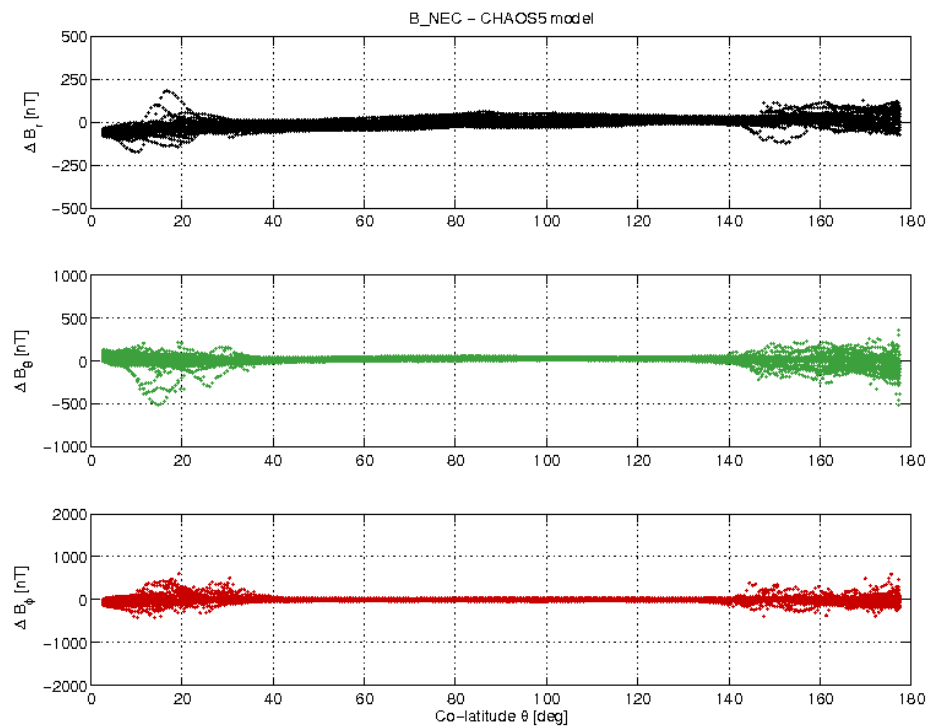
Figure 3-21: S/C C day 26/12 B_{NEC} - B_{Chaos} difference vs colatitude.
