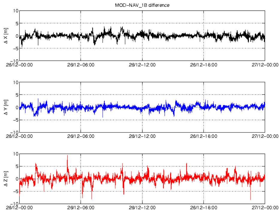
Figure 3-5: Difference MOD-GPSNAV, S/C C, 26/12. From top to bottom: X, Y and Z-axis
