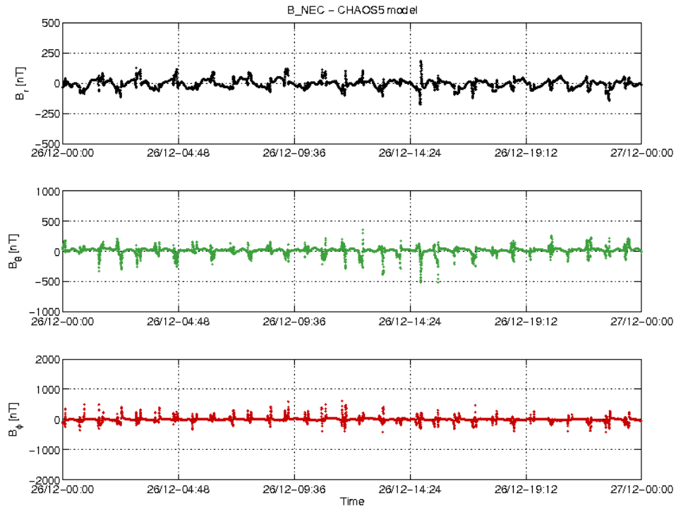
Figure 3-22: S/C C day 26/12 time series of B_{NEC} - B_{Chaos} residuals.
