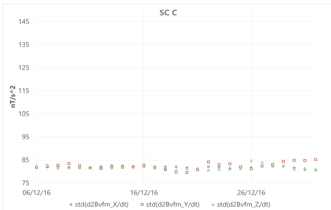
Figure 3-25: Plot of standard deviation of B components in VFM frames.
