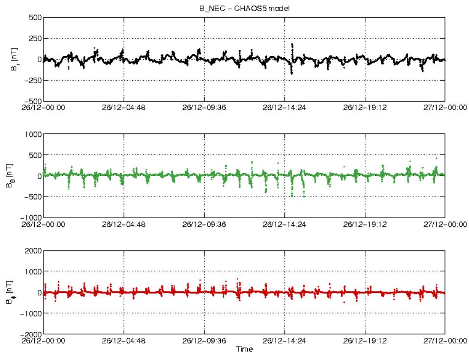
Figure 3-18: S/C A day 26/12: time series of B_{NEC} - B_{Chaos} residuals.
