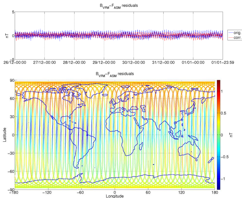
Figure 3-8: ASM-VFM residuals for S/C A, during monitoring period 26/12-01/01. In top figure are plotted: difference between |B_{VFM}| and F_{ASM} (without dB Sun correction) (blue colour), and the residuals with dB Sun corrections (red colour). In bottom figure residuals are presented on the world map.
