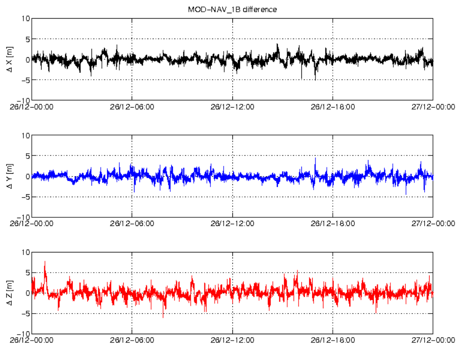
Figure 3-4: Difference MOD-GPSNAV, S/C B, 26/12. From top to bottom: X, Y and Z-axis
