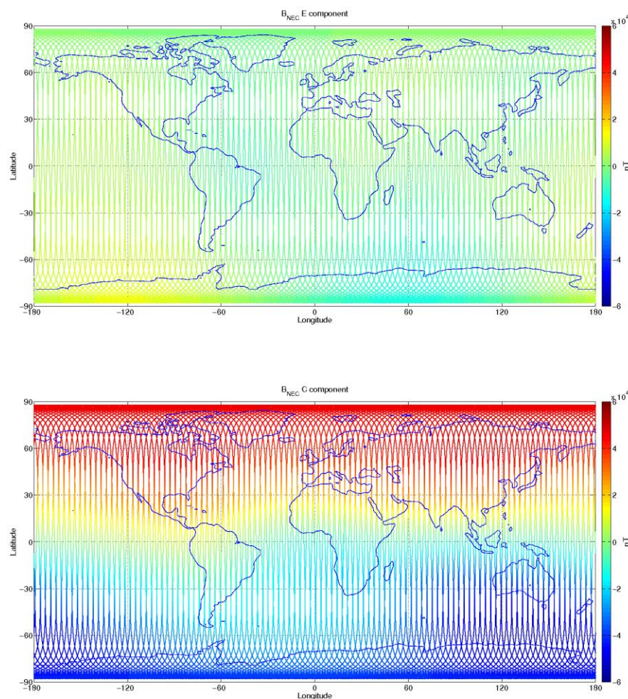
Figure 3-11: S/C B, world map plots of the geomagnetic field and components measured during monitoring period 26/12-01/01. From top to bottom: F-magnetic field from ASM measurement, B_{NEC} components (North, East, and Centre) of magnetic field from VFM measurement.
