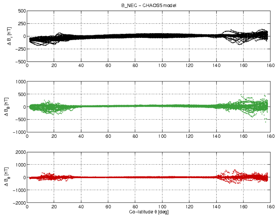
Figure 3-19: S/C B day 26/12 B_{\text{NEC}} - B_{\text{Chaos}} difference vs colatitude.
