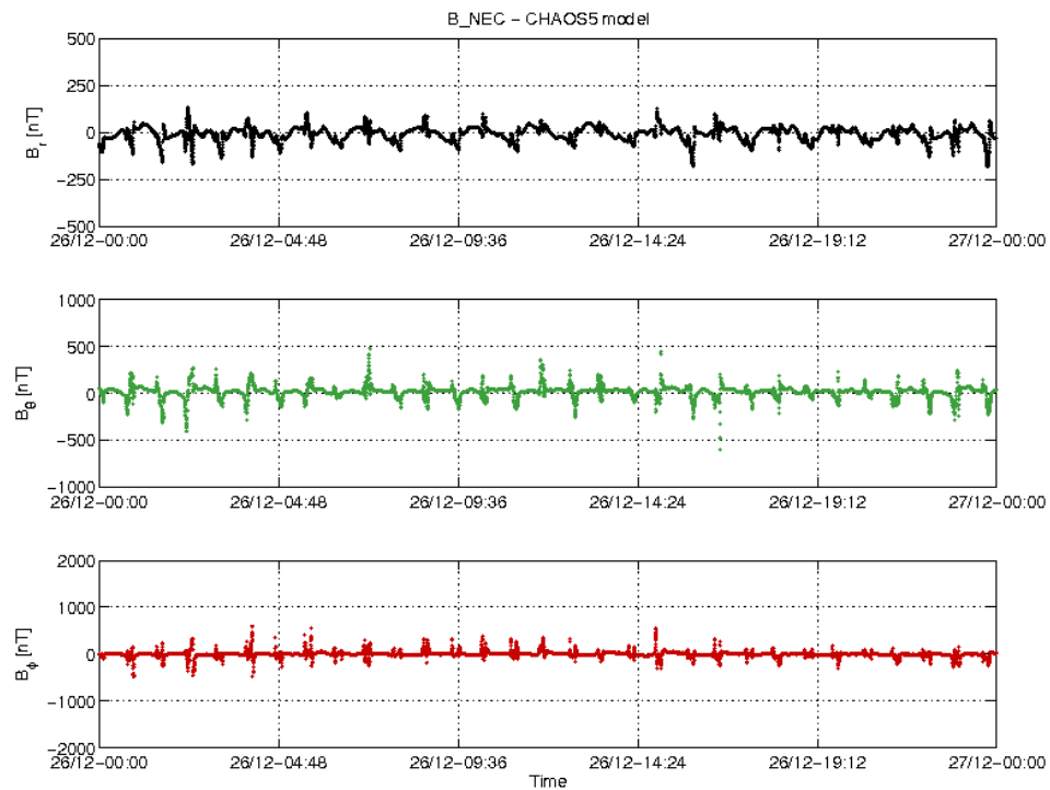
Figure 3-20: S/C B day 26/12 time series of B_{NEC} - B_{Chaos} residuals.
