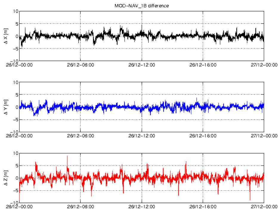
Figure 3-3: Difference MOD-GPSNAV, S/C A, 26/12. From top to bottom: X, Y and Z-axis
