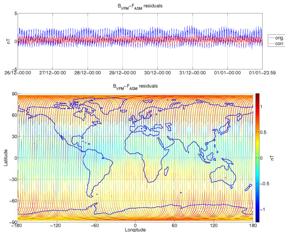
Figure 3-9: ASM-VFM residuals for S/C B, during monitoring period 26/12-01/01. In top figure are plotted: difference between |B_{VFM}| and F_{ASM} (without dB_Sun correction) (blue colour), and the residuals with dB_Sun corrections (red colour). In bottom figure residuals are presented on the world map.
