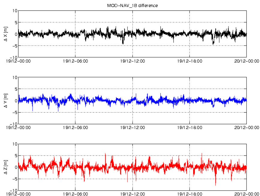
Figure 3-3: Difference MOD-GPSNAV, S/C A, 19/12. From top to bottom: X, Y and Z-axis
