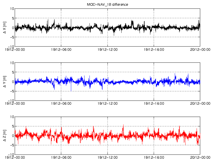
Figure 3-4: Difference MOD-GPSNAV, S/C B, 19/12. From top to bottom: X, Y and Z-axis
