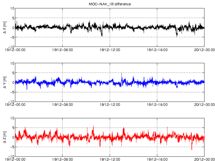
Figure 3-5: Difference MOD-GPSNAV, S/C C, 19/12. From top to bottom: X, Y and Z-axis
