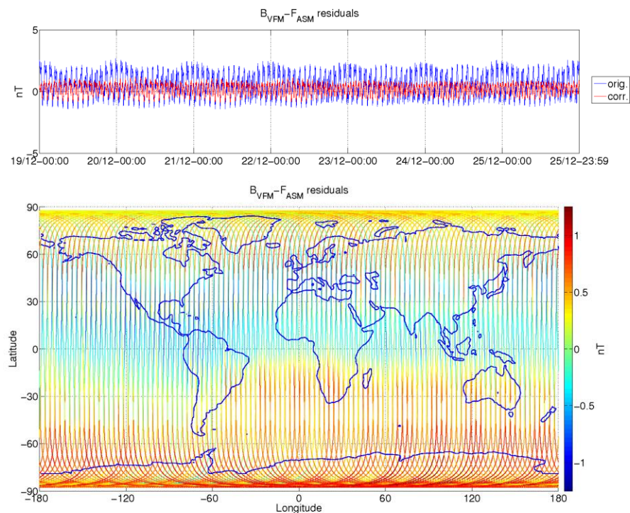
Figure 3-9: ASM-VFM residuals for S/C B, during monitoring period 19/12-25/12. In top figure are plotted: difference between |B_{VFM}| and F_{ASM} (without dB_{Sun} correction) (blue colour), and the residuals with dB_{Sun} corrections (red colour). In bottom figure residuals are presented on the world map.
