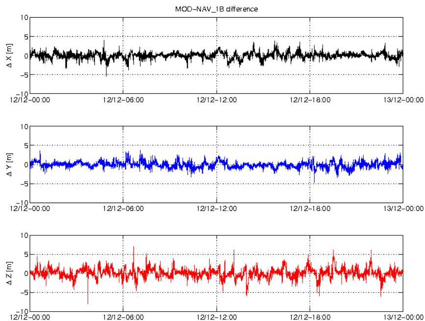
Figure 3-4: Difference MOD-GPSNAV, S/C B, 12/12. From top to bottom: X, Y and Z-axis
