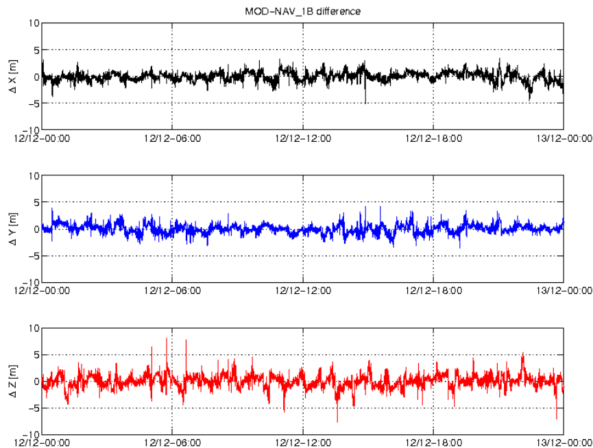
Figure 3-5: Difference MOD-GPSNAV, S/C C, 12/12. From top to bottom: X, Y and Z-axis
