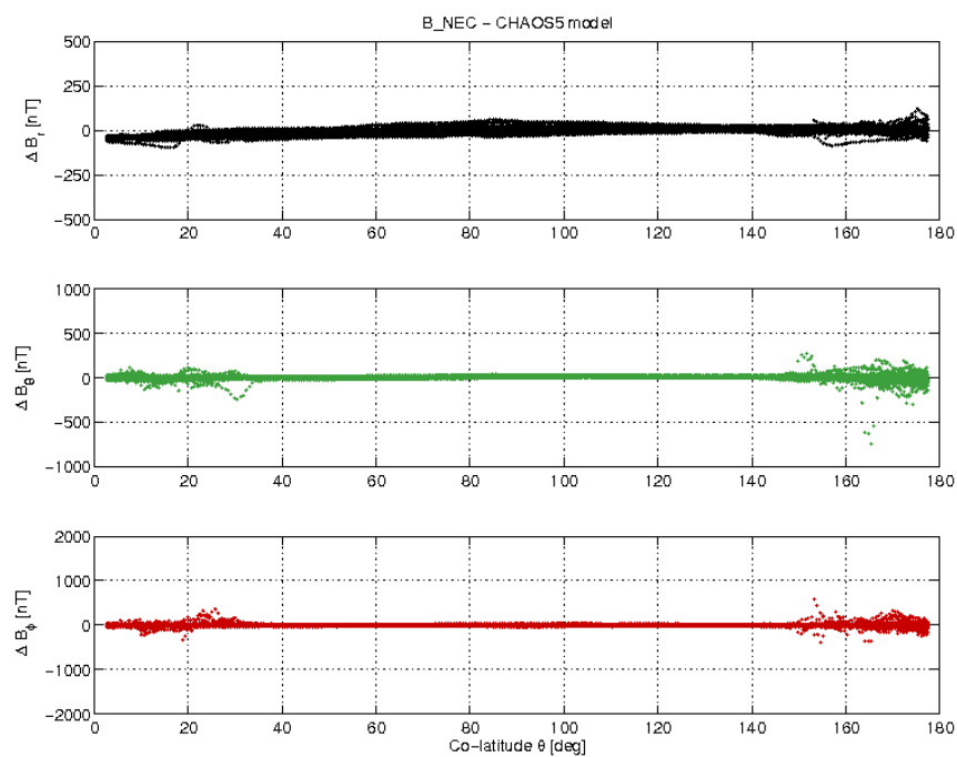
Figure 3-17: S/C A day 12/12 B_{NEC} - B_{Chaos} vs colatitude.
