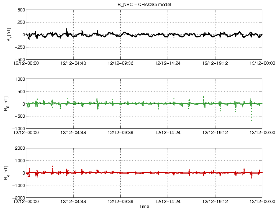
Figure 3-22: S/C C day 12/12 time series of B_{NEC} - B_{Chaos} residuals.
