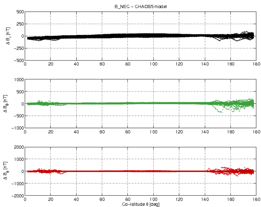
Figure 3-19: S/C B day 12/12 B_{NEC} - B_{Chao5} difference vs colatitude.
