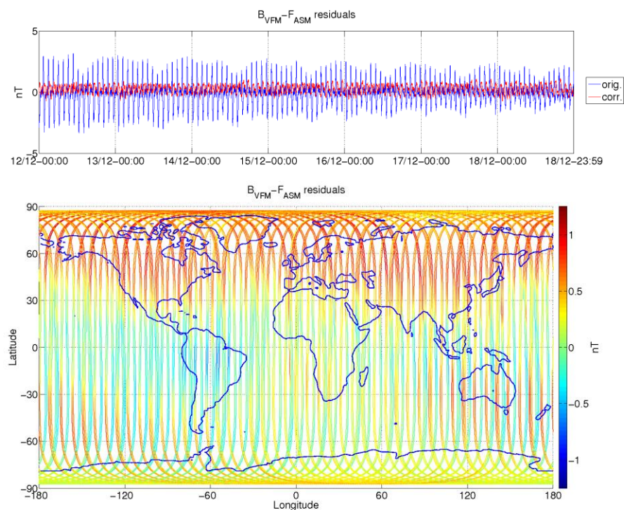
Figure 3-8: ASM-VFM residuals for S/C A, during monitoring period 12/12-18/12. In top figure are plotted: difference between |B_{VFM}| and F_{ASM} (without dB_Sun correction) (blue colour), and the residuals with dB_Sun corrections (red colour). In bottom figure residuals are presented on the world map.
