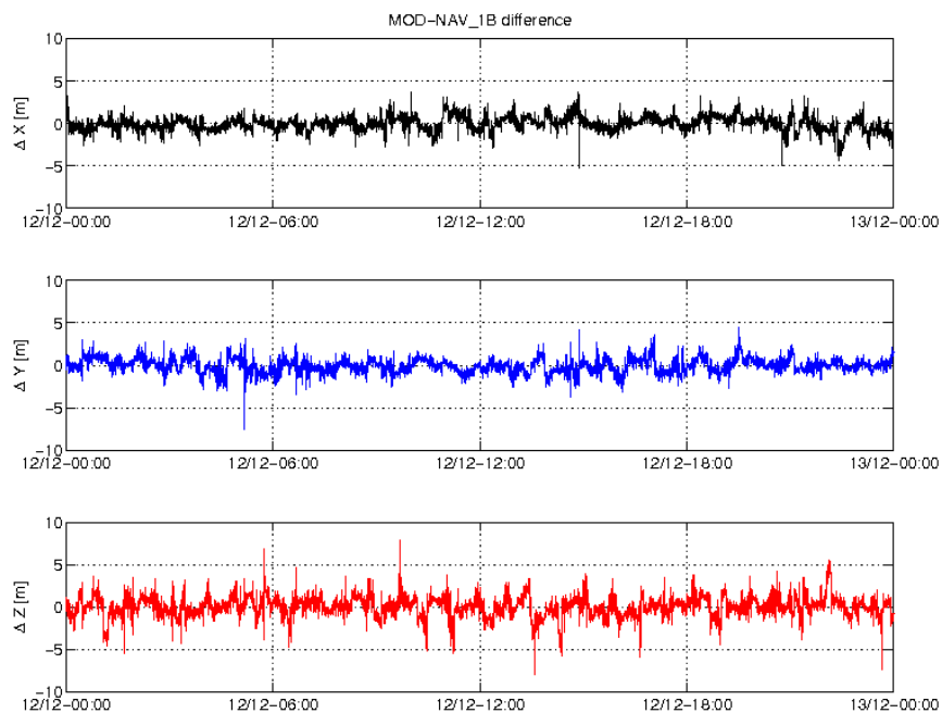
Figure 3-3: Difference MOD-GPSNAV, S/C A, 12/12. From top to bottom: X, Y and Z-axis
