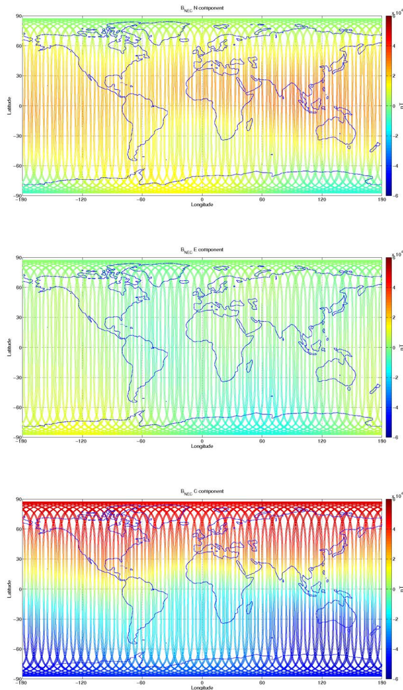
Figure 3-12: S/C C, world map plots of the geomagnetic field and components measured during monitoring period 12/12-18/12. From top to bottom: B_{NEC} components (North, East, and Centre) of magnetic field from VFM measurement.
