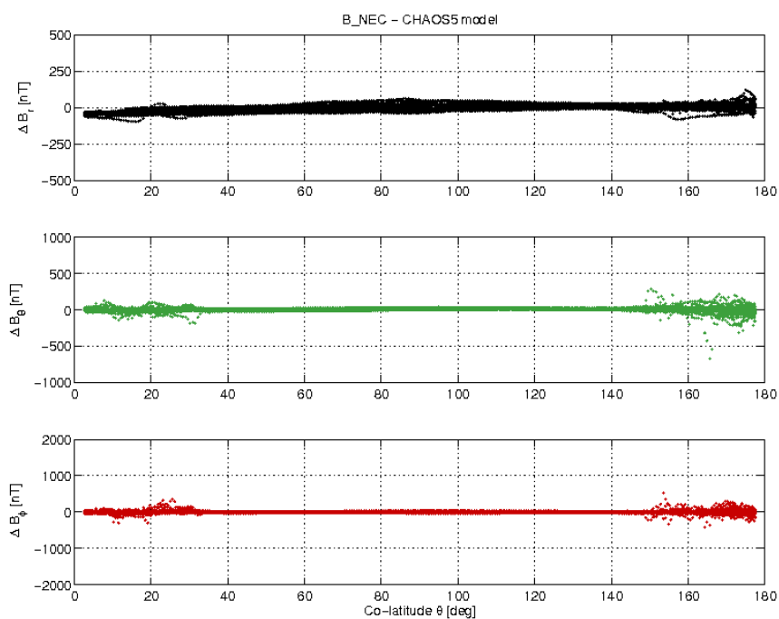
Figure 3-21: S/C C day 12/12 B_{NEC} - B_{Chao5} difference vs colatitude.
