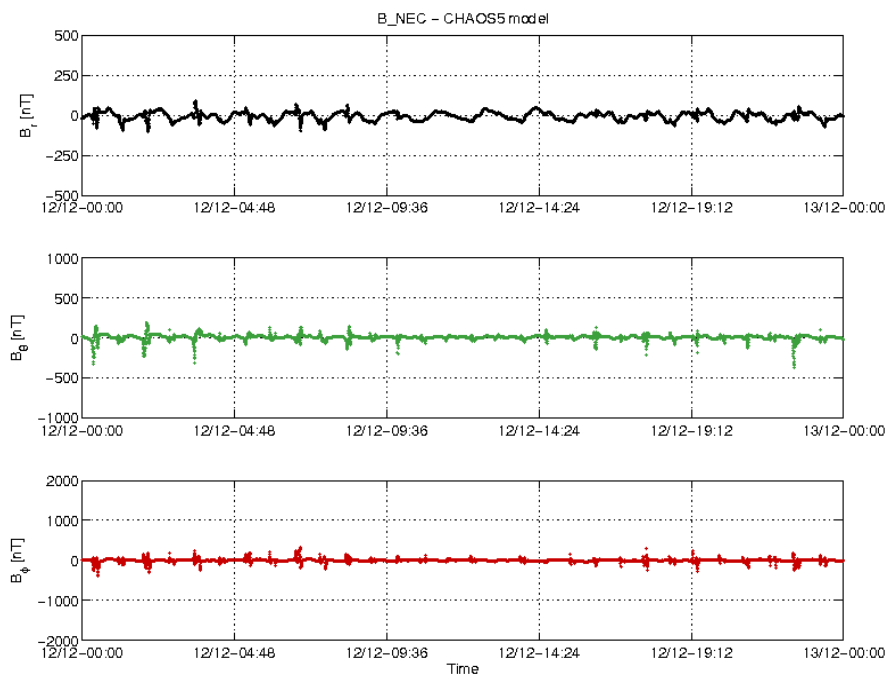
Figure 3-20: S/C B day 12/12 time series of B_{NEC} - B_{Chao5} residuals.
