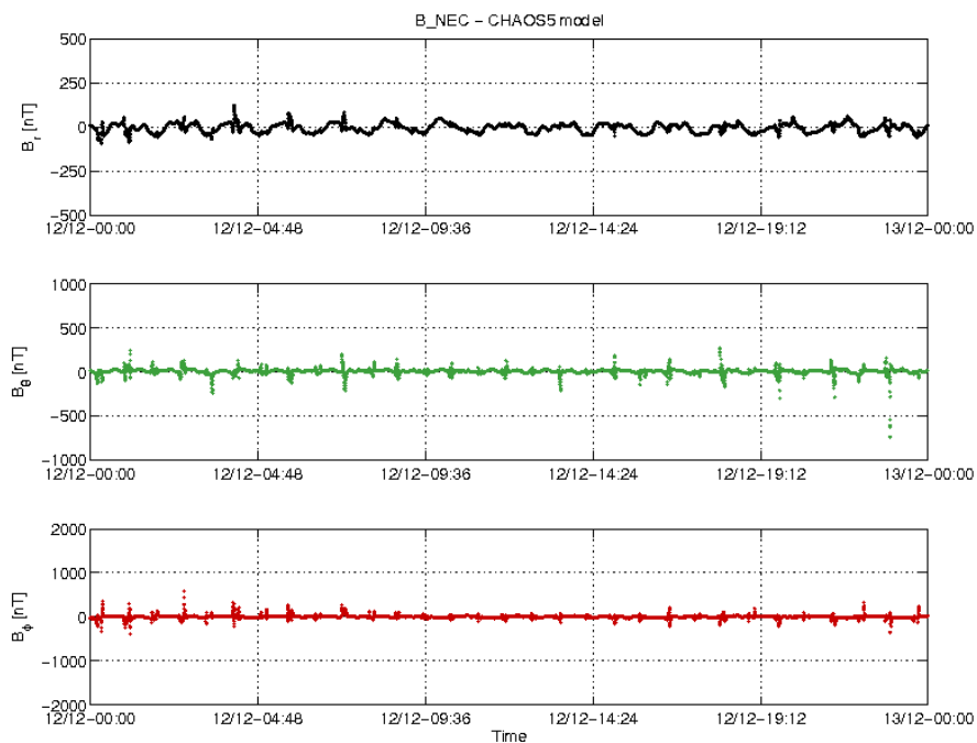
Figure 3-18: S/C A day 12/12: time series of B_{NEC} - B_{Chao5} residuals.
