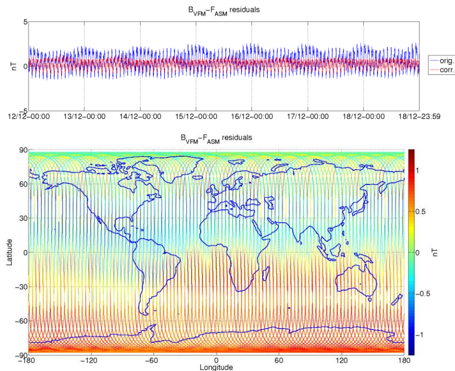
Figure 3-9: ASM-VFM residuals for S/C B, during monitoring period 12/12-18/12. In top figure are plotted: difference between |B_{VFM}| and F_{ASM} (without dB_{Sun} correction) (blue colour), and the residuals with dB_{Sun} corrections (red colour). In bottom figure residuals are presented on the world map.
