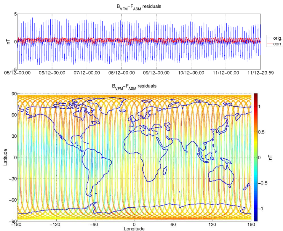
Figure 3-8: ASM-VFM residuals for S/C A, during monitoring period 05/12-11/12. In top figure are plotted: difference between |B_{VFM}| and F_{ASM} (without dB_Sun correction) (blue colour), and the residuals with dB_Sun corrections (red colour). In bottom figure residuals are presented on the world map.
