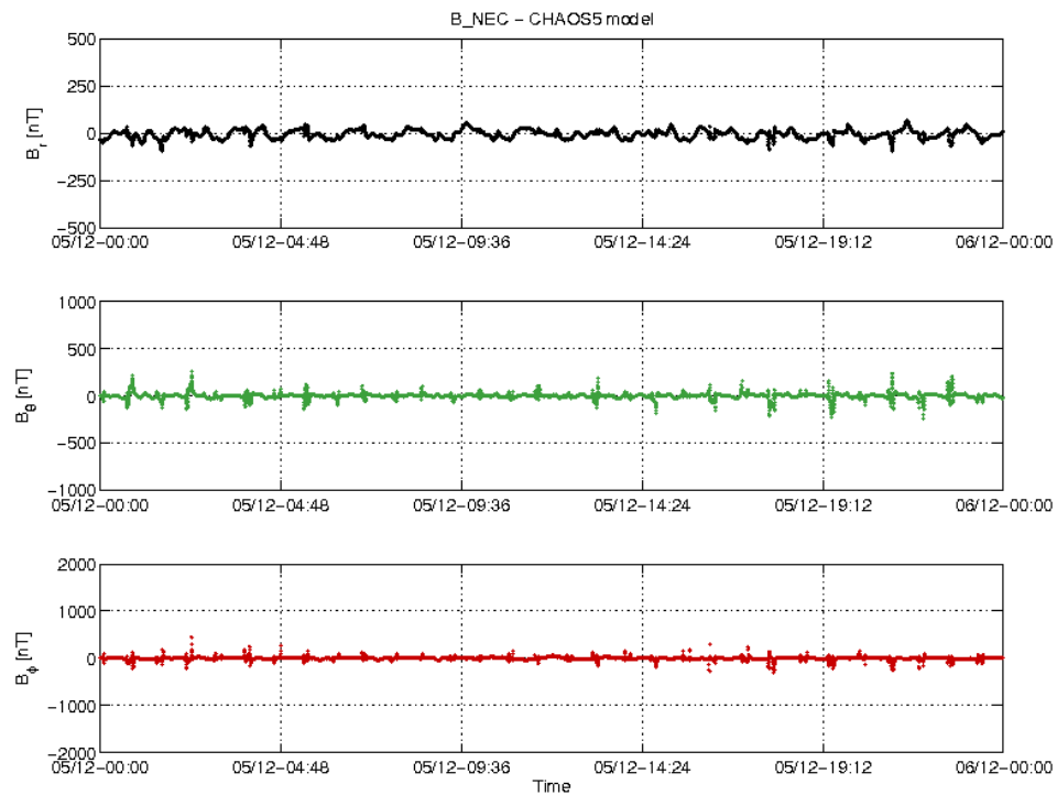
Figure 3-18: S/C A day 05/12: time series of B_{NEC} - B_{Chaos} residuals.
