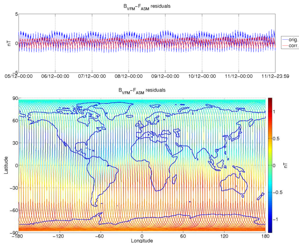
Figure 3-9: ASM-VFM residuals for S/C B, during monitoring period 05/12-11/12. In top figure are plotted: difference between |B_{VFM}| and F_{ASM} (without dB_{Sun} correction) (blue colour), and the residuals with dB_{Sun} corrections (red colour). In bottom figure residuals are presented on the world map.
