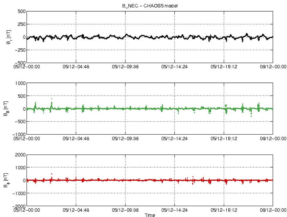
Figure 3-22: S/C C day 05/12 time series of B_{\text{NEC}} - B_{\text{Chaos}} residuals.
