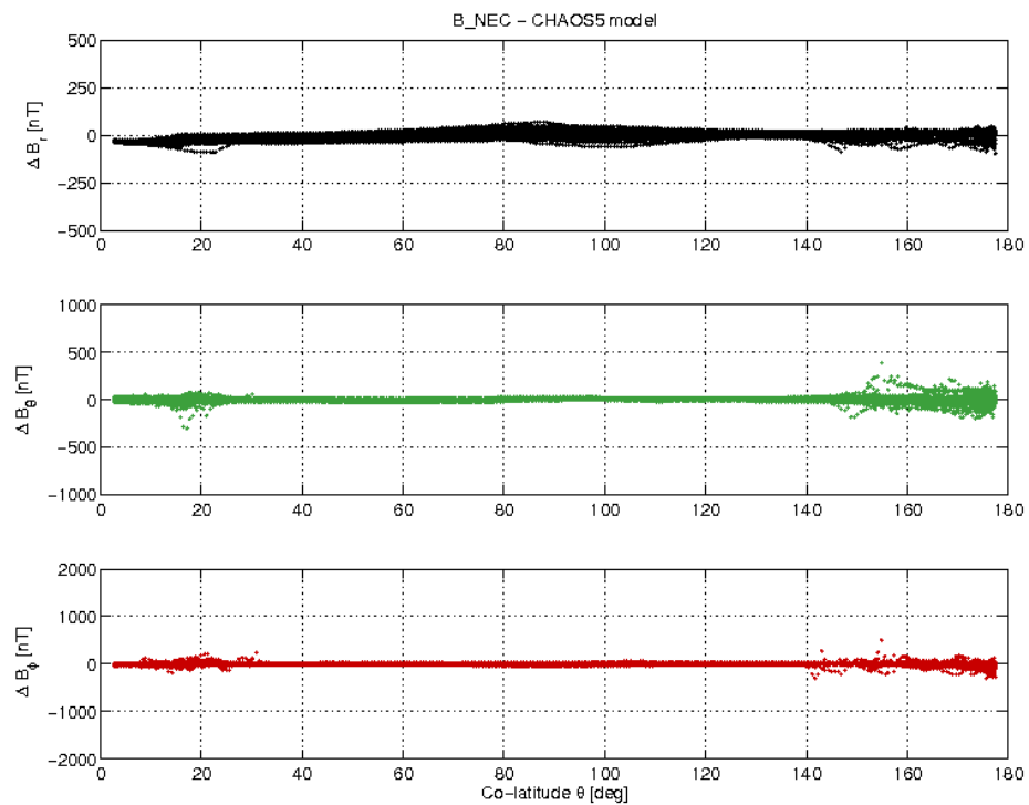
Figure 3-21: S/C C day 05/12 B_{\text{NEC}} - B_{\text{Chaos}} difference vs colatitude.
