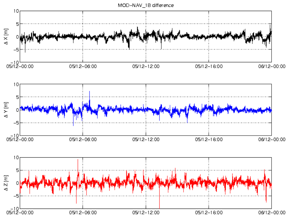
Figure 3-5: Difference MOD-GPSNAV, S/C C, 05/12. From top to bottom: X, Y and Z-axis
