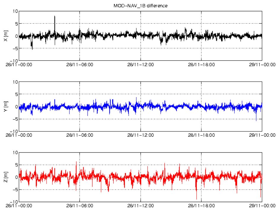
Figure 3-4: Difference MOD-GPSNAV, S/C B, 28/11. From top to bottom: X, Y and Z-axis
