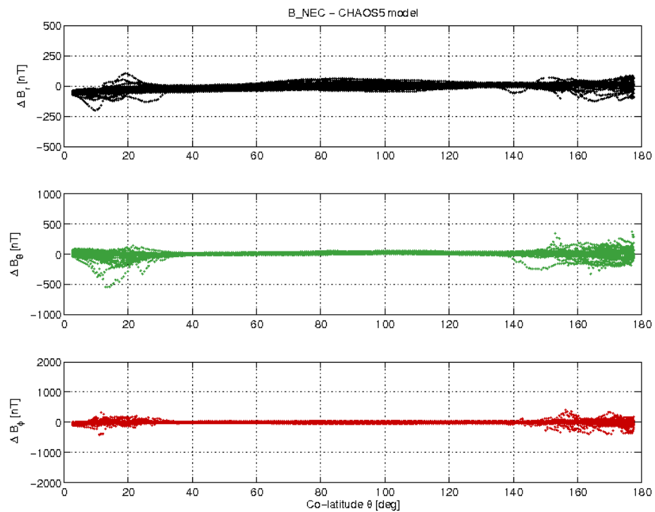
Figure 3-21: S/C C day 28/11 B_{NEC} - B_{Chaos} difference vs colatitude.
