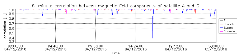
Figure 3-13: Correlation in magnetic data between satellite A and C for B_{north} , B_{east} , and B_{center} components of B_{NEC} are the components of the magnetic field vector in NEC frame
