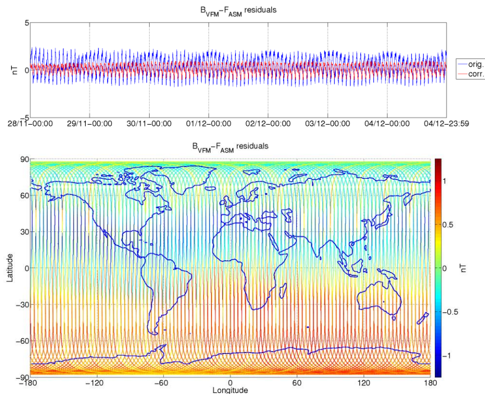
Figure 3-9: ASM-VFM residuals for S/C B, during monitoring period 28/11-04/12. In top figure are plotted: difference between |B_{VFM}| and F_{ASM} (without dB_{Sun} correction) (blue colour), and the residuals with dB_{Sun} corrections (red colour). In bottom figure residuals are presented on the world map.
