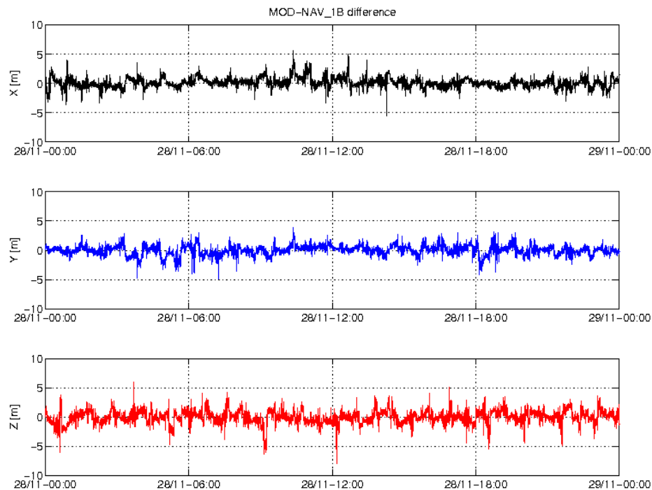
Figure 3-5: Difference MOD-GPSNAV, S/C C, 28/11. From top to bottom: X, Y and Z-axis
