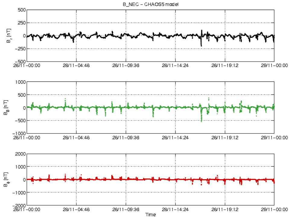
Figure 3-22: S/C C day 28/11 time series of B_{NEC} - B_{Chaos} residuals.
