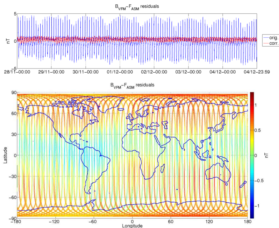
Figure 3-8: ASM-VFM residuals for S/C A, during monitoring period 28/11-04/12. In top figure are plotted: difference between |B_{VFM}| and F_{ASM} (without dB_{Sun} correction) (blue colour), and the residuals with dB_{Sun} corrections (red colour). In bottom figure residuals are presented on the world map.
