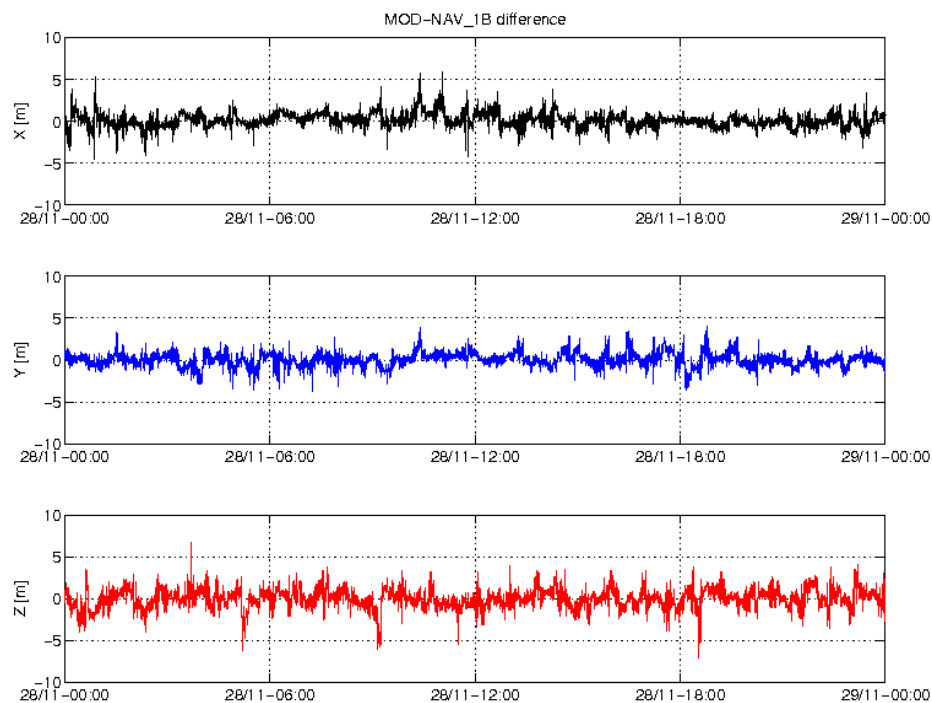
Figure 3-3: Difference MOD-GPSNAV, S/C A, 28/11. From top to bottom: X, Y and Z-axis
