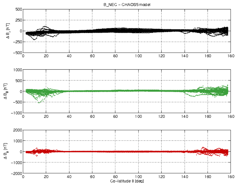
Figure 3-17: S/C A day 28/11 B_{NEC} - B_{Chaos} vs colatitude.
