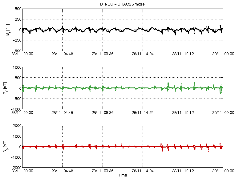
Figure 3-20: S/C B day 28/11 time series of B_{NEC} - B_{Chaos} residuals.
