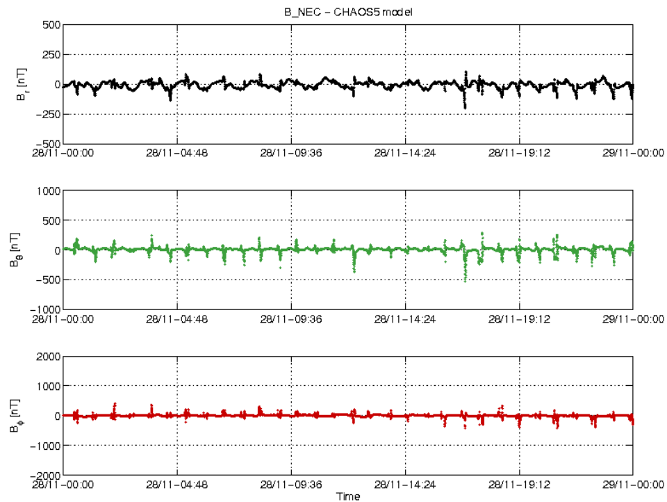
Figure 3-18: S/C A day 28/11: time series of B_{NEC} - B_{Chaos} residuals.
