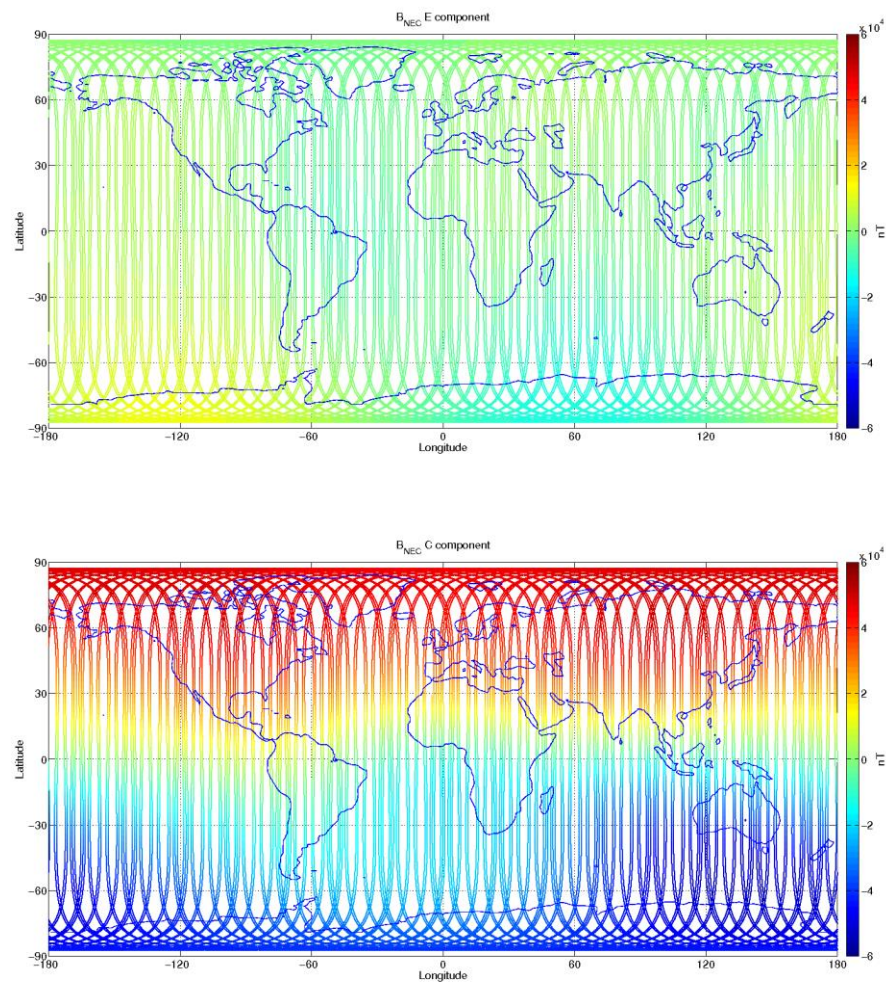
Figure 3-10: S/C A, world map plots of the geomagnetic field and components measured during monitoring period 28/11-04/12. From top to bottom: F-magnetic field from ASM measurement, B_{NEC} components (North, East, and Centre) of magnetic field from VFM measurement.
