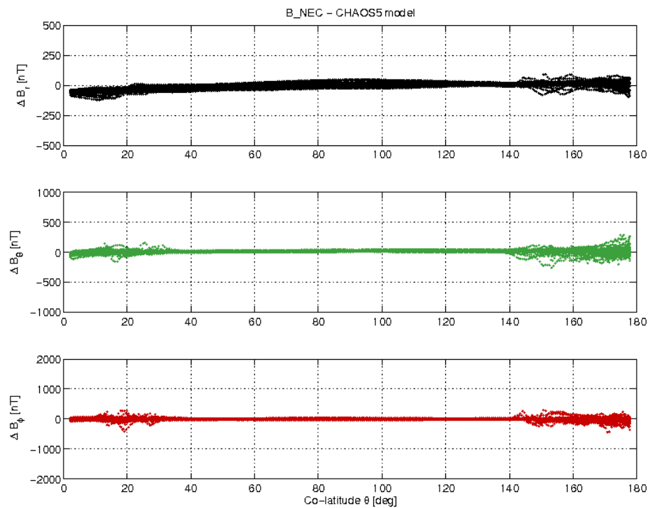
Figure 3-19: S/C B day 28/11 B_{NEC} - B_{Chaos} difference vs colatitude.
