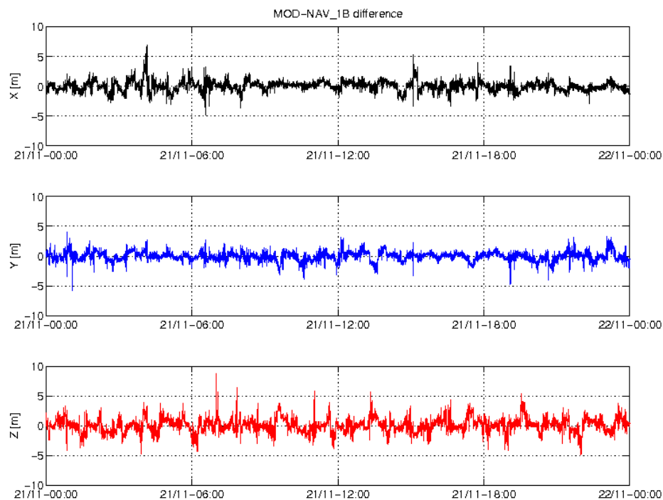
Figure 3-4: Difference MOD-GPSNAV, S/C B, 21/11. From top to bottom: X, Y and Z-axis
