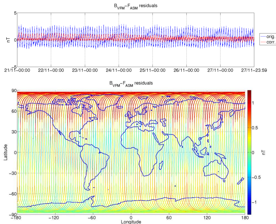
Figure 3-9: ASM-VFM residuals for S/C B, during monitoring period 21/11-27/11. In top figure are plotted: difference between |B_{VFM}| and F_{ASM} (without dB_{Sun} correction) (blue colour), and the residuals with dB_{Sun} corrections (red colour). In bottom figure residuals are presented on the world map.
