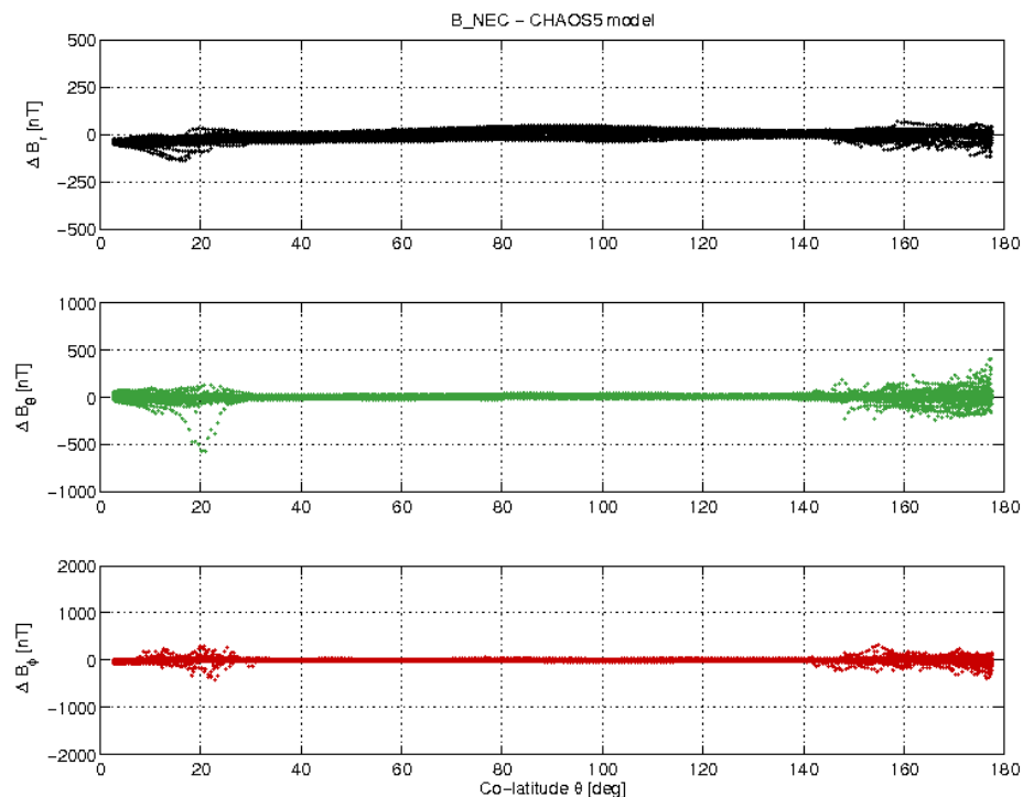
Figure 3-17: S/C A day 21/11 B_{NEC} - B_{Chaos} vs colatitude.
