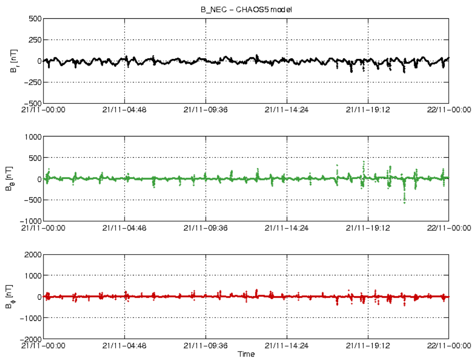
Figure 3-18: S/C A day 21/11: time series of B_{NEC} - B_{Chaos} residuals.
