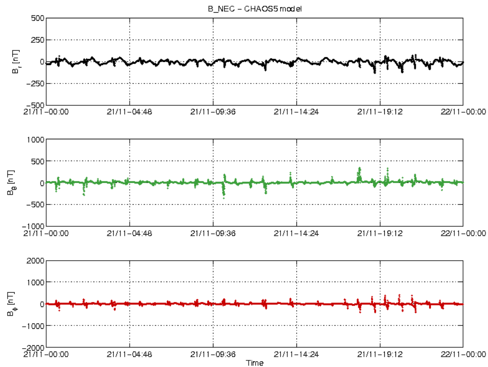
Figure 3-20: S/C B day 21/11 time series of B_{NEC} - B_{Chaos} residuals.
