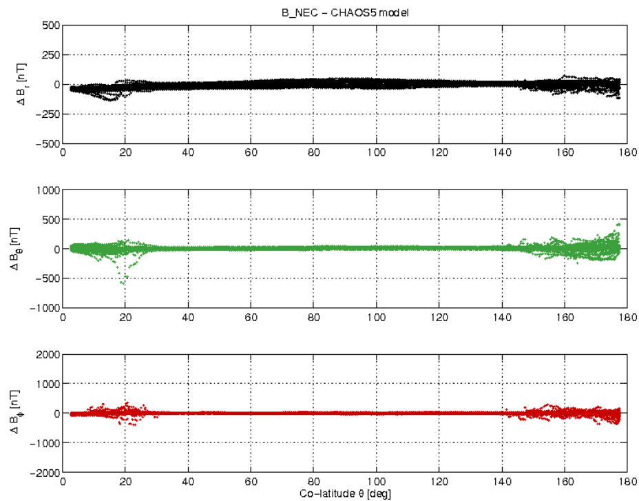
Figure 3-21: S/C C day 21/11 B_{\text{NEC}} - B_{\text{Chaos}} difference vs colatitude.
