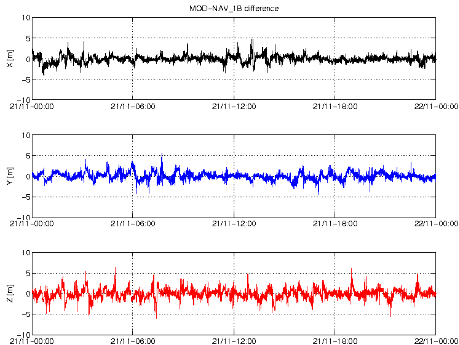
Figure 3-5: Difference MOD-GPSNAV, S/C C, 21/11. From top to bottom: X, Y and Z-axis
