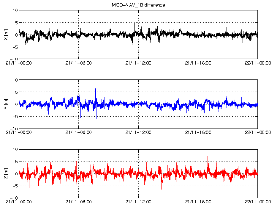
Figure 3-3: Difference MOD-GPSNAV, S/C A, 21/11. From top to bottom: X, Y and Z-axis
