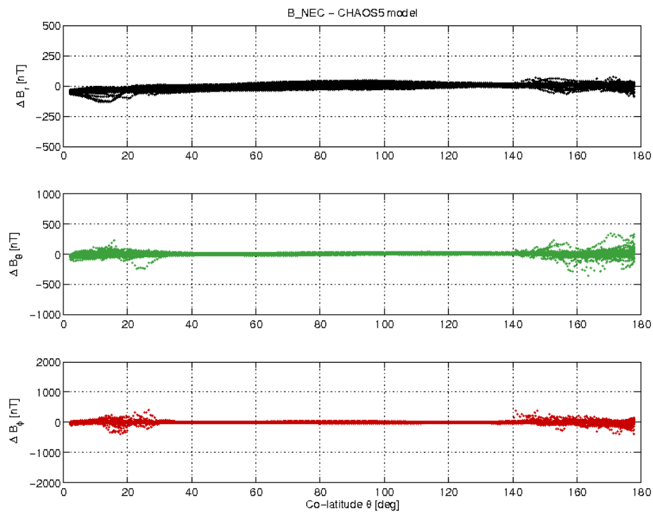
Figure 3-19: S/C B day 21/11 B_{NEC} - B_{Chaos} difference vs colatitude.
