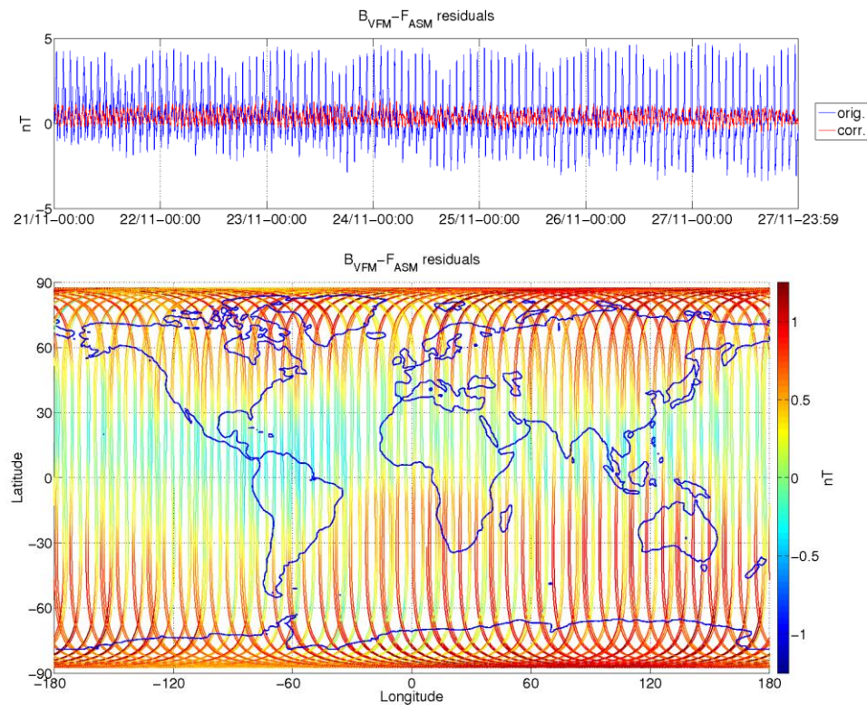
Figure 3-8: ASM-VFM residuals for S/C A, during monitoring period 21/11-27/11. In top figure are plotted: difference between |B_{VFM}| and F_{ASM} (without dB_{Sun} correction) (blue colour), and the residuals with dB_{Sun} corrections (red colour). In bottom figure residuals are presented on the world map.
