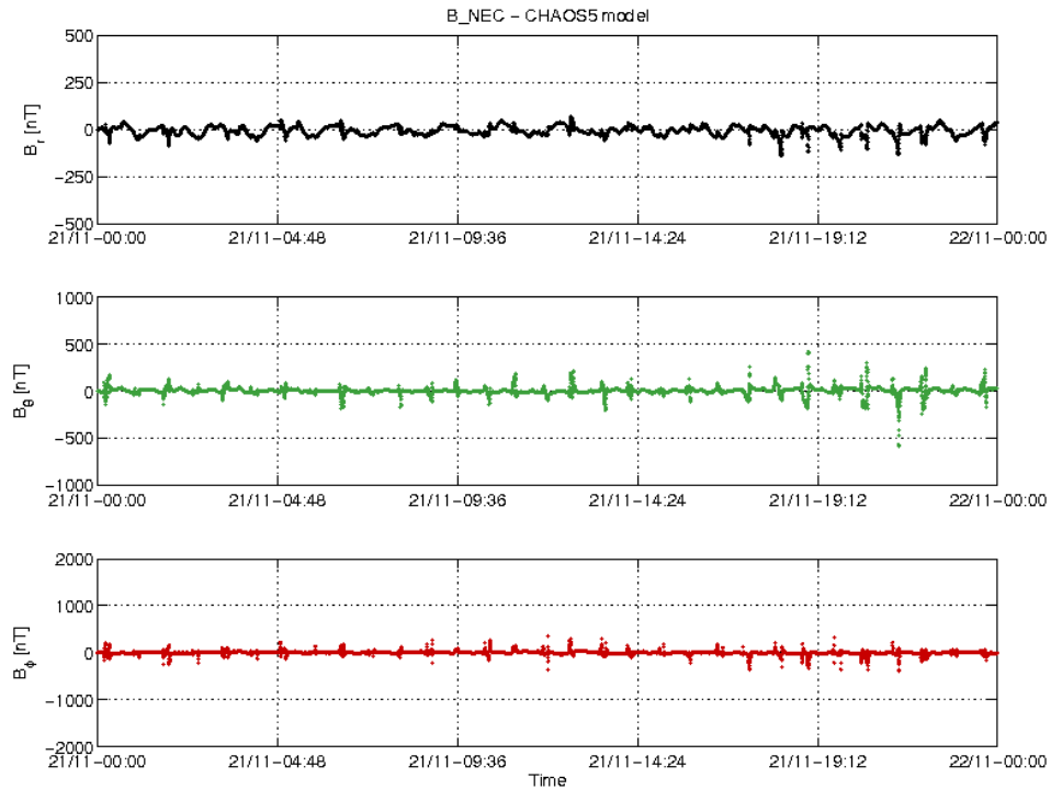
Figure 3-22: S/C C day 21/11 time series of B_{NEC} - B_{Chaos} residuals.
