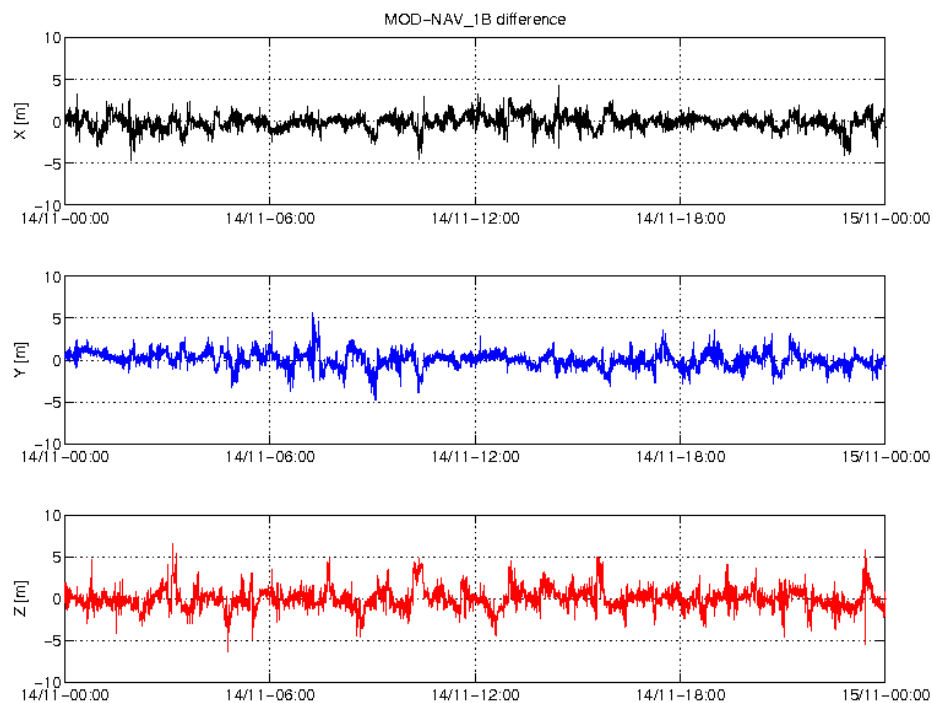
Figure 3-3: Difference MOD-GPSNAV, S/C A, 14/11. From top to bottom: X, Y and Z-axis
