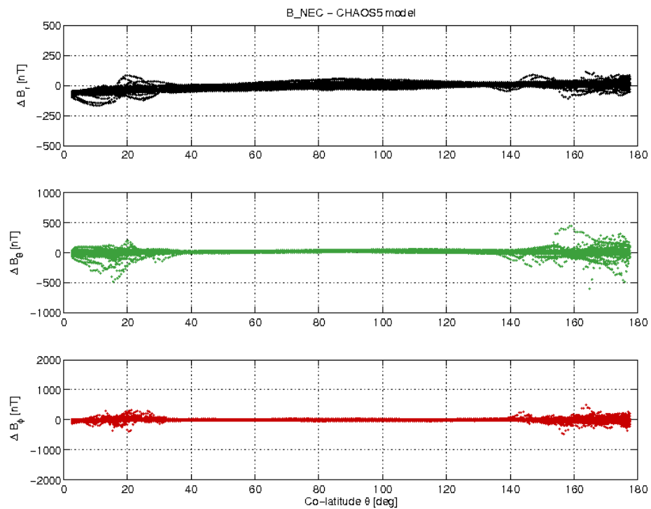
Figure 3-21: S/C C day 14/11 B_{\text{NEC}} - B_{\text{Chaos}} difference vs colatitude.
