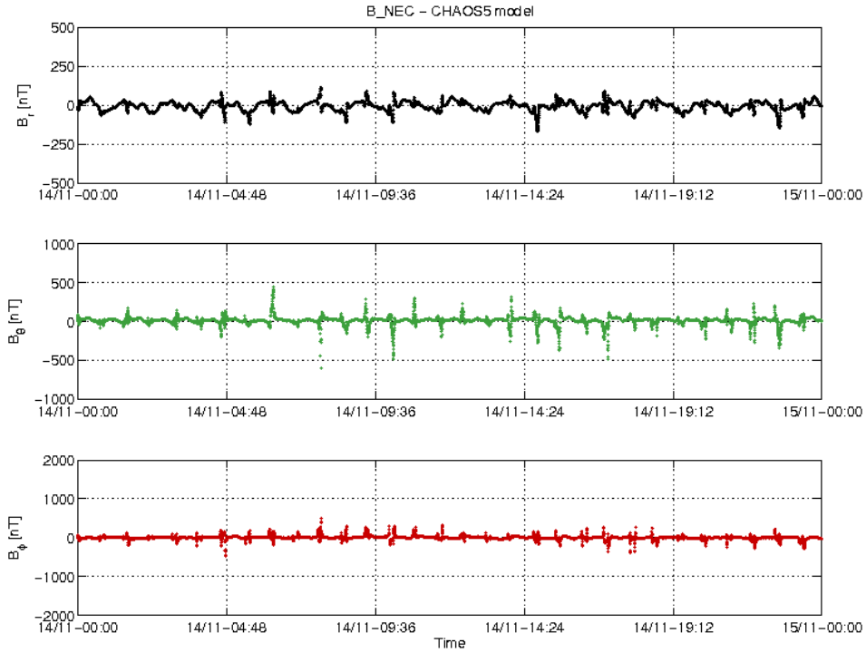
Figure 3-22: S/C C day 14/11 time series of B_{NEC} - B_{Chaos} residuals.
