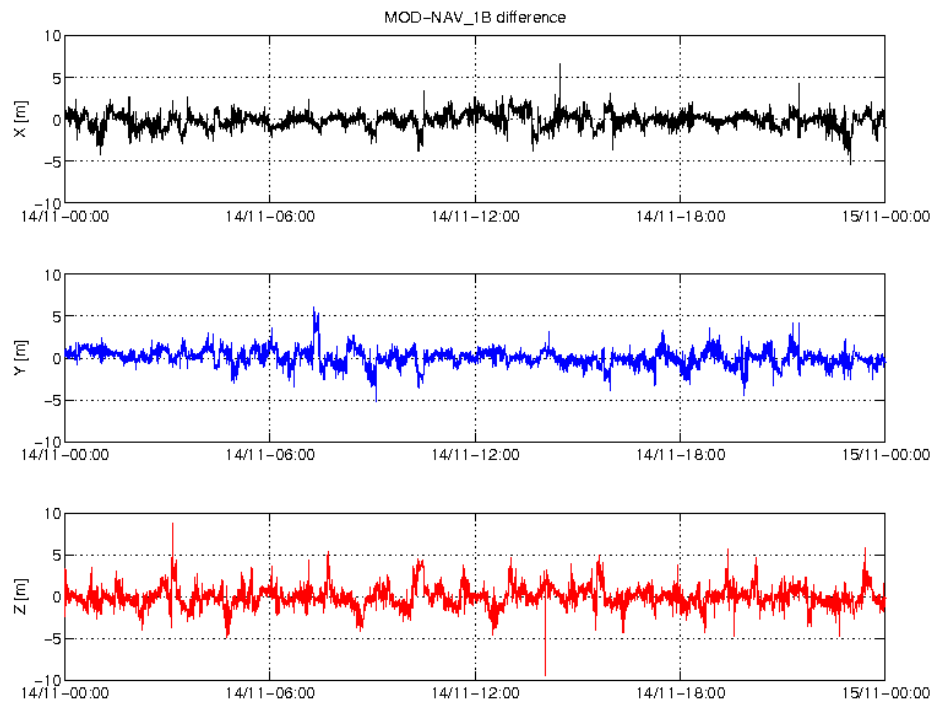
Figure 3-5: Difference MOD-GPSNAV, S/C C, 14/11. From top to bottom: X, Y and Z-axis
