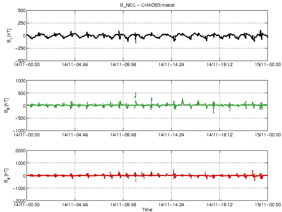
Figure 3-20: S/C B day 14/11 time series of B_{NEC} - B_{Chaos} residuals.
