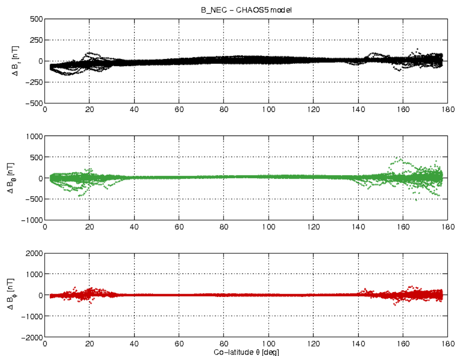
Figure 3-17: S/C A day 14/11 B_{NEC} - B_{Chaos} vs colatitude.
