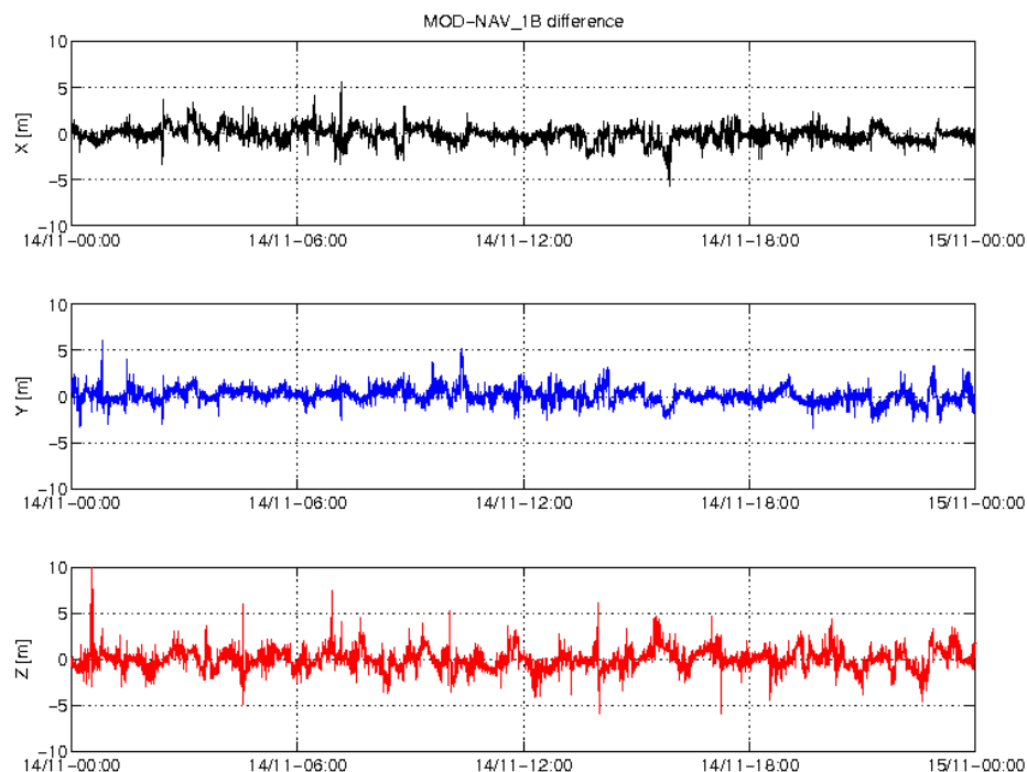
Figure 3-4: Difference MOD-GPSNAV, S/C B, 14/11. From top to bottom: X, Y and Z-axis
