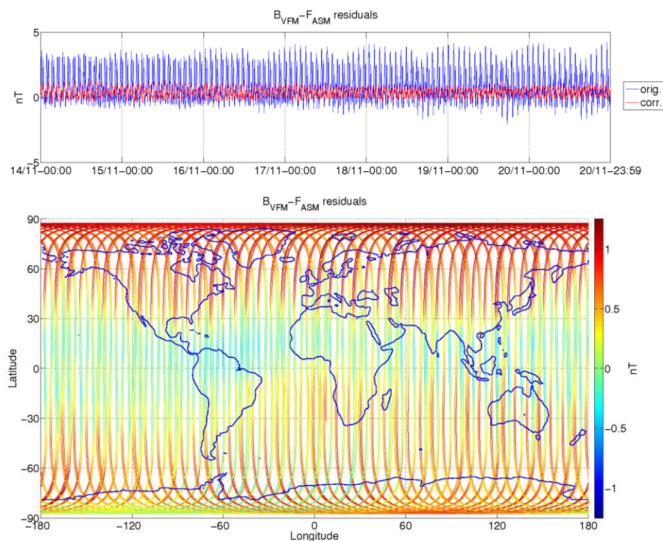
Figure 3-8: ASM-VFM residuals for S/C A, during monitoring period 14/11-20/11. In top figure are plotted: difference between |B_{VFM}| and F_{ASM} (without dB_{Sun} correction) (blue colour), and the residuals with dB_{Sun} corrections (red colour). In bottom figure residuals are presented on the world map.
