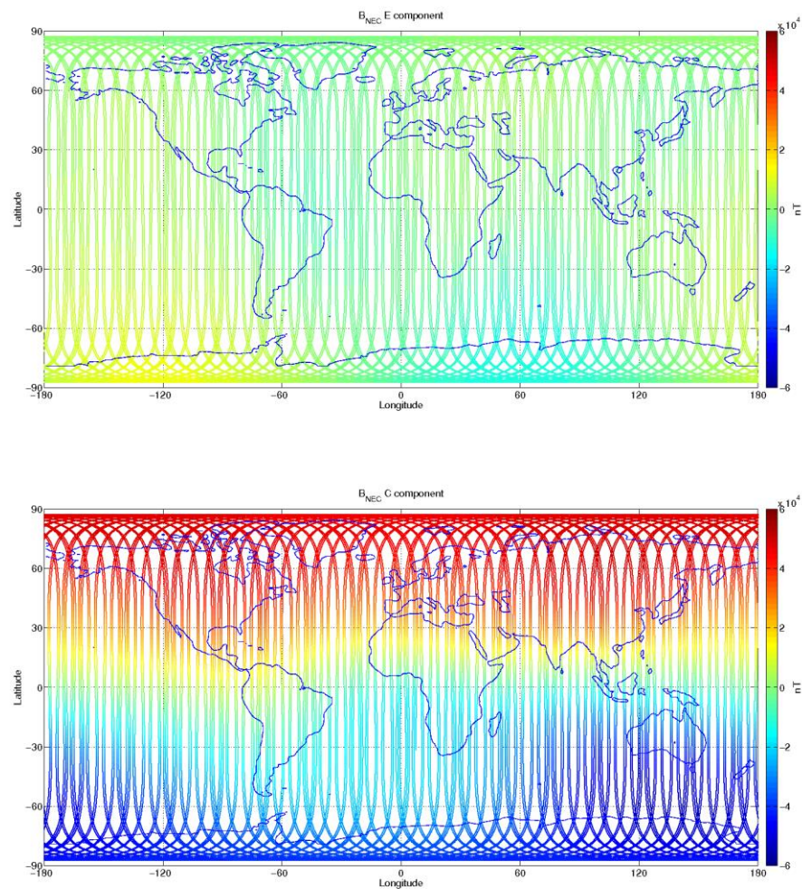
Figure 3-10: S/C A, world map plots of the geomagnetic field and components measured during monitoring period 14/11-20/11. From top to bottom: F-magnetic field from ASM measurement, B_{NEC} components (North, East, and Centre) of magnetic field from VFM measurement.
