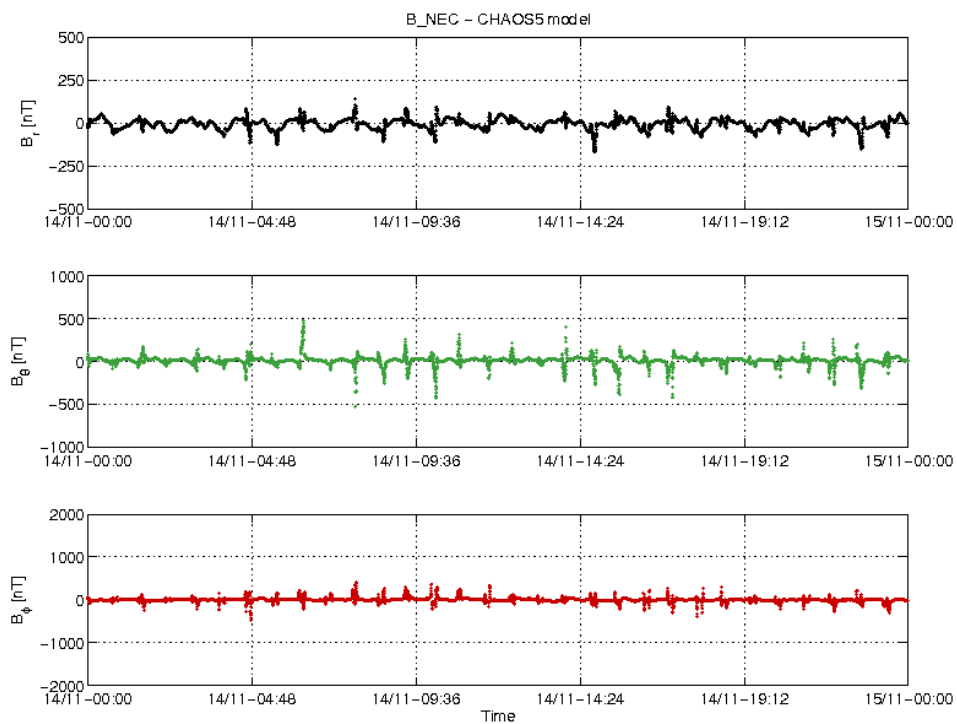
Figure 3-18: S/C A day 14/11: time series of B_{NEC} - B_{Chaos} residuals.
