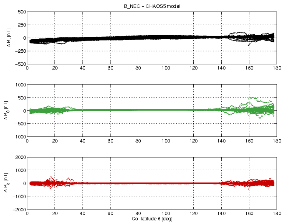
Figure 3-19: S/C B day 14/11 B_{NEC} - B_{Chaos} difference vs colatitude.
