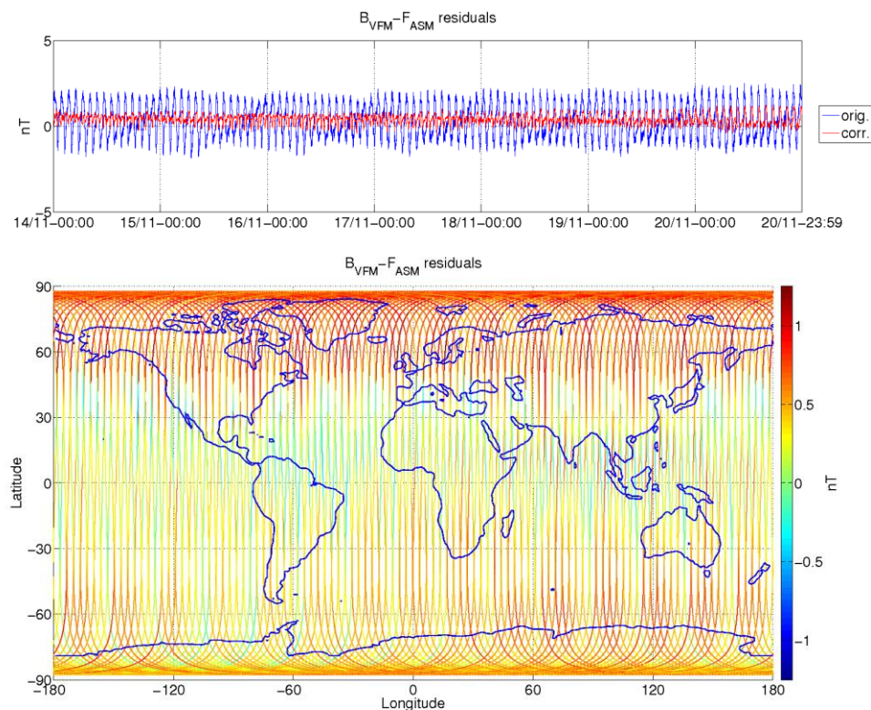
Figure 3-9: ASM-VFM residuals for S/C B, during monitoring period 14/11-20/11. In top figure are plotted: difference between |B_{VFM}| and F_{ASM} (without dB_Sun correction) (blue colour), and the residuals with dB_Sun corrections (red colour). In bottom figure residuals are presented on the world map.
