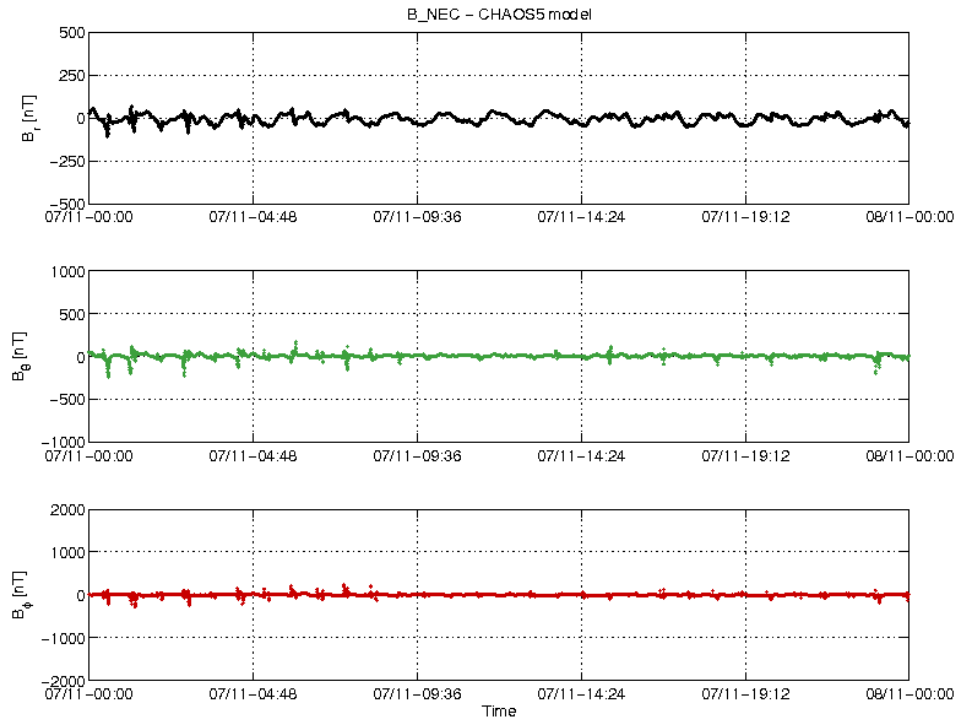
Figure 3-22: S/C C day 07/11 time series of B_{NEC} - B_{Chaos} residuals.
