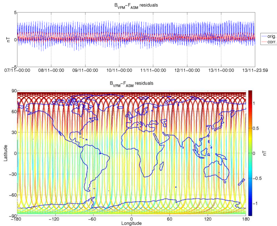
Figure 3-8: ASM-VFM residuals for S/C A, during monitoring period 07/11-13/11. In top figure are plotted: difference between |B_{VFM}| and F_{ASM} (without dB_{Sun} correction) (blue colour), and the residuals with dB_{Sun} corrections (red colour). In bottom figure residuals are presented on the world map.
