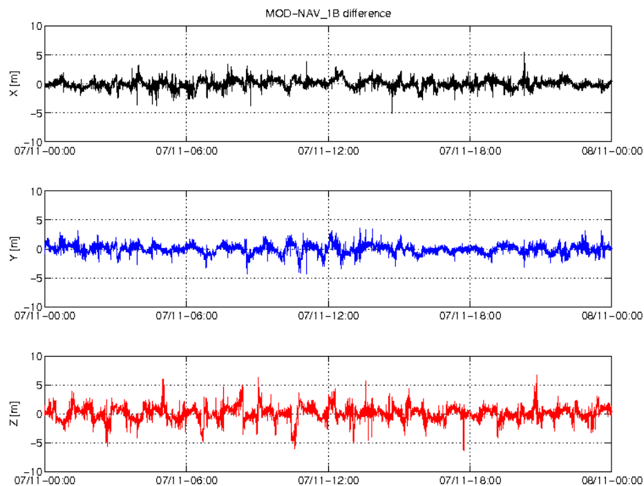
Figure 3-4: Difference MOD-GPSNAV, S/C B, 07/11. From top to bottom: X, Y and Z-axis
