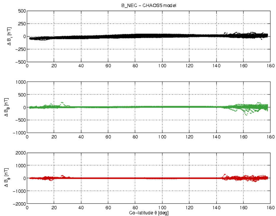
Figure 3-19: S/C B day 07/11 B_{NEC} - B_{CHAOS5} difference vs colatitude.
