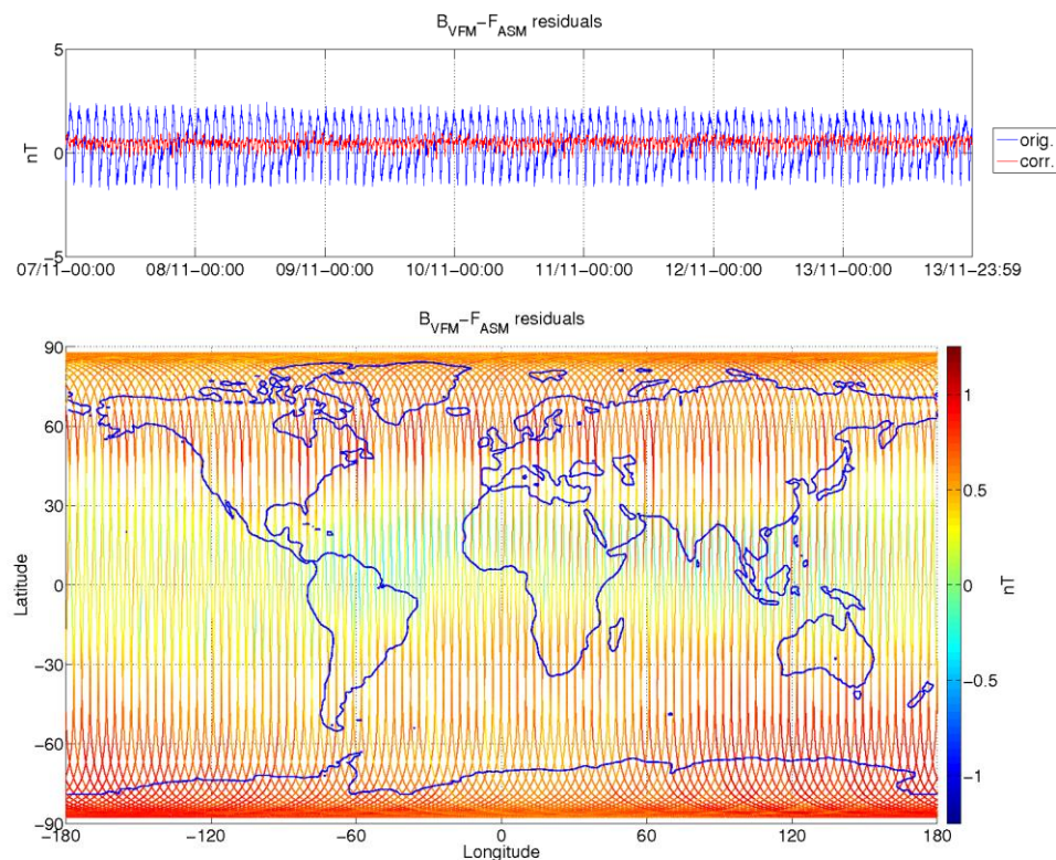
Figure 3-9: ASM-VFM residuals for S/C B, during monitoring period 07/11-13/11. In top figure are plotted: difference between |B_{VFM}| and F_{ASM} (without dB_Sun correction) (blue colour), and the residuals with dB_Sun corrections (red colour). In bottom figure residuals are presented on the world map.
