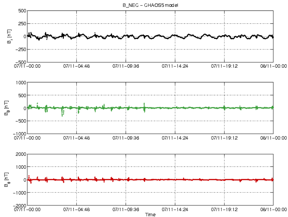
Figure 3-20: S/C B day 07/11 time series of B_{NEC} - B_{Chaos} residuals.
