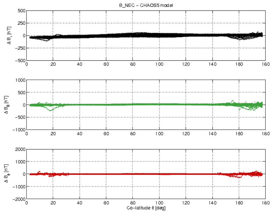
Figure 3-21: S/C C day 07/11 B_{NEC} - B_{Chaos} difference vs colatitude.
