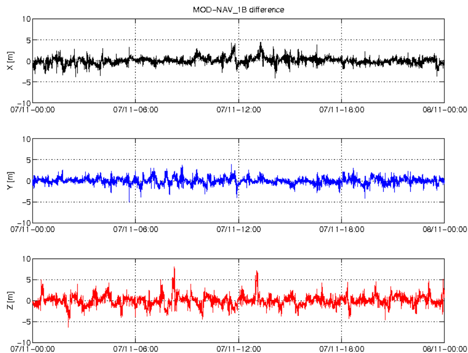
Figure 3-3: Difference MOD-GPSNAV, S/C A, 07/11. From top to bottom: X, Y and Z-axis
