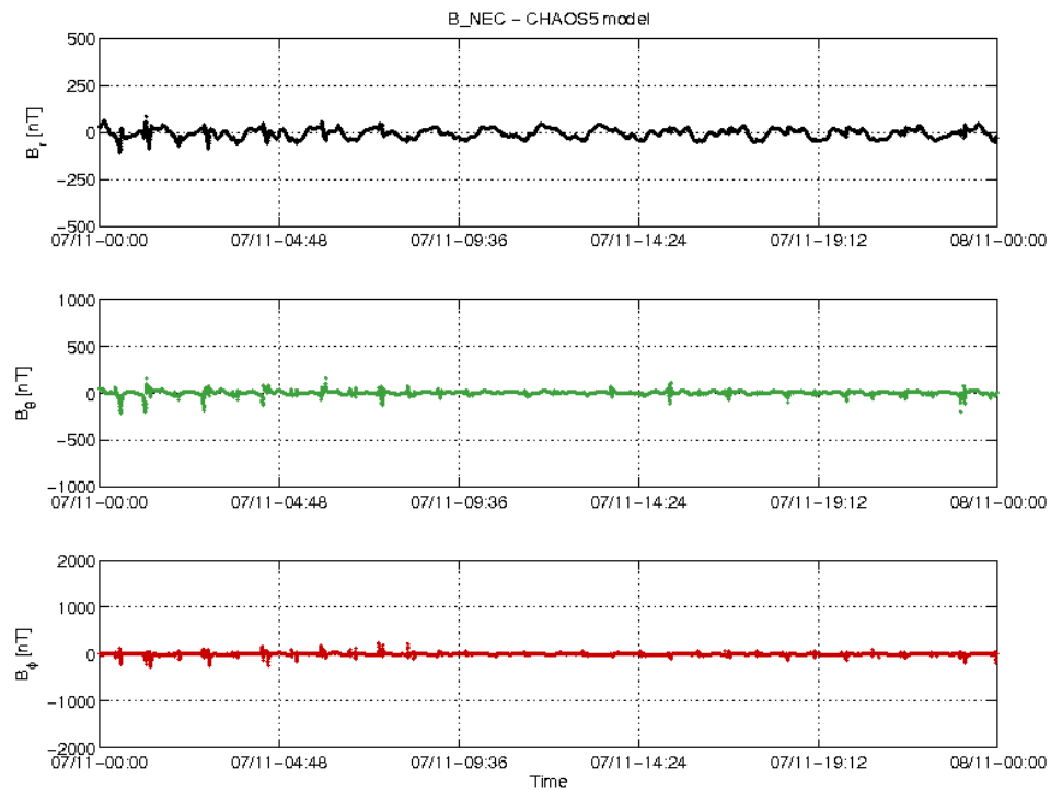
Figure 3-18: S/C A day 07/11: time series of B_{NEC} - B_{Chaos} residuals.
