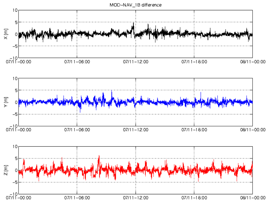
Figure 3-5: Difference MOD-GPSNAV, S/C C, 07/11. From top to bottom: X, Y and Z-axis
