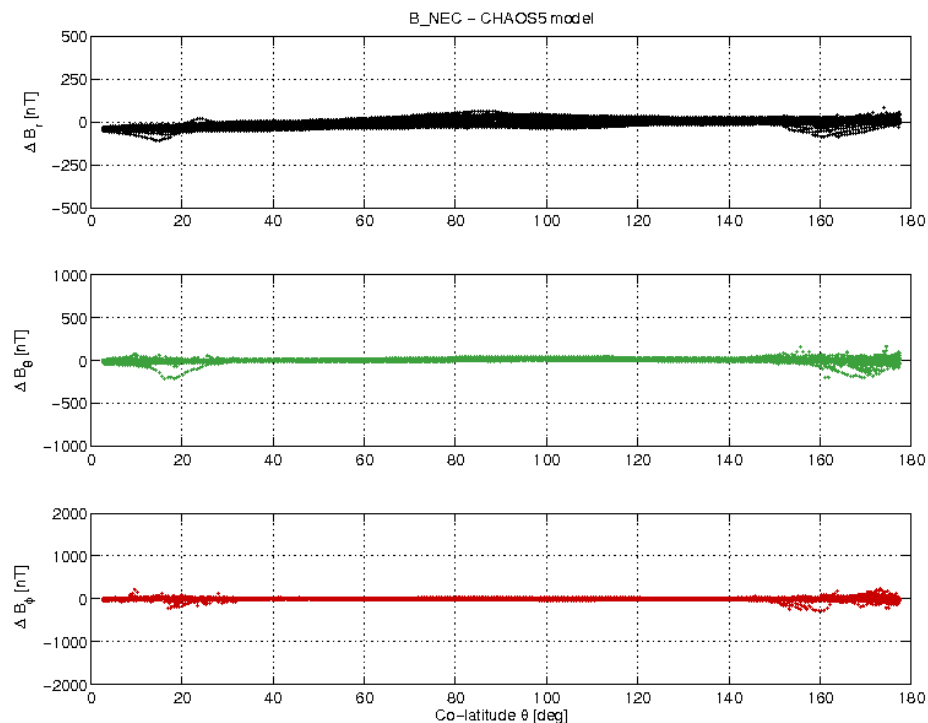
Figure 3-17: S/C A day 07/11 B_{NEC} - B_{Chaos} vs colatitude.
