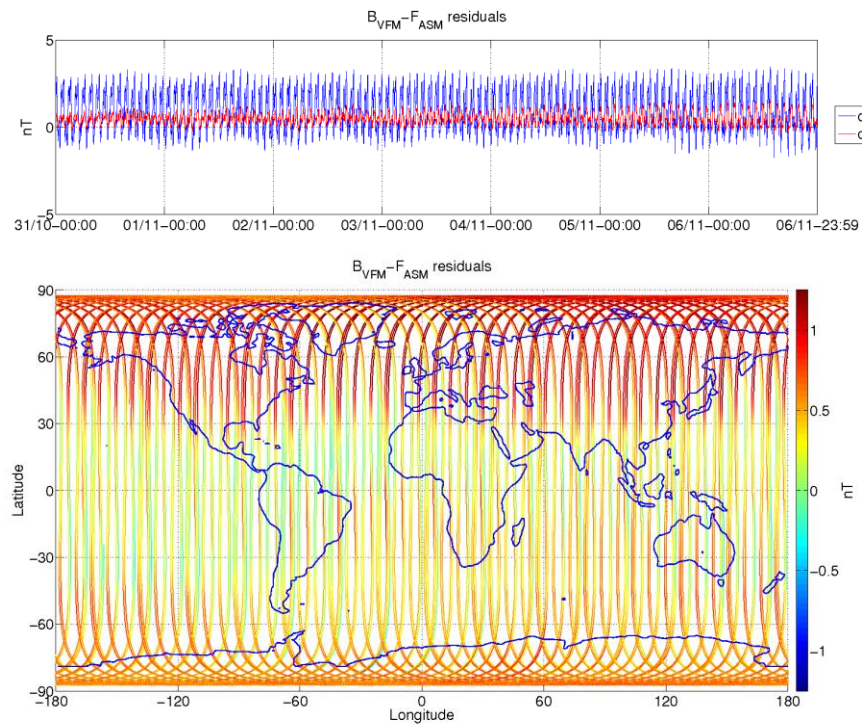
Figure 3-8: ASM-VFM residuals for S/C A, during monitoring period 31/10-06/11. In top figure are plotted: difference between |B_{VFM}| and F_{ASM} (without dB_Sun correction) (blue colour), and the residuals with dB_Sun corrections (red colour). In bottom figure residuals are presented on the world map.
