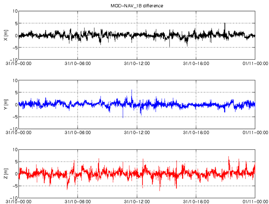
Figure 3-4: Difference MOD-GPSNAV, S/C B, 31/10. From top to bottom: X, Y and Z-axis
