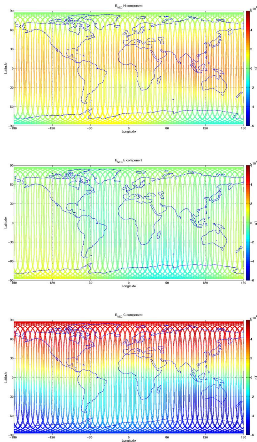
Figure 3-12: S/C C, world map plots of the geomagnetic field and components measured during monitoring period 31/10-06/11. From top to bottom: B_{NEC} components (North, East, and Centre) of magnetic field from VFM measurement.
