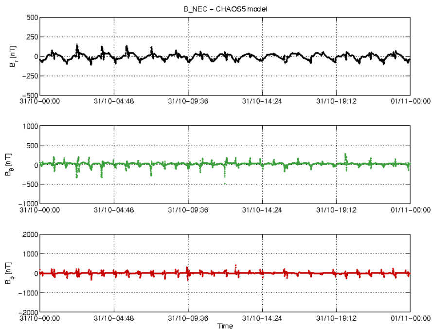
Figure 3-20: S/C B day 31/10 time series of B_{NEC} - B_{CHaos} residuals.
