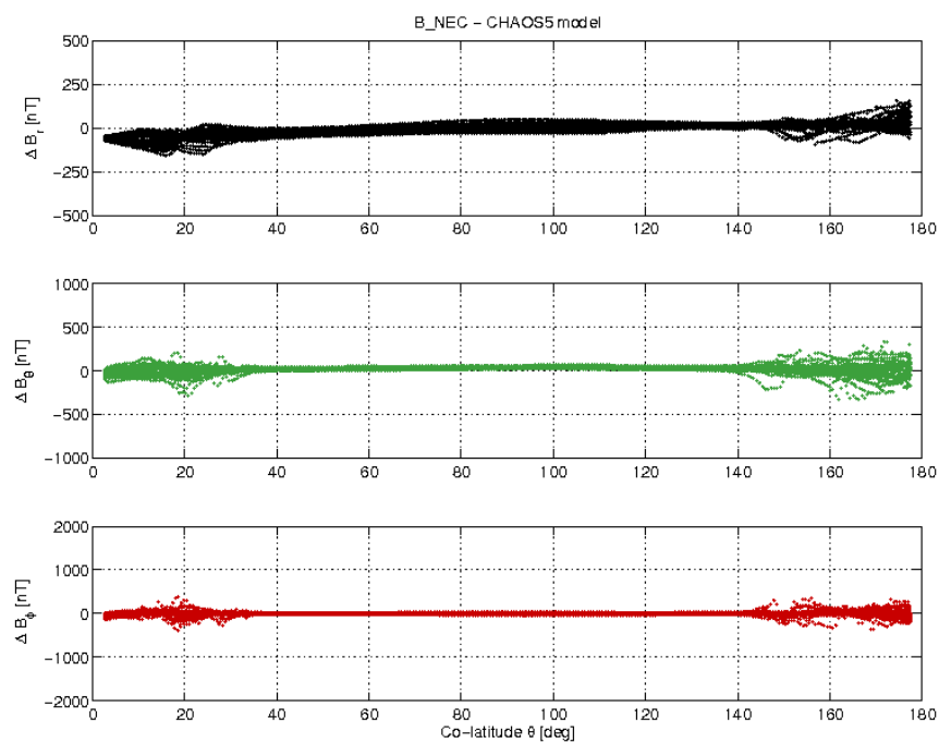
Figure 3-17: S/C A day 31/10 B_{NEC} - B_{Chaos} vs colatitude.
