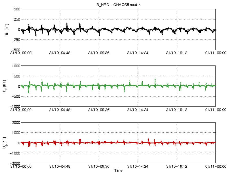
Figure 3-18: S/C A day 31/10: time series of B_{NEC} - B_{Chao5} residuals.
