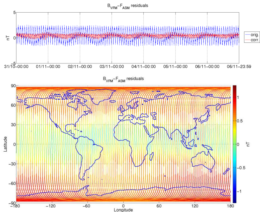
Figure 3-9: ASM-VFM residuals for S/C B, during monitoring period 31/10-06/11. In top figure are plotted: difference between |B_{VFM}| and F_{ASM} (without dB_{Sun} correction) (blue colour), and the residuals with dB_{Sun} corrections (red colour). In bottom figure residuals are presented on the world map.
