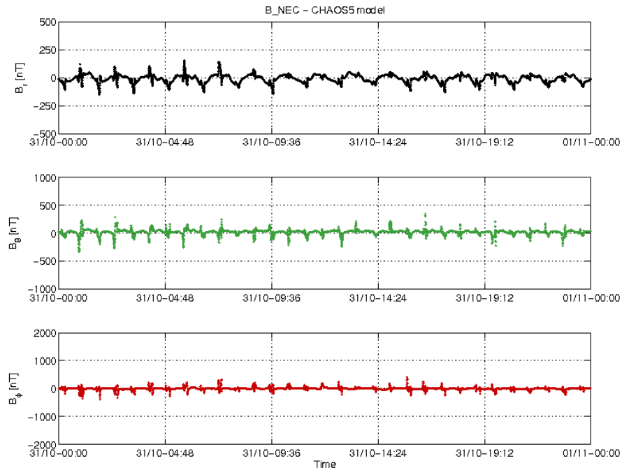
Figure 3-22: S/C C day 31/10 time series of B_{NEC} - B_{Chaos} residuals.
