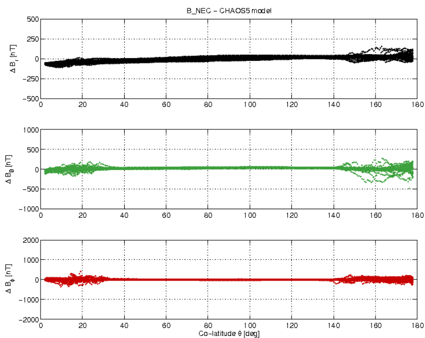
Figure 3-19: S/C B day 31/10 B_{NEC} - B_{Chao5} difference vs colatitude.
