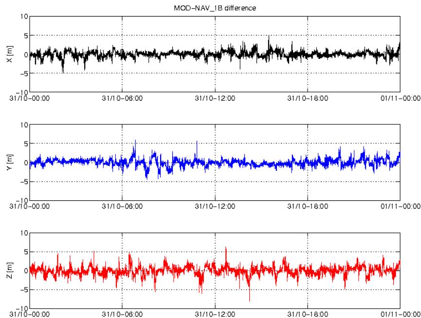
Figure 3-5: Difference MOD-GPSNAV, S/C C, 31/10. From top to bottom: X, Y and Z-axis
