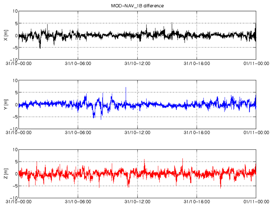
Figure 3-3: Difference MOD-GPSNAV, S/C A, 31/10. From top to bottom: X, Y and Z-axis
