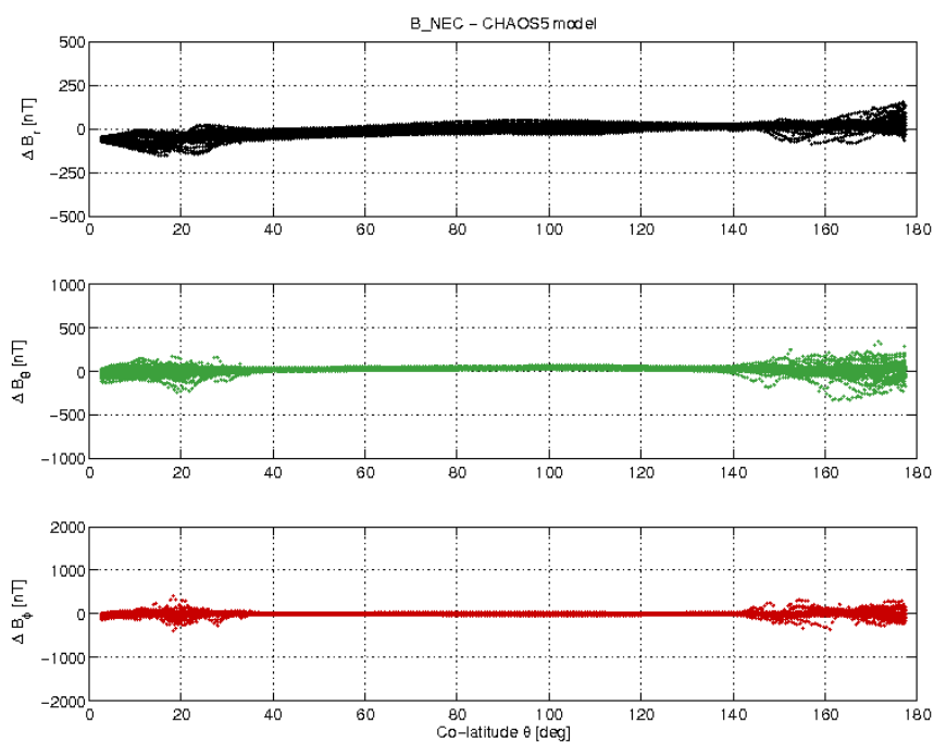
Figure 3-21: S/C C day 31/10 B_{NEC} - B_{CHaos} difference vs colatitude.
