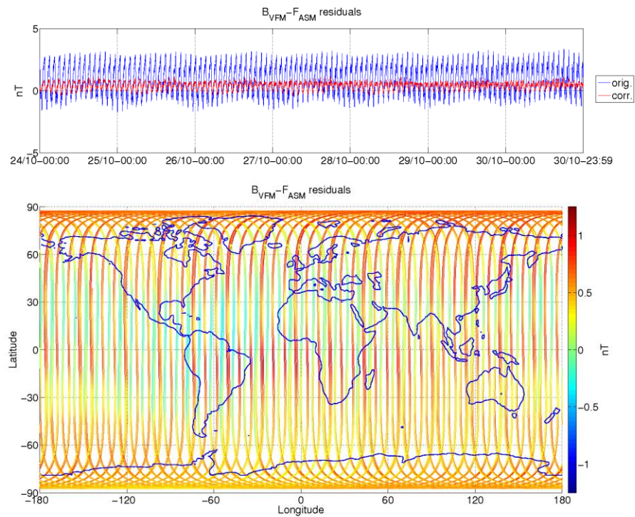
Figure 3-8: ASM-VFM residuals for S/C A, during monitoring period 24/10-30/10. In top figure are plotted: difference between |B_{VFM}| and F_{ASM} (without dB_Sun correction) (blue colour), and the residuals with dB_Sun corrections (red colour). In bottom figure residuals are presented on the world map.
