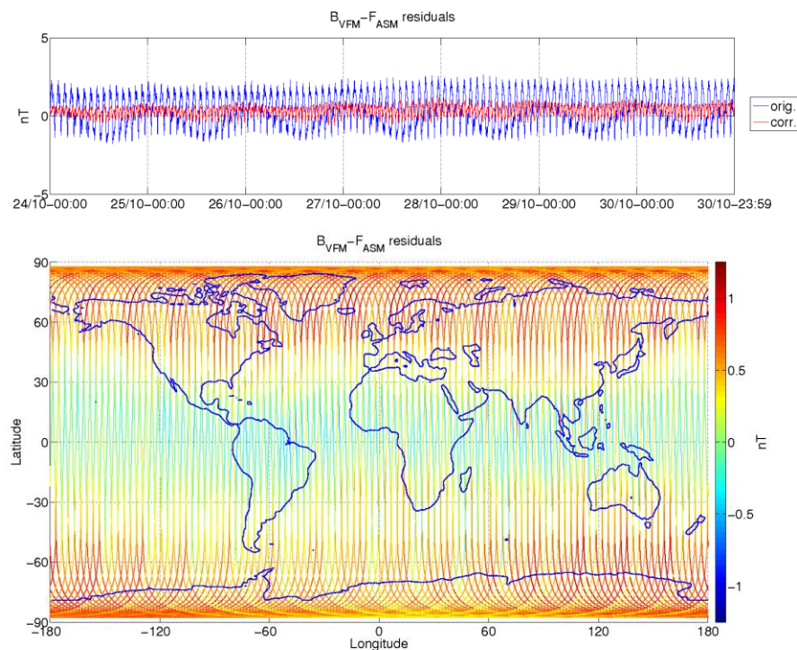
Figure 3-9: ASM-VFM residuals for S/C B, during monitoring period 24/10-30/10. In top figure are plotted: difference between |B_{VFM}| and F_{ASM} (without dB_{Sun} correction) (blue colour), and the residuals with dB_{Sun} corrections (red colour). In bottom figure residuals are presented on the world map.
