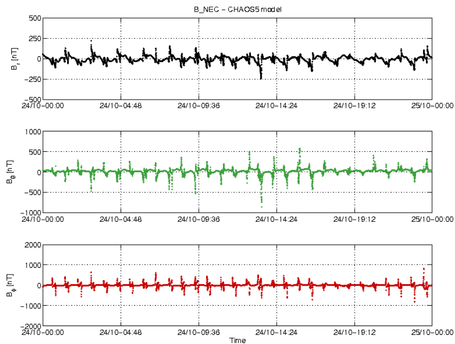
Figure 3-20: S/C B day 24/10 time series of B_{NEC} - B_{Chaos} residuals.
