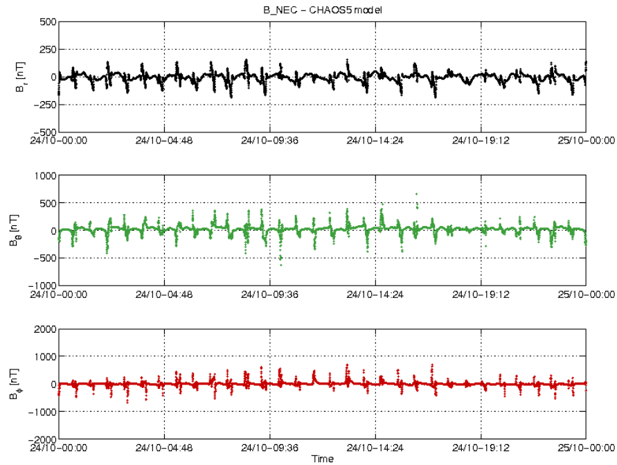
Figure 3-22: S/C C day 24/10 time series of B_{\text{NEC}} - B_{\text{Chaos}} residuals.
