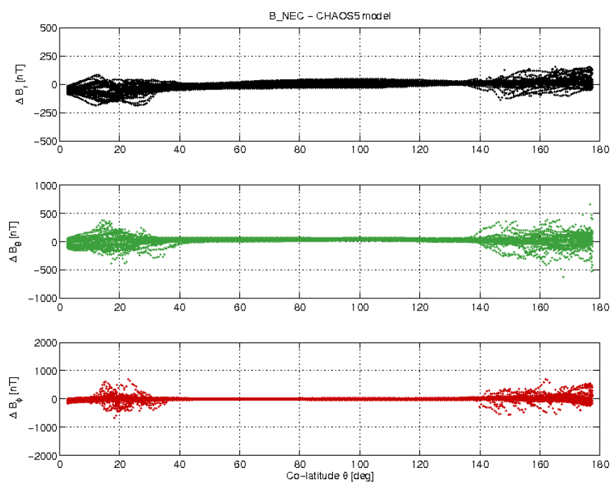
Figure 3-21: S/C C day 24/10 B_{NEC} - B_{Chaos} difference vs colatitude.
