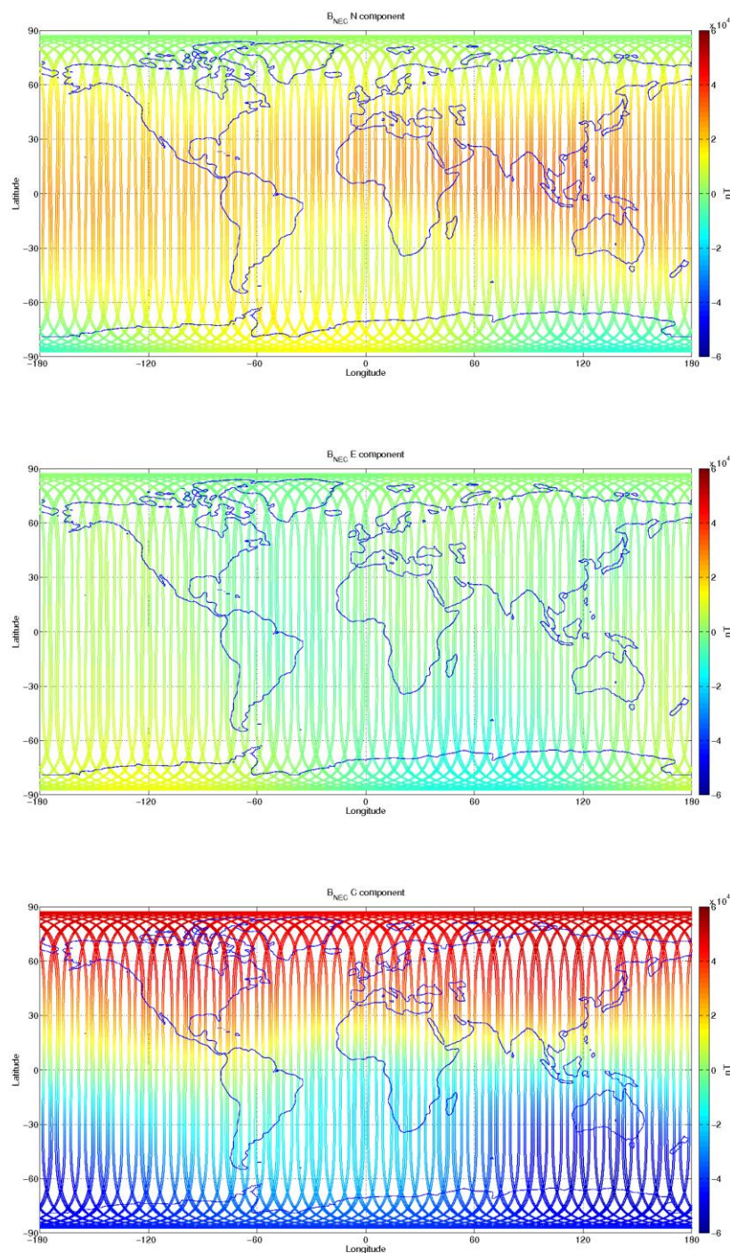
Figure 3-12: S/C C, world map plots of the geomagnetic field and components measured during monitoring period 24/10-30/10. From top to bottom: B_{NEC} components (North, East, and Centre) of magnetic field from VFM measurement.
