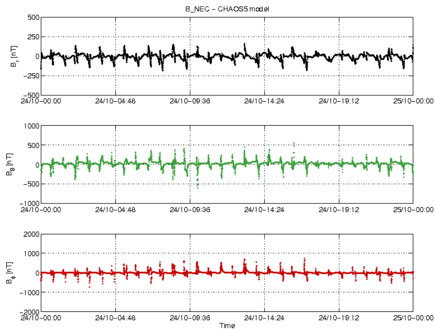
Figure 3-18: S/C A day 24/10: time series of B_{NEC} - B_{Chaos} residuals.
