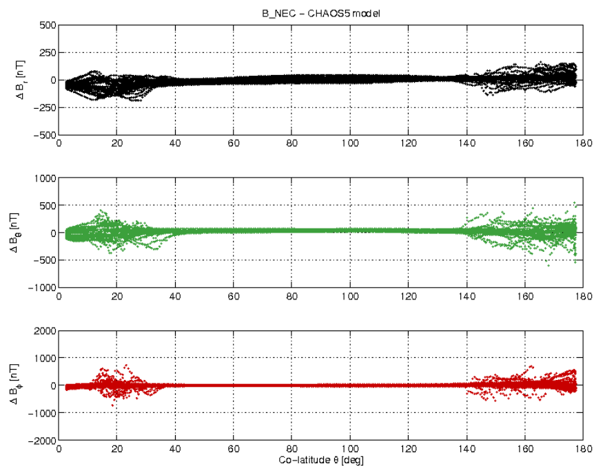
Figure 3-17: S/C A day 24/10 B_{NEC} - B_{Chaos} vs colatitude.
