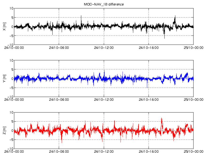
Figure 3-4: Difference MOD-GPSNAV, S/C B, 24/10. From top to bottom: X, Y and Z-axis
