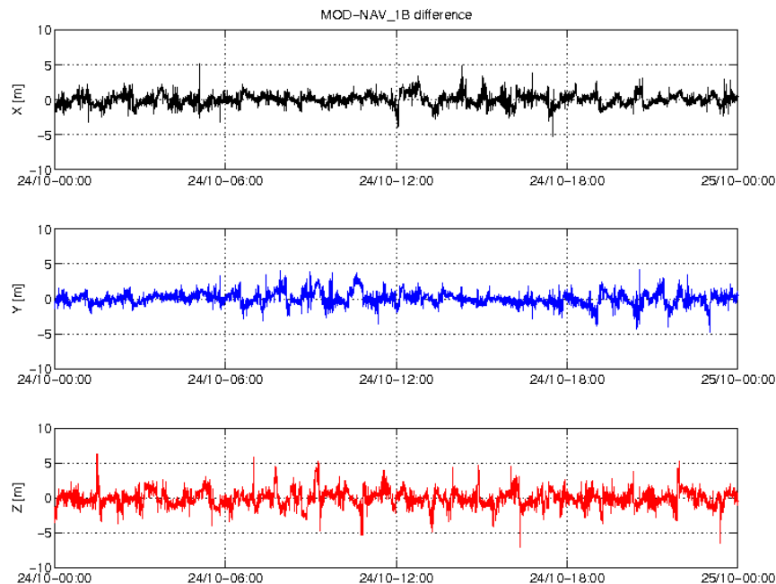
Figure 3-5: Difference MOD-GPSNAV, S/C C, 24/10. From top to bottom: X, Y and Z-axis
