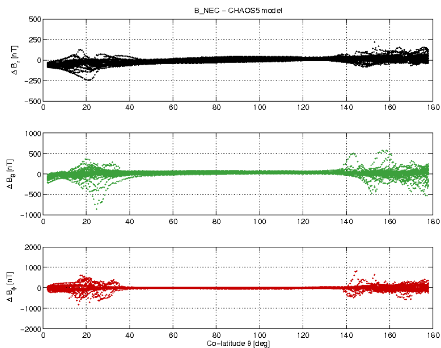
Figure 3-19: S/C B day 24/10 B_{NEC} - B_{Chaos} difference vs colatitude.
