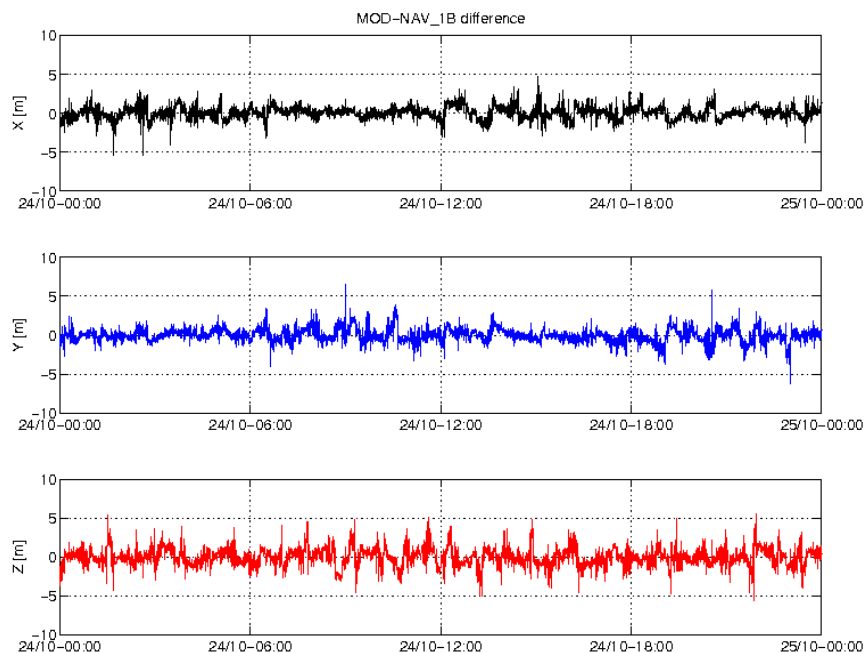
Figure 3-3: Difference MOD-GPSNAV, S/C A, 24/10. From top to bottom: X, Y and Z-axis
