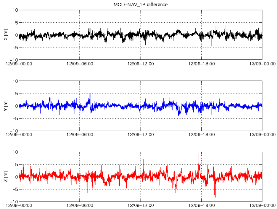
Figure 4: Difference MOD-GPSNAV, S/C B, 12/09. From top to bottom: X, Y and Z-axis
