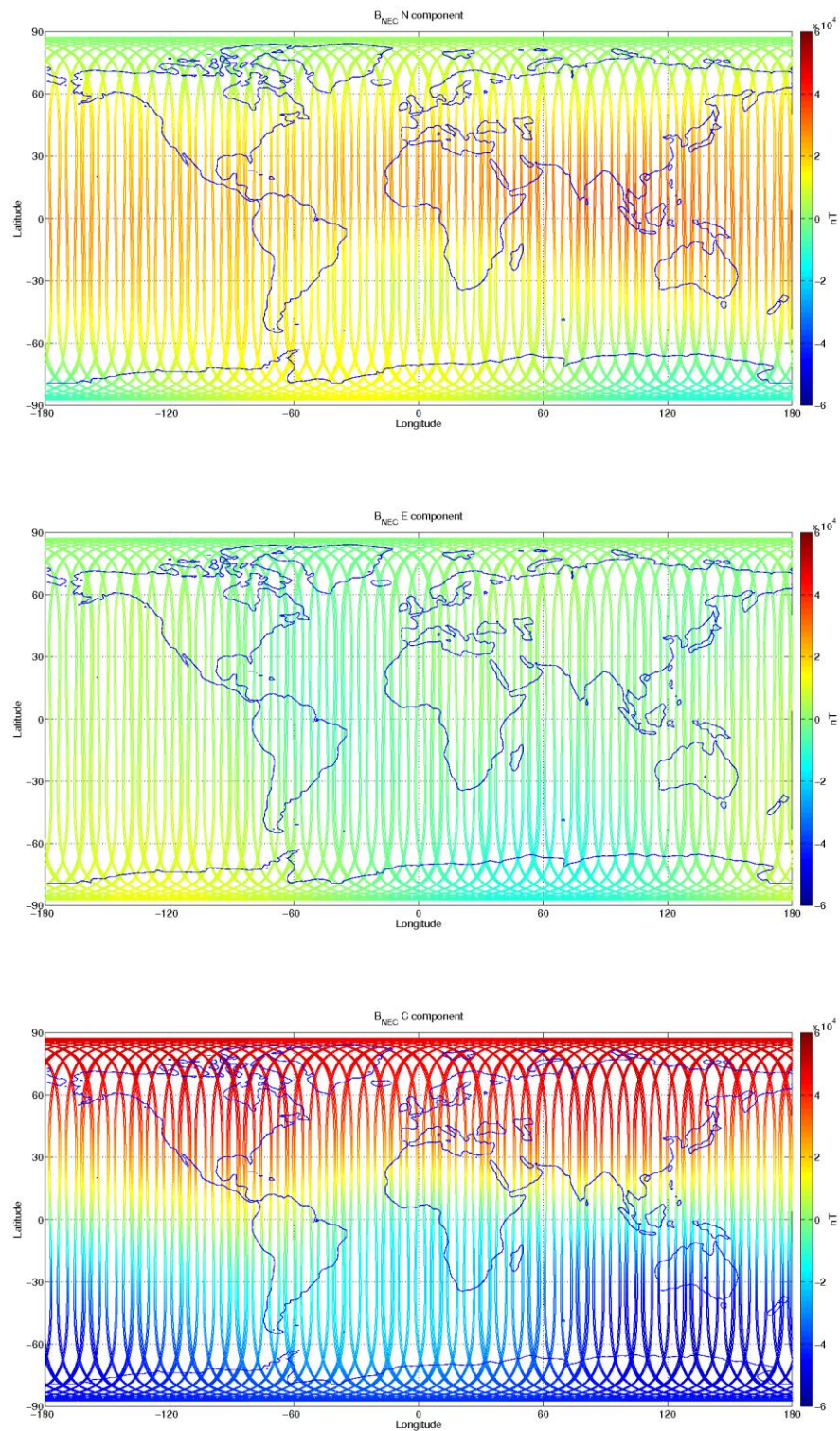
Figure 12: S/C C, world map plots of the geomagnetic field and components measured during monitoring period 12/09-18/09. From top to bottom: B NEC components (North, East, and Centre) of magnetic field from VFM measurement.
