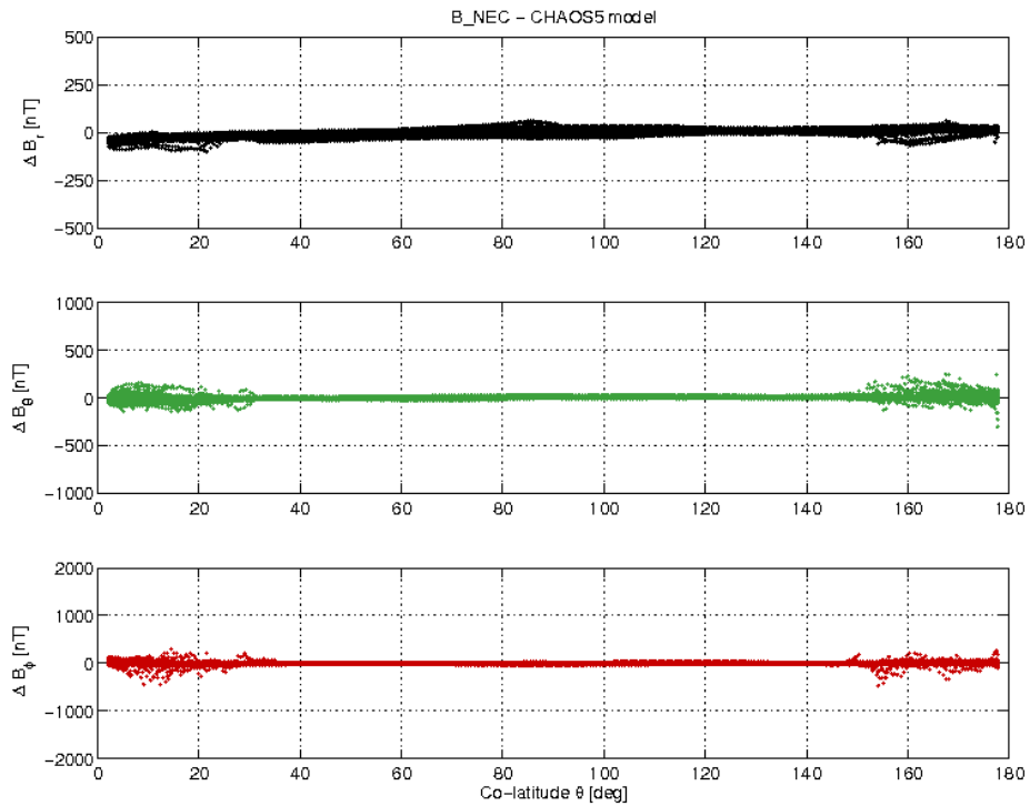
Figure 19: S/C B day 12/09 B_{NEC} - B_{Chaos} difference vs colatitude.
