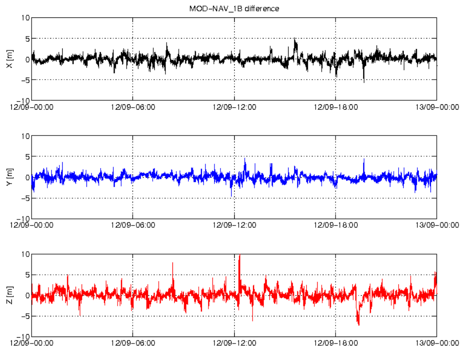
Figure 5: Difference MOD-GPSNAV, S/C C, 12/09. From top to bottom: X, Y and Z-axis
