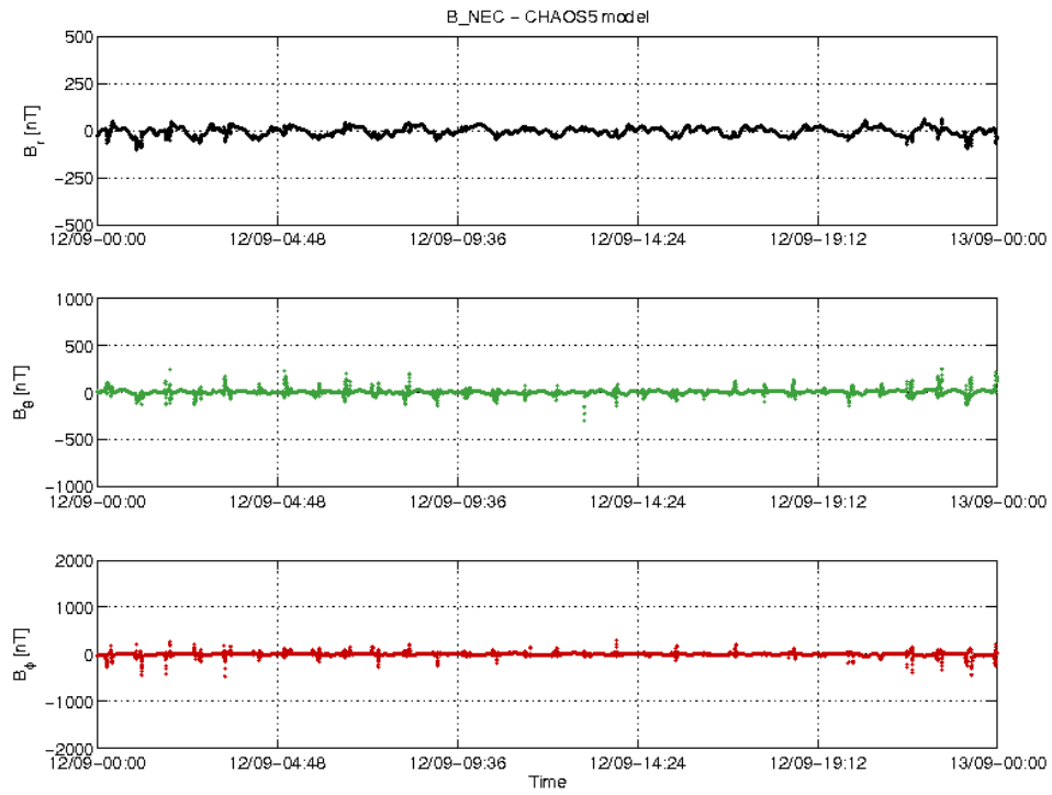
Figure 20: S/C B day 12/09 time series of B_{NEC} - B_{Chaos} residuals.
