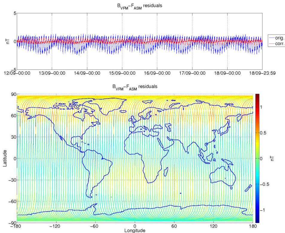
Figure 9: ASM-VFM residuals for S/C B, during monitoring period 12/09-18/09. In top figure are plotted: difference between |B_{VFM}| and F_{ASM} (without dB_{Sun} correction) (blue colour), and the residuals with dB_{Sun} corrections (red colour). In bottom figure residuals are presented on the world map.
