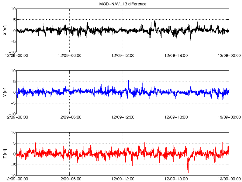
Figure 3: Difference MOD-GPSNAV, S/C A, 12/09. From top to bottom: X, Y and Z-axis
