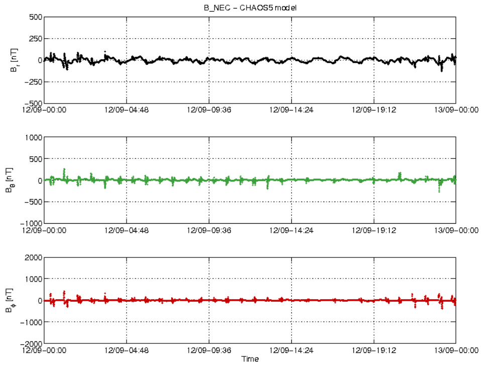
Figure 18: S/C A day 12/09: time series of B_{NEC} - B_{Chaos} residuals.
