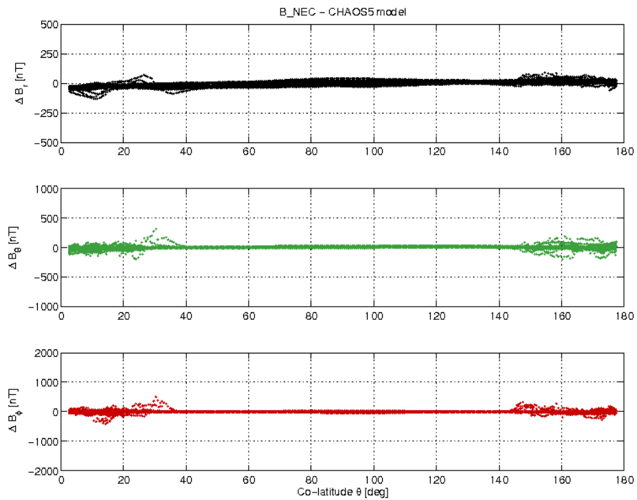
Figure 21: S/C C day 12/09 B_{NEC} - B_{Chaos} difference vs colatitude.
