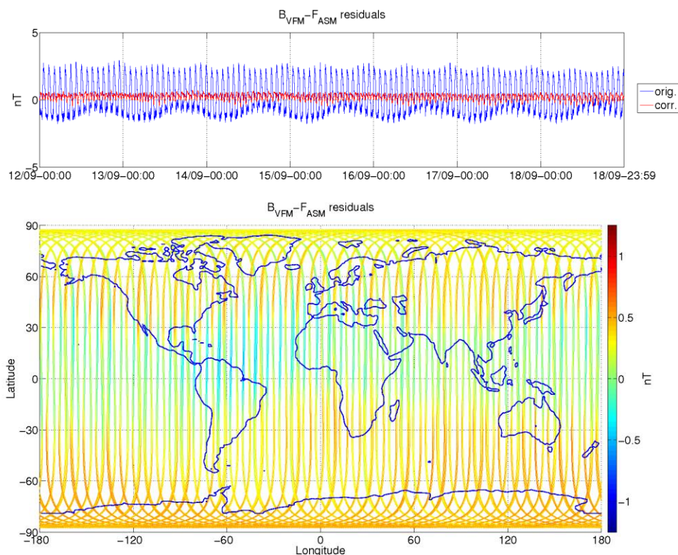
Figure 8: ASM-VFM residuals for S/C A, during monitoring period 12/09-18/09. In top figure are plotted: difference between |B_{VFM}| and F_{ASM} (without dB_{Sun} correction) (blue colour), and the residuals with dB_{Sun} corrections (red colour). In bottom figure residuals are presented on the world map.
