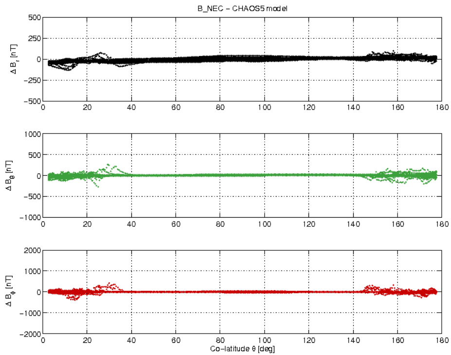
Figure 17: S/C A day 12/09 B_{NEC} - B_{Chaos} vs colatitude.
