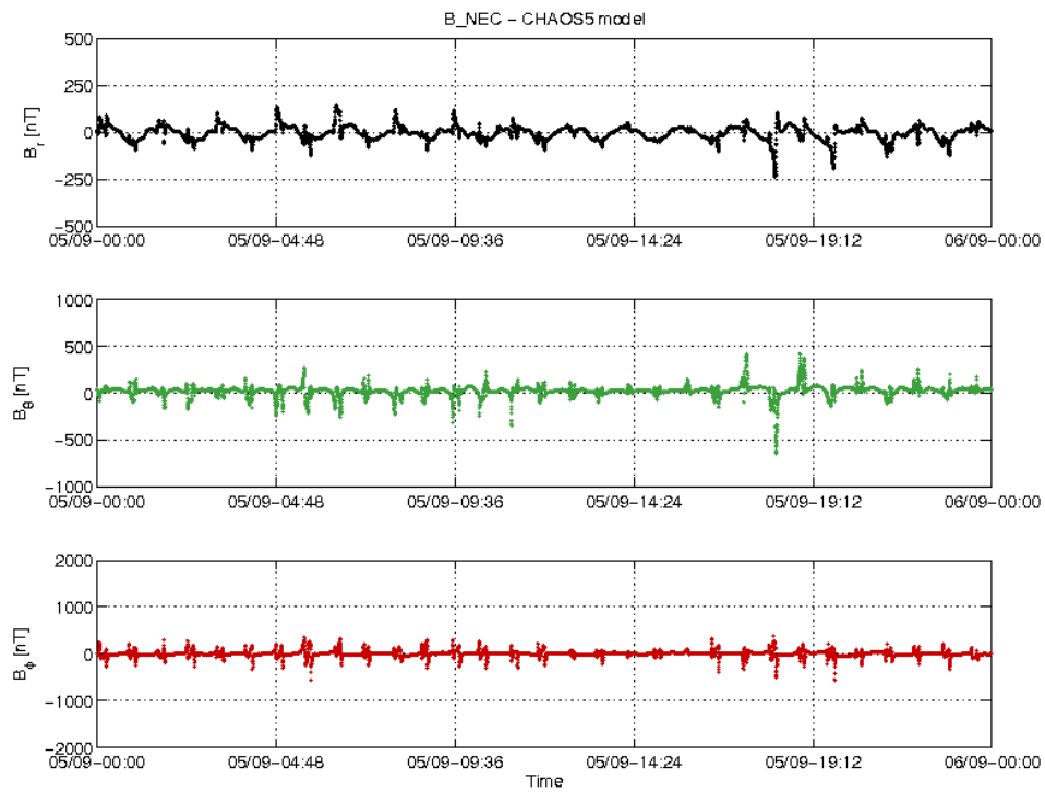
Figure 22: S/C C day 05/09 time series of B_{NEC} - B_{Chaos} residuals.
