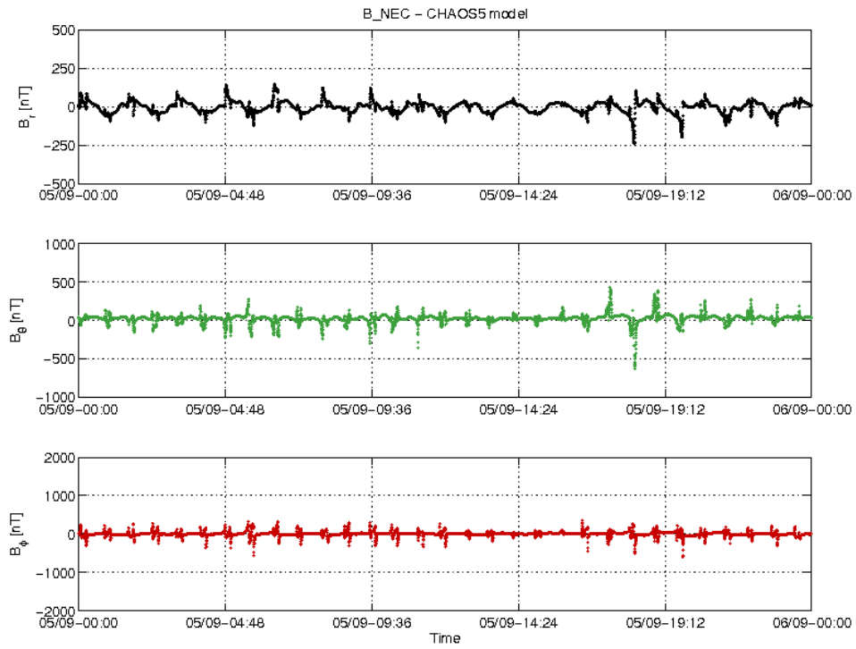
Figure 18: S/C A day 05/09: time series of B_{NEC} - B_{Chaos} residuals.
