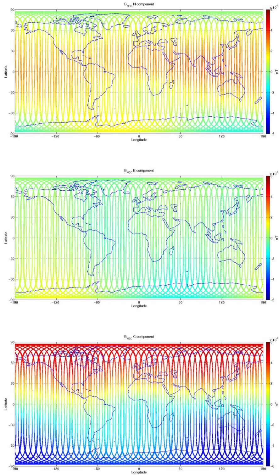
Figure 12: S/C C, world map plots of the geomagnetic field and components measured during monitoring period 05/09-11/09. From top to bottom: B_{NEC} components (North, East, and Centre) of magnetic field from VFM measurement.
