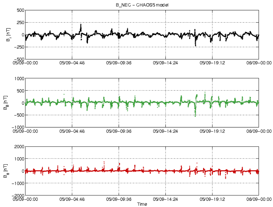
Figure 20: S/C B day 05/09 time series of B_{NEC} - B_{Chaos} residuals.
