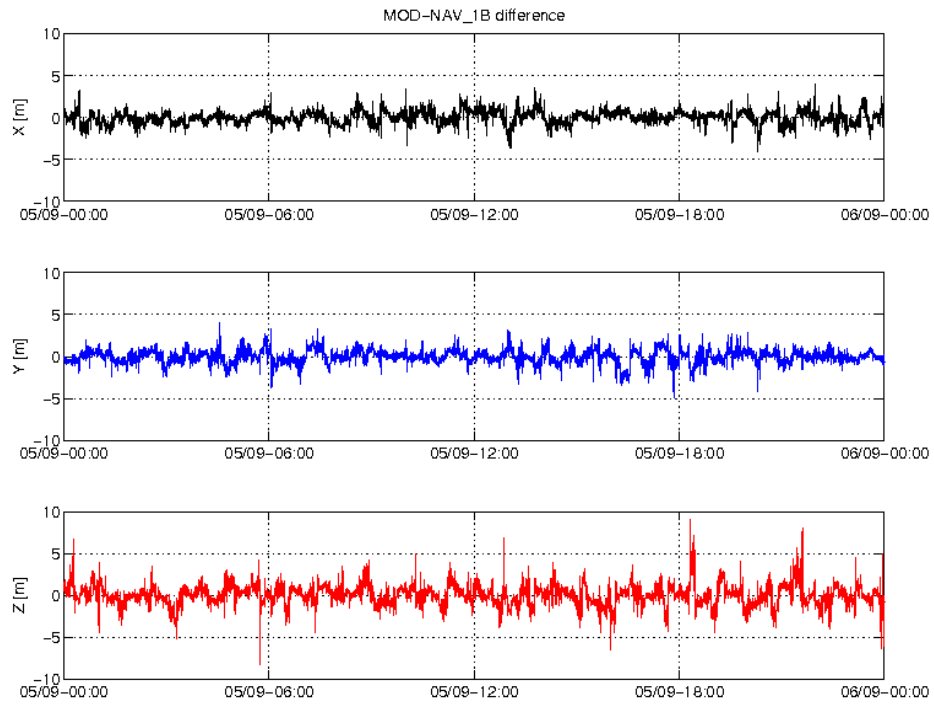
Figure 4: Difference MOD-GPSNAV, S/C B, 05/09. From top to bottom: X, Y and Z-axis
