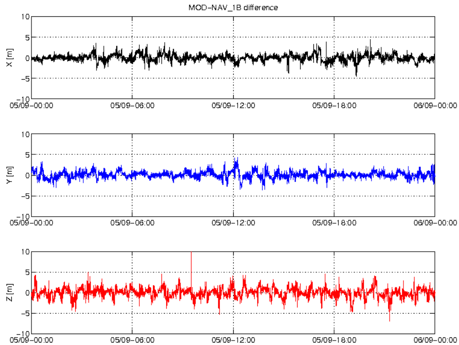
Figure 5: Difference MOD-GPSNAV, S/C C, 05/09. From top to bottom: X, Y and Z-axis
