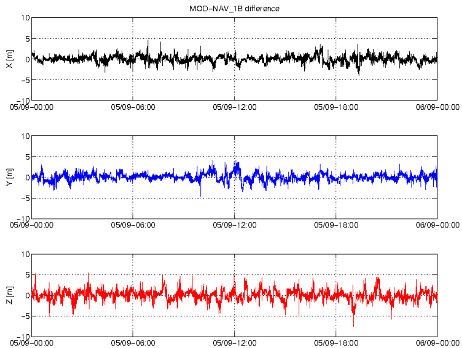
Figure 3: Difference MOD-GPSNAV, S/C A, 05/09. From top to bottom: X, Y and Z-axis
