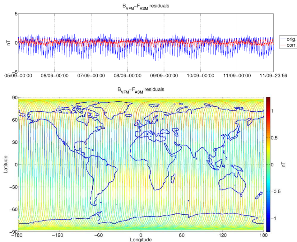
Figure 9: ASM-VFM residuals for S/C B, during monitoring period 05/09-11/09. In top figure are plotted: difference between |B_{VFM}| and F_{ASM} (without dB_{Sun} correction) (blue colour), and the residuals with dB_{Sun} corrections (red colour). In bottom figure residuals are presented on the world map.
