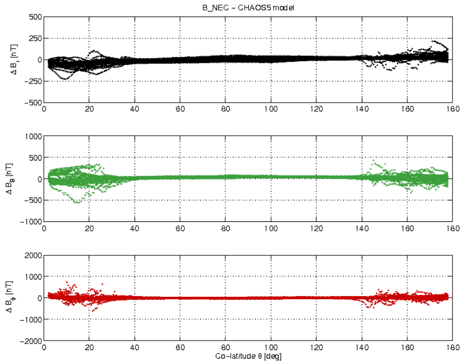
Figure 19: S/C B day 05/09 B_{NEC} - B_{Chaos} difference vs colatitude.
