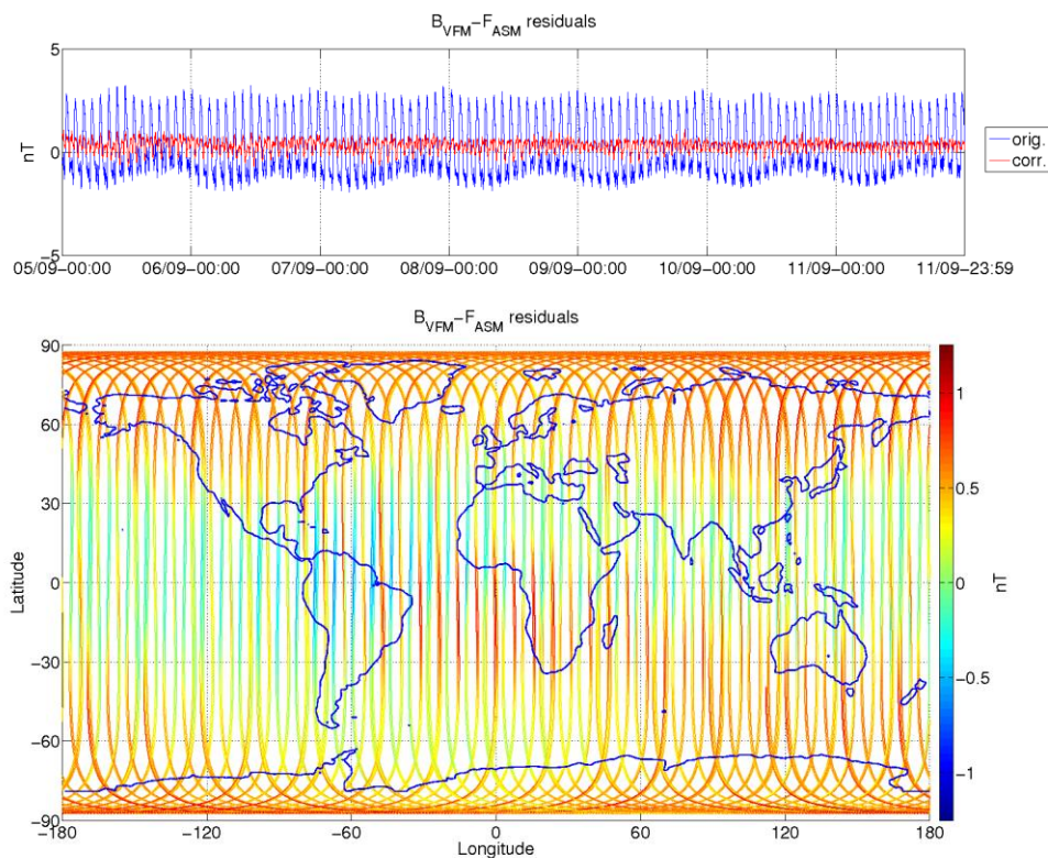
Figure 8: ASM-VFM residuals for S/C A, during monitoring period 05/09-11/09. In top figure are plotted: difference between |B_{VFM}| and F_{ASM} (without dB_{Sun} correction) (blue colour), and the residuals with dB_{Sun} corrections (red colour). In bottom figure residuals are presented on the world map.
