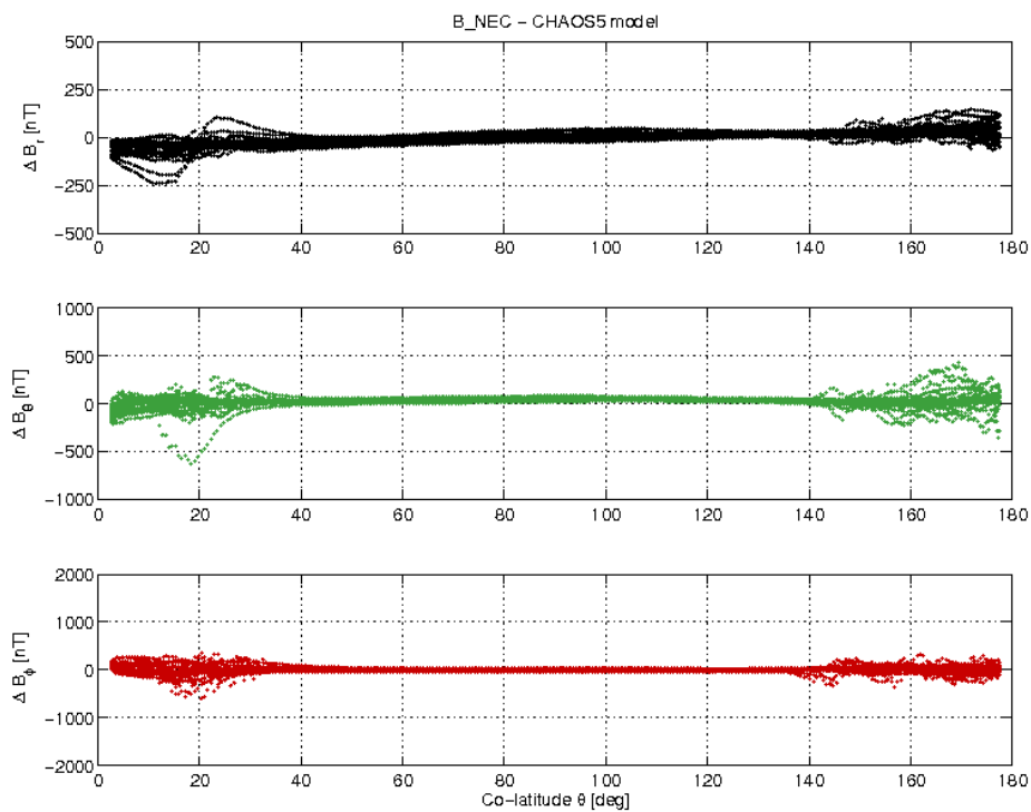
Figure 17: S/C A day 05/09 B_{NEC} - B_{Chaos} vs colatitude.
