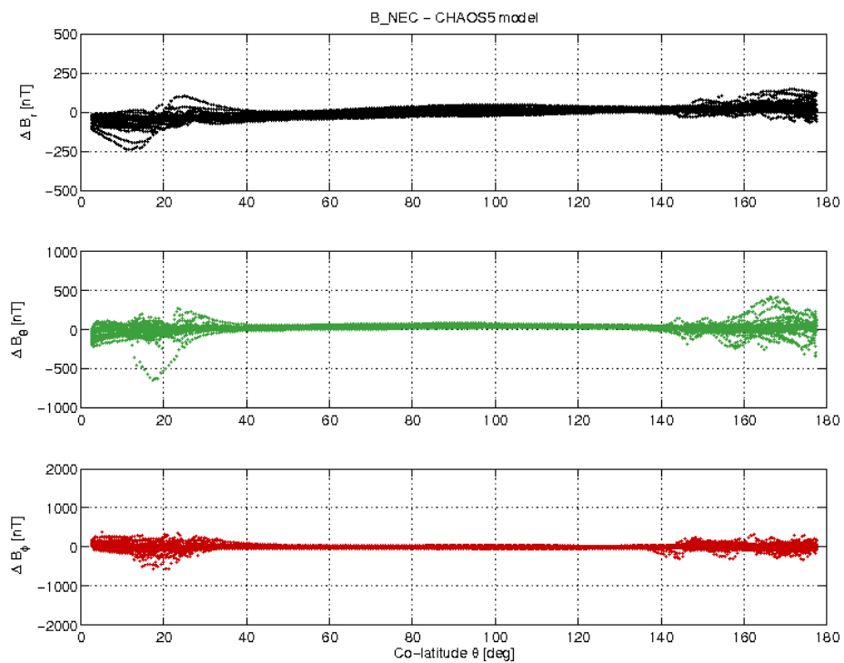
Figure 21: S/C C day 05/09 B_{NEC} - B_{Chaos} difference vs colatitude.
