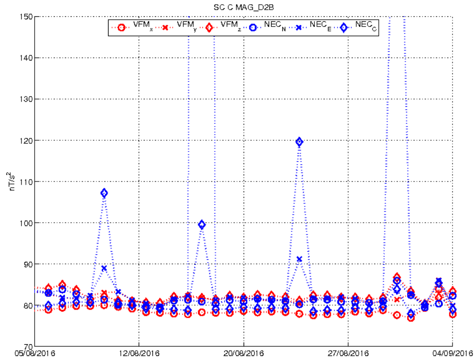
Figure 25: Plot of standard deviation of the second derivative of B components in VFM and NEC frames.
