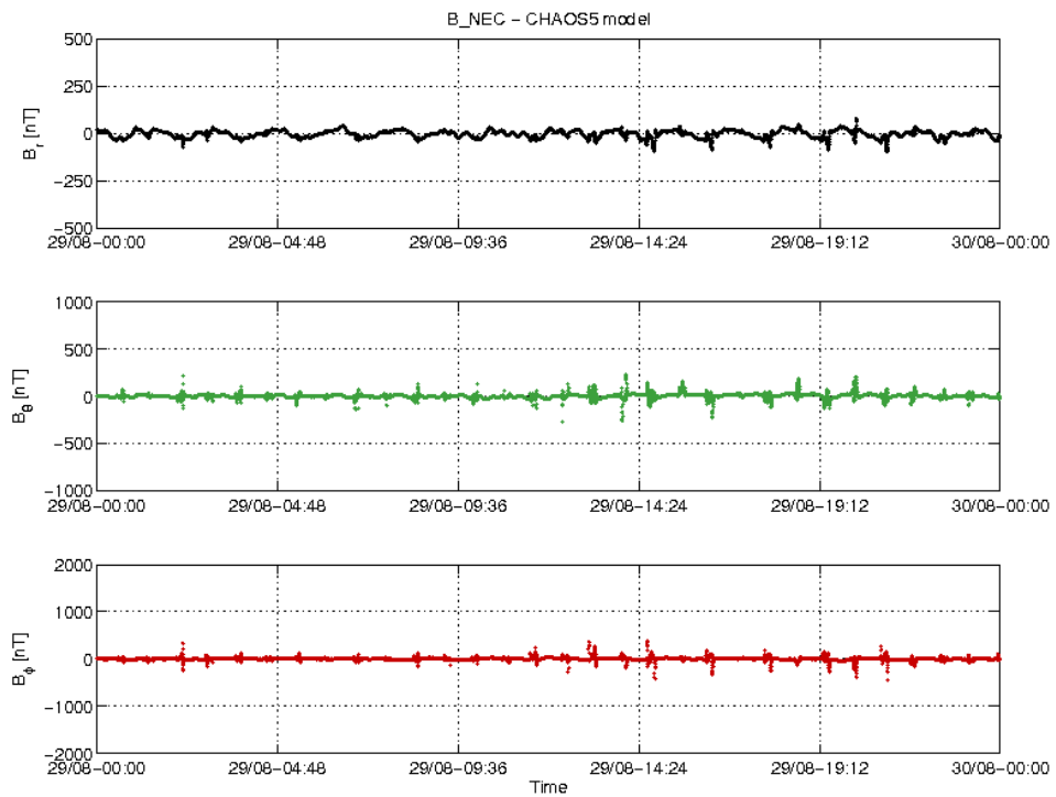
Figure 22: S/C C day 29/08 time series of B_{NEC} - B_{Chaos} residuals.
