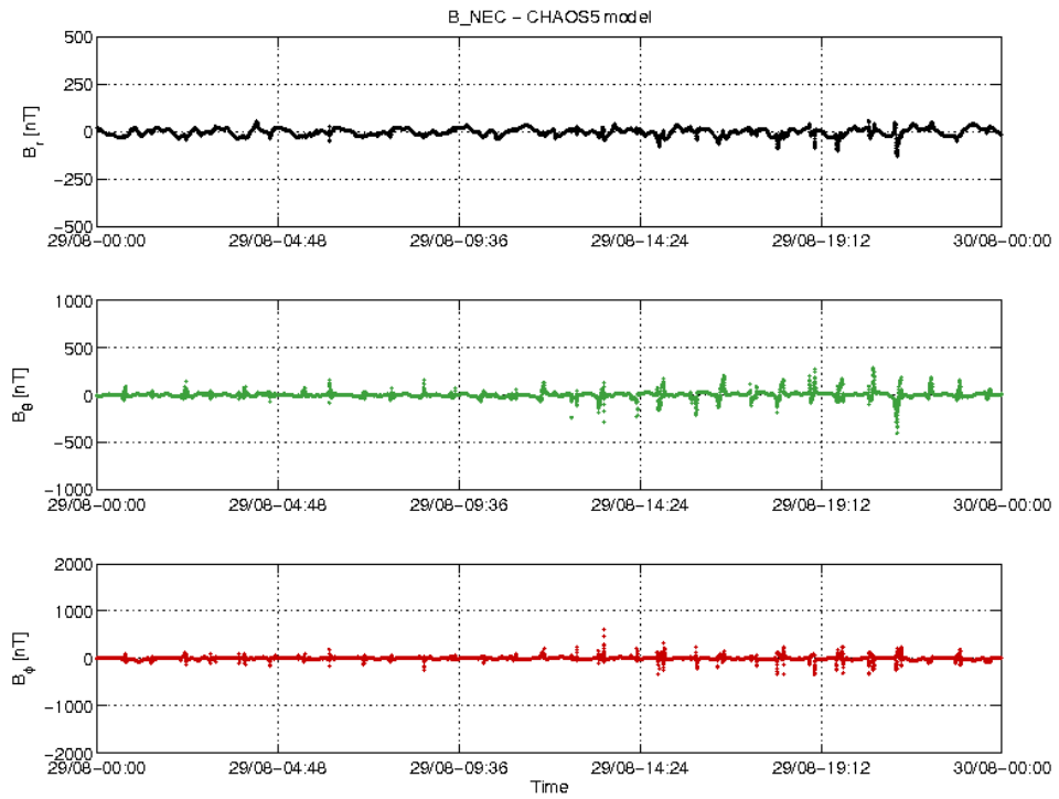
Figure 20: S/C B day 29/08 time series of B_{NEC} - B_{Chaos} residuals.
