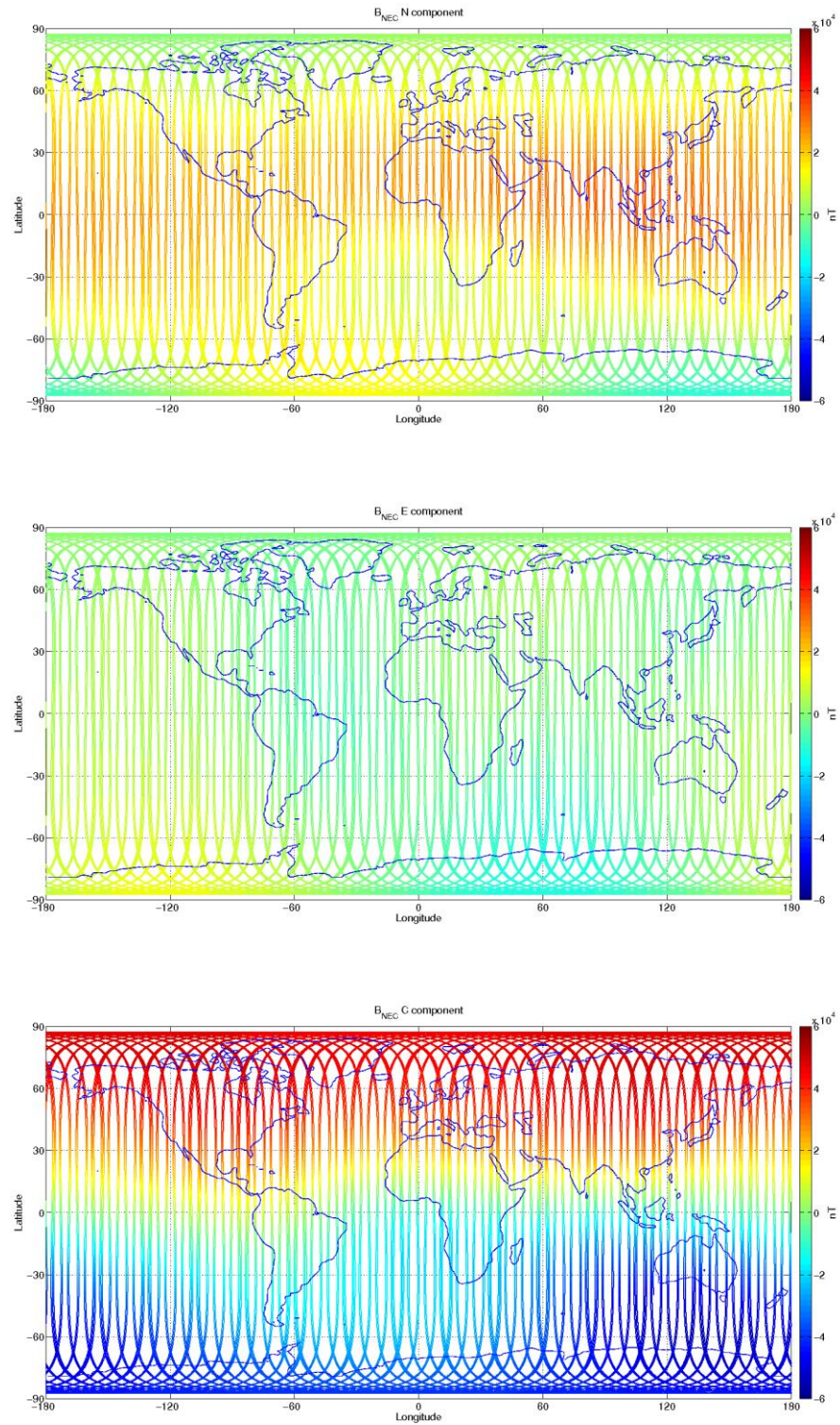
Figure 12: S/C C, world map plots of the geomagnetic field and components measured during monitoring period 29/08-04/09. From top to bottom: B NEC components (North, East, and Centre) of magnetic field from VFM measurement.
