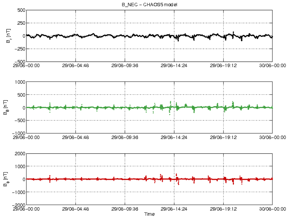
Figure 18: S/C A day 29/08: time series of B_{NEC} - B_{Chaos} residuals.
