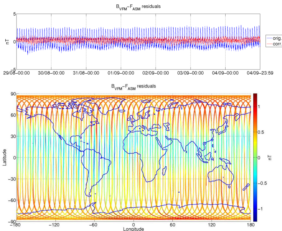
Figure 8: ASM-VFM residuals for S/C A, during monitoring period 29/08-04/09. In top figure are plotted: difference between |B_{VFM}| and F_{ASM} (without dB_Sun correction) (blue colour), and the residuals with dB_Sun corrections (red colour). In bottom figure residuals are presented on the world map.
