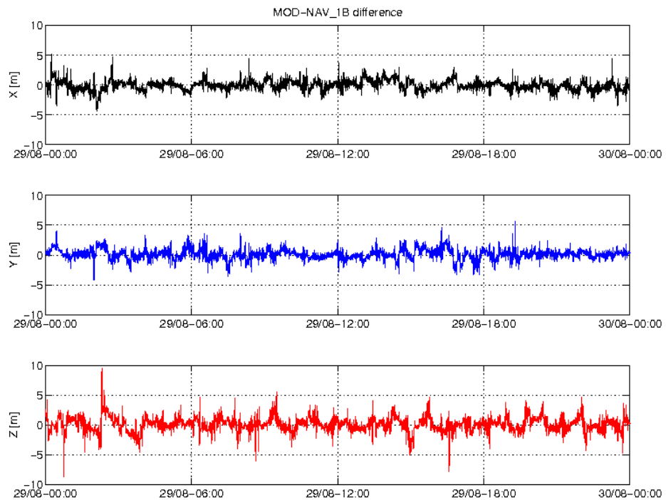
Figure 4: Difference MOD-GPSNAV, S/C B, 29/08. From top to bottom: X, Y and Z-axis
