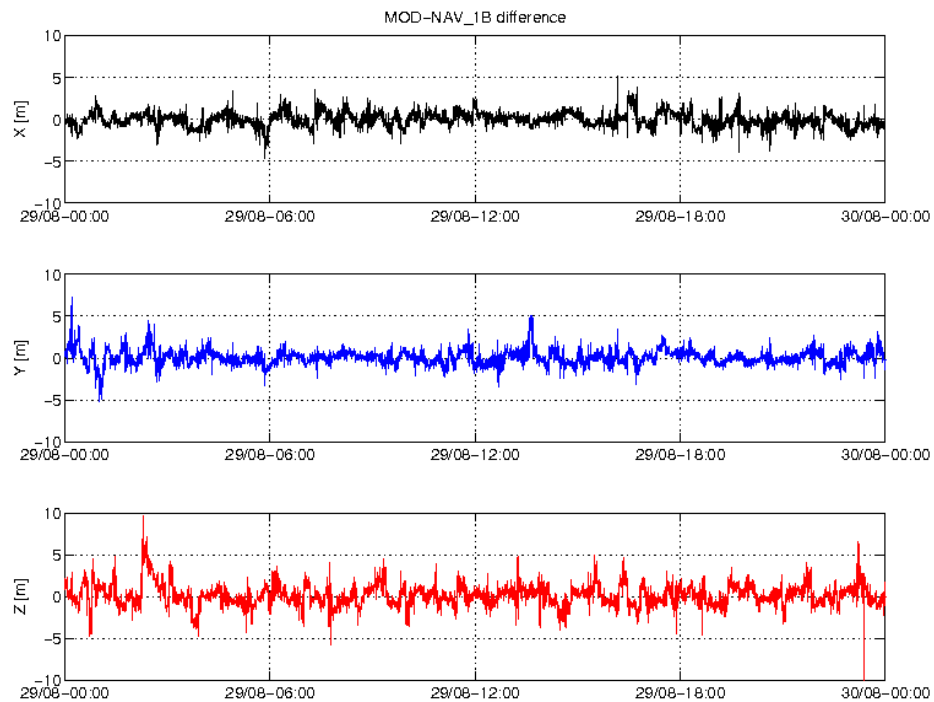
Figure 5: Difference MOD-GPSNAV, S/C C, 29/08. From top to bottom: X, Y and Z-axis
