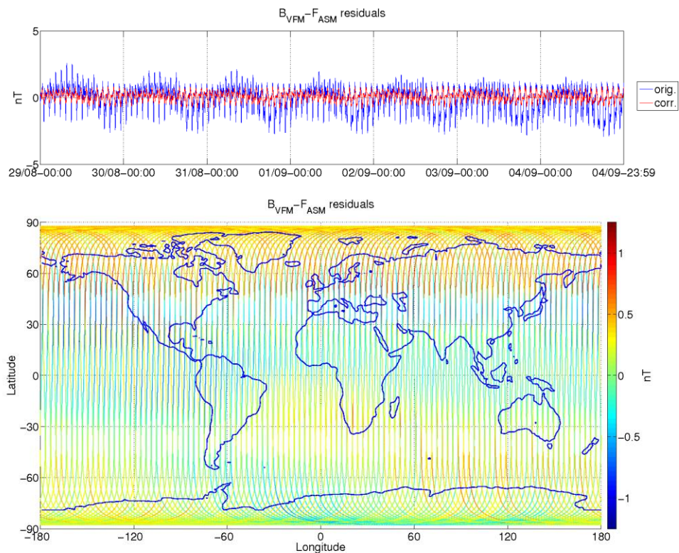
Figure 9: ASM-VFM residuals for S/C B, during monitoring period 29/08-04/09. In top figure are plotted: difference between |B_{VFM}| and F_{ASM} (without dB Sun correction) (blue colour), and the residuals with dB Sun corrections (red colour). In bottom figure residuals are presented on the world map.
