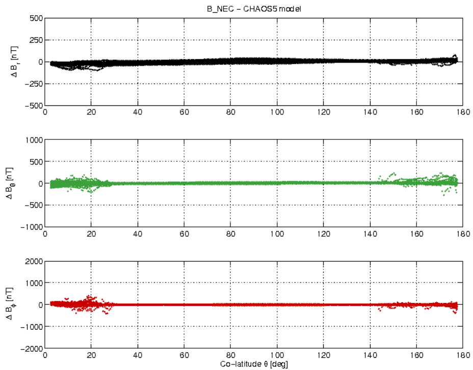
Figure 17: S/C A day 29/08 B_{NEC} - B_{Chaos} vs colatitude.
