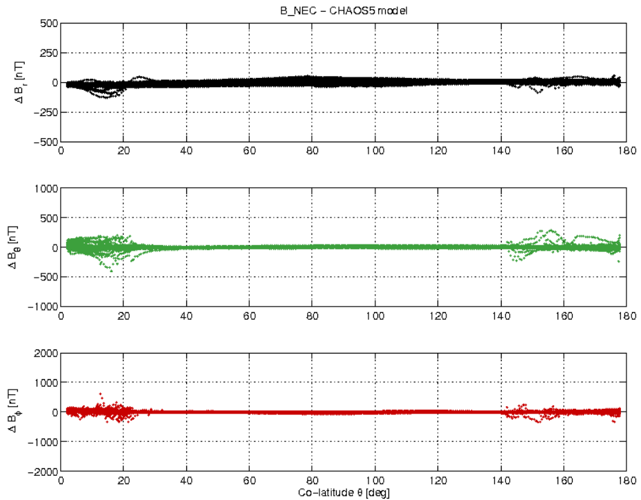
Figure 19: S/C B day 29/08 B_{NEC} - B_{Chaos} difference vs colatitude.
