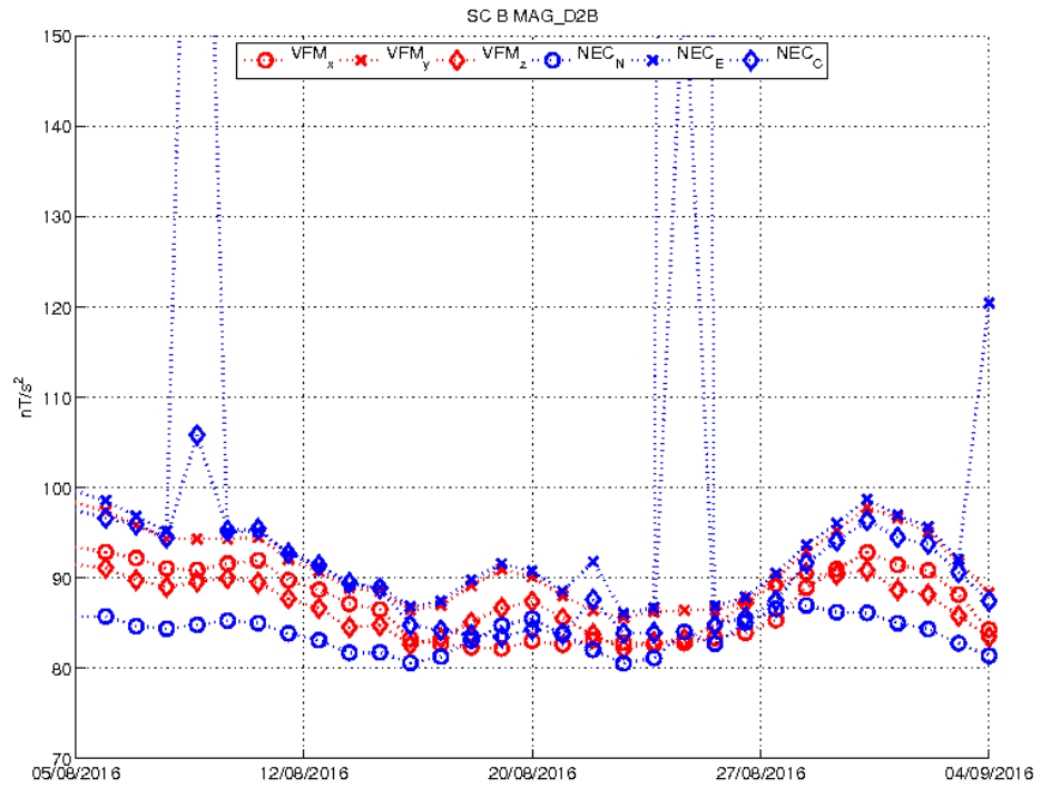
Figure 24: Plot of standard deviation of the second derivative of B components in VFM and NEC frames.
