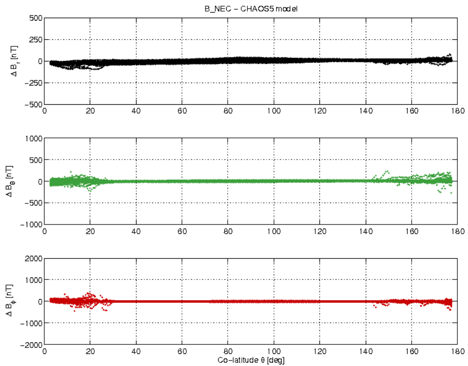
Figure 21: S/C C day 29/08 B_{NEC} - B_{Chaos} difference vs colatitude.
