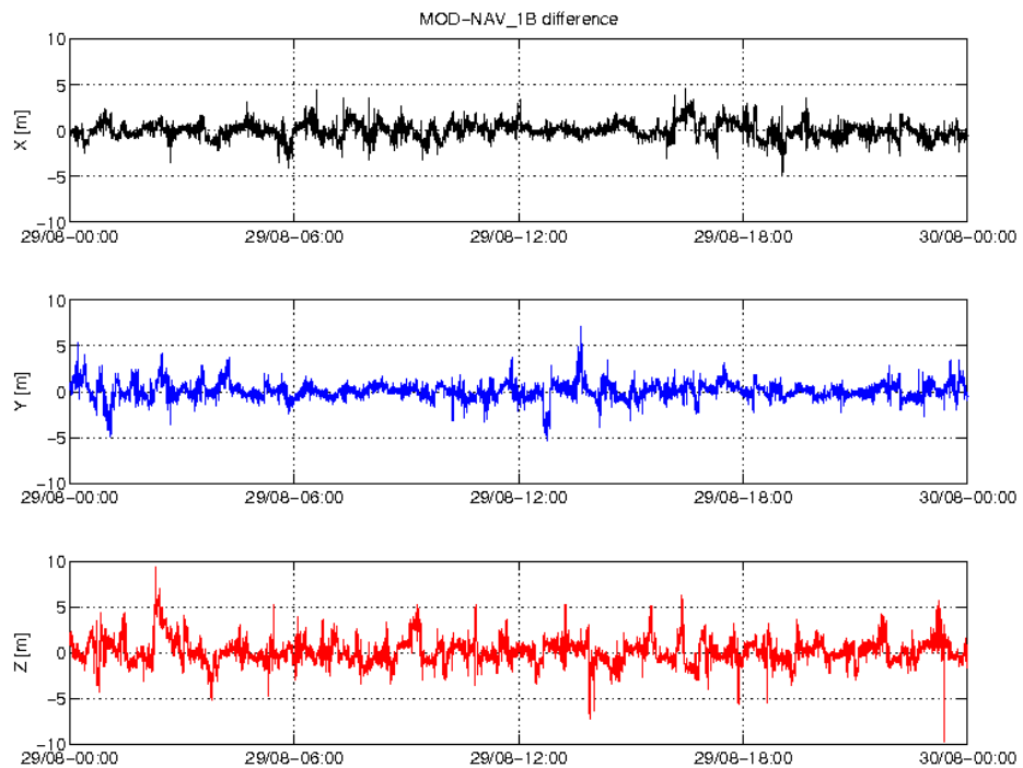
Figure 3: Difference MOD-GPSNAV, S/C A, 29/08. From top to bottom: X, Y and Z-axis
