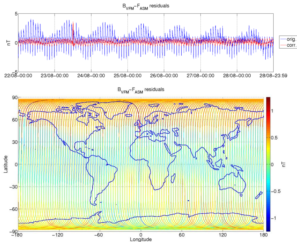
Figure 9: ASM-VFM residuals for S/C B, during monitoring period 22/08-28/08. In top figure are plotted: difference between |B_{VFM}| and F_{ASM} (without dB_Sun correction) (blue colour), and the residuals with dB_Sun corrections (red colour). In bottom figure residuals are presented on the world map.
