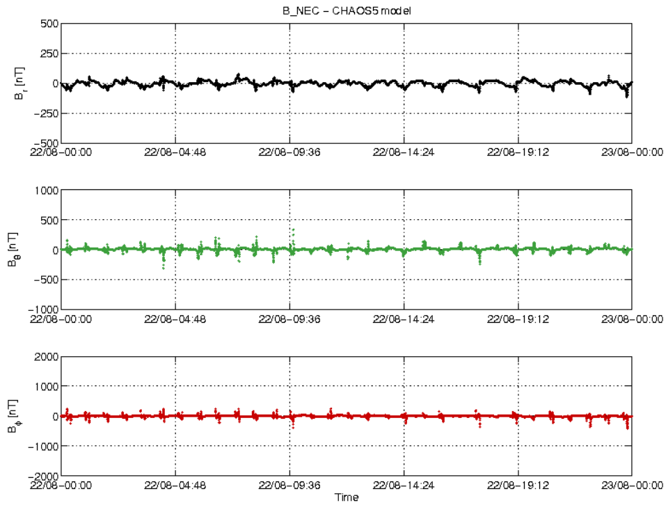
Figure 22: S/C C day 22/08 time series of B_{NEC} - B_{Chaos} residuals.
