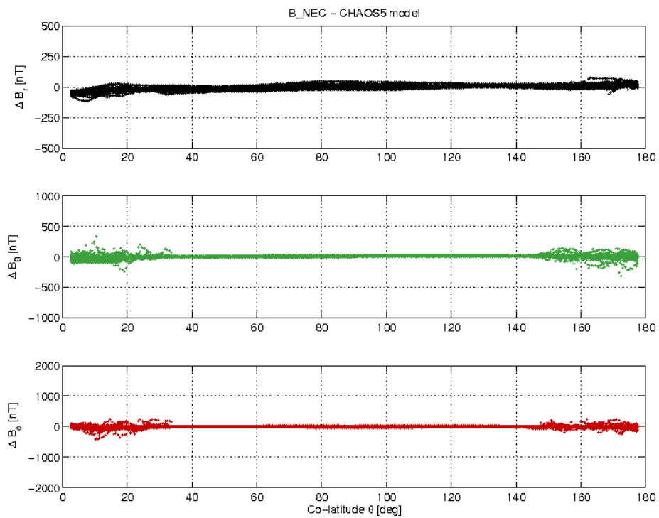
Figure 21: S/C C day 22/08 B_{NEC} - B_{Chaos} difference vs colatitude.
