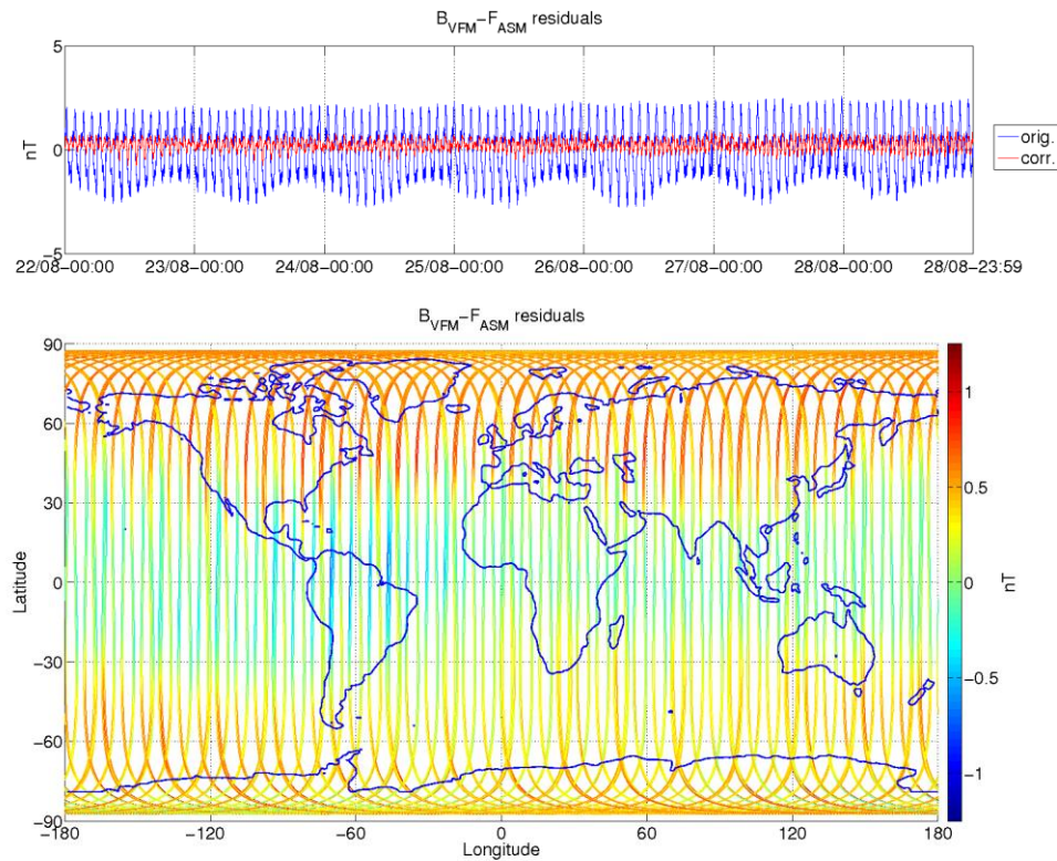
Figure 8: ASM-VFM residuals for S/C A, during monitoring period 22/08-28/08. In top figure are plotted: difference between |B_{VFM}| and F_{ASM} (without dB_Sun correction) (blue colour), and the residuals with dB_Sun corrections (red colour). In bottom figure residuals are presented on the world map.
