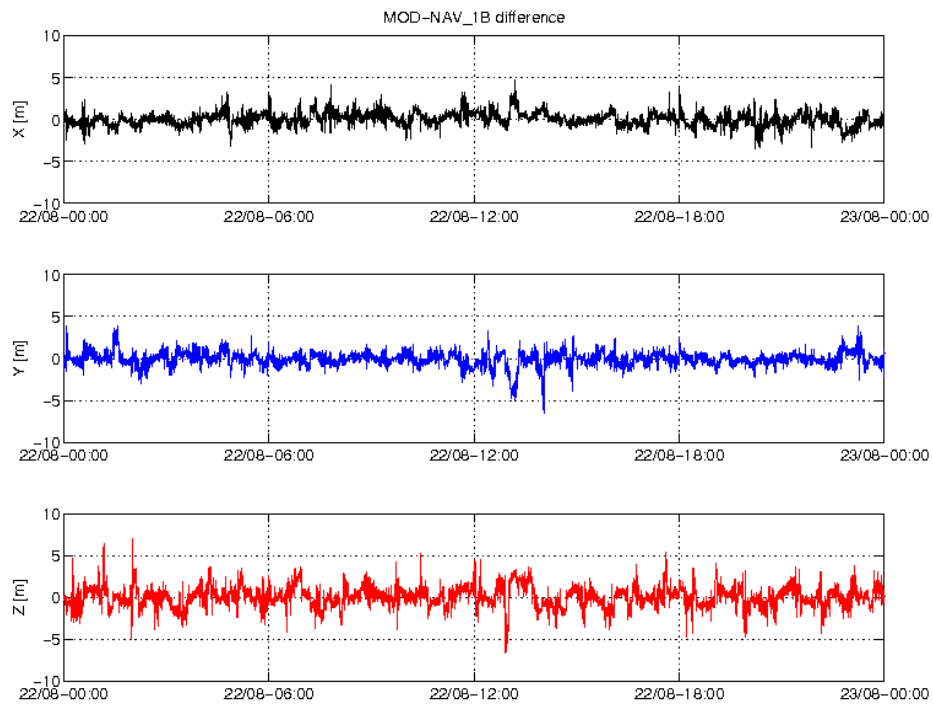
Figure 3: Difference MOD-GPSNAV, S/C A, 22/08. From top to bottom: X, Y and Z-axis
