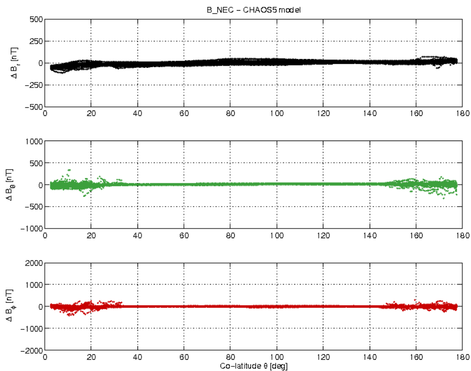
Figure 17: S/C A day 22/08 B_{NEC} - B_{Chaos} vs colatitude.
