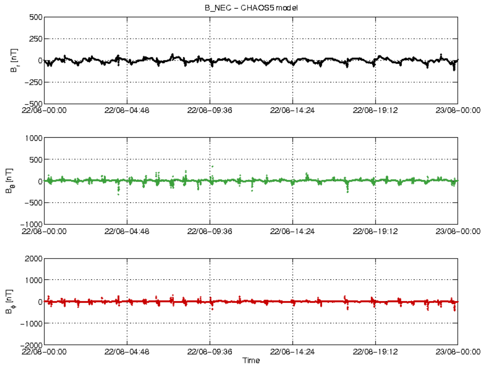
Figure 18: S/C A day 22/08: time series of B_{NEC} - B_{Chaos} residuals.
