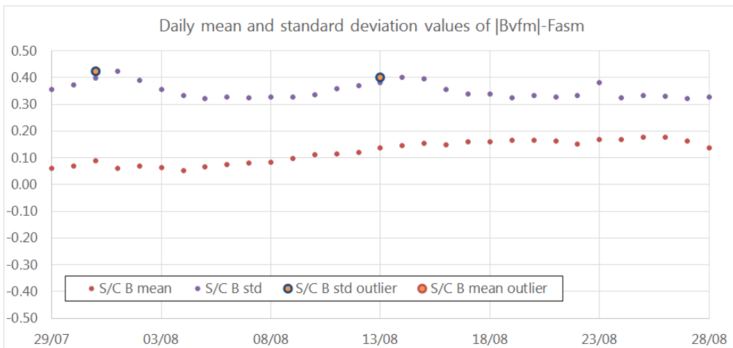
Figure 7: Daily mean and standard deviation values of ASM-VFM residuals (defined as dF=|B_{VFM}|-F_{ASM} ) for S/C B. The standard deviation jump on 23/08 is caused by collision avoidance manoeuvre.
