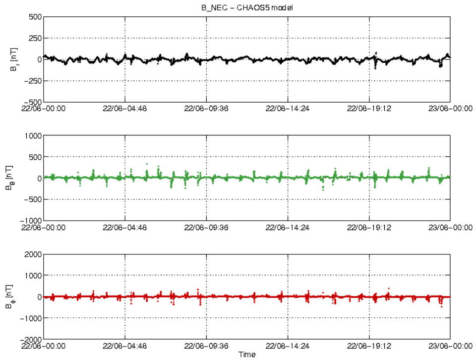
Figure 20: S/C B day 22/08 time series of B_{NEC} - B_{Chaos} residuals.
