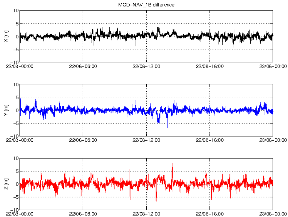
Figure 5: Difference MOD-GPSNAV, S/C C, 22/08. From top to bottom: X, Y and Z-axis
