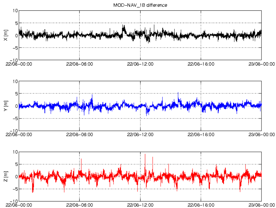
Figure 4: Difference MOD-GPSNAV, S/C B, 22/08. From top to bottom: X, Y and Z-axis
