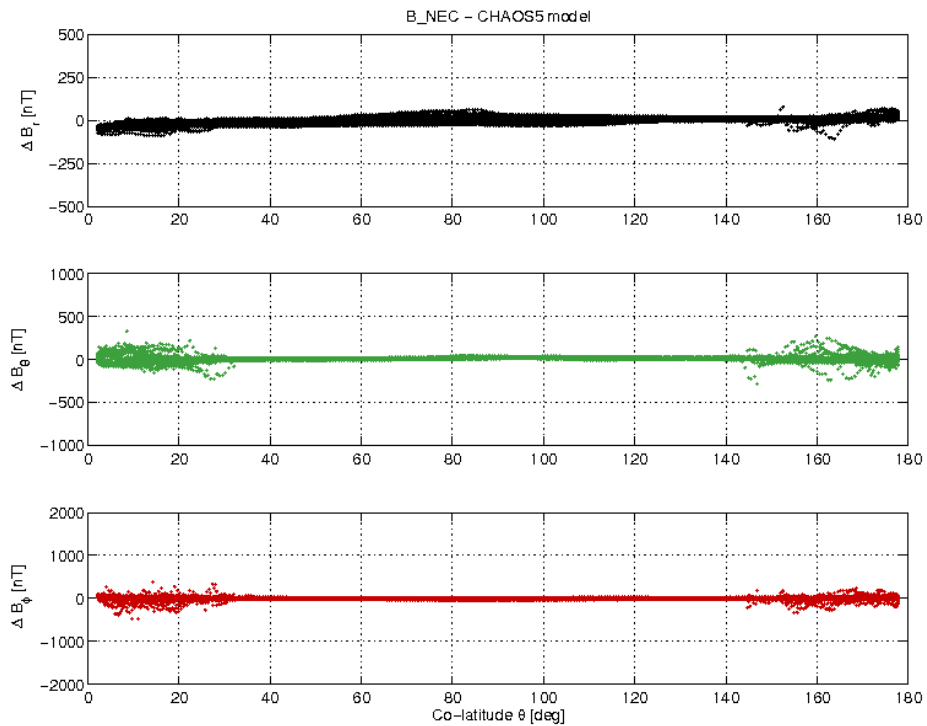
Figure 19: S/C B day 22/08 B_{NEC} - B_{Chaos} difference vs colatitude.
