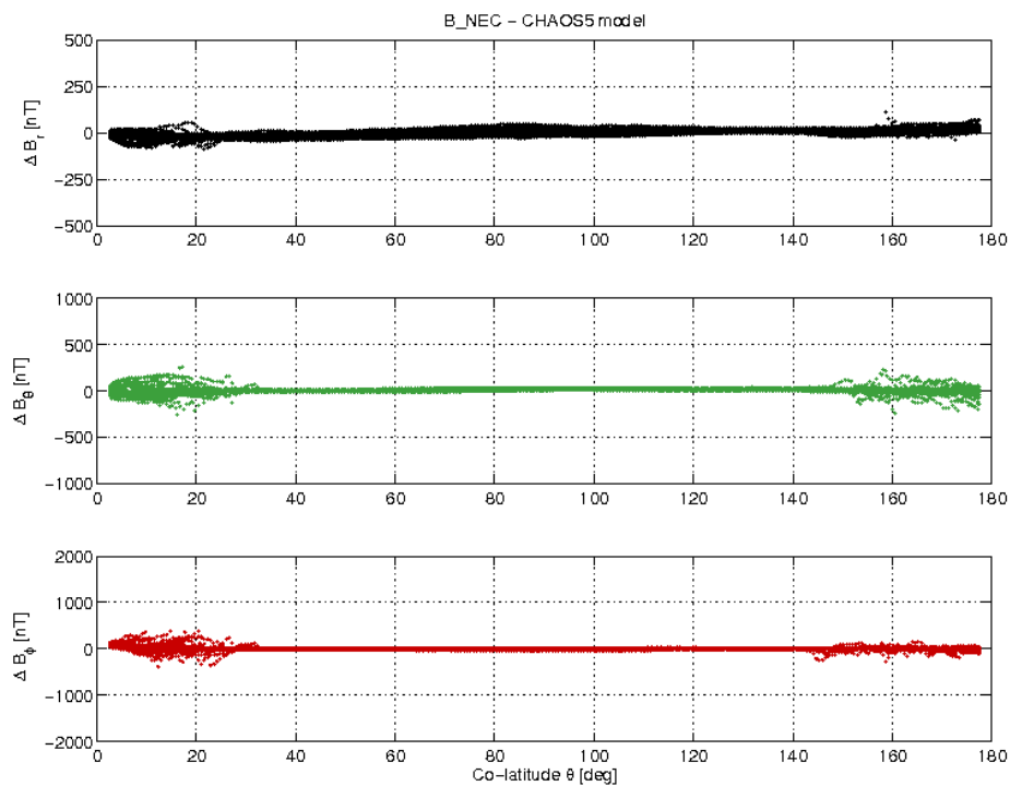
Figure 17: S/C A day 15/08 B_{NEC} - B_{Chaos} vs colatitude.
