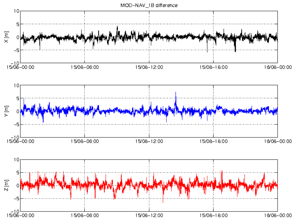
Figure 5: Difference MOD-GPSNAV, S/C C, 15/08. From top to bottom: X, Y and Z-axis
