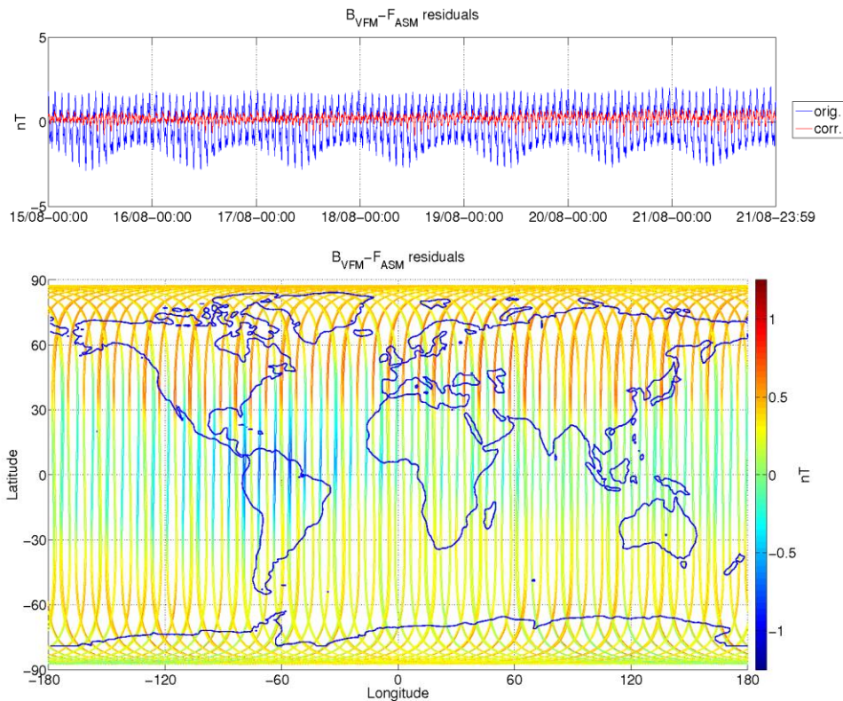
Figure 8: ASM-VFM residuals for S/C A, during monitoring period 15/08-21/08. In top figure are plotted: difference between |B_{VFM}| and F_{ASM} (without dB_Sun correction) (blue colour), and the residuals with dB_Sun corrections (red colour). In bottom figure residuals are presented on the world map.
