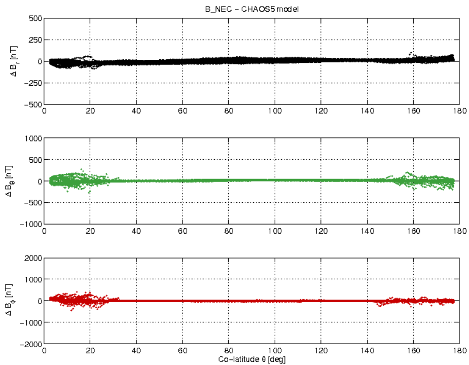
Figure 21: S/C C day 15/08 B_{NEC} - B_{Chaos} difference vs colatitude.
