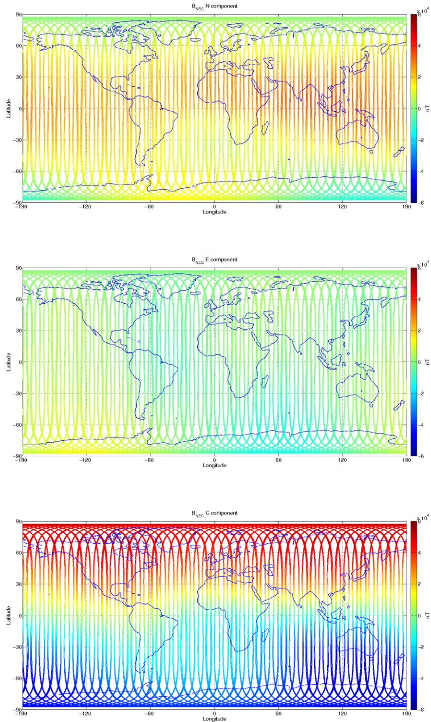
Figure 12: S/C C, world map plots of the geomagnetic field and components measured during monitoring period 15/08-21/08. From top to bottom: B NEC components (North, East, and Centre) of magnetic field from VFM measurement.
