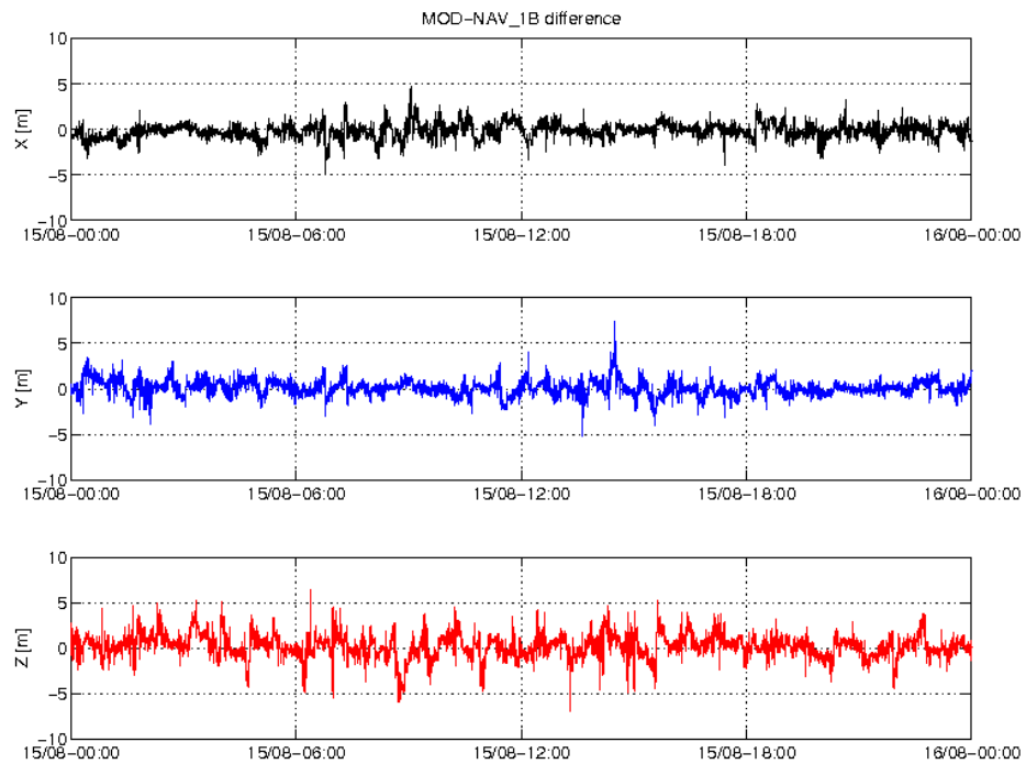
Figure 3: Difference MOD-GPSNAV, S/C A, 15/08. From top to bottom: X, Y and Z-axis
