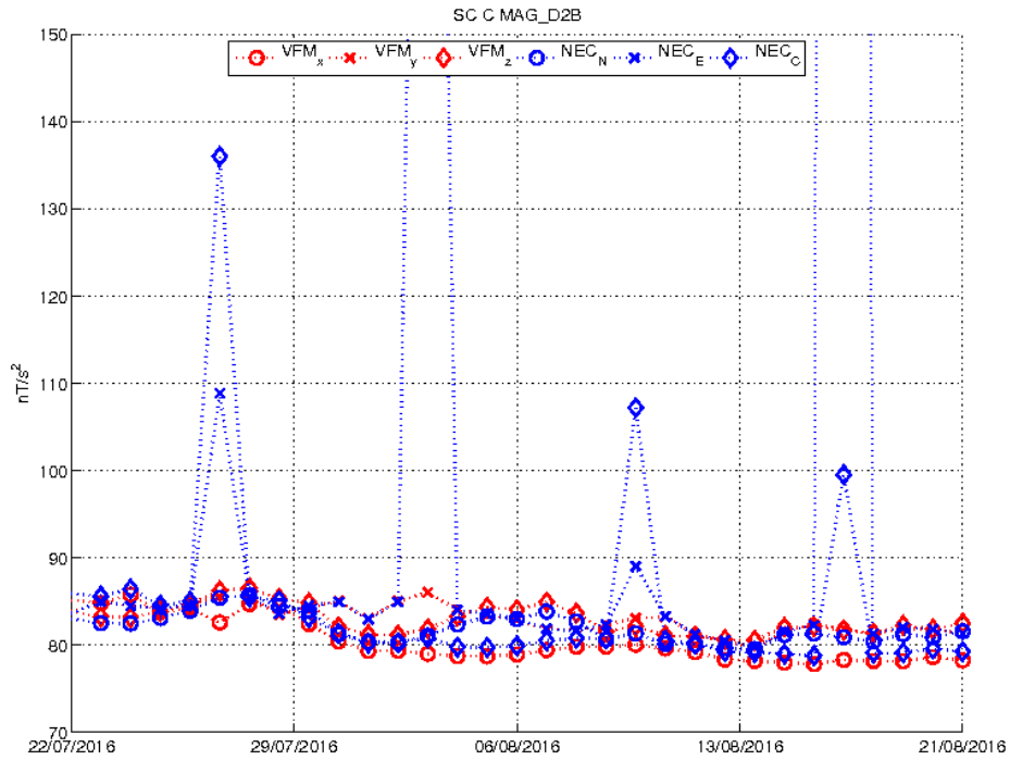
Figure 25: Plot of the daily standard deviation of the second derivative of B components in VFM and NEC frames for the last month.
