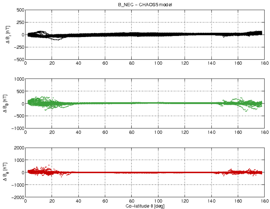
Figure 19: S/C B day 15/08 B_{NEC} - B_{Chaos} difference vs colatitude.
