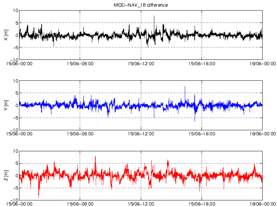
Figure 4: Difference MOD-GPSNAV, S/C B, 15/08. From top to bottom: X, Y and Z-axis
