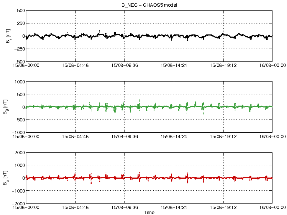
Figure 22: S/C C day 15/08 time series of B_{NEC} - B_{CHAOS} residuals.
