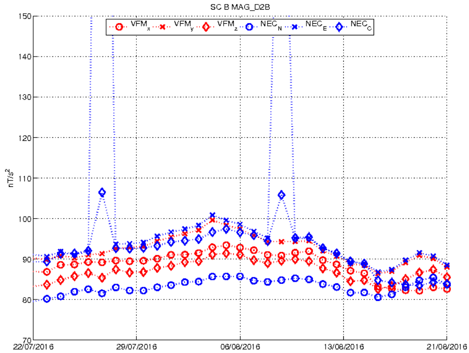
Figure 24: Plot of the daily standard deviation of the second derivative of B components in VFM and NEC frames for the last month.
