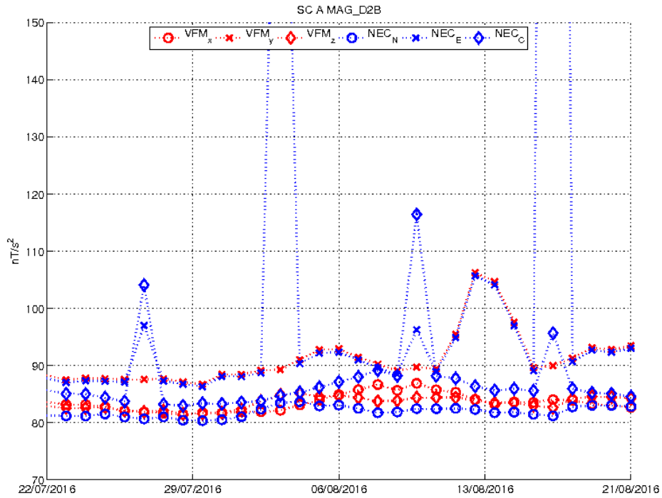
Figure 23: Plot of the daily standard deviation of the second derivative of B components in VFM and NEC frames for the last month.
