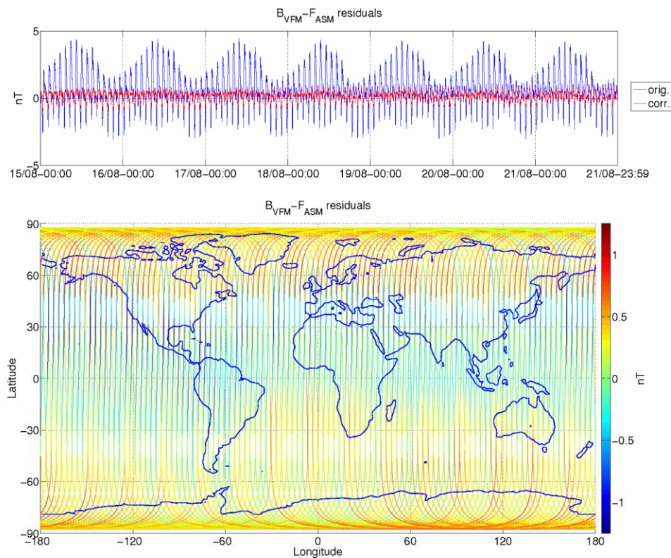
Figure 9: ASM-VFM residuals for S/C B, during monitoring period 15/08-21/08. In top figure are plotted: difference between |B_{VFM}| and F_{ASM} (without dB_{Sun} correction) (blue colour), and the residuals with dB_{Sun} corrections (red colour). In bottom figure residuals are presented on the world map.
