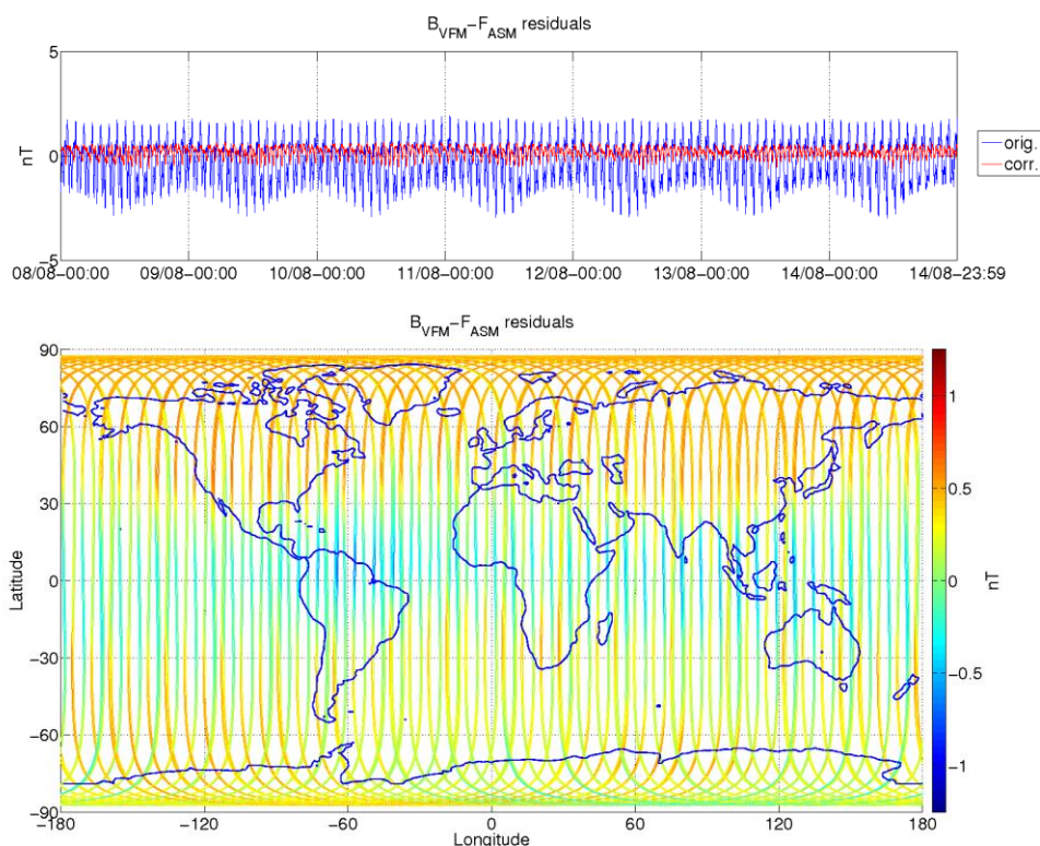
Figure 8: ASM-VFM residuals for S/C A, during monitoring period 08/08-14/08. In top figure are plotted: difference between |B_{VFM}| and F_{ASM} (without dB_Sun correction) (blue colour), and the residuals with dB_Sun corrections (red colour). In bottom figure residuals are presented on the world map.
