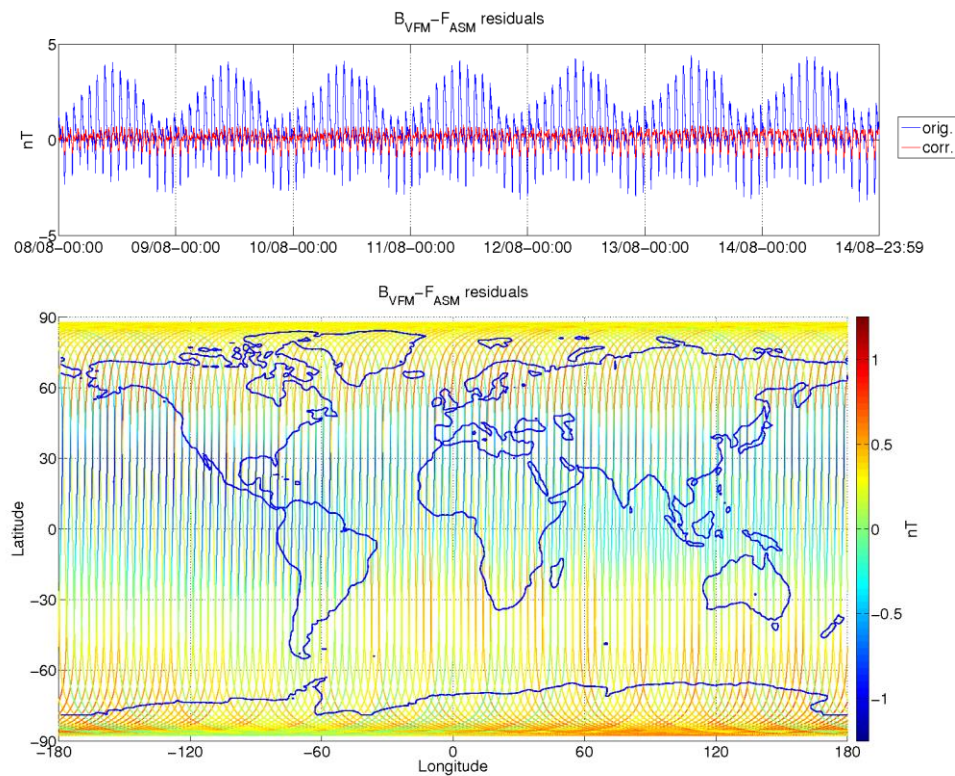
Figure 9: ASM-VFM residuals for S/C B, during monitoring period 08/08-14/08. In top figure are plotted: difference between |B_{VFM}| and F_{ASM} (without dB_Sun correction) (blue colour), and the residuals with dB_Sun corrections (red colour). In bottom figure residuals are presented on the world map.
