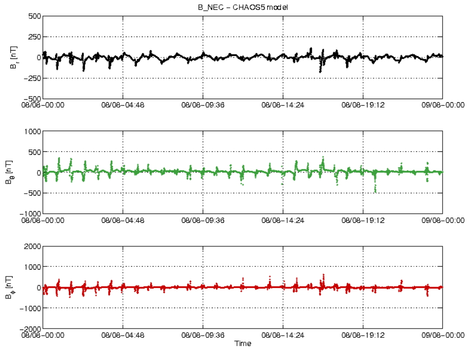
Figure 20: S/C B day 08/08 time series of B_{NEC} - B_{Chaos} residuals.
