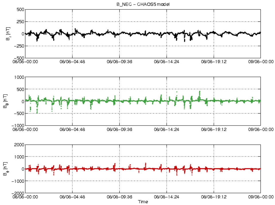
Figure 18: S/C A day 08/08: time series of B_{NEC} - B_{Chaos} residuals.
