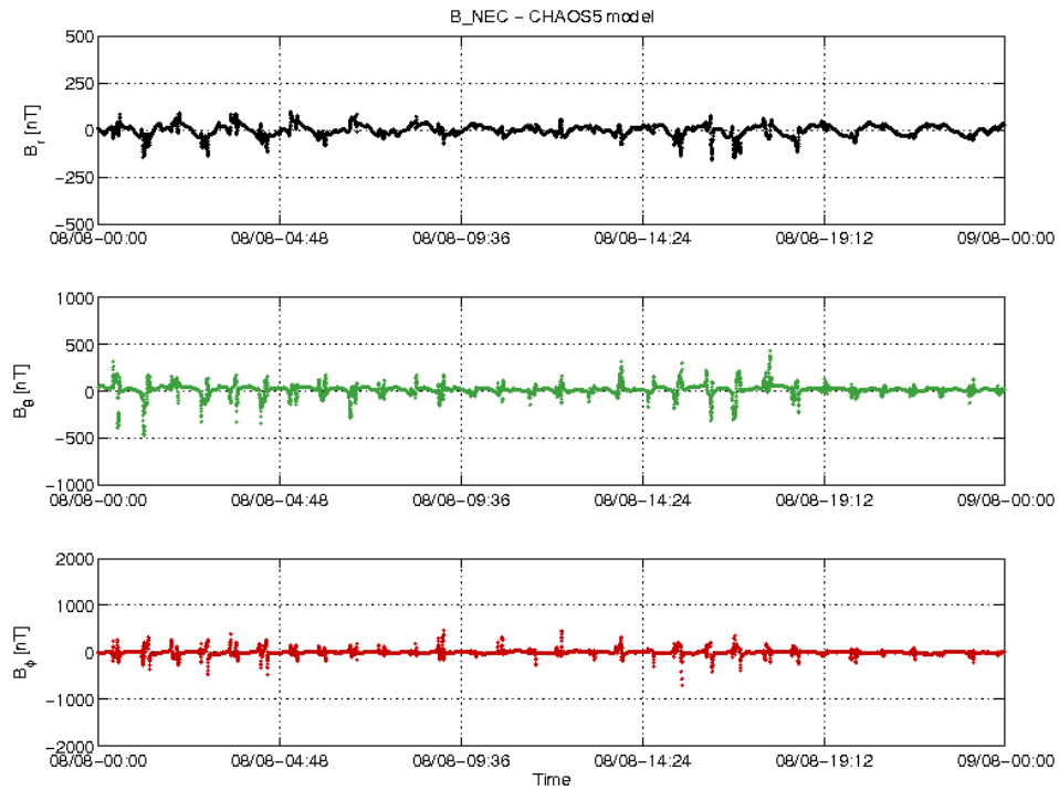
Figure 22: S/C C day 08/08 time series of B_{NEC} - B_{Chaos} residuals.
