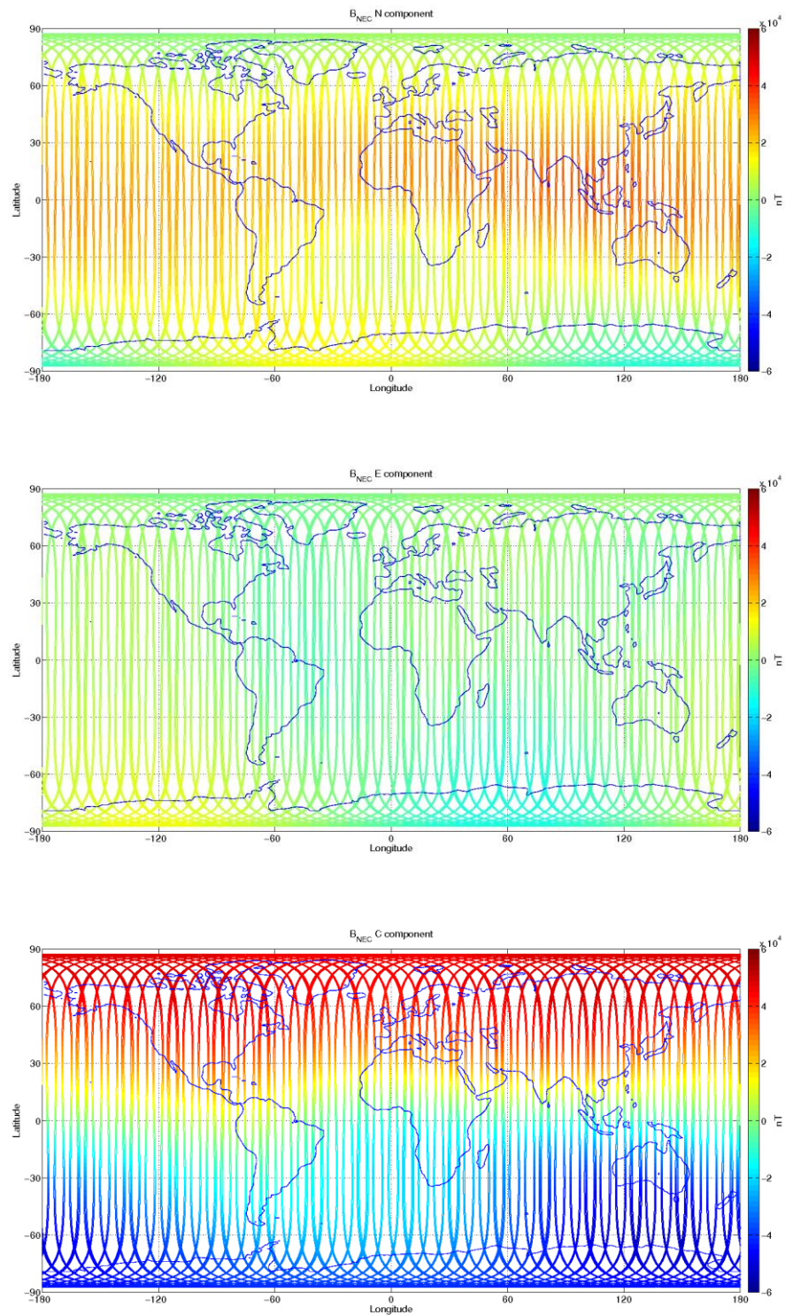
Figure 12: S/C C, world map plots of the geomagnetic field and components measured during monitoring period 08/08-14/08. From top to bottom: B NEC components (North, East, and Centre) of magnetic field from VFM measurement.
