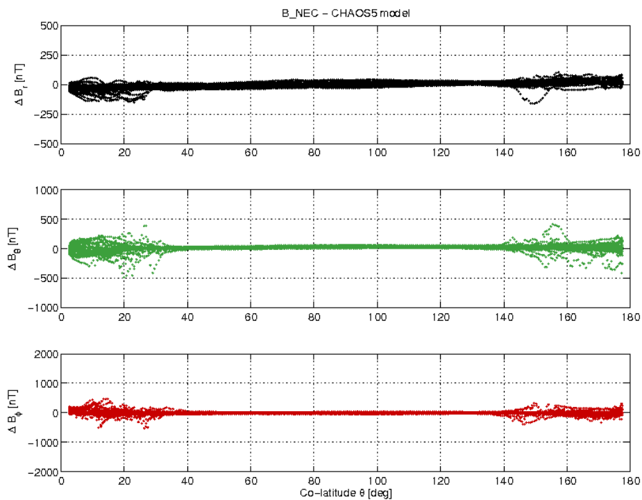
Figure 17: S/C A day 08/08 B_{NEC} - B_{Chaos} vs colatitude.
