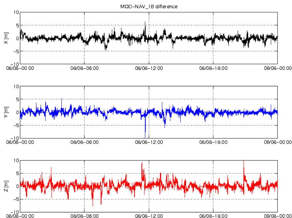
Figure 5: Difference MOD-GPSNAV, S/C C, 08/08. From top to bottom: X, Y and Z-axis
