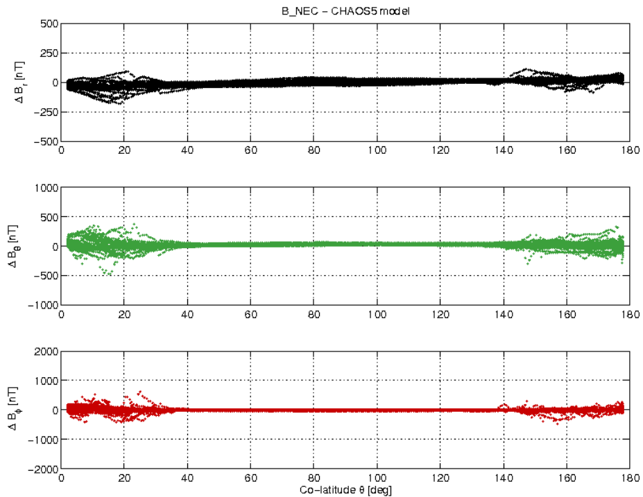
Figure 19: S/C B day 08/08 B_{NEC} - B_{Chaos} difference vs colatitude.
