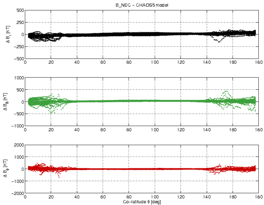
Figure 21: S/C C day 08/08 B_{NEC} - B_{Chaos} difference vs colatitude.
