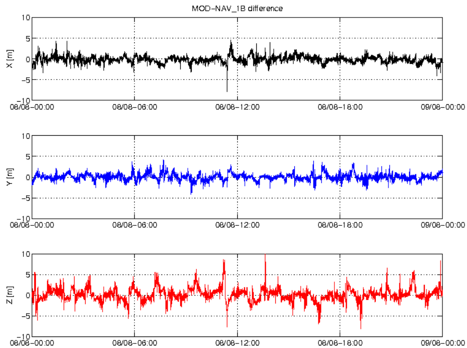
Figure 4: Difference MOD-GPSNAV, S/C B, 08/08. From top to bottom: X, Y and Z-axis
