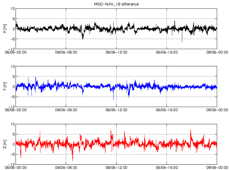
Figure 3: Difference MOD-GPSNAV, S/C A, 08/08. From top to bottom: X, Y and Z-axis
