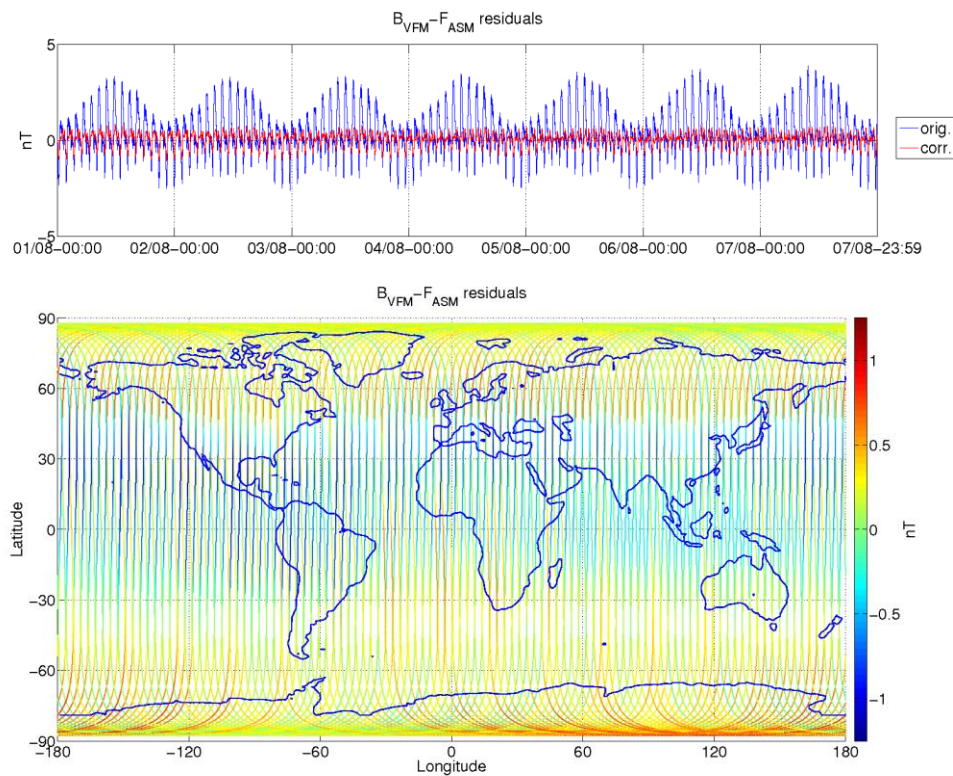
Figure 9: ASM-VFM residuals for S/C B, during monitoring period 01/08-07/08. In top figure are plotted: difference between |B_{VFM}| and F_{ASM} (without dB_Sun correction) (blue colour), and the residuals with dB_Sun corrections (red colour). In bottom figure residuals are presented on the world map.
