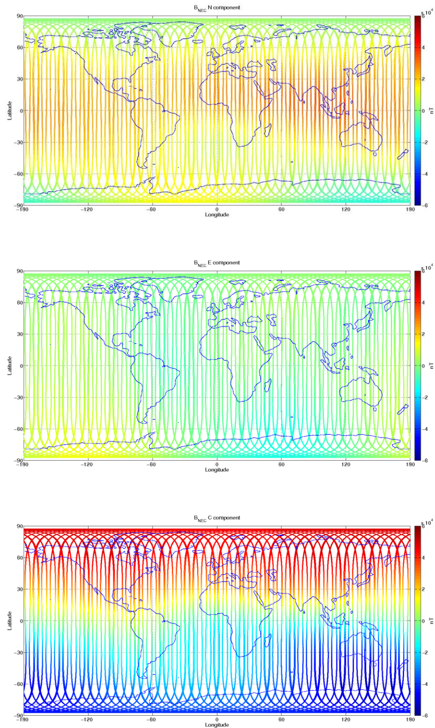
Figure 12: S/C C, world map plots of the geomagnetic field and components measured during monitoring period 01/08-07/08. From top to bottom: B_{NEC} components (North, East, and Centre) of magnetic field from VFM measurement.
