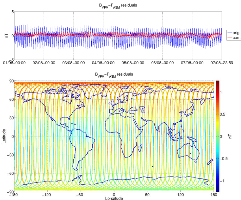
Figure 8: ASM-VFM residuals for S/C A, during monitoring period 01/08-07/08. In top figure are plotted: difference between |B VFM | and F ASM (without dB Sun correction) (blue colour), and the residuals with dB Sun corrections (red colour). In bottom figure residuals are presented on the world map.
