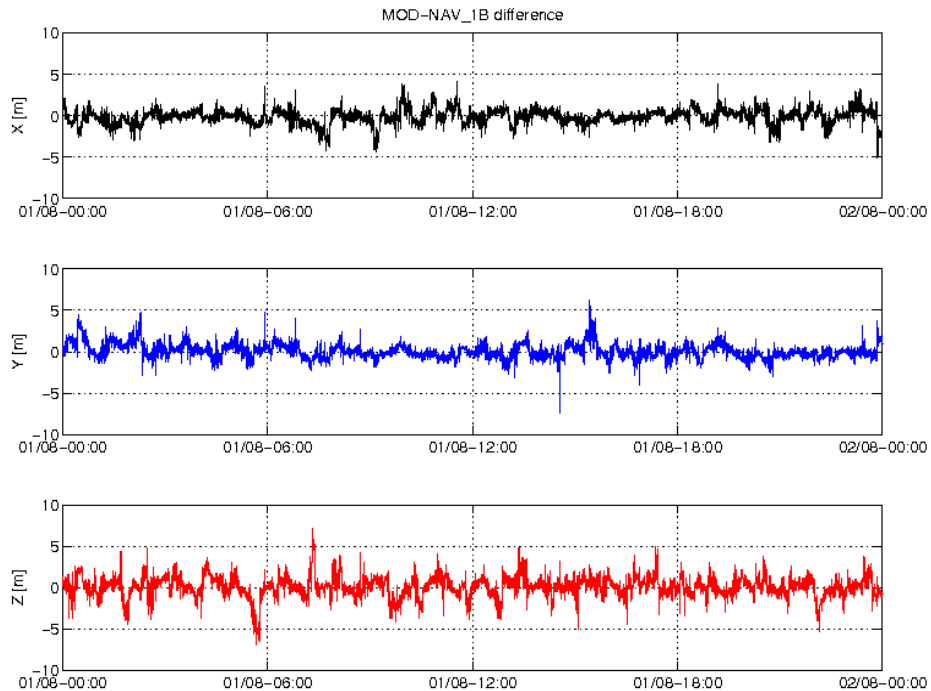
Figure 5: Difference MOD-GPSNAV, S/C C, 01/08. From top to bottom: X, Y and Z-axis
