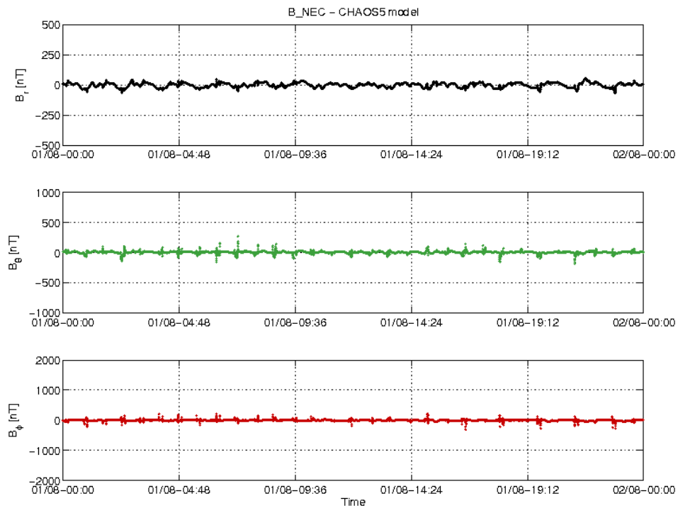
Figure 22: S/C C day 01/08 time series of B_{NEC} - B_{Chaos} residuals.
