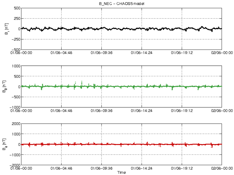
Figure 18: S/C A day 01/08: time series of B_{NEC} - B_{Chaos} residuals.
