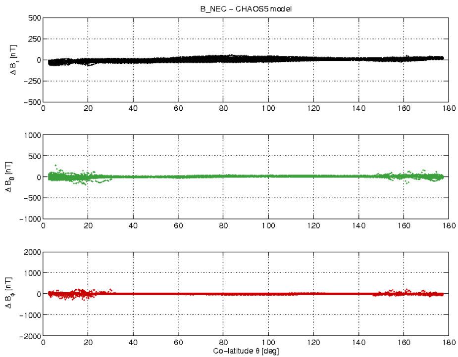
Figure 21: S/C C day 01/08 B_{NEC} - B_{Chaos} difference vs colatitude.
