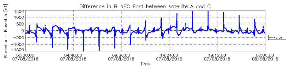
Figure 15: Difference in B_{NEC} East component between S/C A and S/C C.
