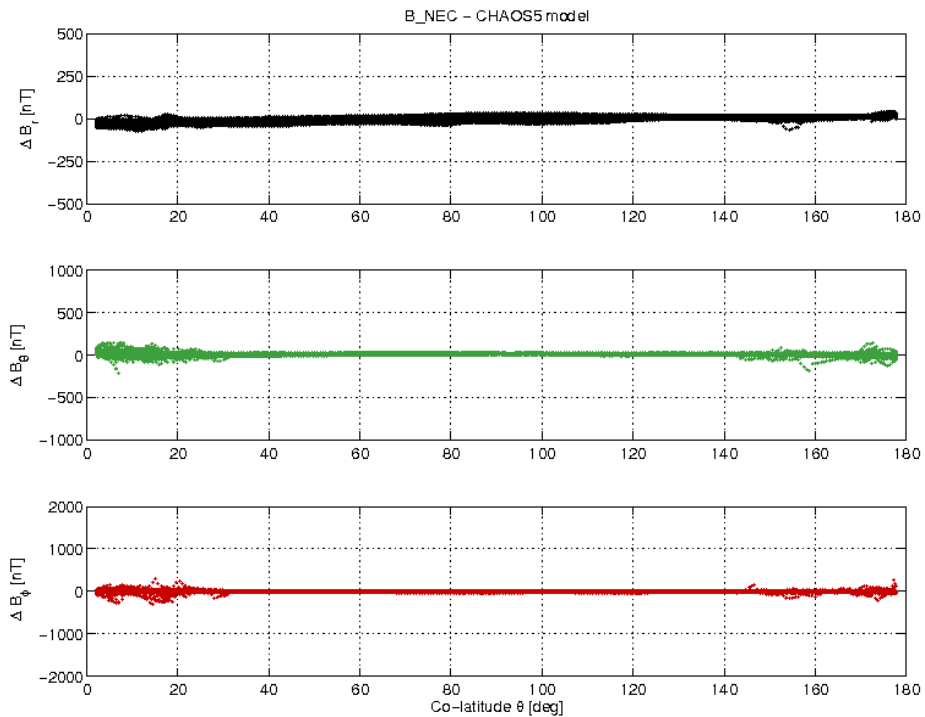
Figure 19: S/C B day 01/08 B_{NEC} - B_{Chaos} difference vs colatitude.
