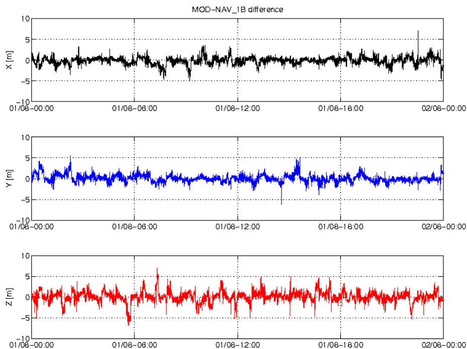
Figure 3: Difference MOD-GPSNAV, S/C A, 01/08. From top to bottom: X, Y and Z-axis
