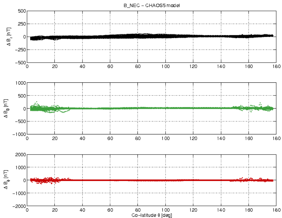
Figure 17: S/C A day 01/08 B_{NEC} - B_{Chaos} vs colatitude.
