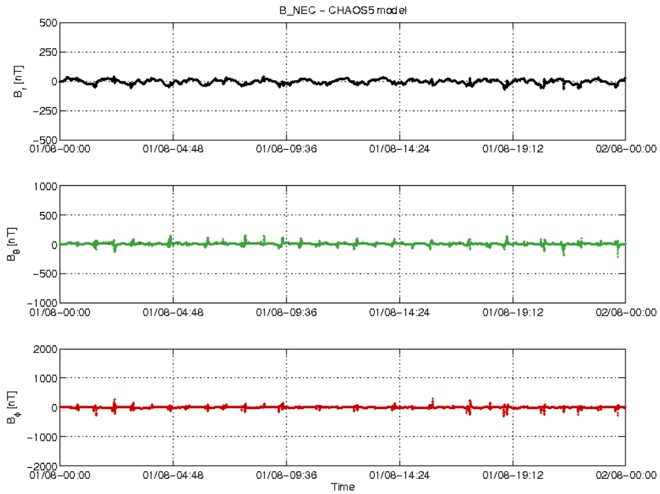
Figure 20: S/C B day 01/08 time series of B_{NEC} - B_{Chaos} residuals.
