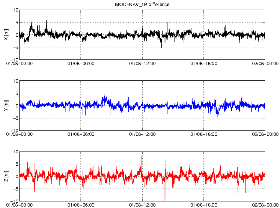
Figure 4: Difference MOD-GPSNAV, S/C B, 01/08. From top to bottom: X, Y and Z-axis
