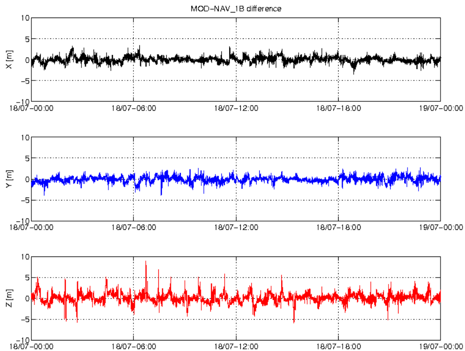
Figure 4: Difference MOD-GPSNAV, S/C B, 18/07. From top to bottom: X, Y and Z-axis
