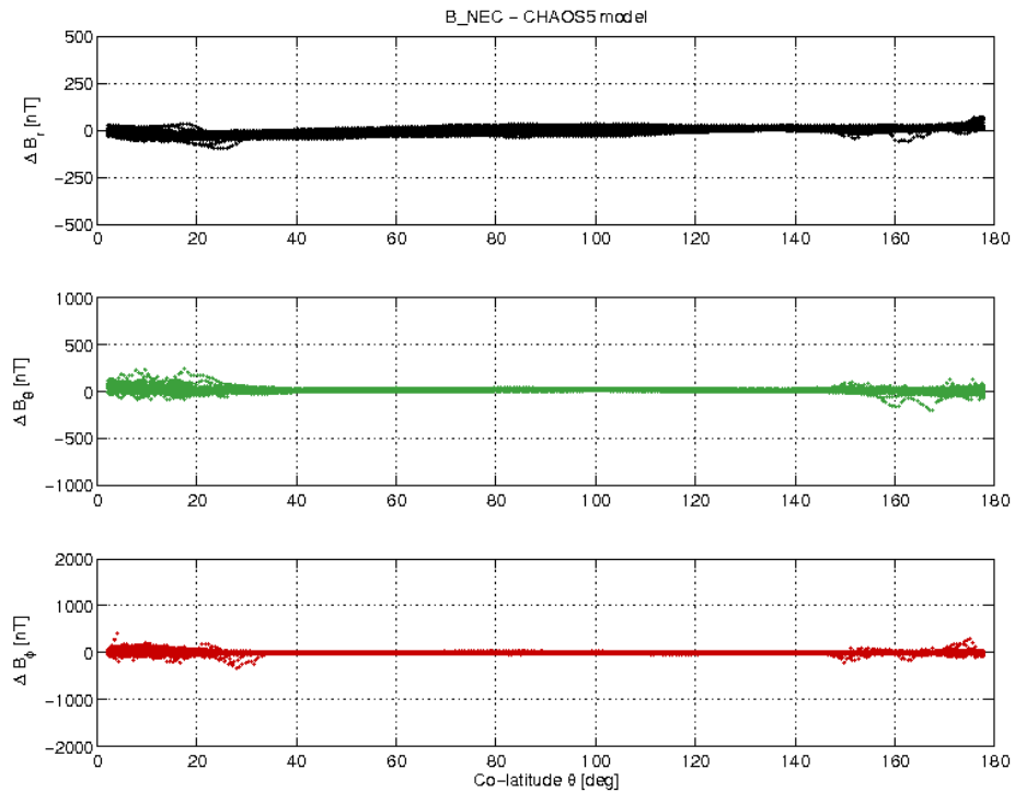
Figure 19: S/C B day 18/07 B_{NEC} - B_{Chaos} difference vs colatitude.
