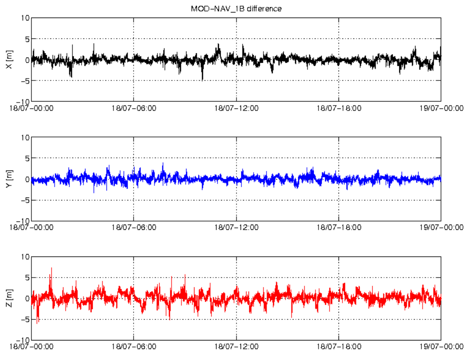
Figure 3: Difference MOD-GPSNAV, S/C A, 18/07. From top to bottom: X, Y and Z-axis
