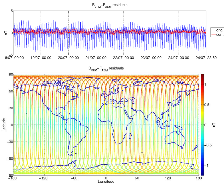
Figure 8: ASM-VFM residuals for S/C A, during monitoring period 18/07-24/07. In top figure are plotted: difference between |B_{VFM}| and F_{ASM} (without dB_{Sun} correction) (blue colour), and the residuals with dB_{Sun} corrections (red colour). In bottom figure residuals are presented on the world map.
