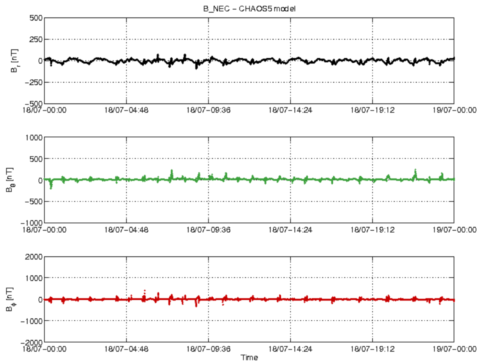
Figure 20: S/C B day 18/07 time series of B_{NEC} - B_{Chaos} residuals.
