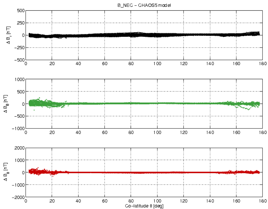
Figure 17: S/C A day 18/07 B_{NEC} - B_{Chaos} vs colatitude.
