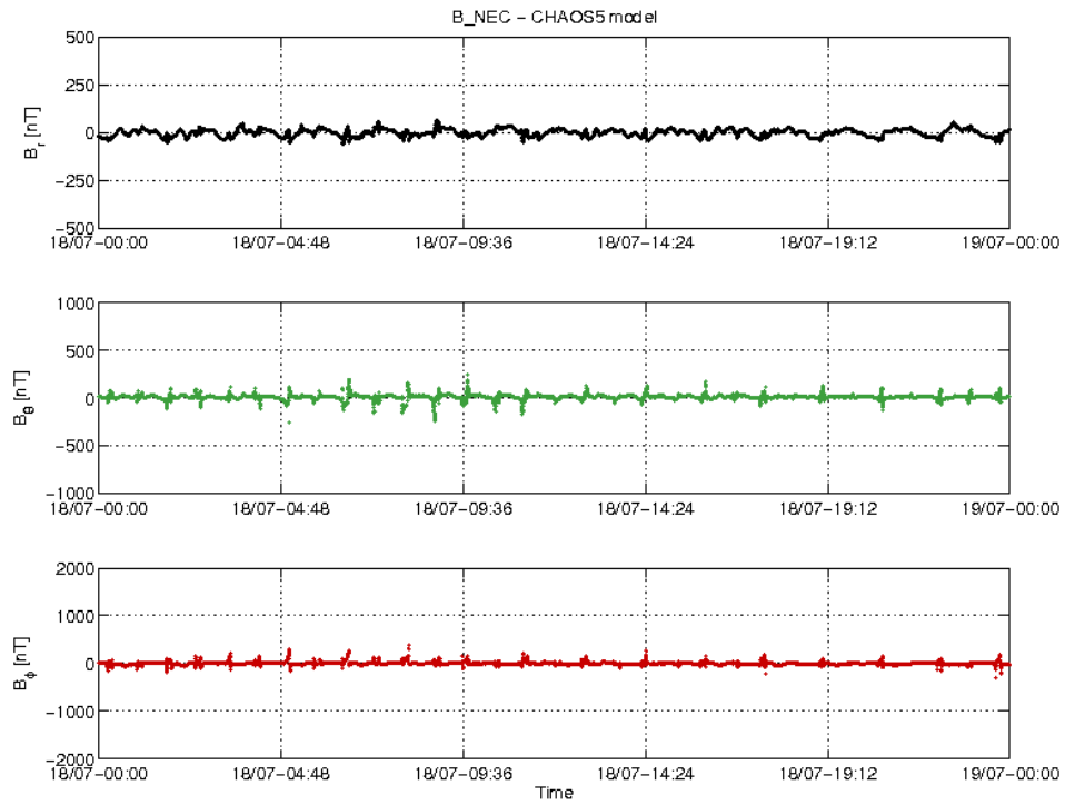
Figure 18: S/C A day 18/07: time series of B_{NEC} - B_{Chaos} residuals.
