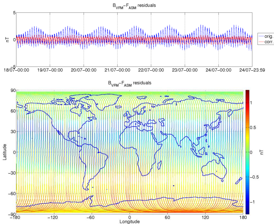
Figure 9: ASM-VFM residuals for S/C B, during monitoring period 18/07-24/07. In top figure are plotted: difference between |B_{VFM}| and F_{ASM} (without dB_{Sun} correction) (blue colour), and the residuals with dB_{Sun} corrections (red colour). In bottom figure residuals are presented on the world map.
