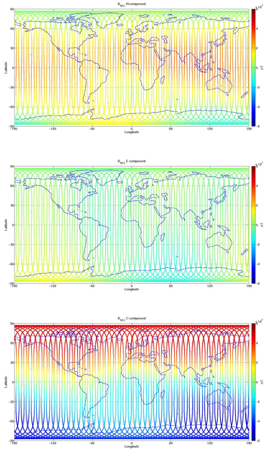
Figure 12: S/C C, world map plots of the geomagnetic field and components measured during monitoring period 18/07-24/07. From top to bottom: B NEC components (North, East, and Centre) of magnetic field from VFM measurement.
