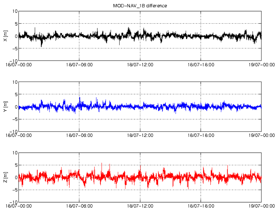
Figure 5: Difference MOD-GPSNAV, S/C C, 18/07. From top to bottom: X, Y and Z-axis
