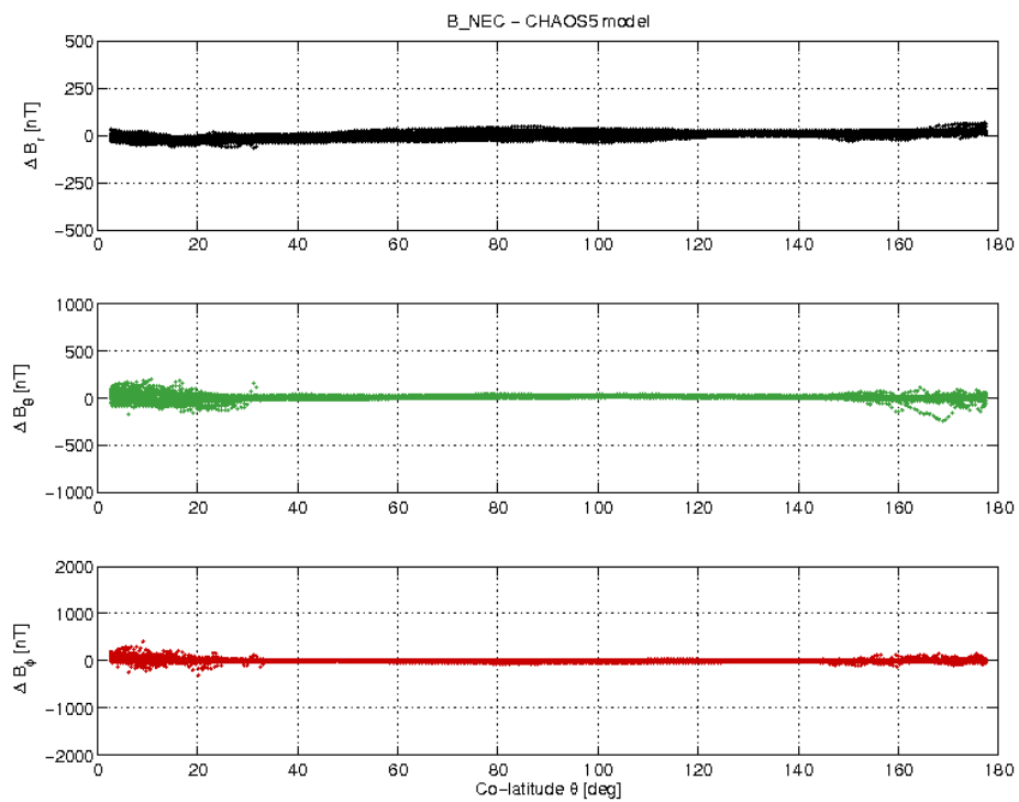
Figure 21: S/C C day 18/07 B_{NEC} - B_{Chaos} difference vs colatitude.
