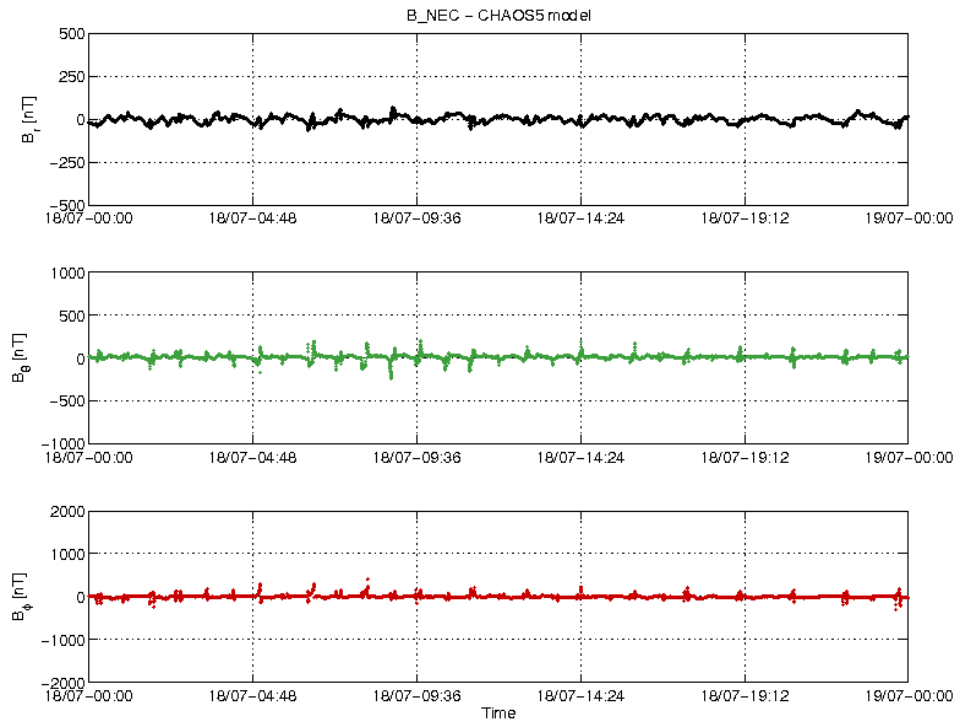
Figure 22: S/C C day 18/07 time series of B_{NEC} - B_{Chaos} residuals.
