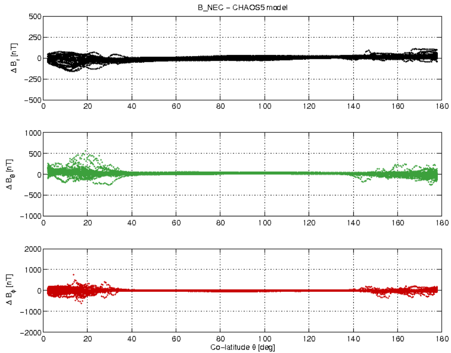
Figure 19: S/C B day 11/07 B_{NEC} - B_{Chaos} difference vs colatitude.
