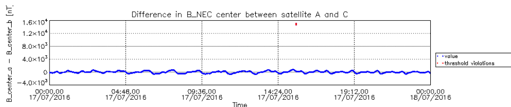
Figure 16: Difference in B NEC Center component between S/C A and S/C C.
