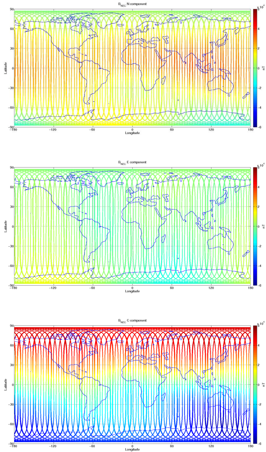
Figure 12: S/C C, world map plots of the geomagnetic field and components measured during monitoring period 11/07-17/07. From top to bottom: B NEC components (North, East, and Centre) of magnetic field from VFM measurement.
