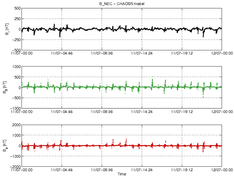
Figure 18: S/C A day 11/07: time series of B_{NEC} - B_{Chaos} residuals.
