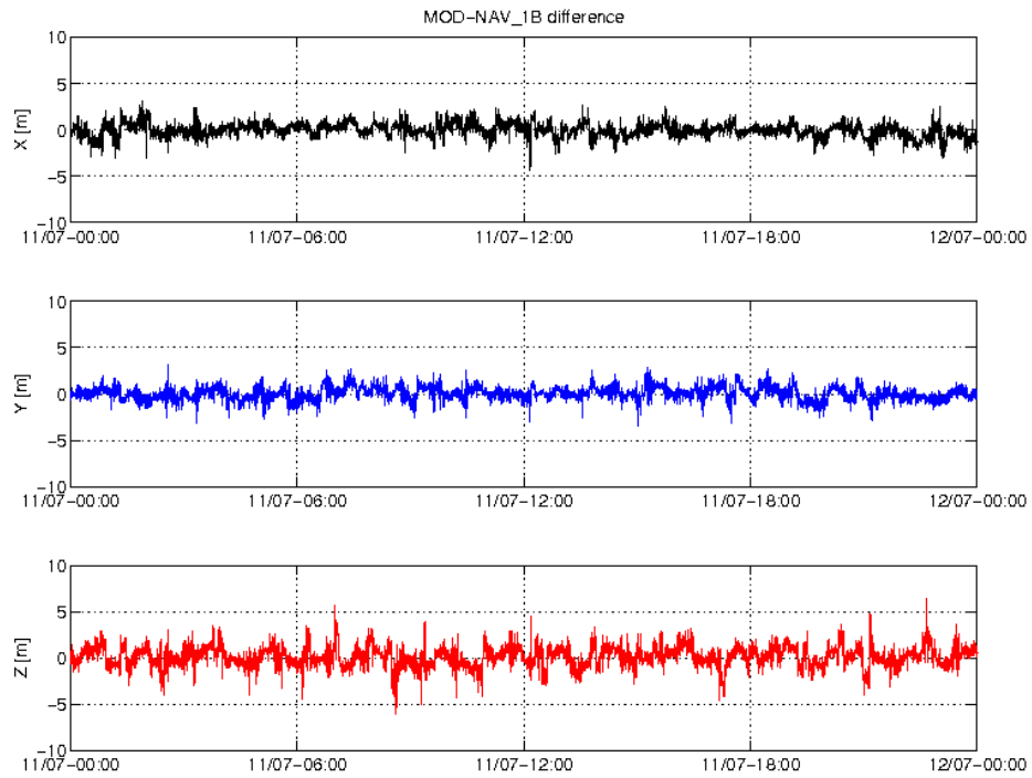
Figure 3: Difference MOD-GPSNAV, S/C A, 11/07. From top to bottom: X, Y and Z-axis
