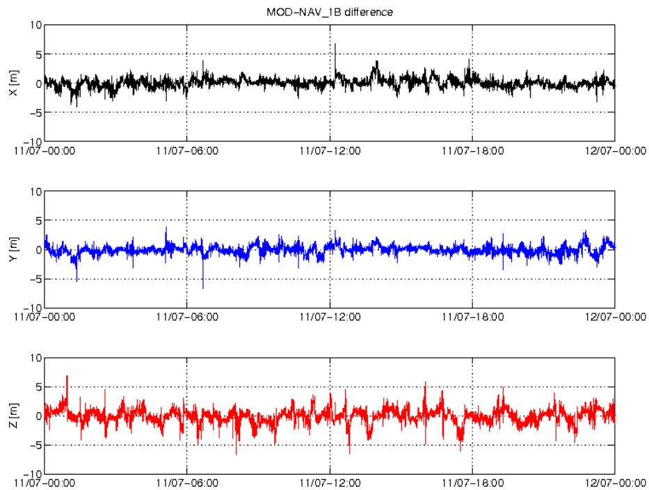
Figure 4: Difference MOD-GPSNAV, S/C B, 11/07. From top to bottom: X, Y and Z-axis
