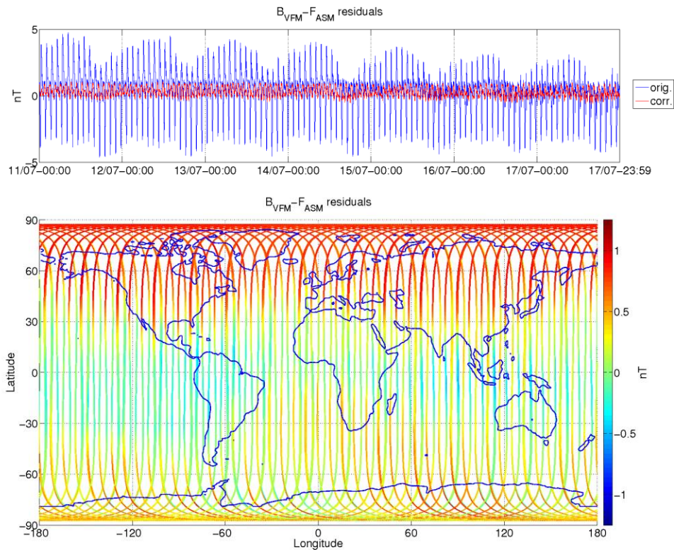
Figure 8: ASM-VFM residuals for S/C A, during monitoring period 11/07-17/07. In top figure are plotted: difference between |B_{VFM}| and F_{ASM} (without dB_{Sun} correction) (blue colour), and the residuals with dB_{Sun} corrections (red colour). In bottom figure residuals are presented on the world map.
