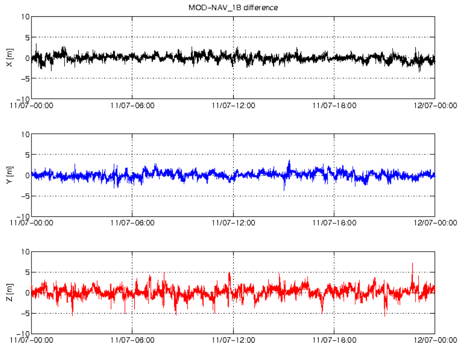
Figure 5: Difference MOD-GPSNAV, S/C C, 11/07. From top to bottom: X, Y and Z-axis
