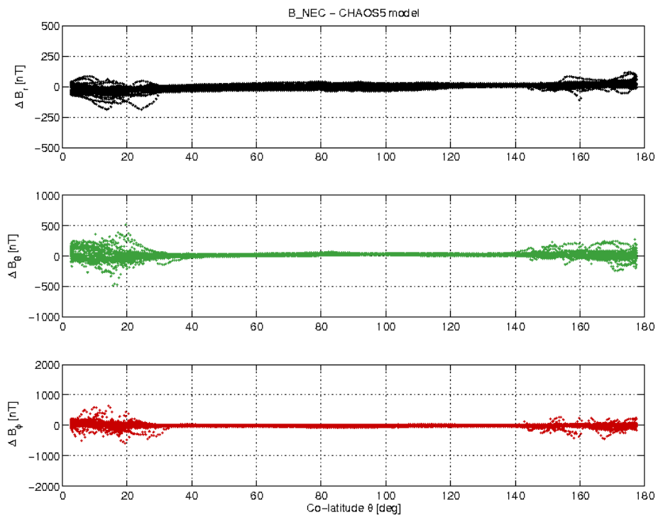
Figure 17: S/C A day 11/07 B_{NEC} - B_{Chaos} vs colatitude.
