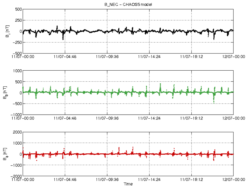
Figure 22: S/C C day 11/07 time series of B_{NEC} - B_{Chaos} residuals.
