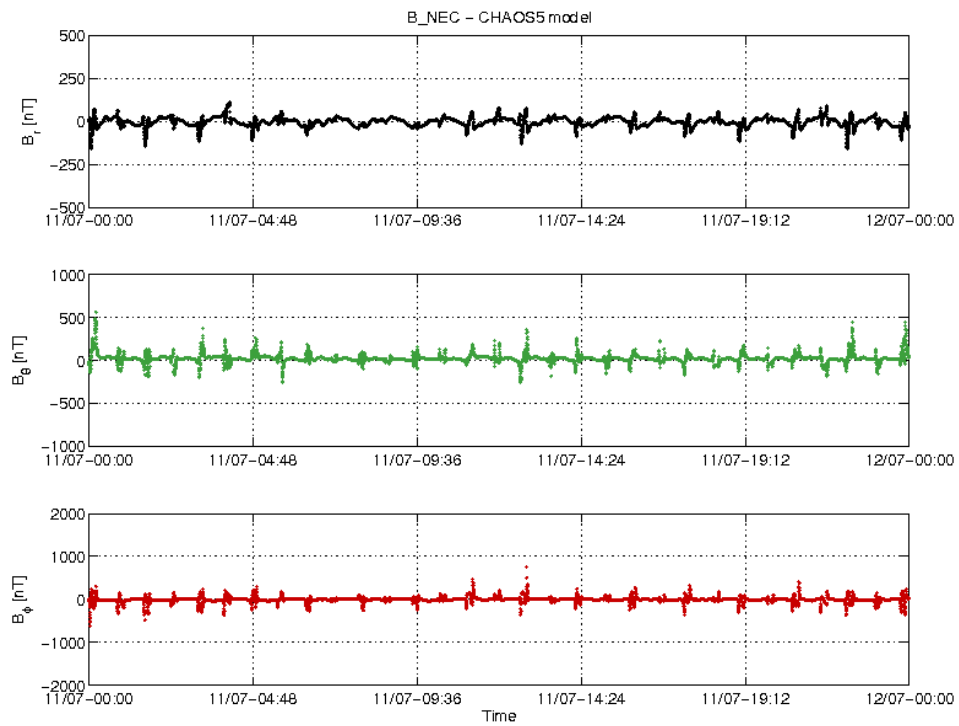
Figure 20: S/C B day 11/07 time series of B_{NEC} - B_{Chaos} residuals.
