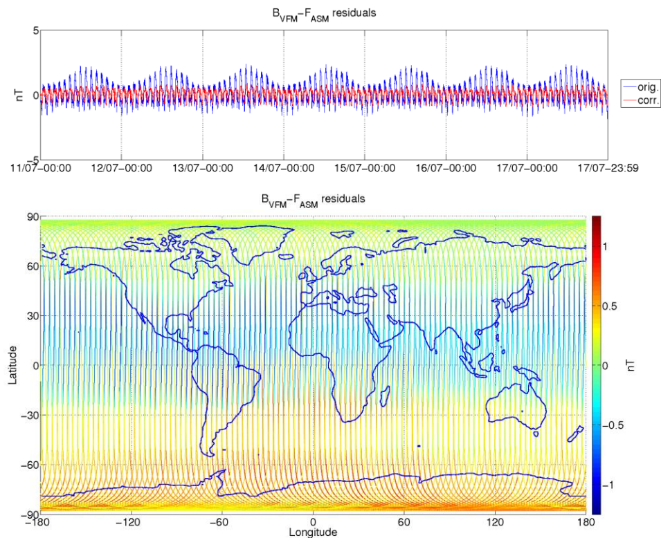
Figure 9: ASM-VFM residuals for S/C B, during monitoring period 11/07-17/07. In top figure are plotted: difference between |B_{VFM}| and F_{ASM} (without dB Sun correction) (blue colour), and the residuals with dB Sun corrections (red colour). In bottom figure residuals are presented on the world map.
