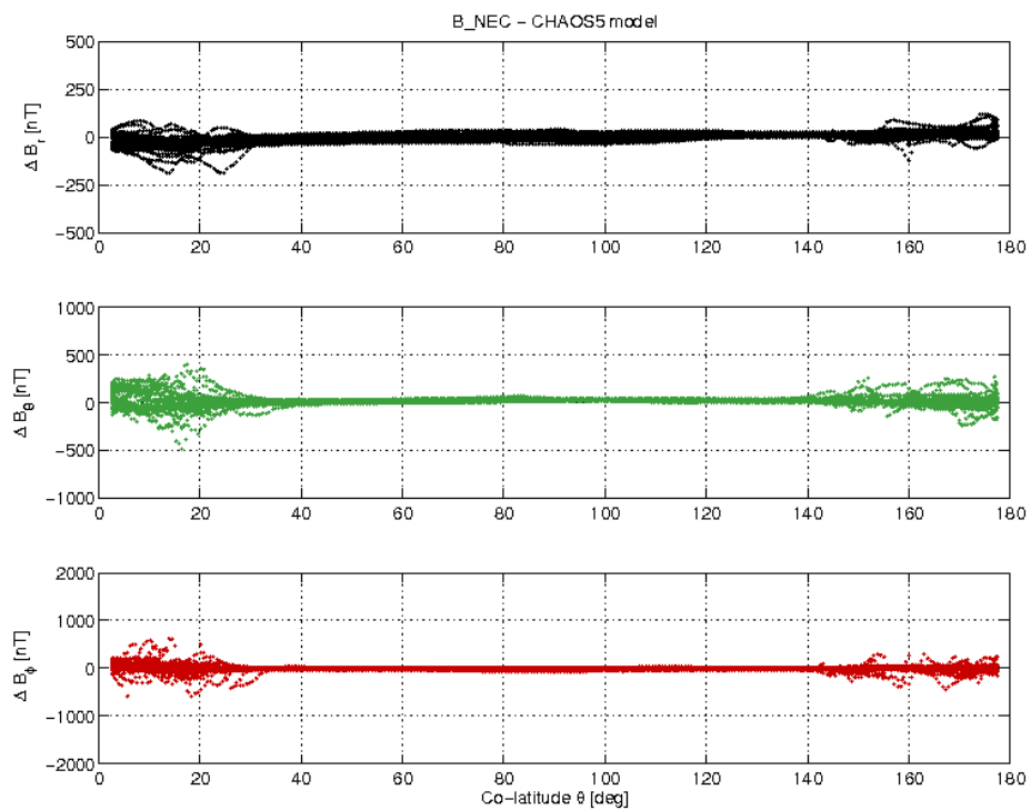
Figure 21: S/C C day 11/07 B_{NEC} - B_{Chaos} difference vs colatitude.
