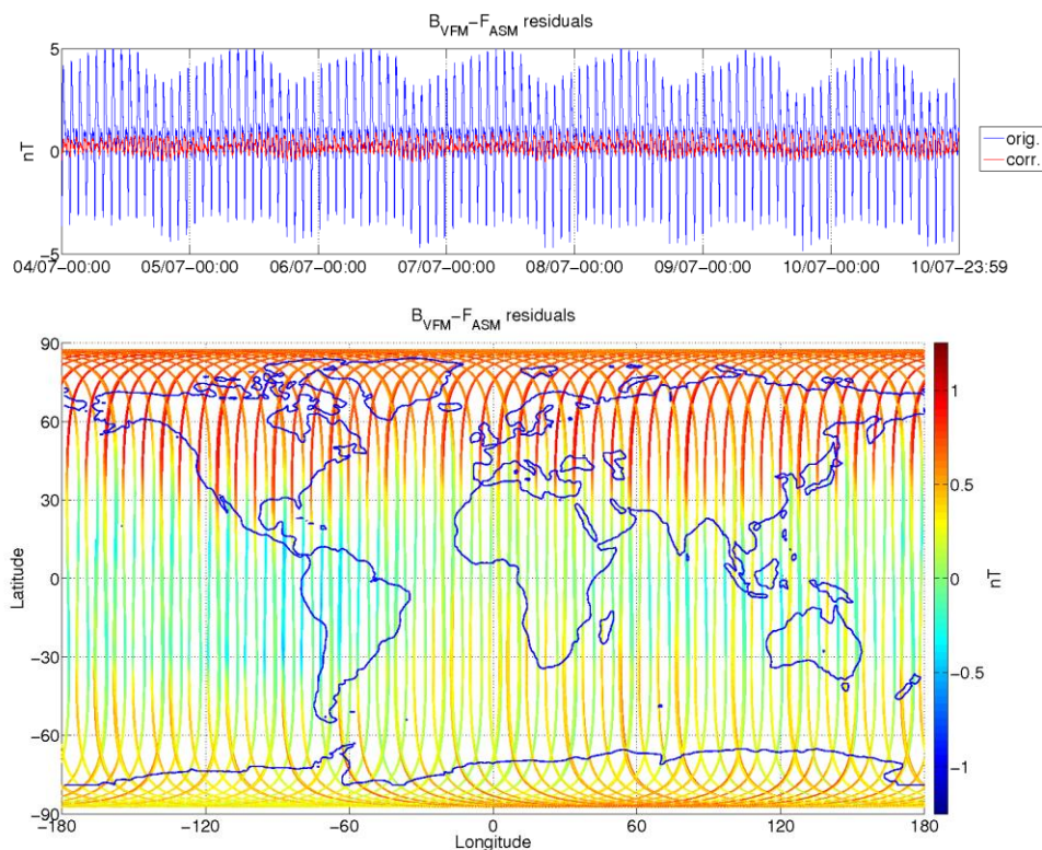
Figure 8: ASM-VFM residuals for S/C A, during monitoring period 04/07-10/07. In top figure are plotted: difference between |B_{VFM}| and F_{ASM} (without dB_{Sun} correction) (blue colour), and the residuals with dB_{Sun} corrections (red colour). In bottom figure residuals are presented on the world map.
