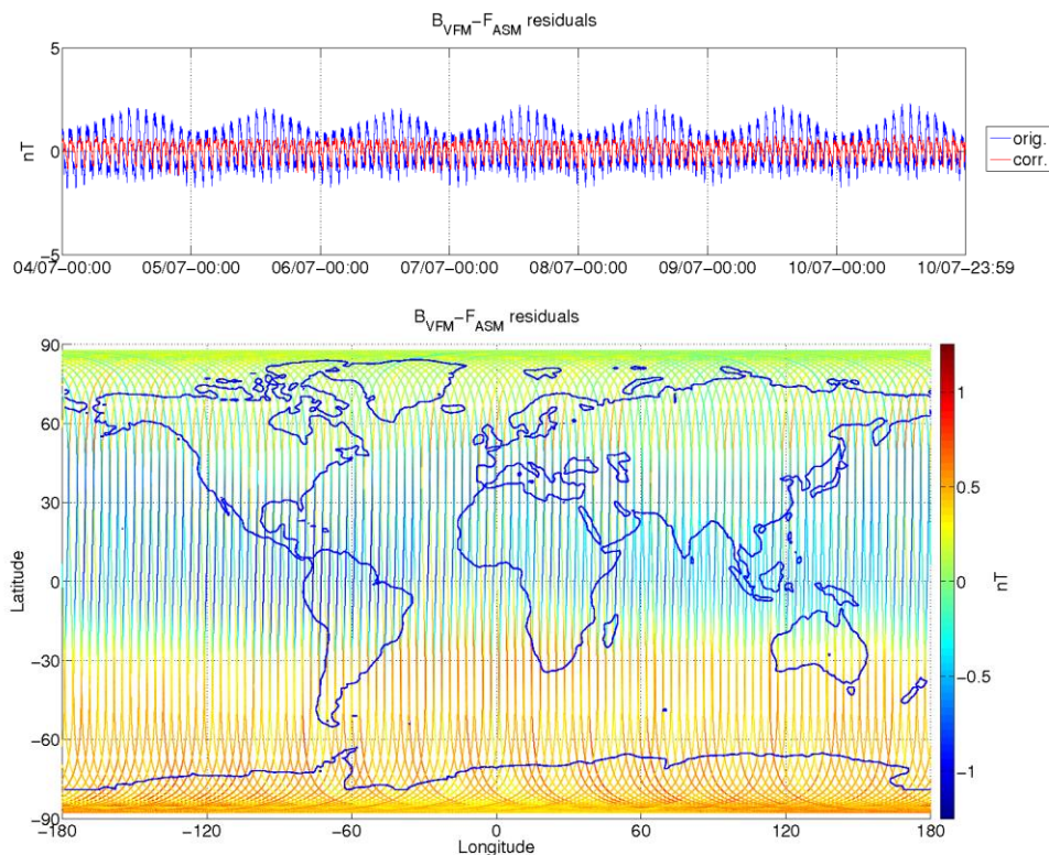
Figure 9: ASM-VFM residuals for S/C B, during monitoring period 04/07-10/07. In top figure are plotted: difference between |B_{VFM}| and F_{ASM} (without dB_Sun correction) (blue colour), and the residuals with dB_Sun corrections (red colour). In bottom figure residuals are presented on the world map.
