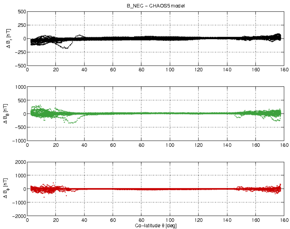
Figure 21: S/C C day 04/07 B_{NEC} - B_{Chaos} difference vs colatitude.
