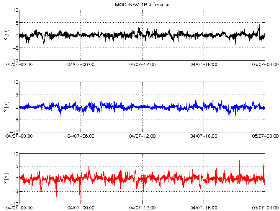
Figure 3: Difference MOD-GPSNAV, S/C A, 04/07. From top to bottom: X, Y and Z-axis
