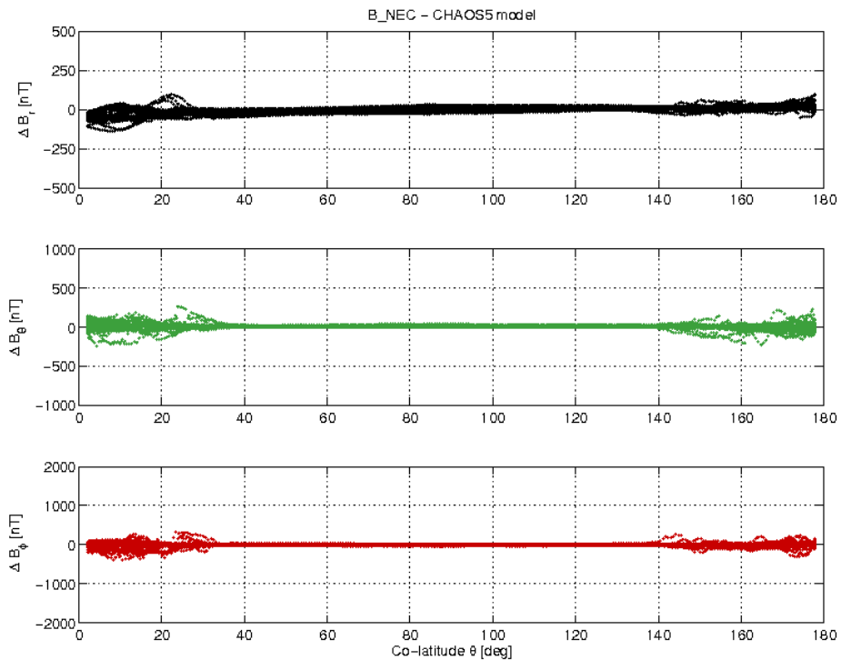
Figure 19: S/C B day 04/07 B_{NEC} - B_{Chaos} difference vs colatitude.
