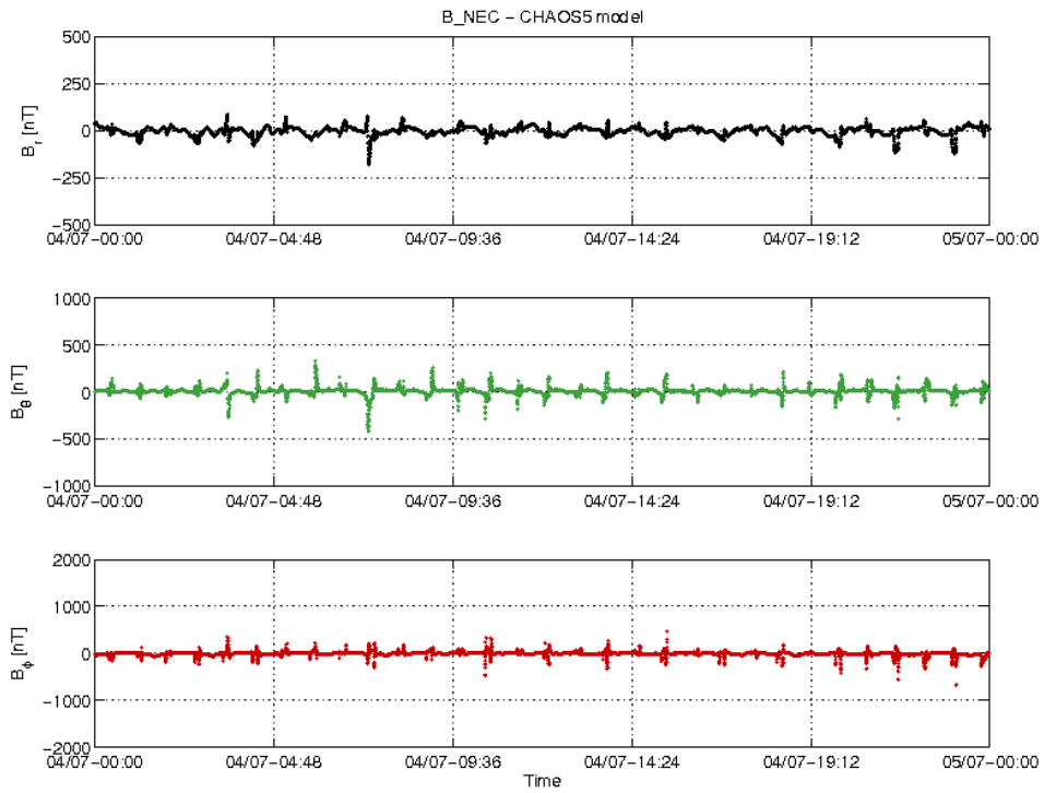
Figure 18: S/C A day 04/07: time series of B_{NEC} - B_{Chaos} residuals.
