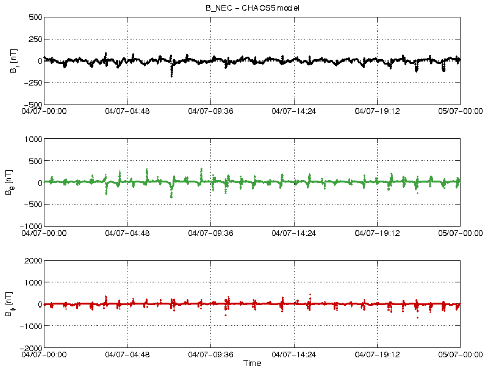
Figure 22: S/C C day 04/07 time series of B_{NEC} - B_{Chaos} residuals.
