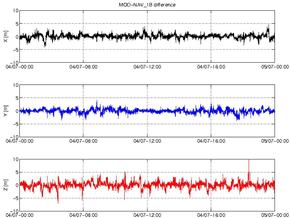
Figure 5: Difference MOD-GPSNAV, S/C C, 04/07. From top to bottom: X, Y and Z-axis
