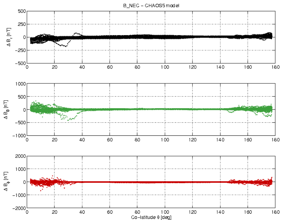
Figure 17: S/C A day 04/07 B_{NEC} - B_{Chaos} vs colatitude.
