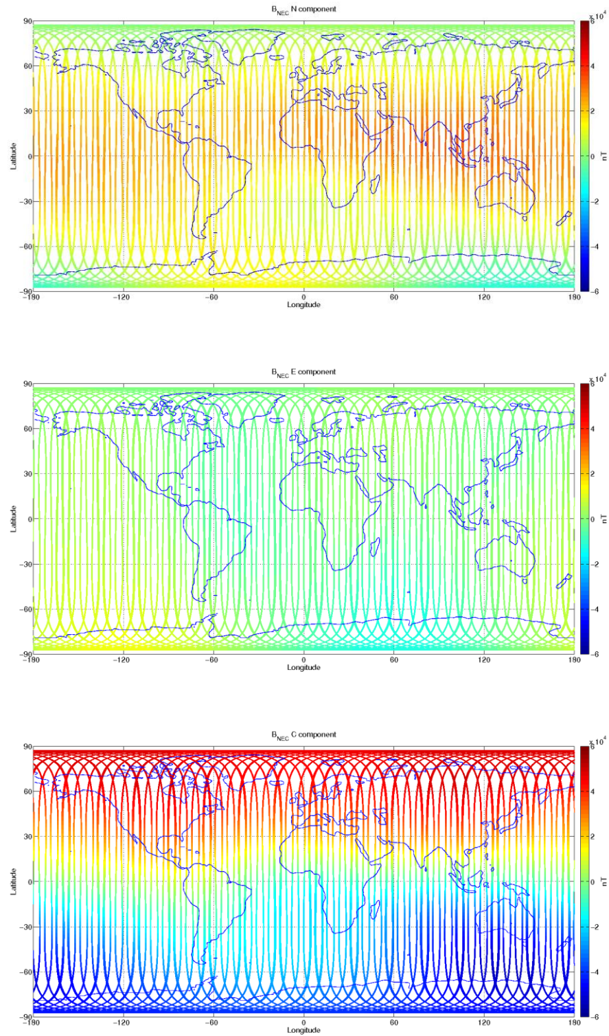
Figure 12: S/C C, world map plots of the geomagnetic field and components measured during monitoring period 04/07-10/07. From top to bottom: B NEC components (North, East, and Centre) of magnetic field from VFM measurement.
