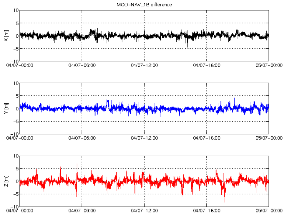
Figure 4: Difference MOD-GPSNAV, S/C B, 04/07. From top to bottom: X, Y and Z-axis
