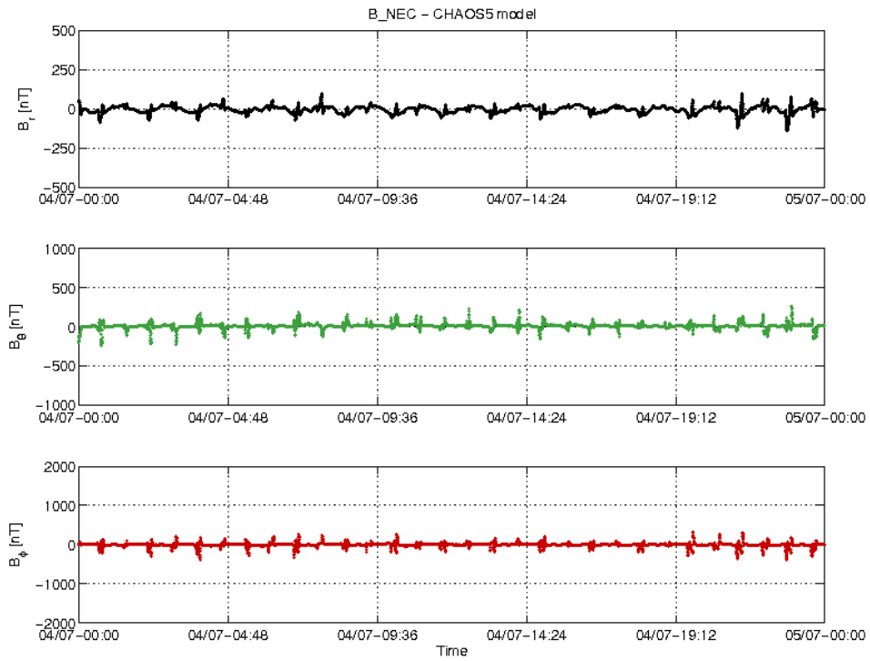
Figure 20: S/C B day 04/07 time series of B_{NEC} - B_{Chaos} residuals.
