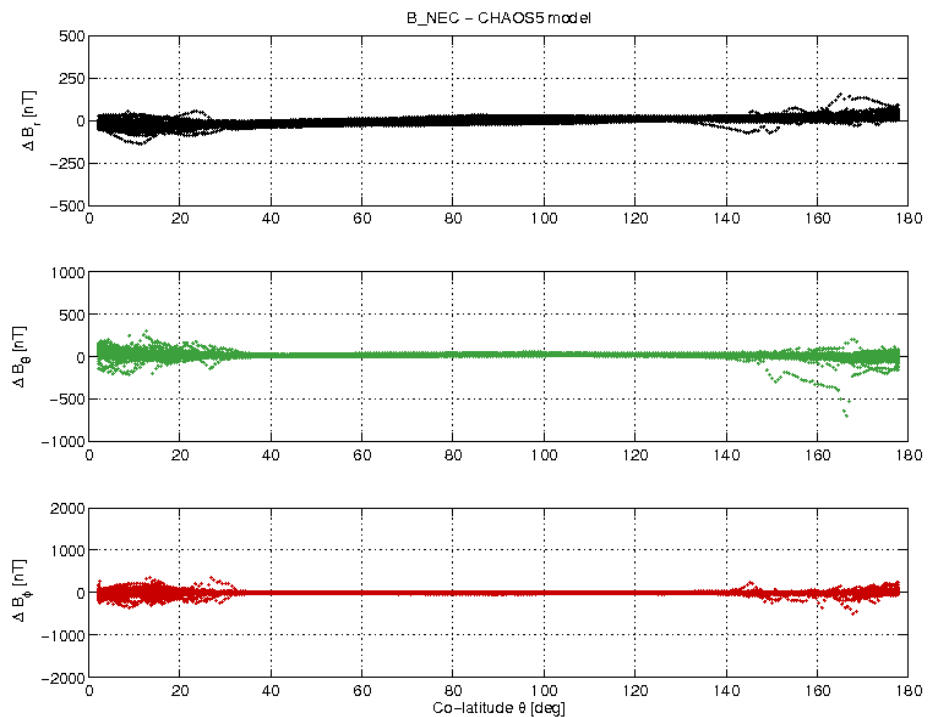
Figure 19: S/C B day 27/06 B_{NEC} - B_{Chaos} difference vs colatitude.
