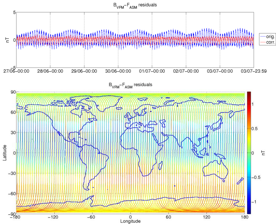
Figure 9: ASM-VFM residuals for S/C B, during monitoring period 27/06-03/07. In top figure are plotted: difference between |B_{VFM}| and F_{ASM} (without dB_Sun correction) (blue colour), and the residuals with dB_Sun corrections (red colour). In bottom figure residuals are presented on the world map.
