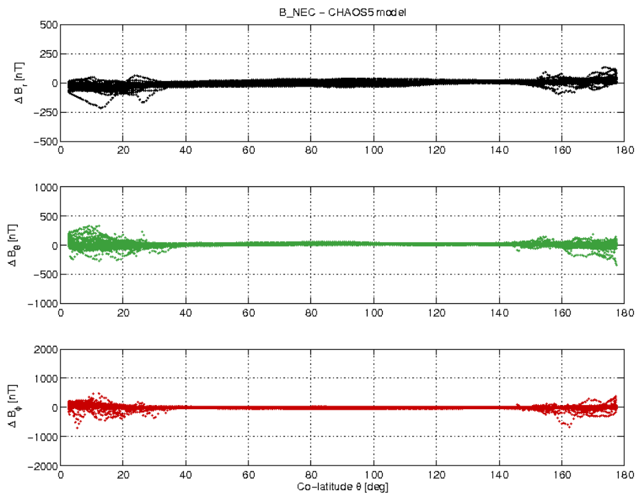
Figure 21: S/C C day 27/06 B_{NEC} - B_{Chaos} difference vs colatitude.
