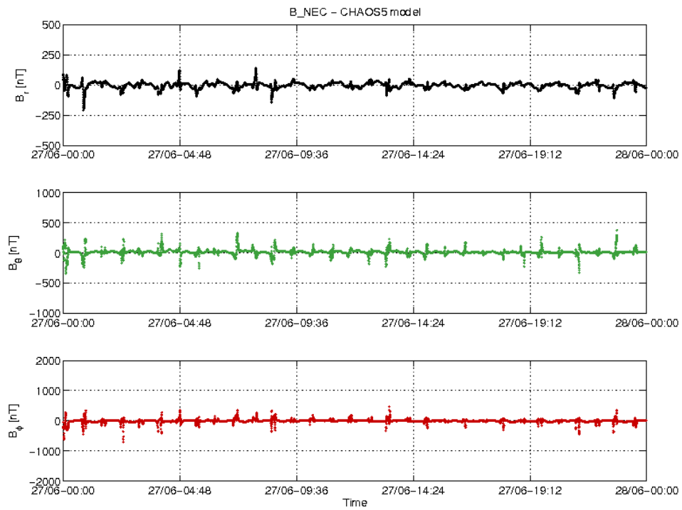
Figure 18: S/C A day 27/06: time series of B_{NEC} - B_{Chaos} residuals.
