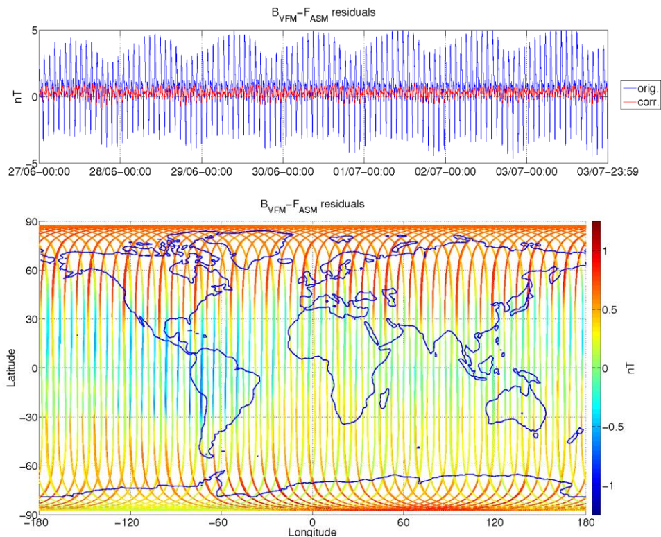
Figure 8: ASM-VFM residuals for S/C A, during monitoring period 27/06-03/07. In top figure are plotted: difference between |B_{VFM}| and F_{ASM} (without dB_Sun correction) (blue colour), and the residuals with dB_Sun corrections (red colour). In bottom figure residuals are presented on the world map.
