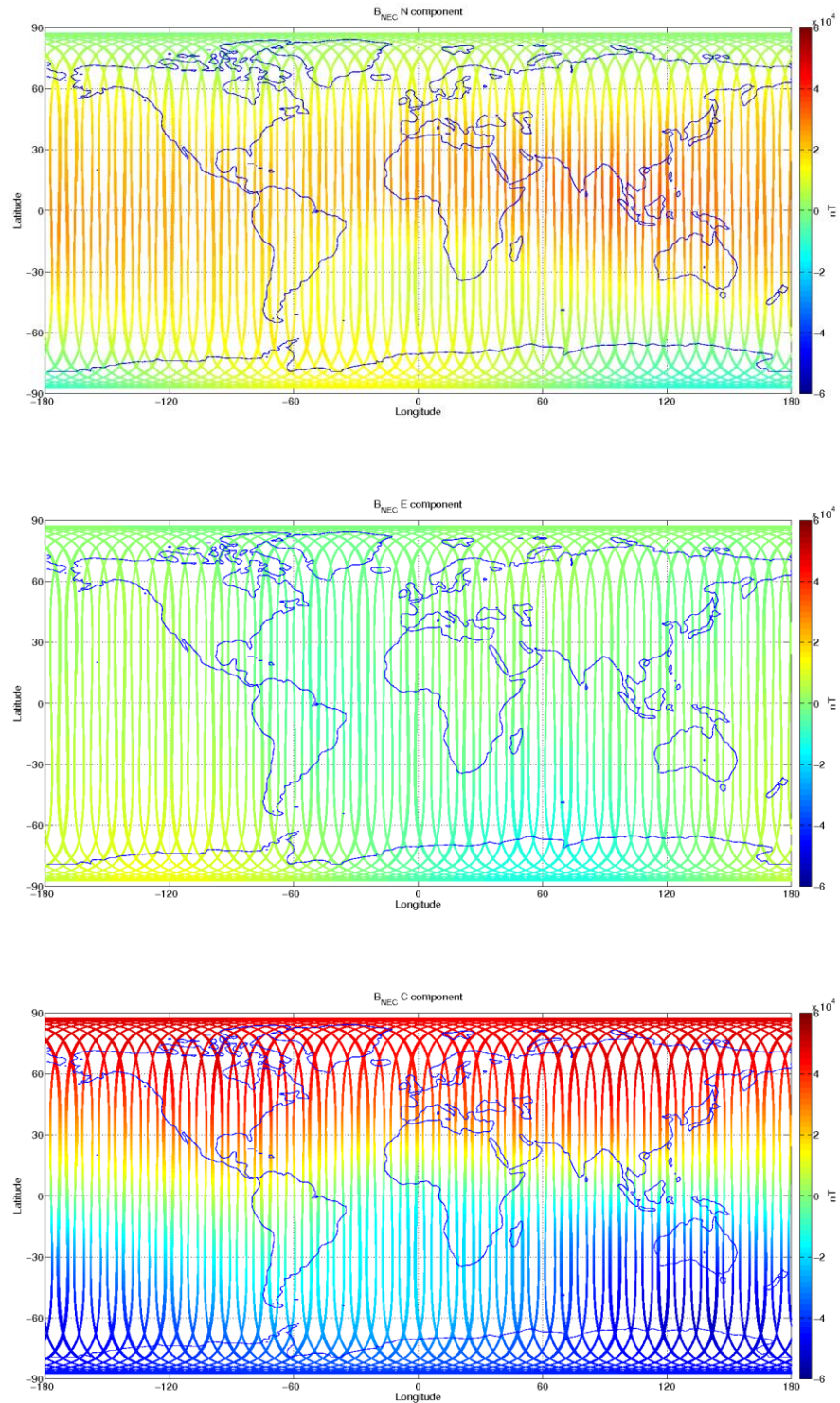
Figure 12: S/C C, world map plots of the geomagnetic field and components measured during monitoring period 27/06-03/07. From top to bottom: B NEC components (North, East, and Centre) of magnetic field from VFM measurement.
