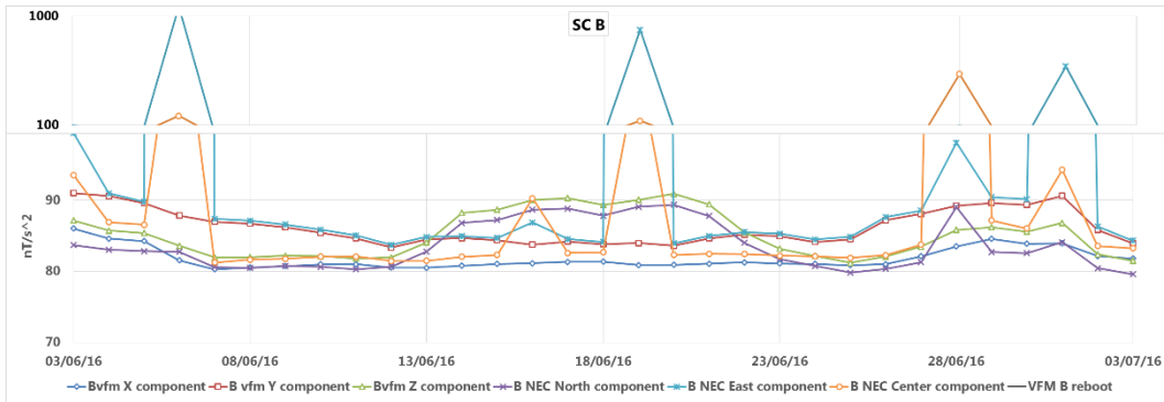
Figure 24: Plot of standard deviation of B components in VFM and NEC frames. Please note the mixed (linear + logarithmic) vertical axis (in range 100-1000 is given in logarithmic scale).
