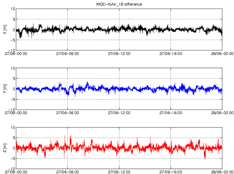
Figure 5: Difference MOD-GPSNAV, S/C C, 27/06. From top to bottom: X, Y and Z-axis
