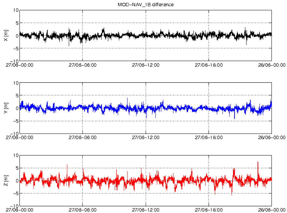
Figure 4: Difference MOD-GPSNAV, S/C B, 27/06. From top to bottom: X, Y and Z-axis
