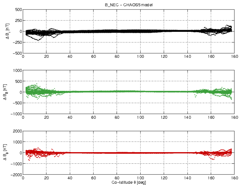
Figure 17: S/C A day 27/06 B_{NEC} - B_{Chaos} vs colatitude.
