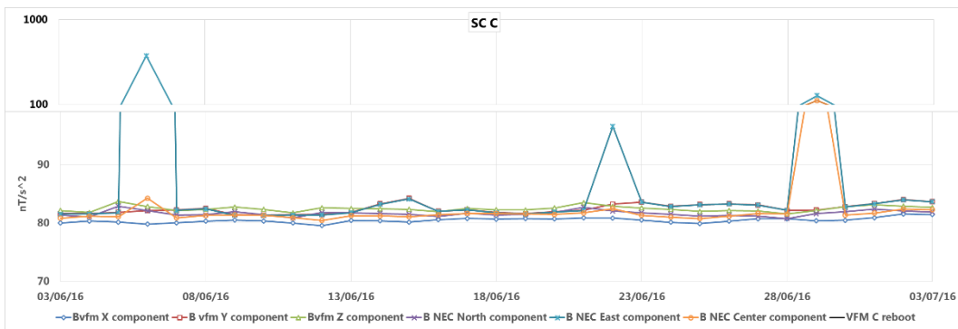
Figure 25: Plot of standard deviation of B components in VFM and NEC frames. Please note the mixed (linear + logarithmic) vertical axis (in range 100-1000 is given in logarithmic scale).
