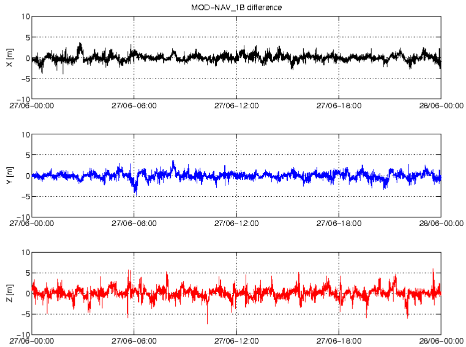
Figure 3: Difference MOD-GPSNAV, S/C A, 27/06. From top to bottom: X, Y and Z-axis
