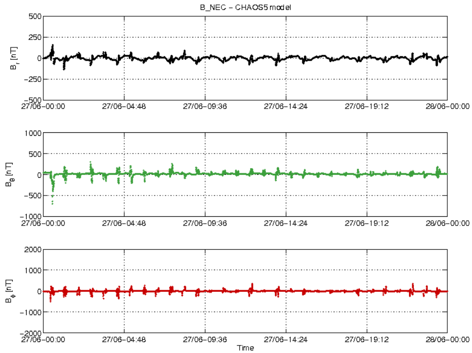
Figure 20: S/C B day 27/06 time series of B_{NEC} - B_{Chaos} residuals.
