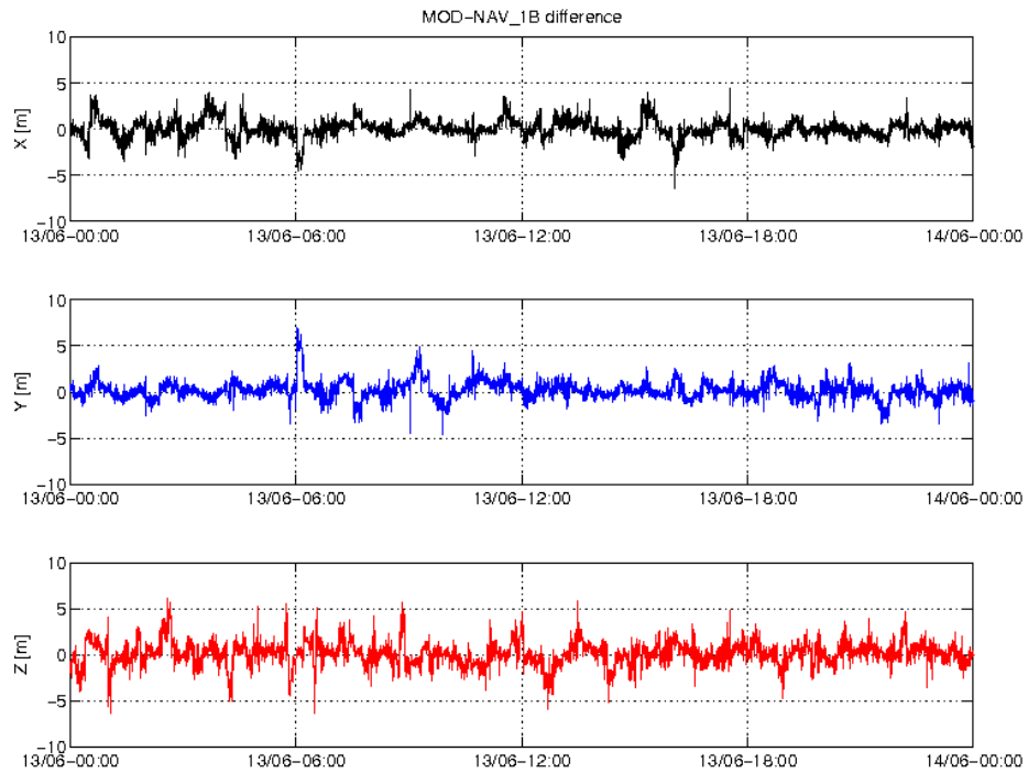
Figure 3: Difference MOD-GPSNAV, S/C A, 13/06. From top to bottom: X, Y and Z-axis
