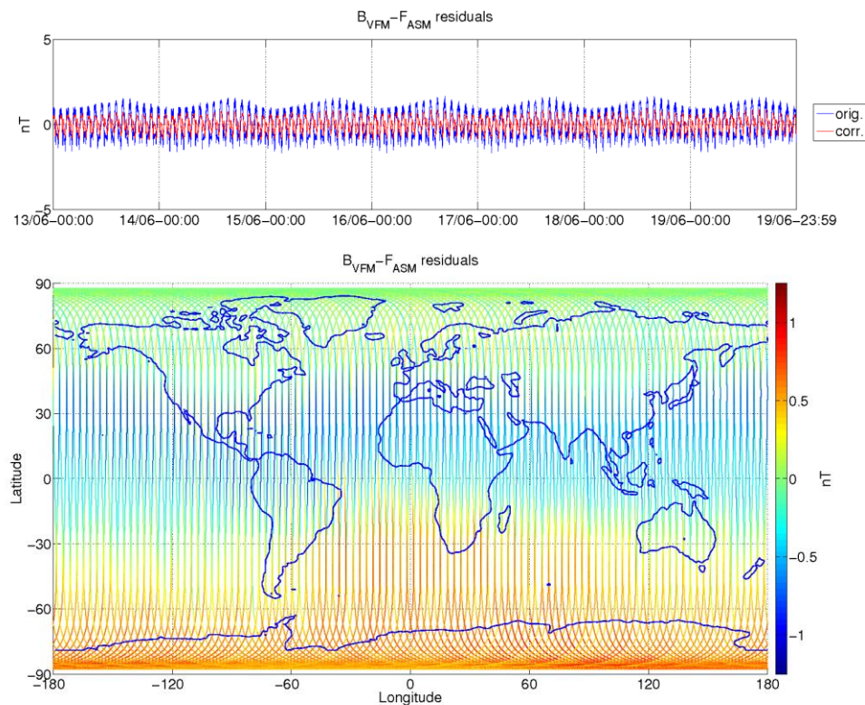
Figure 9: ASM-VFM residuals for S/C B, during monitoring period 13/06-19/06. In top figure are plotted: difference between |B_{VFM}| and F_{ASM} (without dB Sun correction) (blue colour), and the residuals with dB Sun corrections (red colour). In bottom figure residuals are presented on the world map.
