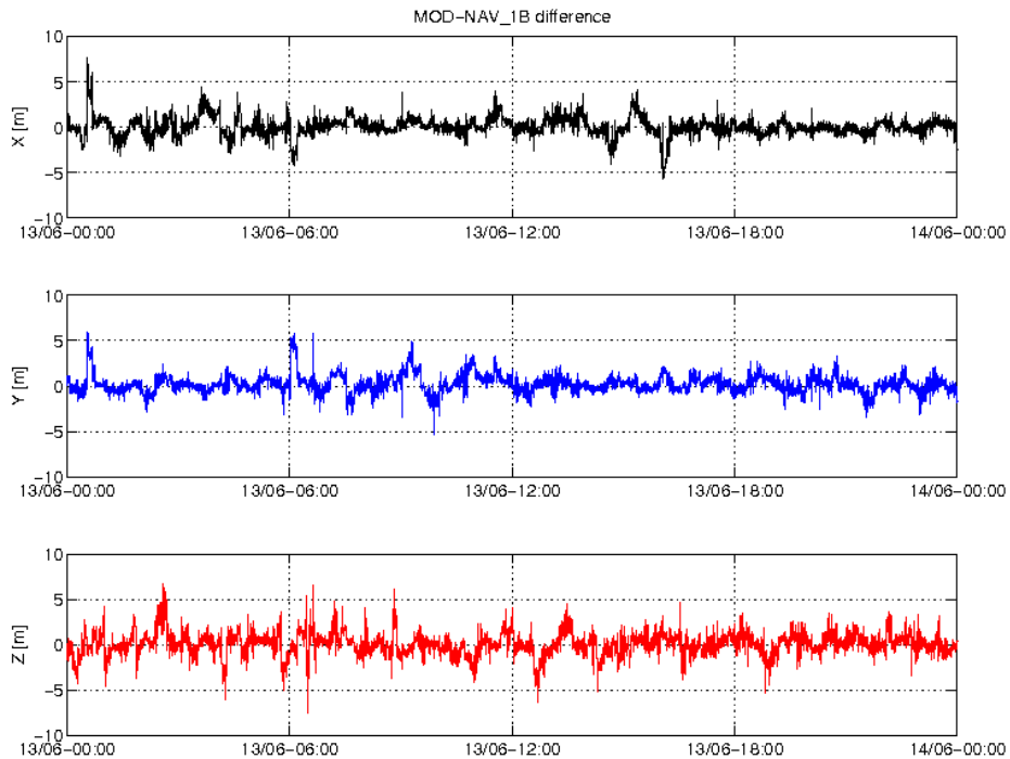
Figure 5: Difference MOD-GPSNAV, S/C C, 13/06. From top to bottom: X, Y and Z-axis
