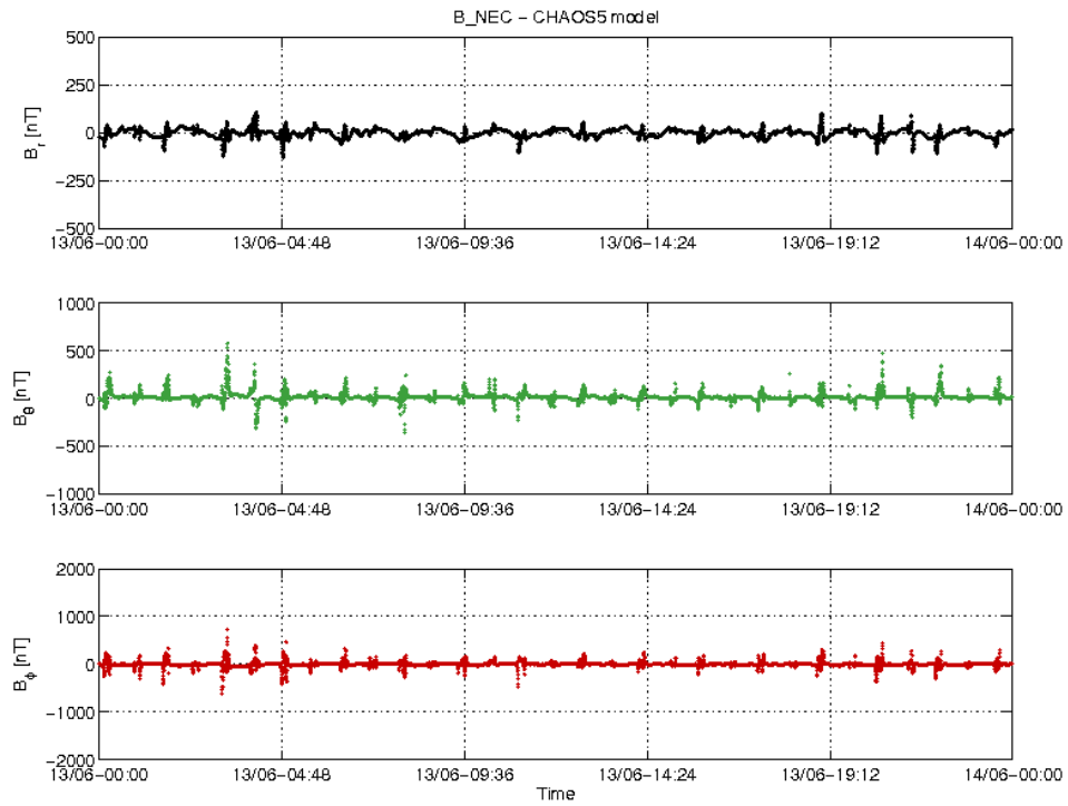
Figure 18: S/C A day 13/06: time series of B_{NEC} - B_{Chaos} residuals.
