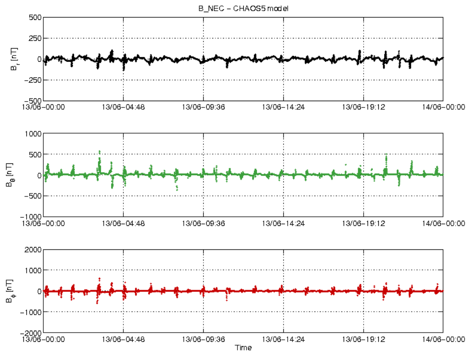
Figure 22: S/C C day 13/06 time series of B_{NEC} - B_{Chaos} residuals.
