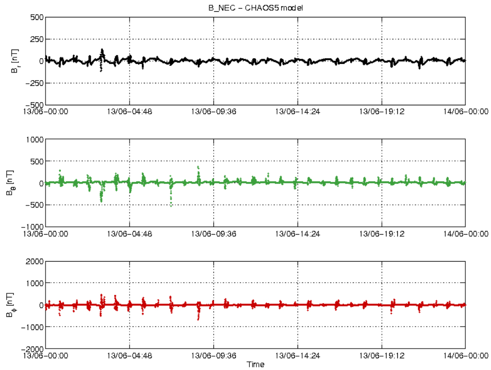
Figure 20: S/C B day 13/06 time series of B_{NEC} - B_{Chaos} residuals.
