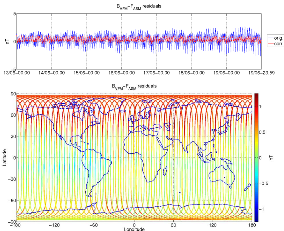
Figure 8: ASM-VFM residuals for S/C A, during monitoring period 13/06-19/06. In top figure are plotted: difference between |B_{VFM}| and F_{ASM} (without dB_{Sun} correction) (blue colour), and the residuals with dB_{Sun} corrections (red colour). In bottom figure residuals are presented on the world map.
