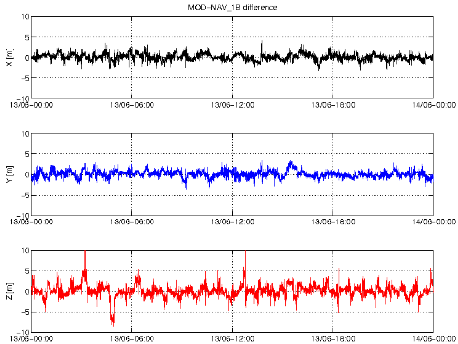
Figure 4: Difference MOD-GPSNAV, S/C B, 13/06. From top to bottom: X, Y and Z-axis
