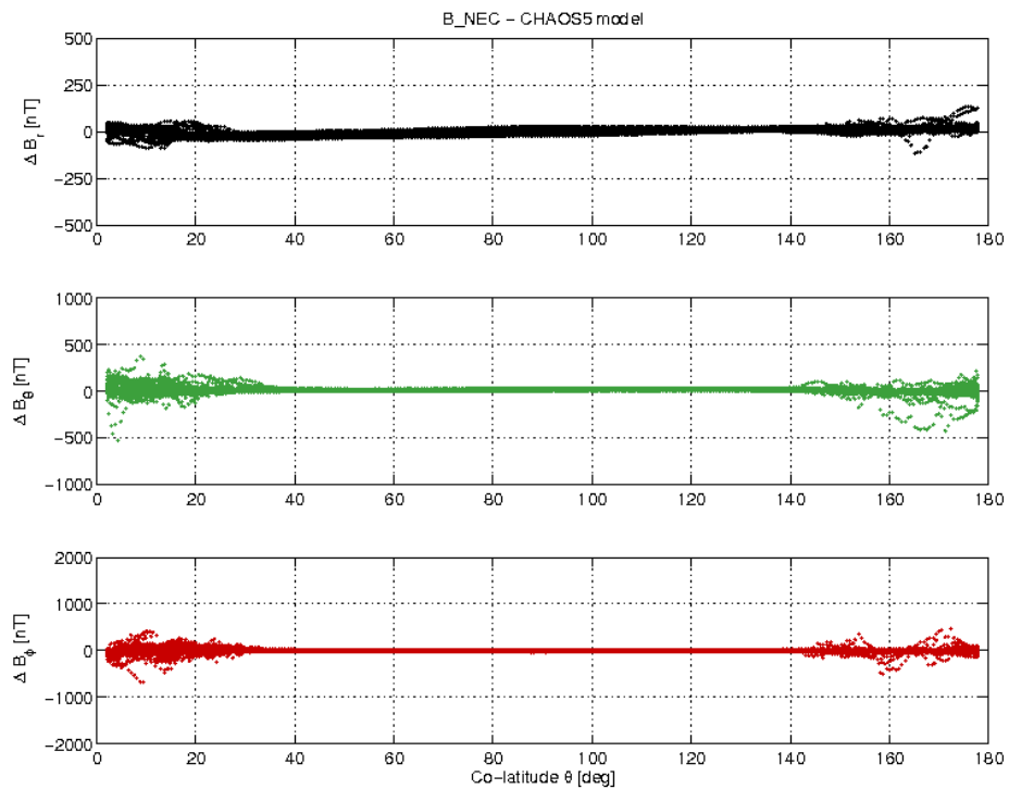
Figure 19: S/C B day 13/06 B_{NEC} - B_{Chaos} difference vs colatitude.
