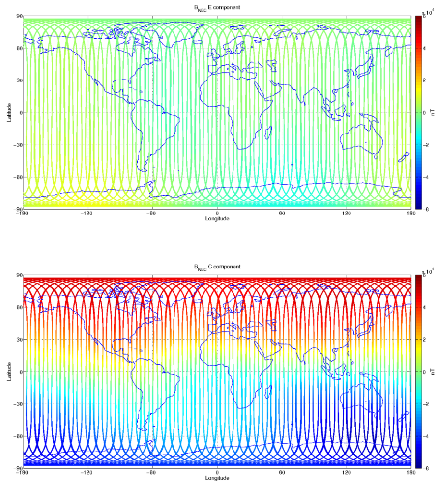
Figure 10: S/C A, world map plots of the geomagnetic field and components measured during monitoring period 13/06-19/06. From top to bottom: F-magnetic field from ASM measurement, B_{NEC} components (North, East, and Centre) of magnetic field from VFM measurement.
