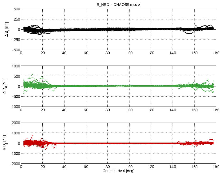
Figure 17: S/C A day 13/06 B_{NEC} - B_{Chaos} vs colatitude.
