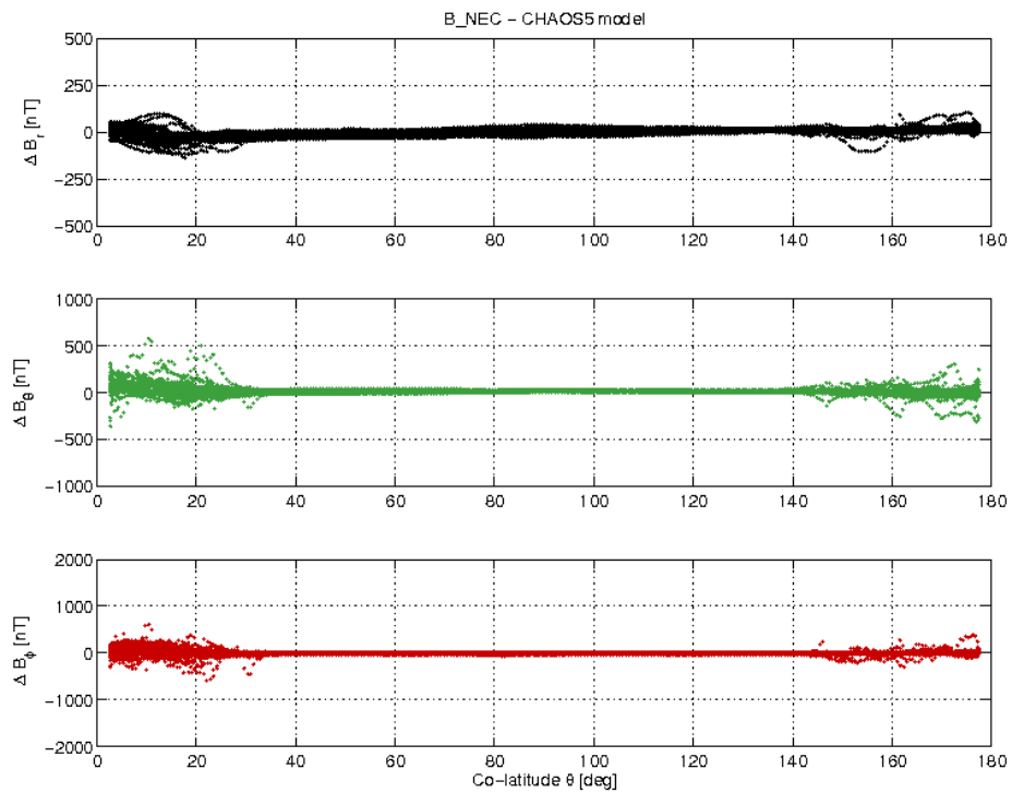
Figure 21: S/C C day 13/06 B_{NEC} - B_{Chaos} difference vs colatitude.
