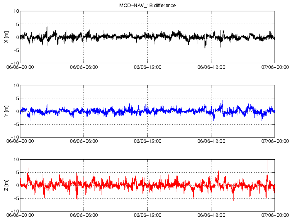
Figure 5: Difference MOD-GPSNAV, S/C C, 06/06. From top to bottom: X, Y and Z-axis
