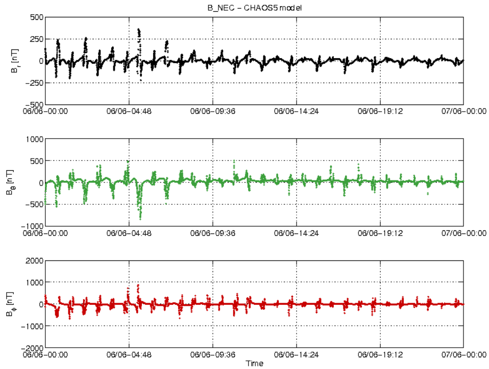
Figure 20: S/C B day 06/06 time series of B_{NEC} - B_{Chaos} residuals.
