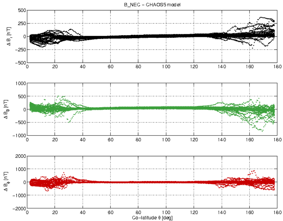
Figure 19: S/C B day 06/06 B_{NEC} - B_{Chaos} difference vs colatitude.
