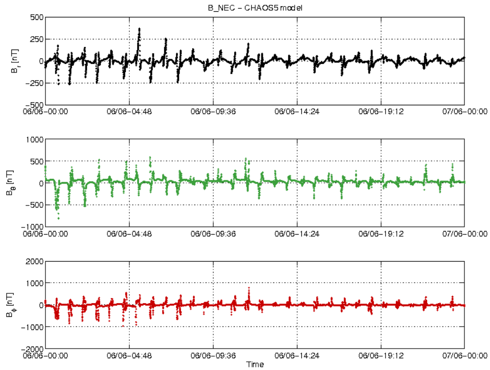
Figure 18: S/C A day 06/06: time series of B_{NEC} - B_{Chaos} residuals.
