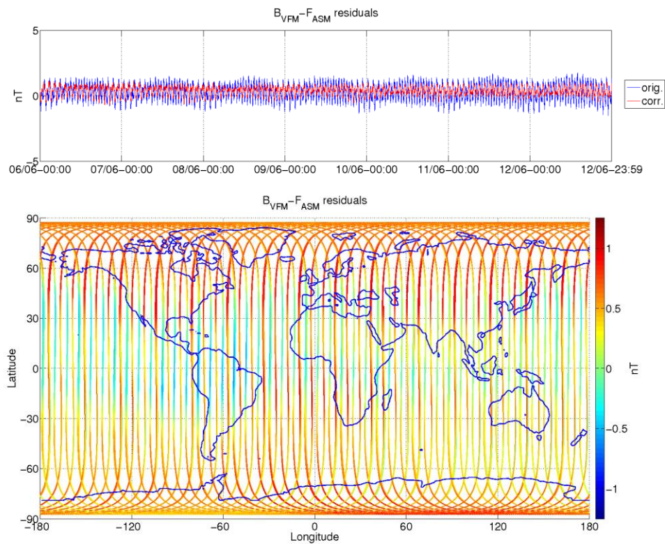
Figure 8: ASM-VFM residuals for S/C A, during monitoring period 06/06-12/06. In top figure are plotted: difference between |B_{VFM}| and F_{ASM} (without dB Sun correction) (blue colour), and the residuals with dB Sun corrections (red colour). In bottom figure residuals are presented on the world map.
