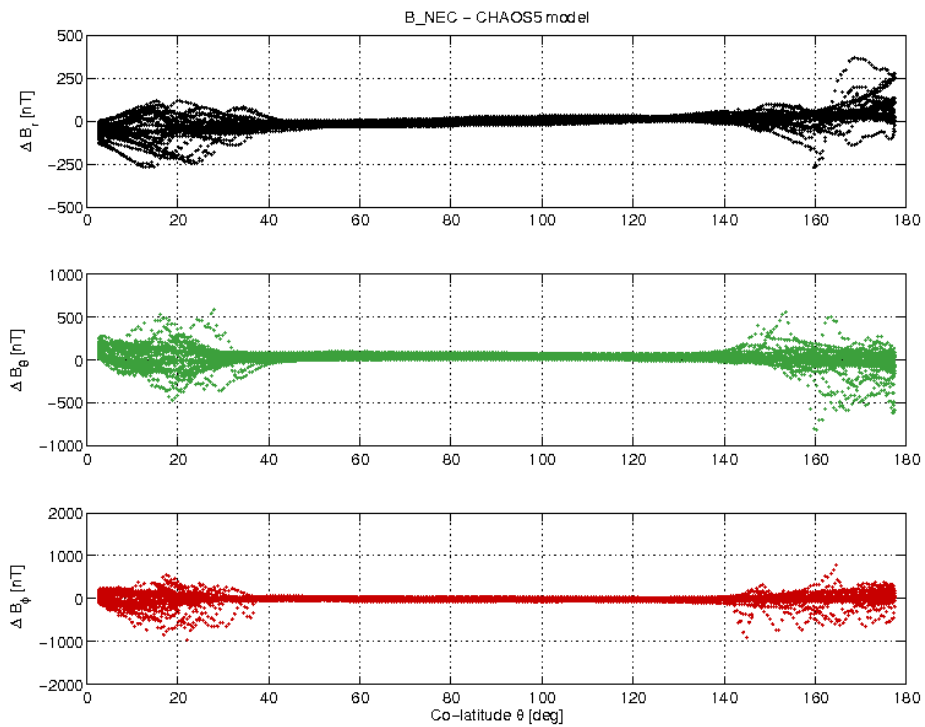
Figure 17: S/C A day 06/06 B_{NEC} - B_{Chaos} vs colatitude.
