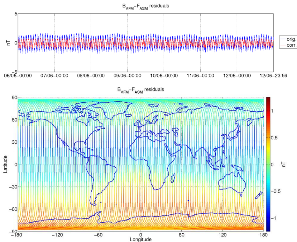
Figure 9: ASM-VFM residuals for S/C B, during monitoring period 06/06-12/06. In top figure are plotted: difference between |B_{VFM}| and F_{ASM} (without dB_{Sun} correction) (blue colour), and the residuals with dB_{Sun} corrections (red colour). In bottom figure residuals are presented on the world map.
