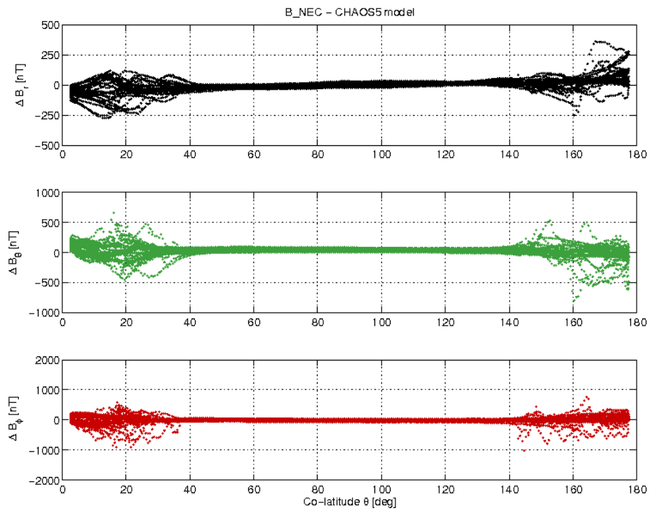
Figure 21: S/C C day 06/06 B_{NEC} - B_{Chaos} difference vs colatitude.
