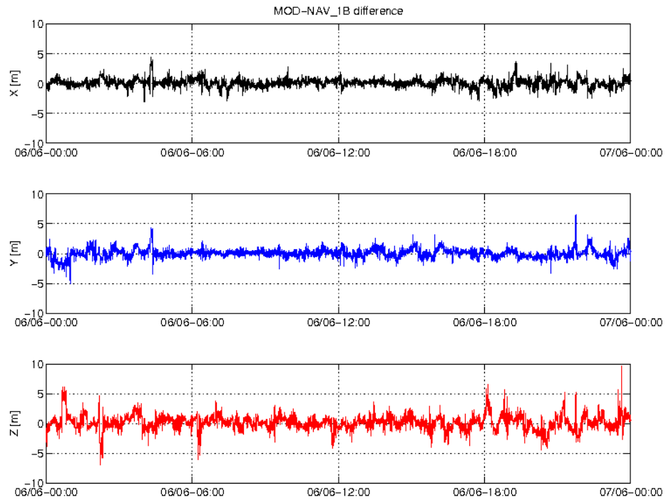
Figure 4: Difference MOD-GPSNAV, S/C B, 06/06. From top to bottom: X, Y and Z-axis
