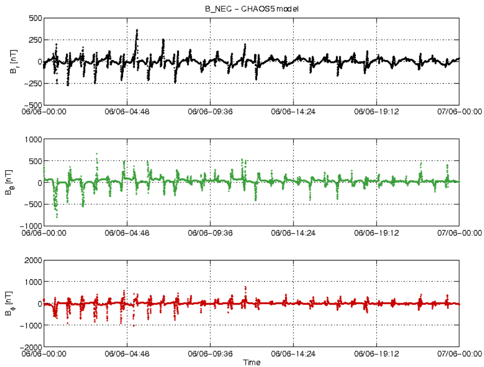
Figure 22: S/C C day 06/06 time series of B_{NEC} - B_{Chaos} residuals.
