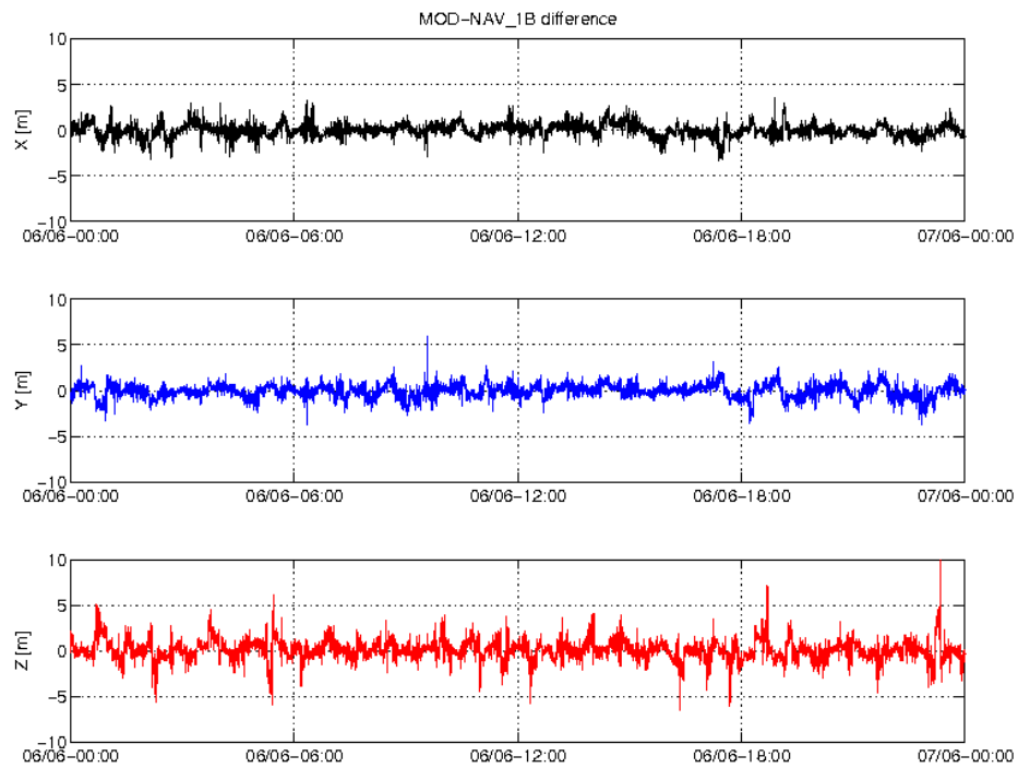
Figure 3: Difference MOD-GPSNAV, S/C A, 06/06. From top to bottom: X, Y and Z-axis
