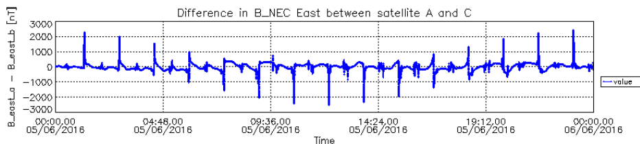
Figure 17: Difference in B NEC East component between S/C A and S/C C.
