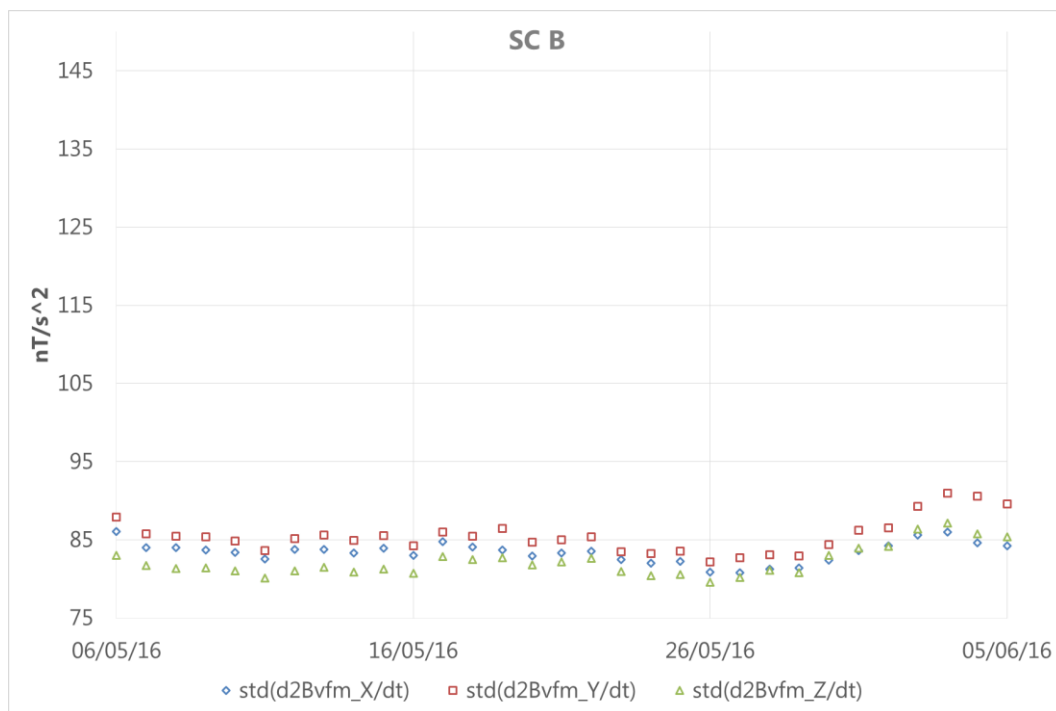
Figure 26: Plot of standard deviation of B components in VFM frames.
