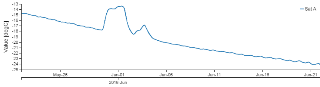
Figure 10: T_CDC temperature of SC A with visible impact of the temperature test.
