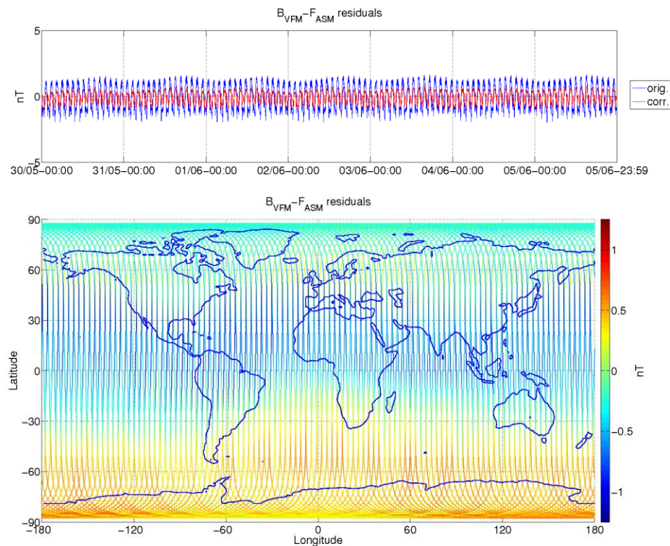
Figure 9: ASM-VFM residuals for S/C B, during monitoring period 30/05-05/06. In top figure are plotted: difference between |B VFM | and F ASM (without dB Sun correction) (blue colour), and the residuals with dB Sun corrections (red colour). In bottom figure residuals are presented on the world map.
