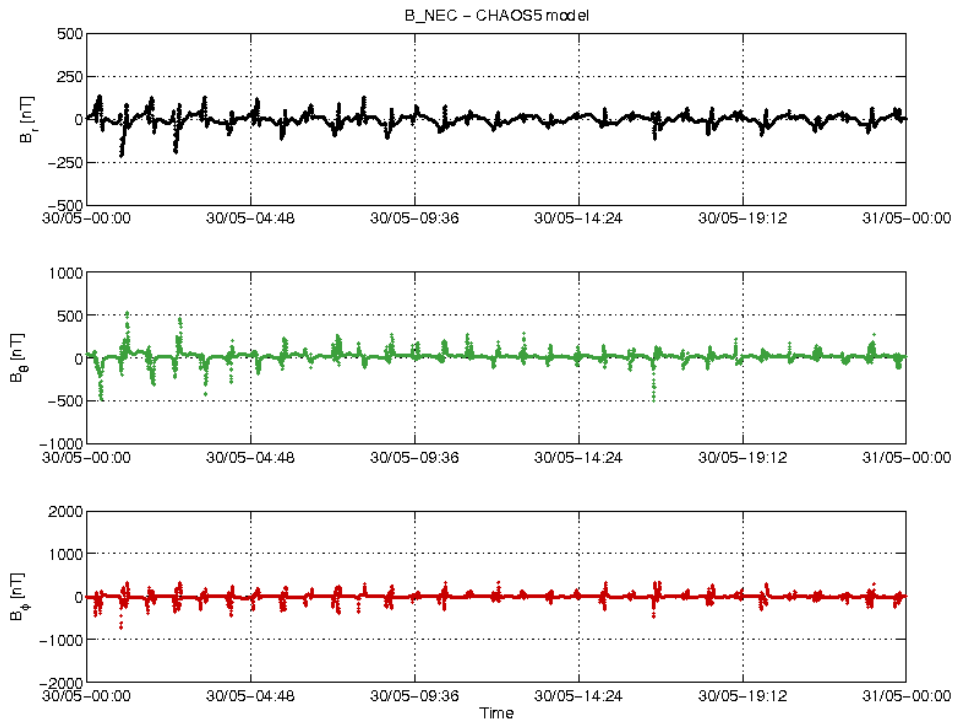
Figure 20: S/C A day 30/05: time series of B_{NEC} - B_{Chaos} residuals.
