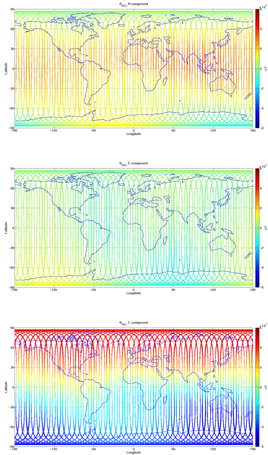
Figure 14: S/C C, world map plots of the geomagnetic field and components measured during monitoring period 30/05-05/06. From top to bottom: B_{NEC} components (North, East, and Centre) of magnetic field from VFM measurement.
