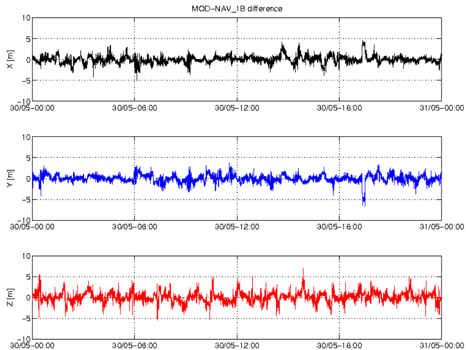
Figure 3: Difference MOD-GPSNAV, S/C A, 30/05. From top to bottom: X, Y and Z-axis.
