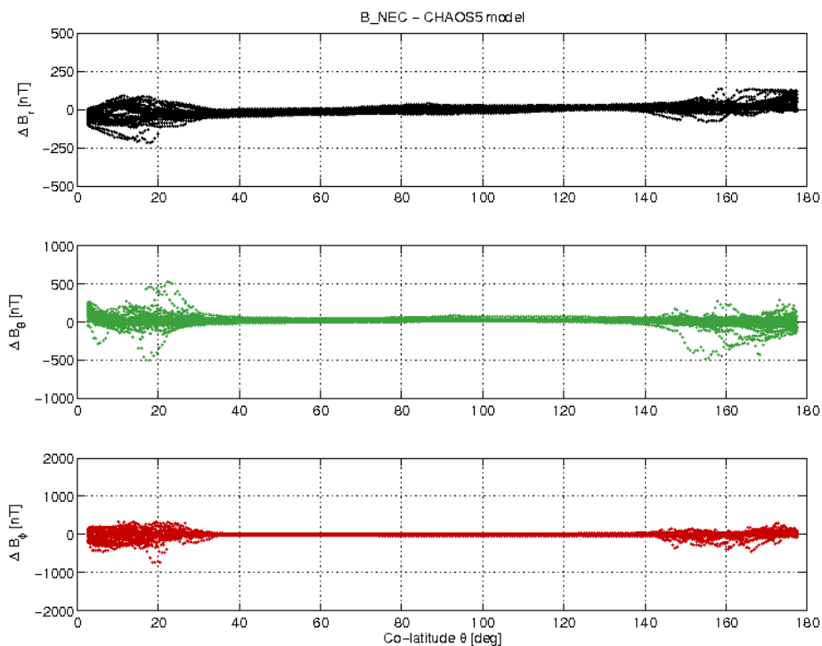
Figure 19: S/C A day 30/05 B_{NEC} - B_{Chaos} vs colatitude.
