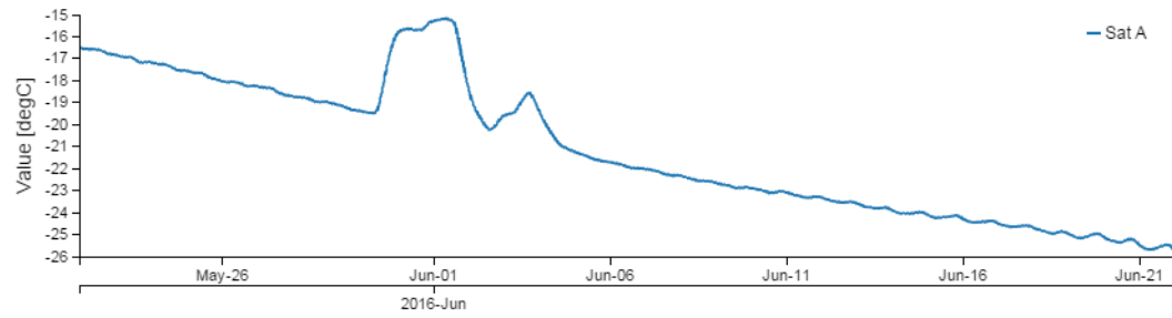
Figure 11: T_CDC temperature of SC A with visible impact of the temperature test.
