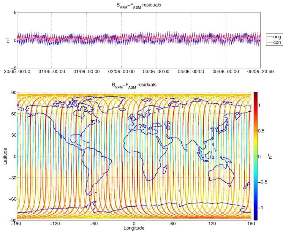
Figure 8: ASM-VFM residuals for S/C A, during monitoring period 30/05-05/06. In top figure are plotted: difference between |B_{VFM}| and F_{ASM} (without dB Sun correction) (blue colour), and the residuals with dB Sun corrections (red colour). In bottom figure residuals are presented on the world map.
