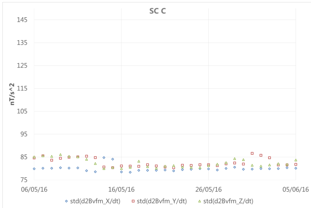
Figure 27: Plot of standard deviation of B components in VFM frames.
