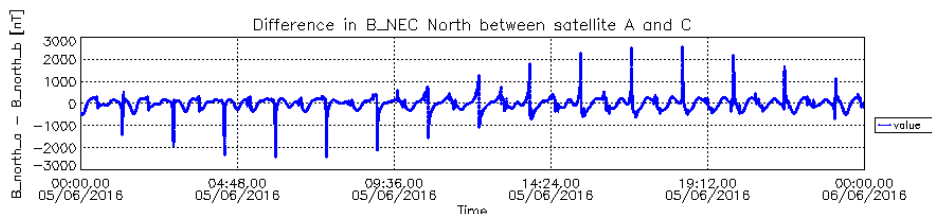
Figure 16: Difference in B NEC North component between S/C A and S/C C.
