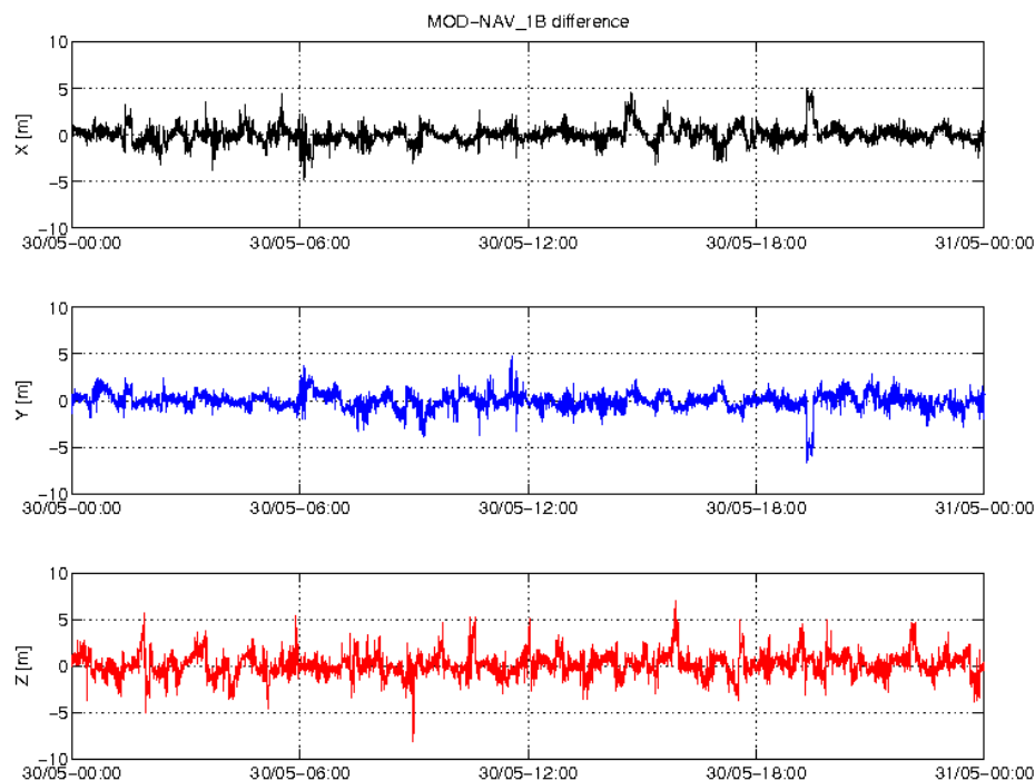
Figure 5: Difference MOD-GPSNAV, S/C C, 30/05. From top to bottom: X, Y and Z-axis.
