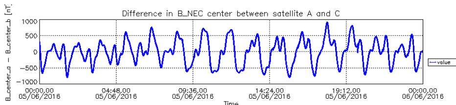
Figure 18: Difference in B NEC Center component between S/C A and S/C C.
