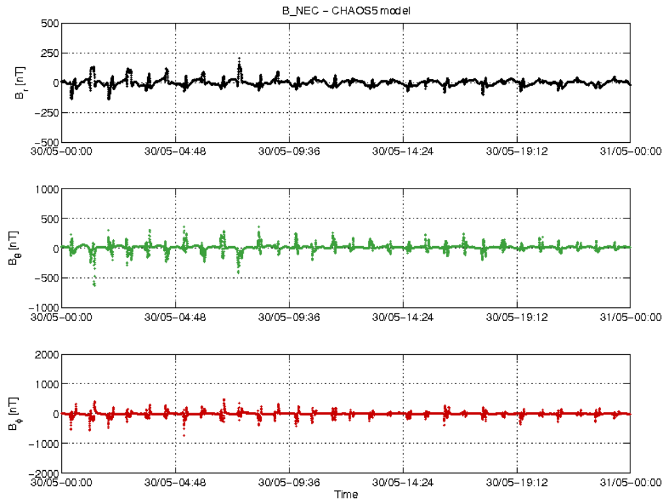
Figure 22: S/C B day 30/05 time series of B_{NEC} - B_{Chaos} residuals.
