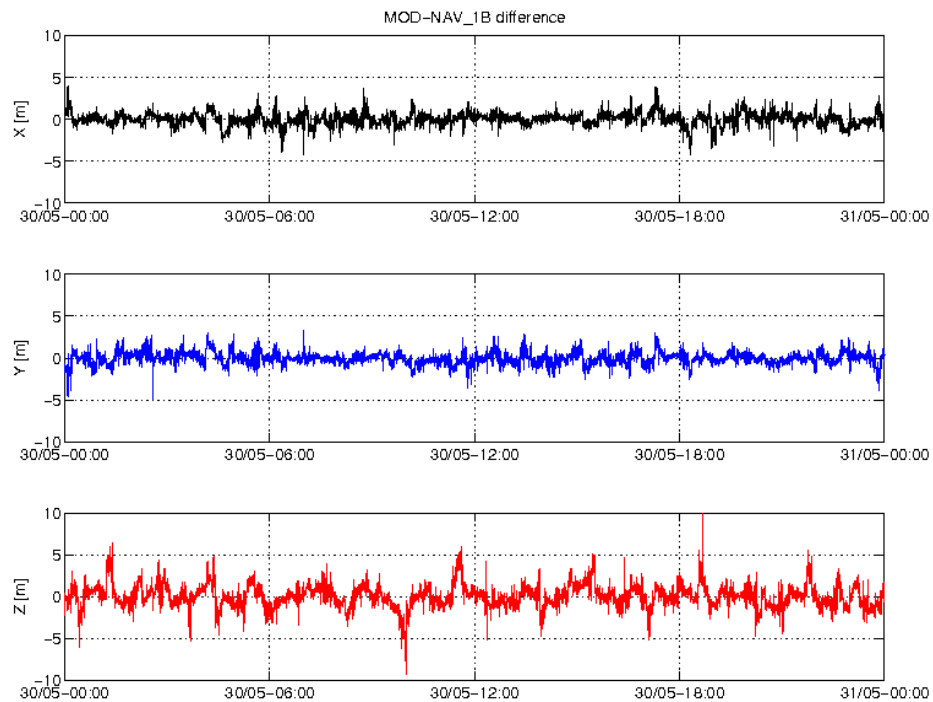
Figure 4: Difference MOD-GPSNAV, S/C B, 30/05. From top to bottom: X, Y and Z-axis.
