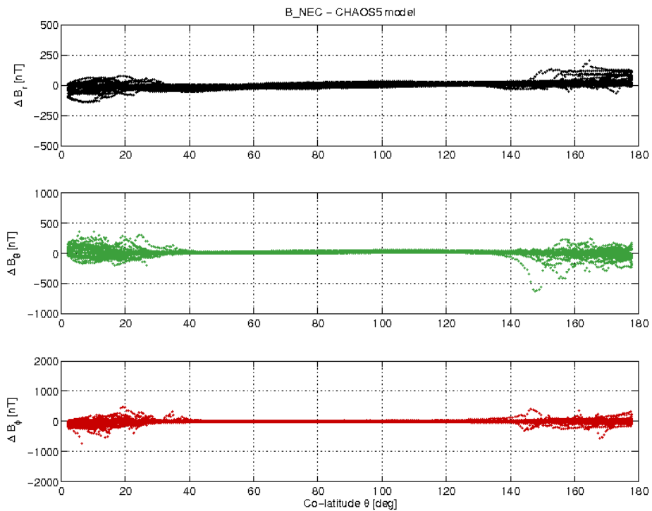
Figure 21: S/C B day 30/05 B_{NEC} - B_{Chaos} difference vs colatitude.
