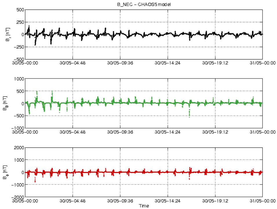
Figure 24: S/C C day 30/05 time series of B_{NEC} - B_{Chaos} residuals.
