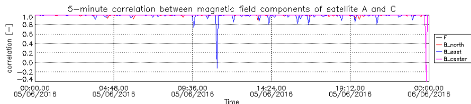
Figure 15: Correlation in magnetic data between satellite A and C for B north , B east , and B center components of B NEC are the components of the magnetic field vector in NEC frame
