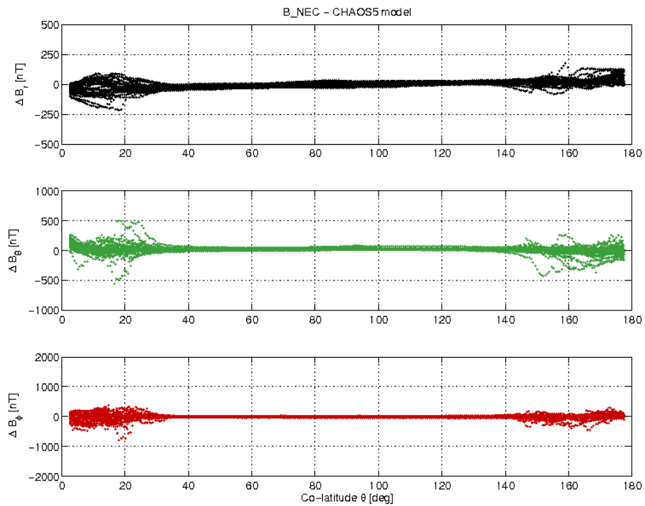
Figure 23: S/C C day 30/05 B_{NEC} - B_{Chaos} difference vs colatitude.
