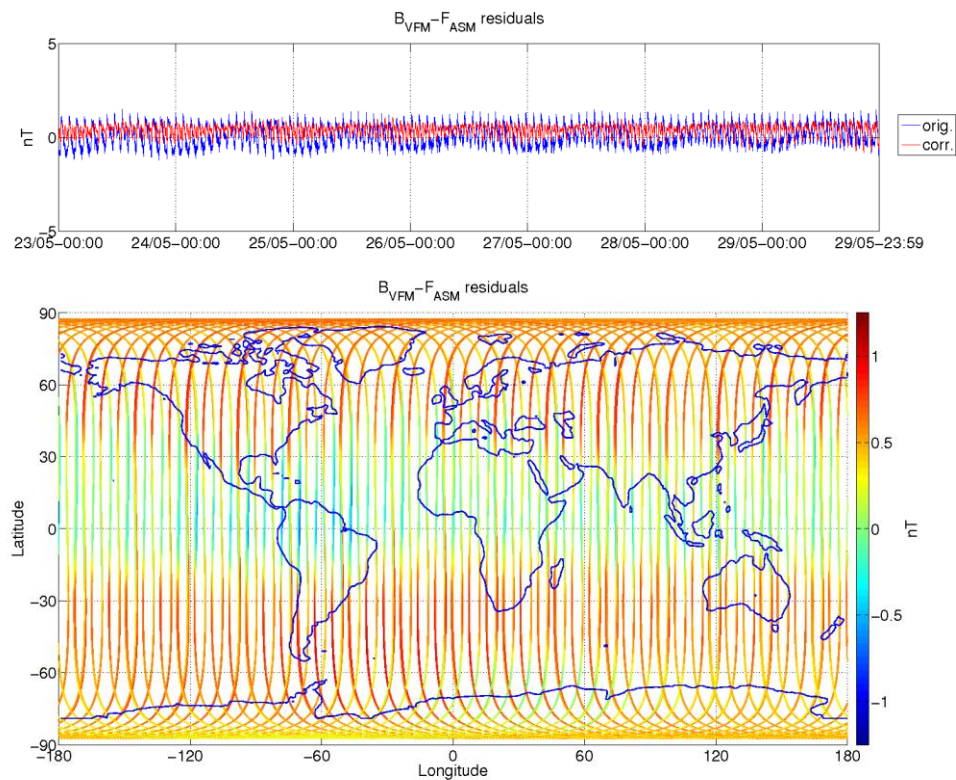
Figure 8: ASM-VFM residuals for S/C A, during monitoring period 23/05-29/05. In top figure are plotted: difference between |B_{VFM}| and F_{ASM} (without dB Sun correction) (blue colour), and the residuals with dB Sun corrections (red colour). In bottom figure residuals are presented on the world map.
