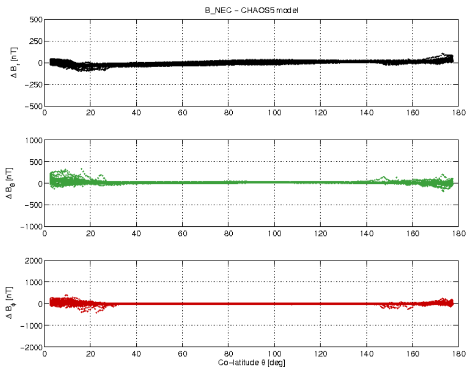
Figure 17: S/C A day 23/05 B_{NEC} - B_{Chaos} vs colatitude.
