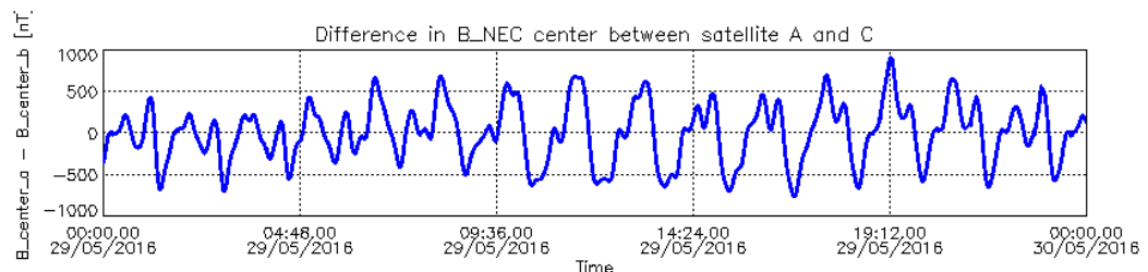
Figure 16 Difference in B_NEC Center component between S/C A and S/C C on 29/05/2016.
