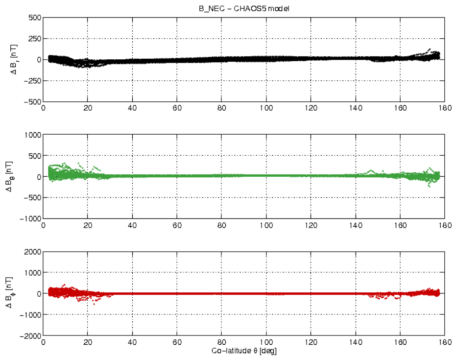
Figure 21 S/C C day 23/05 B_{NEC} - B_{Chaos} difference vs colatitude.
