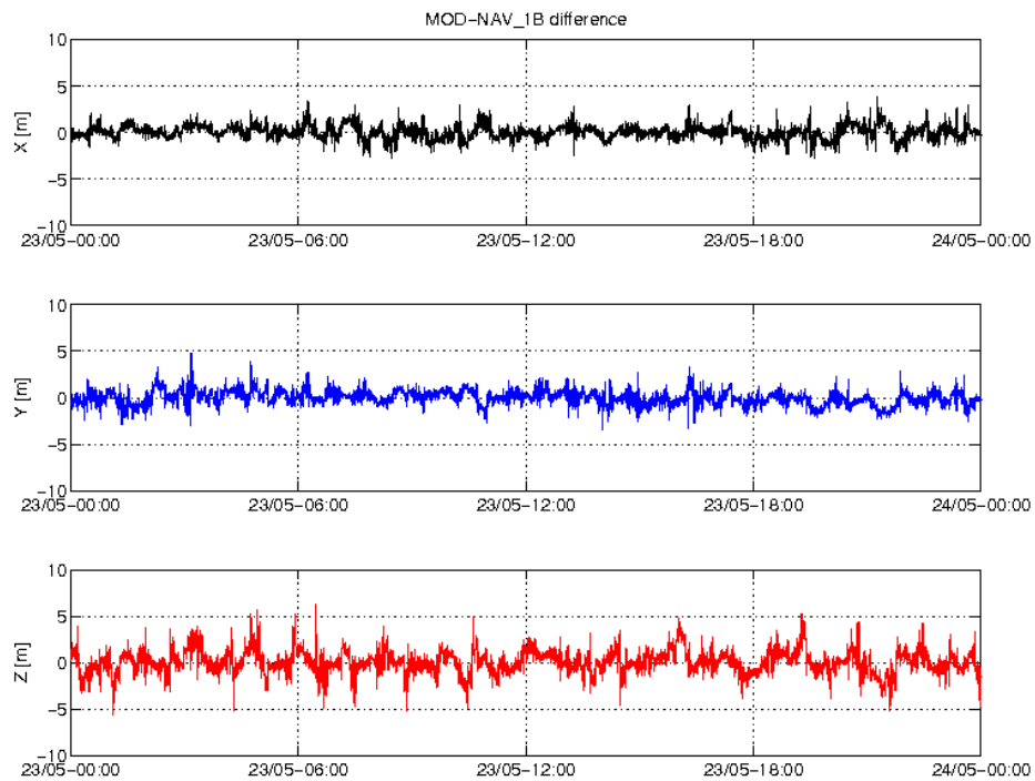
Figure 4: Difference MOD-GPSNAV, S/C B, 23/05. From top to bottom: X, Y and Z-axis
