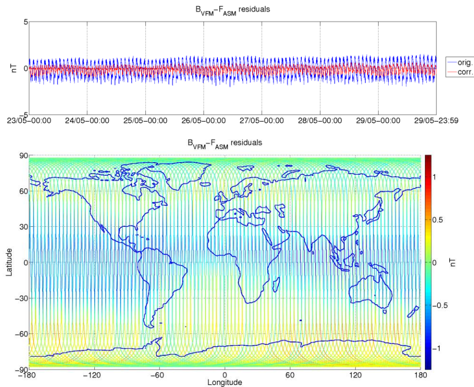
Figure 9: ASM-VFM residuals for S/C B, during monitoring period 23/05-29/05. In top figure are plotted: difference between |B_{VFM}| and F_{ASM} (without dB_{Sun} correction) (blue colour), and the residuals with dB_{Sun} corrections (red colour). In bottom figure residuals are presented on the world map.
