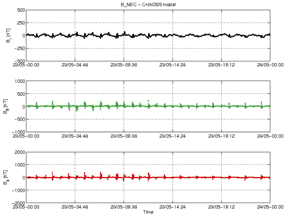
Figure 20 S/C B day 23/05 time series of B_{NEC} - B_{Chaos} residuals.
