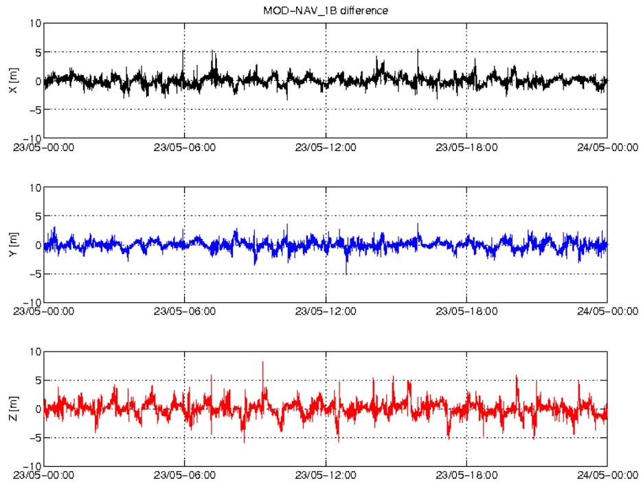
Figure 3: Difference MOD-GPSNAV, S/C A, 23/05. From top to bottom: X, Y and Z-axis
