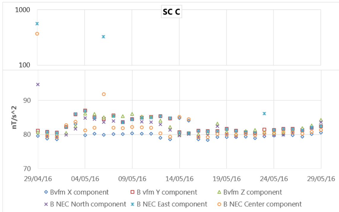
Figure 25: Plot of standard deviation of B components in VFM and NEC frames. Please note the mixed (linear + logarithmic) vertical axis (in range 100-1000 is given in logarithmic scale).
