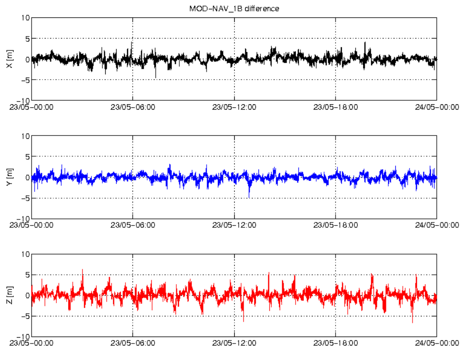
Figure 5: Difference MOD-GPSNAV, S/C C, 23/05. From top to bottom: X, Y and Z-axis
