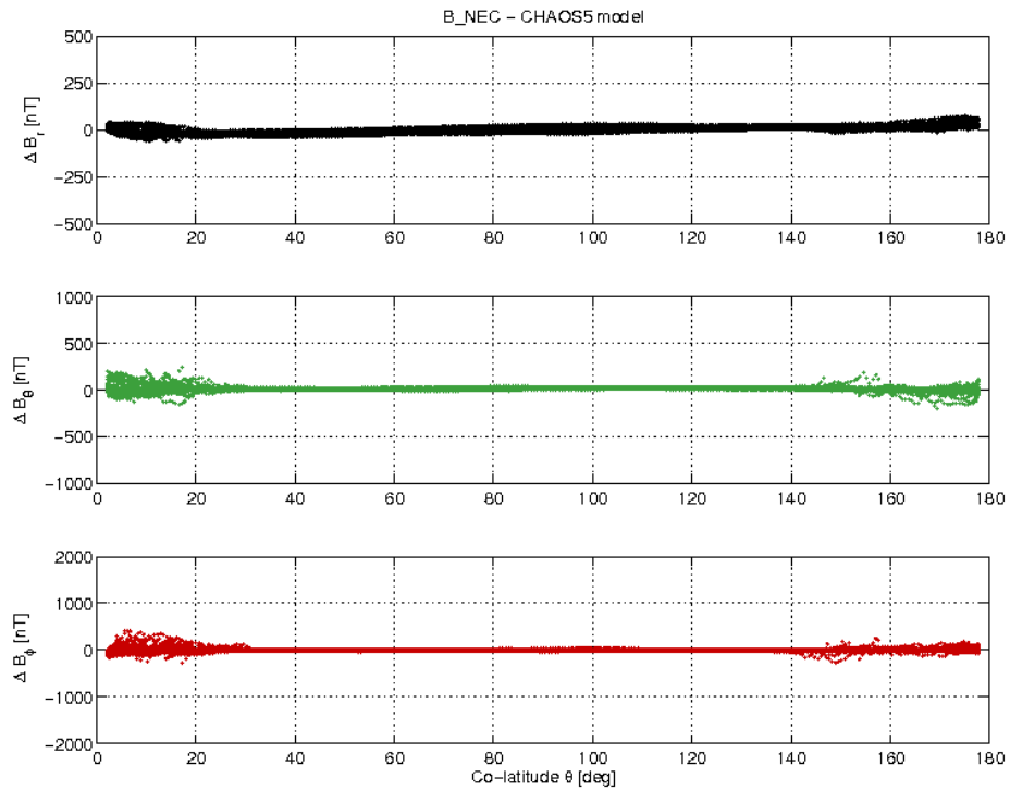
Figure 19: S/C B day 23/05 B_{NEC} - B_{Chaos} difference vs colatitude.
