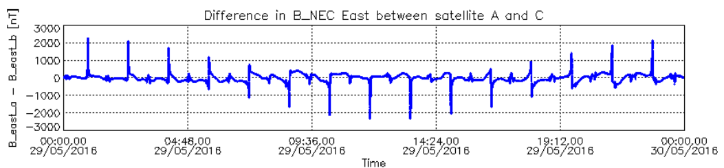
Figure 15 Difference in B_NEC East component between S/C A and S/C C on 29/05/2016.
