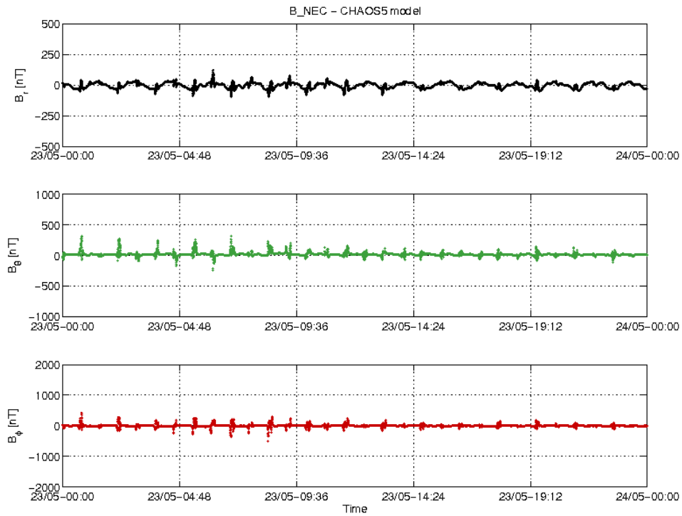
Figure 22 S/C C day 23/05 time series of B_{NEC} - B_{Chaos} residuals.
