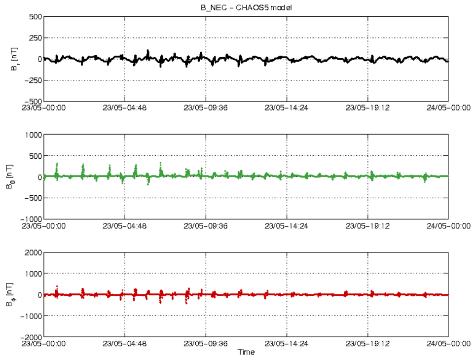
Figure 18: S/C A day 23/05: time series of B_{NEC} - B_{Chaos} residuals.
