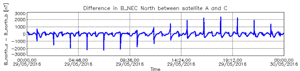
Figure 14 Difference in B_NEC North component between S/C A and S/C C on 29/05/2016.
